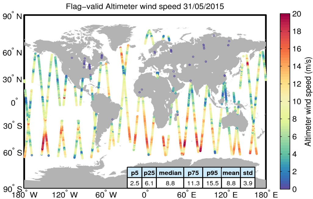
Figure 31. Geographical distribution of flag-valid wind data over oceans and lakes for 31/05/2015. The statistical values shown in the table refer to the wind in m/s and are calculated over all measurements shown in the figure.
