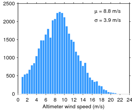
Figure 33. Histogram of flag-valid wind over oceans and lakes for 31/05/2015. The mean ( \mu ) and standard deviation ( \sigma ) are also shown. Note that values larger than 24 m/s are excluded from the histogram for the sake of readability but not from the computation of \mu and \sigma .
