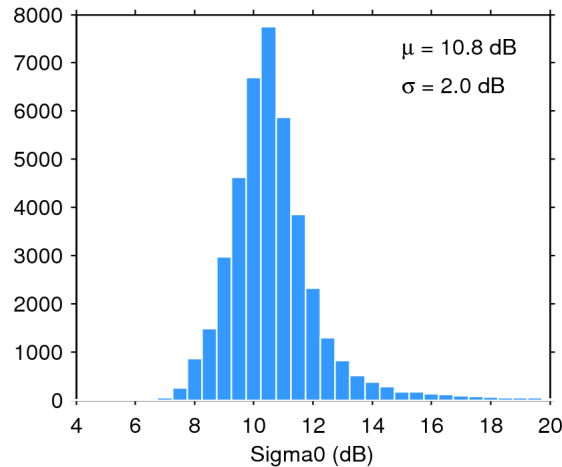
Figure 25. Histogram of flag-valid sigma0 over oceans and lakes for 31/05/2015. The mean ( \mu ) and standard deviation ( \sigma ) are also shown. Note that values outside [4 20] dB are excluded from the histogram for the sake of readability but not from the computation of \mu and \sigma .
