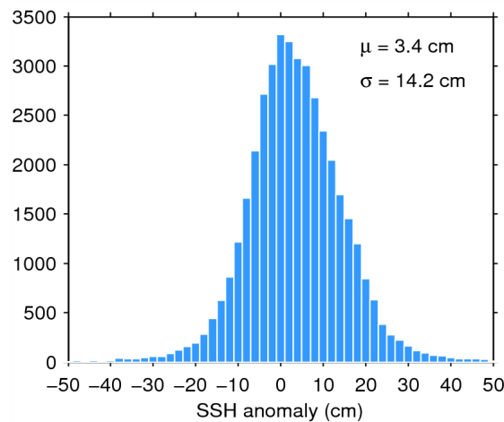
Figure 7. Histogram of flag-valid SSH anomaly over oceans and lakes for 31/05/2015. The mean ( \mu ) and standard deviation ( \sigma ) are also shown. Note that values outside [-50\ 50] cm are excluded from the histogram for the sake of readability but not from the computation of \mu and \sigma .
