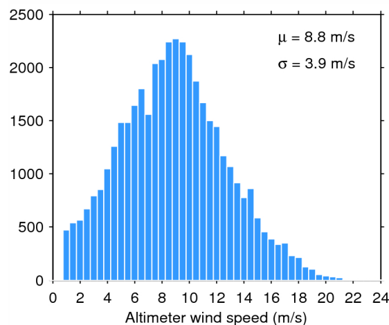
Figure 35. Histogram of science-valid wind over oceans and lakes for 31/05/2015. The mean ( \mu ) and standard deviation ( \sigma ) are also shown. Note that values larger than 24 m/s are excluded from the histogram for the sake of readability but not from the computation of \mu and \sigma .
