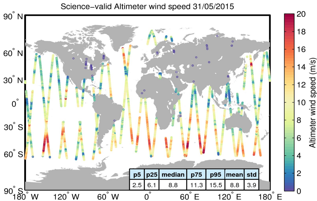
Figure 34. Geographical distribution of science-valid wind data over oceans and lakes for 31/05/2015. The statistical values shown in the table refer to the wind in m/s and are calculated over all measurements shown in the figure. Gray circles denote records that have been rejected based on the editing criteria described in Table 5.
