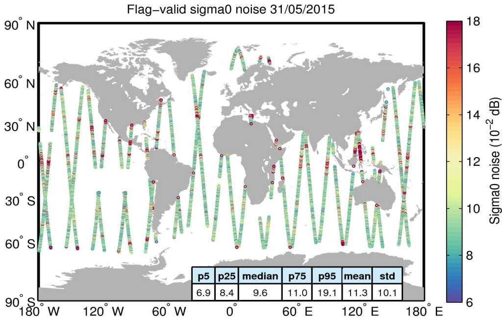
Figure 26. Geographical distribution of flag-valid 20-Hz sigma0 measurement noise over oceans and lakes for 31/05/2015. The statistical values shown in the table refer to the sigma0 noise and are calculated over all measurements shown in the figure.
