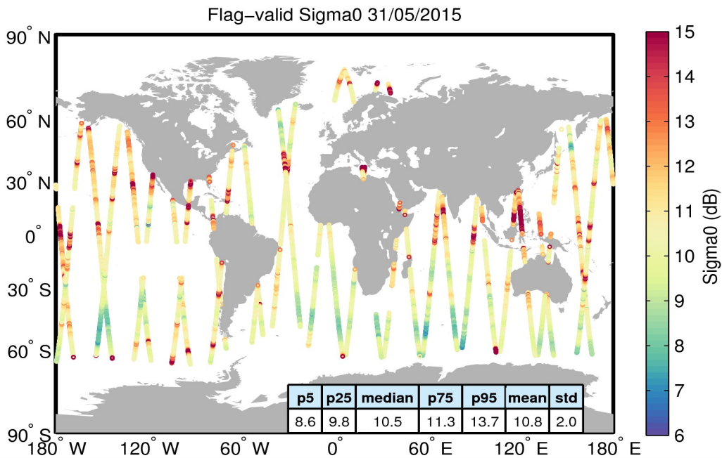
Figure 23. Geographical distribution of flag-valid sigma0 data over oceans and lakes for 31/05/2015. The statistical values shown in the table refer to the sigma0 in dB and are calculated over all measurements shown in the figure.
