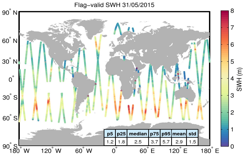
Figure 15. Geographical distribution of flag-valid SWH data over oceans and lakes for 31/05/2015. The statistical values shown in the table refer to the SWH in m and are calculated over all measurements shown in the figure.
