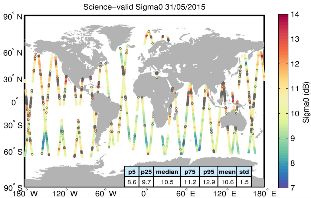
Figure 27. Geographical distribution of science-valid sigma0 data over oceans and lakes for 31/05/2015. The statistical values shown in the table refer to the sigma0 in dB and are calculated over all measurements shown in the figure. Gray circles denote records that have been rejected based on the editing criteria described in Table 4.
