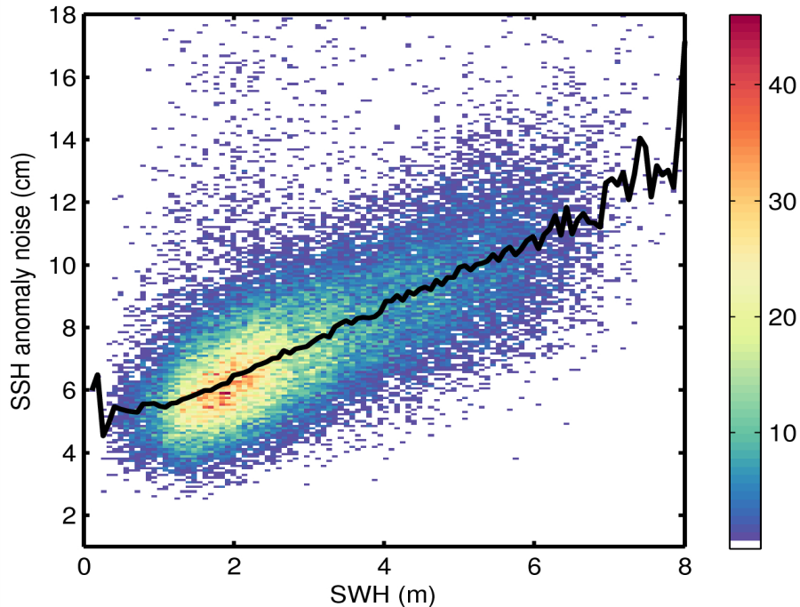
Figure 9. 2D histogram showing flag-valid SSH anomaly noise as a function of SWH for 31/05/2015. The black line denotes the median SSH anomaly as a function of SWH.
