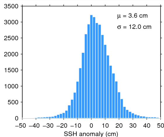
Figure 11. Histogram of science-valid SSH anomaly over oceans and lakes for 31/05/2015. The mean ( \mu ) and standard deviation ( \sigma ) are also shown. Note that values outside [-50 50] cm are excluded from the histogram for the sake of readability but not from the computation of \mu and \sigma .
