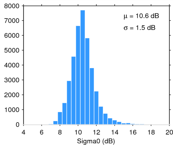
Figure 28. Histogram of science-valid sigma0 over oceans and lakes for 31/05/2015. The mean ( \mu ) and standard deviation ( \sigma ) are also shown. Note that values outside [4 20] dB are excluded from the histogram for the sake of readability but not from the computation of \mu and \sigma .
