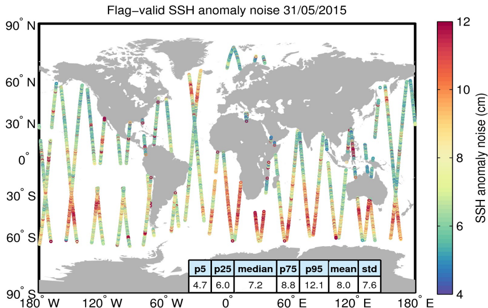
Figure 8. Geographical distribution of flag-valid 20-Hz SSH anomaly measurement noise over oceans and lakes for 31/05/2015. The statistical values shown in the table refer to the SSH anomaly noise and are calculated over all measurements shown in the figure.
