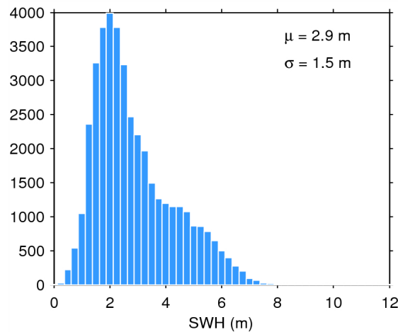
Figure 17. Histogram of flag-valid SWH over oceans and lakes for 31/05/2015. The mean ( \mu ) and standard deviation ( \sigma ) are also shown. Note that values larger than 12 m are excluded from the histogram for the sake of readability but not from the computation of \mu and \sigma .
