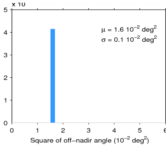
Figure 39. Histogram of flag-valid mispointing over oceans and lakes for 31/05/2015. The mean ( \mu ) and standard deviation ( \sigma ) are also shown. Note that values larger than 6 \times 10^{-2} \text{ deg}^2 are excluded from the histogram for the sake of readability but not from the computation of \mu and \sigma .
