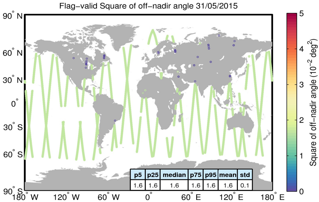
Figure 37. Geographical distribution of flag-valid mispointing data over oceans and lakes for 31/05/2015. The statistical values shown in the table refer to the mispointing in 10^{-2} \text{ deg}^2 and are calculated over all measurements shown in the figure.
