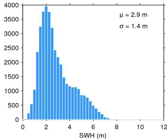
Figure 20. Histogram of science-valid SWH over oceans and lakes for 31/05/2015. The mean ( \mu ) and standard deviation ( \sigma ) are also shown. Note that values larger than 12 m are excluded from the histogram for the sake of readability but not from the computation of \mu and \sigma .
