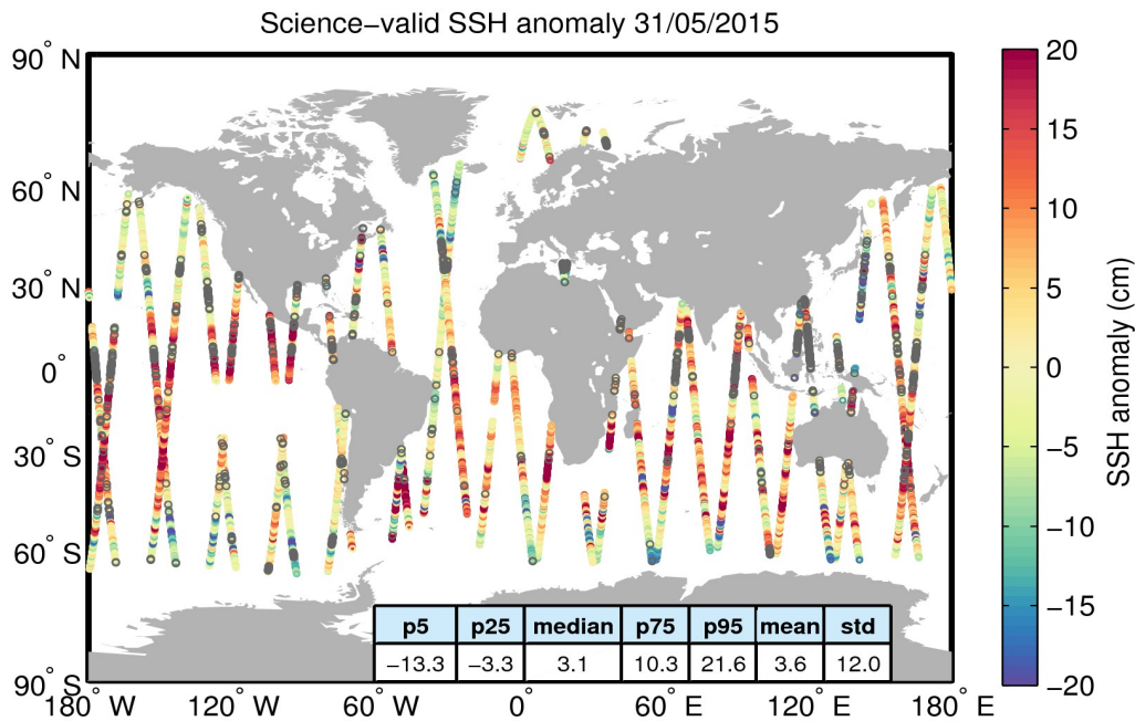
Figure 10. Geographical distribution of science-valid SSH anomaly data over oceans and lakes for 31/05/2015. The statistical values shown in the table refer to the SSH anomaly in cm and are calculated over all measurements shown in the figure. Gray circles denote records that have been rejected based on the editing criteria described in Table 2.
