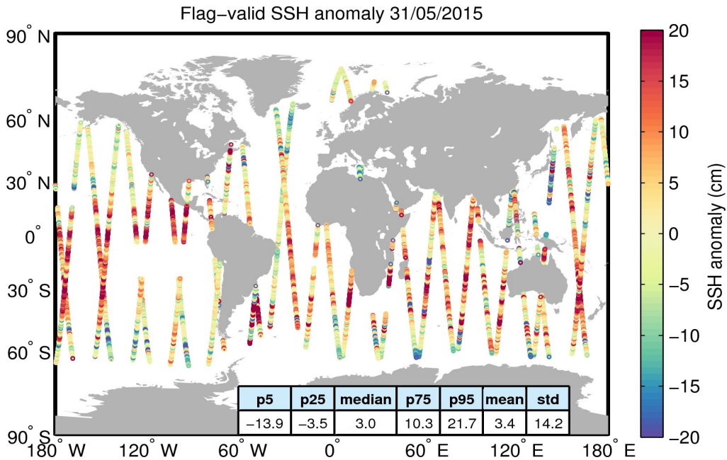
Figure 5. Geographical distribution of flag-valid 1-Hz SSH anomaly data over oceans and lakes for 31/05/2015. The statistical values shown in the table refer to the SSH anomaly in cm and are calculated over all measurements shown in the figure.
