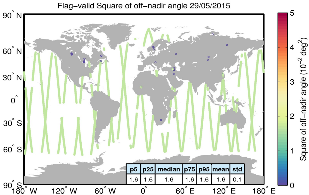
Figure 37. Geographical distribution of flag-valid mispointing data over oceans and lakes for 29/05/2015. The statistical values shown in the table refer to the mispointing in 10^{-2} \text{deg}^2 and are calculated over all measurements shown in the figure.
