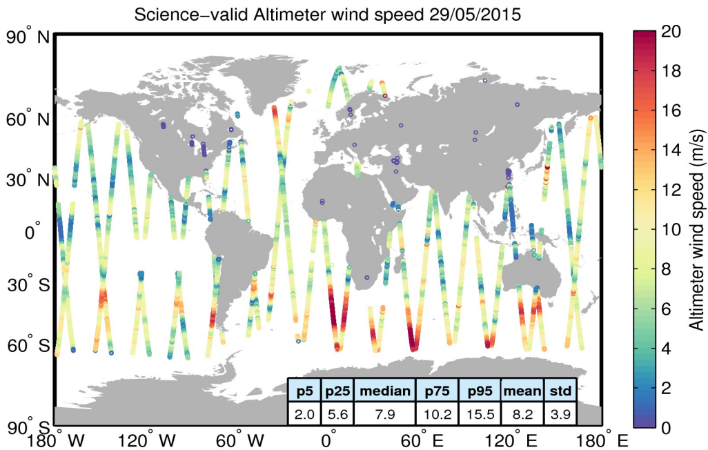
Figure 34. Geographical distribution of science-valid wind data over oceans and lakes for 29/05/2015. The statistical values shown in the table refer to the wind in m/s and are calculated over all measurements shown in the figure. Gray circles denote records that have been rejected based on the editing criteria described in Table 5.
