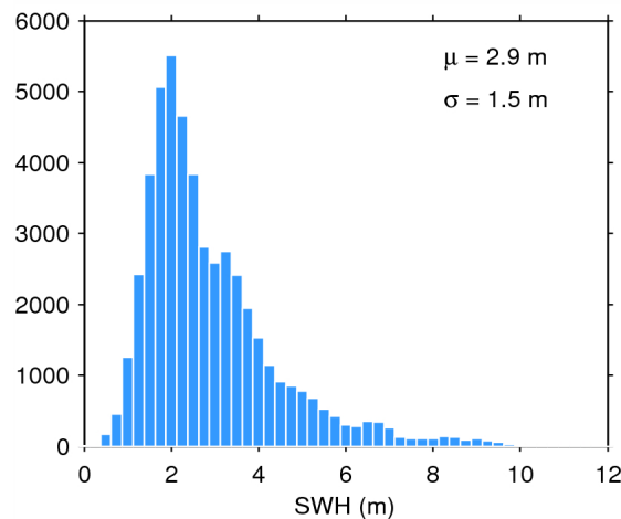
Figure 20. Histogram of science-valid SWH over oceans and lakes for 29/05/2015. The mean ( \mu ) and standard deviation ( \sigma ) are also shown. Note that values larger than 12 m are excluded from the histogram for the sake of readability but not from the computation of \mu and \sigma .
