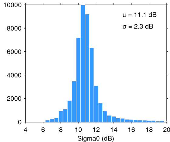
Figure 25. Histogram of flag-valid sigma0 over oceans and lakes for 29/05/2015. The mean ( \mu ) and standard deviation ( \sigma ) are also shown. Note that values outside [4 20] dB are excluded from the histogram for the sake of readability but not from the computation of \mu and \sigma .
