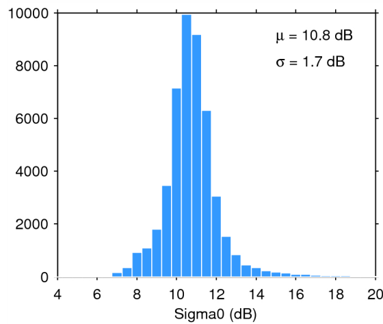
Figure 28. Histogram of science-valid sigma0 over oceans and lakes for 29/05/2015. The mean ( \mu ) and standard deviation ( \sigma ) are also shown. Note that values outside [4 20] dB are excluded from the histogram for the sake of readability but not from the computation of \mu and \sigma .
