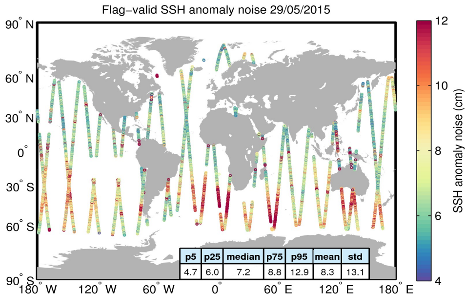
Figure 8. Geographical distribution of flag-valid 20-Hz SSH anomaly measurement noise over oceans and lakes for 29/05/2015. The statistical values shown in the table refer to the SSH anomaly noise and are calculated over all measurements shown in the figure.
