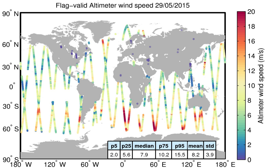
Figure 31. Geographical distribution of flag-valid wind data over oceans and lakes for 29/05/2015. The statistical values shown in the table refer to the wind in m/s and are calculated over all measurements shown in the figure.
