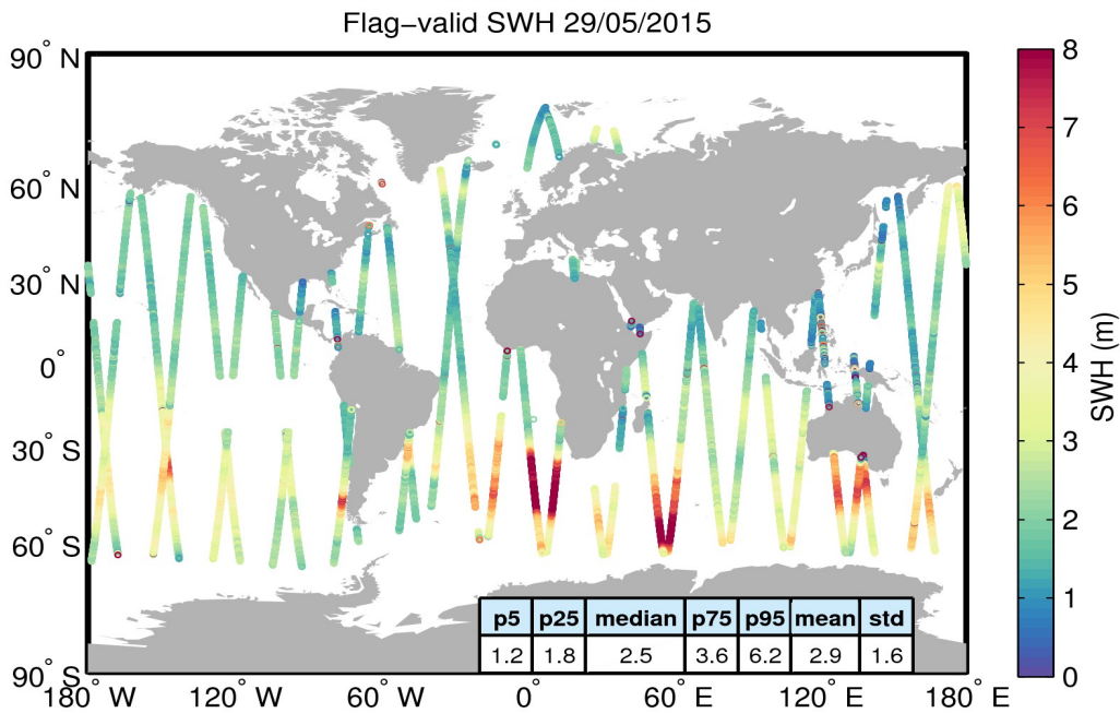
Figure 15. Geographical distribution of flag-valid SWH data over oceans and lakes for 29/05/2015. The statistical values shown in the table refer to the SWH in m and are calculated over all measurements shown in the figure.
