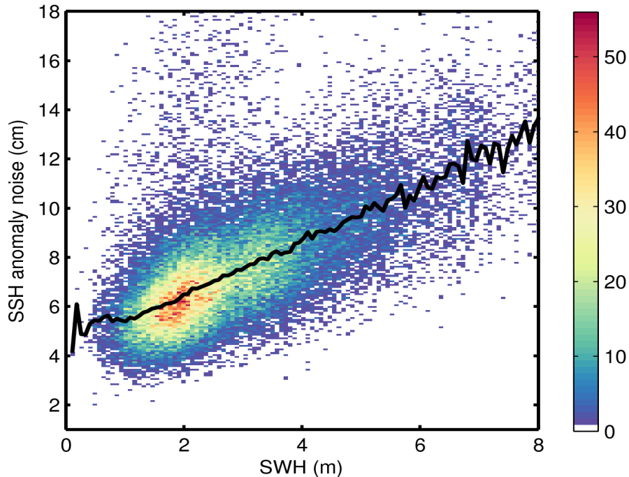
Figure 9. 2D histogram showing flag-valid SSH anomaly noise as a function of SWH for 29/05/2015. The black line denotes the median SSH anomaly as a function of SWH.
