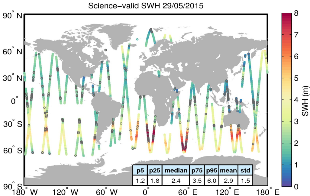
Figure 19. Geographical distribution of science-valid SWH data over oceans and lakes for 29/05/2015. The statistical values shown in the table refer to the SWH in m and are calculated over all measurements shown in the figure. Gray circles denote records that have been rejected based on the editing criteria described in Table 3.
