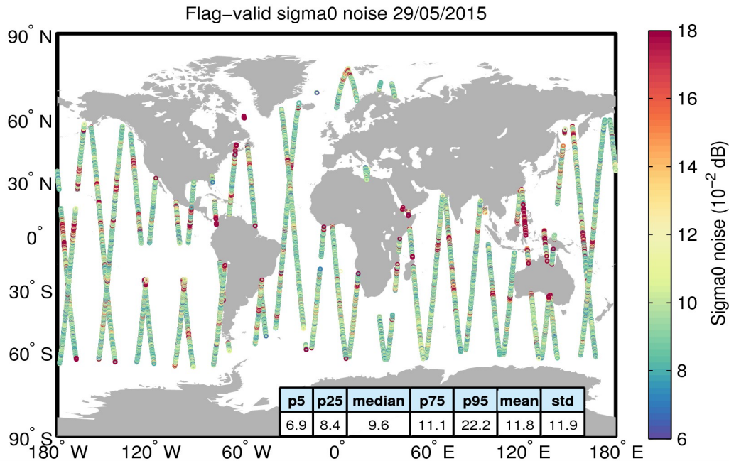
Figure 26. Geographical distribution of flag-valid 20-Hz sigma0 measurement noise over oceans and lakes for 29/05/2015. The statistical values shown in the table refer to the sigma0 noise and are calculated over all measurements shown in the figure.
