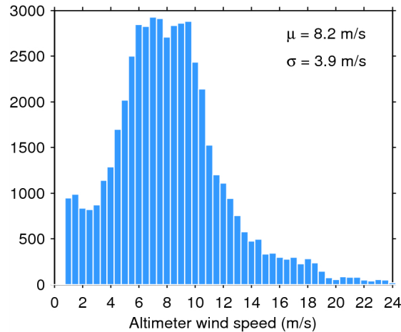
Figure 33. Histogram of flag-valid wind over oceans and lakes for 29/05/2015. The mean ( \mu ) and standard deviation ( \sigma ) are also shown. Note that values larger than 24 m/s are excluded from the histogram for the sake of readability but not from the computation of \mu and \sigma .
