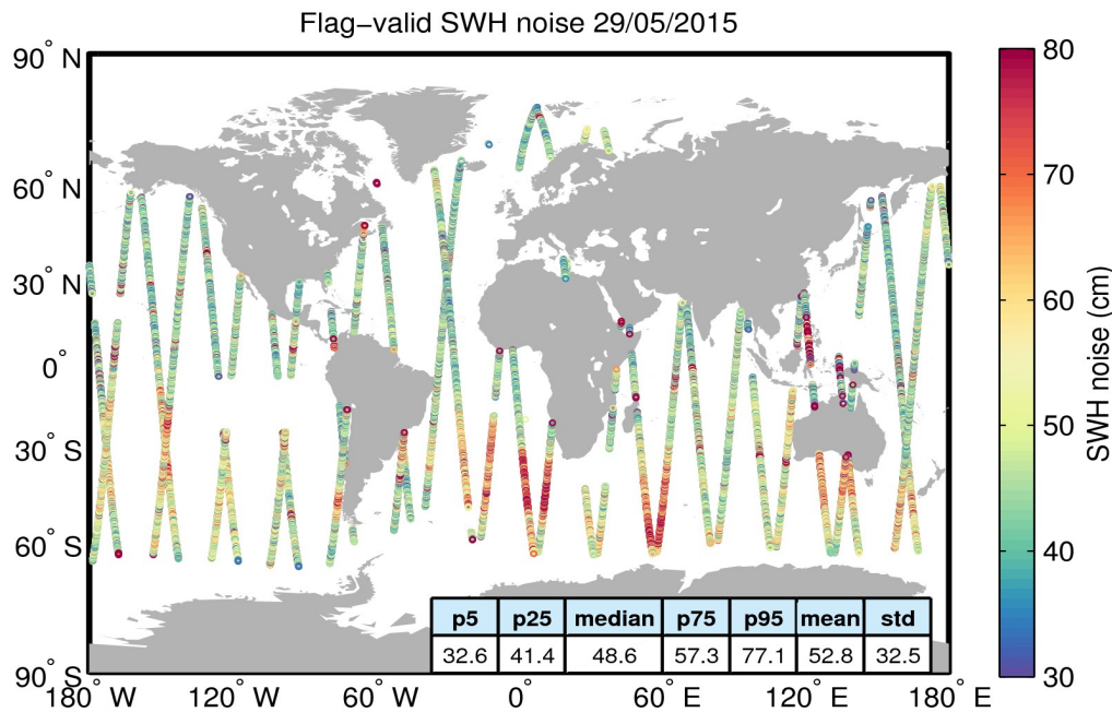
Figure 18. Geographical distribution of flag-valid 20-Hz SWH measurement noise over oceans and lakes for 29/05/2015. The statistical values shown in the figure refer to the SWH noise and are calculated over all measurements shown in the figure.
