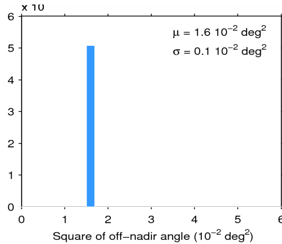
Figure 39. Histogram of flag-valid mispointing over oceans and lakes for 29/05/2015. The mean ( \mu ) and standard deviation ( \sigma ) are also shown. Note that values larger than 6 \cdot 10^{-2} \text{ deg}^2 are excluded from the histogram for the sake of readability but not from the computation of \mu and \sigma .
