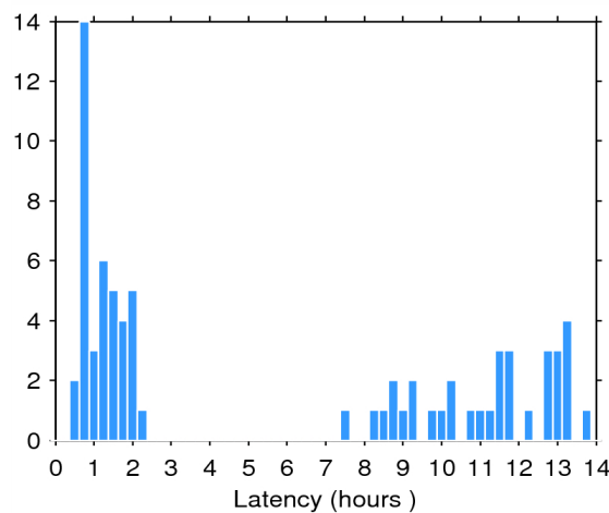
Figure 2. Histogram of the data latency for 28/05/2015. The y-axis denotes the number of files that are made available with a delay of x-hours with respect to the mean time of the records stored in the file.
