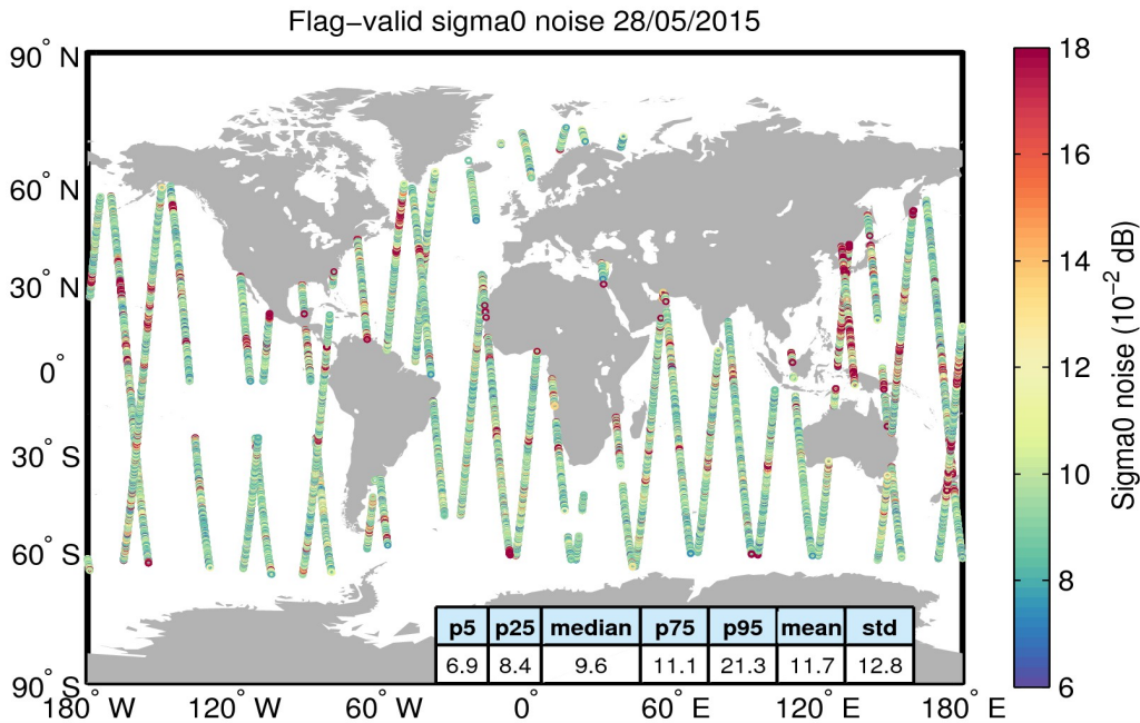
Figure 26. Geographical distribution of flag-valid 20-Hz sigma0 measurement noise over oceans and lakes for 28/05/2015. The statistical values shown in the table refer to the sigma0 noise and are calculated over all measurements shown in the figure.
