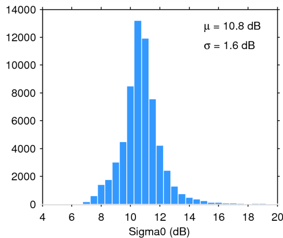
Figure 28. Histogram of science-valid sigma0 over oceans and lakes for 28/05/2015. The mean ( \mu ) and standard deviation ( \sigma ) are also shown. Note that values outside [4 20] dB are excluded from the histogram for the sake of readability but not from the computation of \mu and \sigma .
