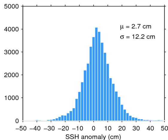
Figure 11. Histogram of science-valid SSH anomaly over oceans and lakes for 28/05/2015. The mean ( \mu ) and standard deviation ( \sigma ) are also shown. Note that values outside [-50 50] cm are excluded from the histogram for the sake of readability but not from the computation of \mu and \sigma .
