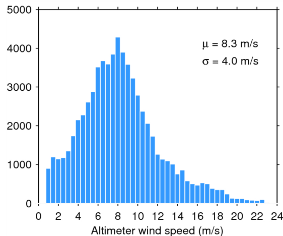
Figure 35. Histogram of science-valid wind over oceans and lakes for 28/05/2015. The mean ( \mu ) and standard deviation ( \sigma ) are also shown. Note that values larger than 24 m/s are excluded from the histogram for the sake of readability but not from the computation of \mu and \sigma .
