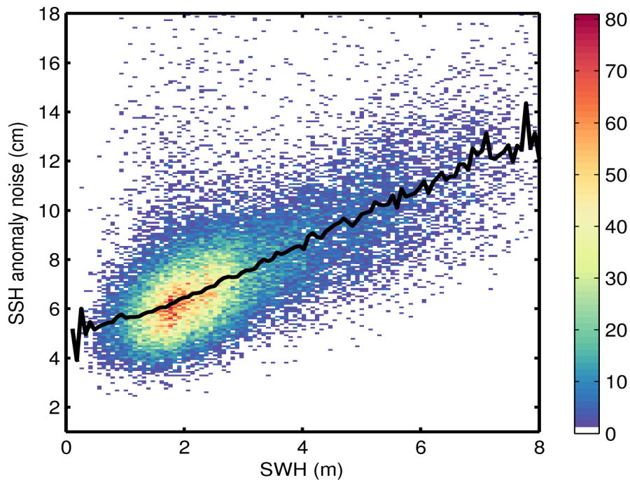
Figure 9. 2D histogram showing flag-valid SSH anomaly noise as a function of SWH for 28/05/2015. The black line denotes the median SSH anomaly as a function of SWH.
