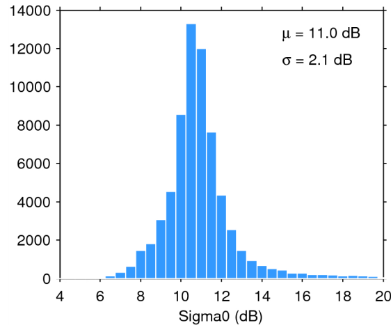
Figure 25. Histogram of flag-valid sigma0 over oceans and lakes for 28/05/2015. The mean ( \mu ) and standard deviation ( \sigma ) are also shown. Note that values outside [4 20] dB are excluded from the histogram for the sake of readability but not from the computation of \mu and \sigma .
