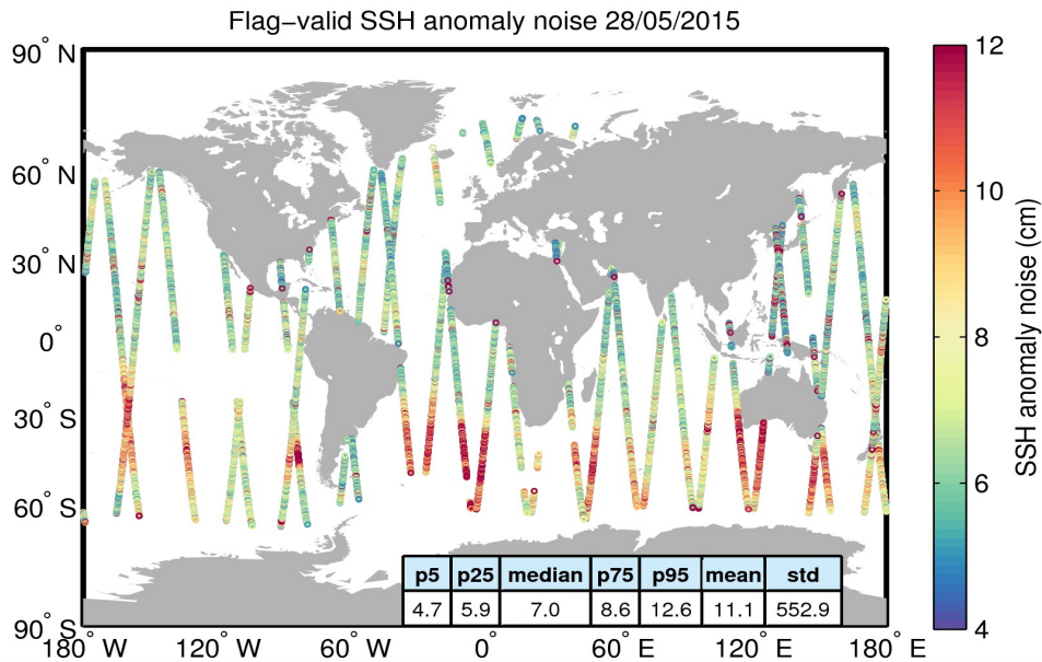
Figure 8. Geographical distribution of flag-valid 20-Hz SSH anomaly measurement noise over oceans and lakes for 28/05/2015. The statistical values shown in the table refer to the SSH anomaly noise and are calculated over all measurements shown in the figure.
