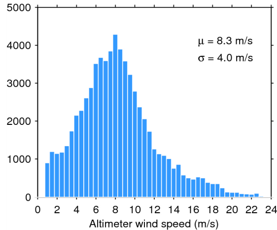
Figure 33. Histogram of flag-valid wind over oceans and lakes for 28/05/2015. The mean ( \mu ) and standard deviation ( \sigma ) are also shown. Note that values larger than 24 m/s are excluded from the histogram for the sake of readability but not from the computation of \mu and \sigma .
