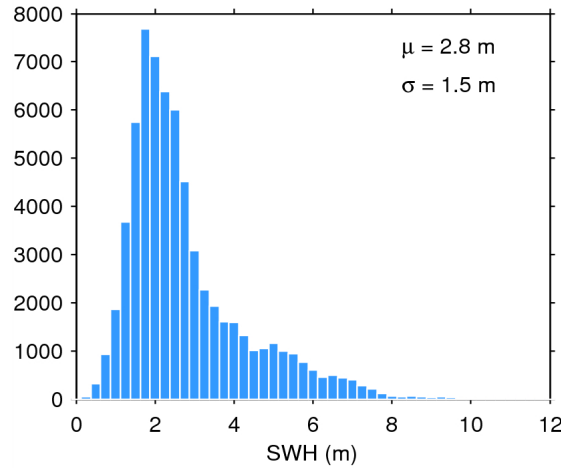
Figure 20. Histogram of science-valid SWH over oceans and lakes for 28/05/2015. The mean ( \mu ) and standard deviation ( \sigma ) are also shown. Note that values larger than 12 m are excluded from the histogram for the sake of readability but not from the computation of \mu and \sigma .
