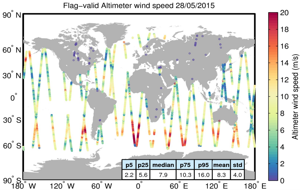
Figure 31. Geographical distribution of flag-valid wind data over oceans and lakes for 28/05/2015. The statistical values shown in the table refer to the wind in m/s and are calculated over all measurements shown in the figure.
