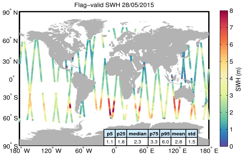
Figure 15. Geographical distribution of flag-valid SWH data over oceans and lakes for 28/05/2015. The statistical values shown in the table refer to the SWH in m and are calculated over all measurements shown in the figure.
