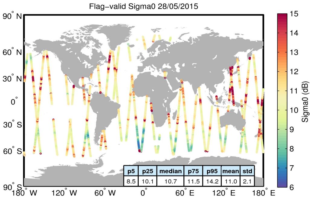
Figure 23. Geographical distribution of flag-valid sigma0 data over oceans and lakes for 28/05/2015. The statistical values shown in the table refer to the sigma0 in dB and are calculated over all measurements shown in the figure.
