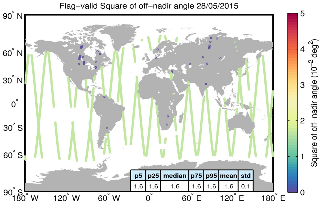
Figure 37. Geographical distribution of flag-valid mispointing data over oceans and lakes for 28/05/2015. The statistical values shown in the table refer to the mispointing in 10^{-2} \text{ deg}^2 and are calculated over all measurements shown in the figure.
