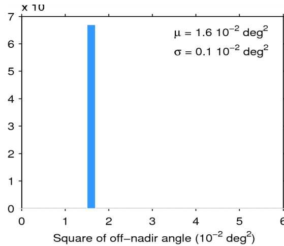
Figure 39. Histogram of flag-valid mispointing over oceans and lakes for 28/05/2015. The mean ( \mu ) and standard deviation ( \sigma ) are also shown. Note that values larger than 6 \cdot 10^{-2} \text{ deg}^2 are excluded from the histogram for the sake of readability but not from the computation of \mu and \sigma .
