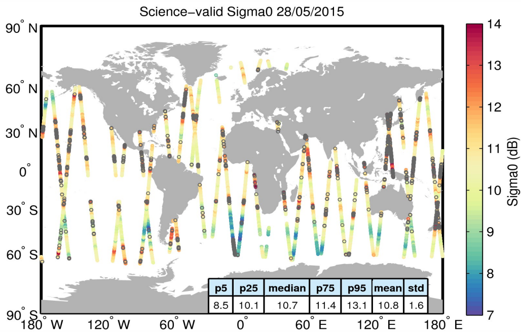
Figure 27. Geographical distribution of science-valid sigma0 data over oceans and lakes for 28/05/2015. The statistical values shown in the table refer to the sigma0 in dB and are calculated over all measurements shown in the figure. Gray circles denote records that have been rejected based on the editing criteria described in Table 4.
