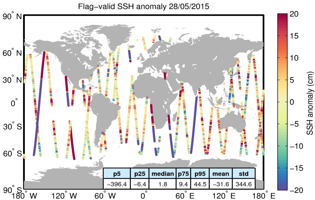
Figure 5. Geographical distribution of flag-valid 1-Hz SSH anomaly data over oceans and lakes for 28/05/2015. The statistical values shown in the table refer to the SSH anomaly in cm and are calculated over all measurements shown in the figure.
