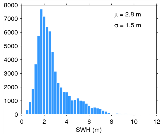
Figure 17. Histogram of flag-valid SWH over oceans and lakes for 28/05/2015. The mean ( \mu ) and standard deviation ( \sigma ) are also shown. Note that values larger than 12 m are excluded from the histogram for the sake of readability but not from the computation of \mu and \sigma .
