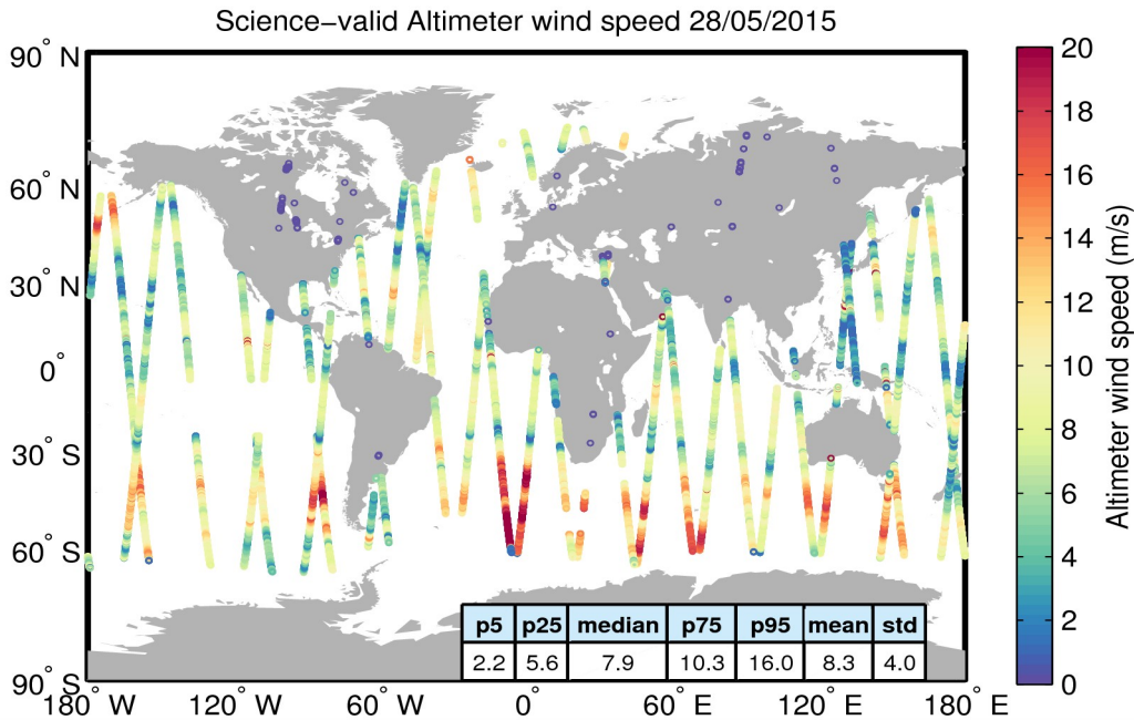
Figure 34. Geographical distribution of science-valid wind data over oceans and lakes for 28/05/2015. The statistical values shown in the table refer to the wind in m/s and are calculated over all measurements shown in the figure. Gray circles denote records that have been rejected based on the editing criteria described in Table 5.
