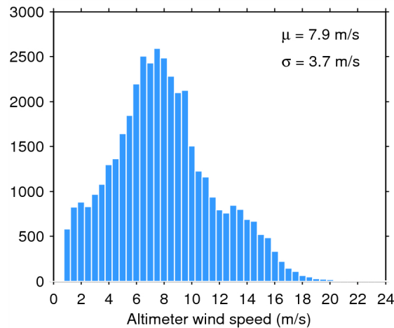
Figure 33. Histogram of flag-valid wind over oceans and lakes for 27/05/2015. The mean ( \mu ) and standard deviation ( \sigma ) are also shown. Note that values larger than 24 m/s are excluded from the histogram for the sake of readability but not from the computation of \mu and \sigma .
