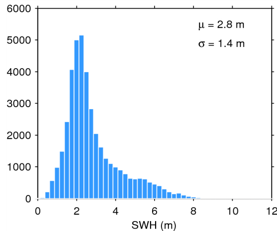
Figure 20. Histogram of science-valid SWH over oceans and lakes for 27/05/2015. The mean ( \mu ) and standard deviation ( \sigma ) are also shown. Note that values larger than 12 m are excluded from the histogram for the sake of readability but not from the computation of \mu and \sigma .
