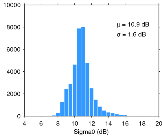
Figure 28. Histogram of science-valid sigma0 over oceans and lakes for 27/05/2015. The mean ( \mu ) and standard deviation ( \sigma ) are also shown. Note that values outside [4 20] dB are excluded from the histogram for the sake of readability but not from the computation of \mu and \sigma .
