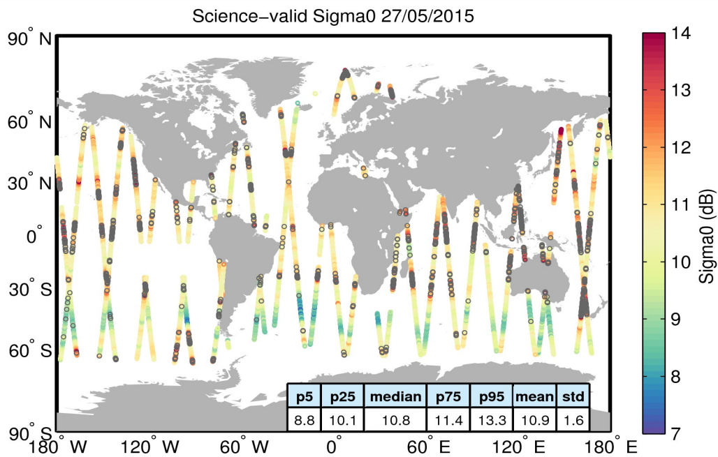
Figure 27. Geographical distribution of science-valid sigma0 data over oceans and lakes for 27/05/2015. The statistical values shown in the table refer to the sigma0 in dB and are calculated over all measurements shown in the figure. Gray circles denote records that have been rejected based on the editing criteria described in Table 4.
