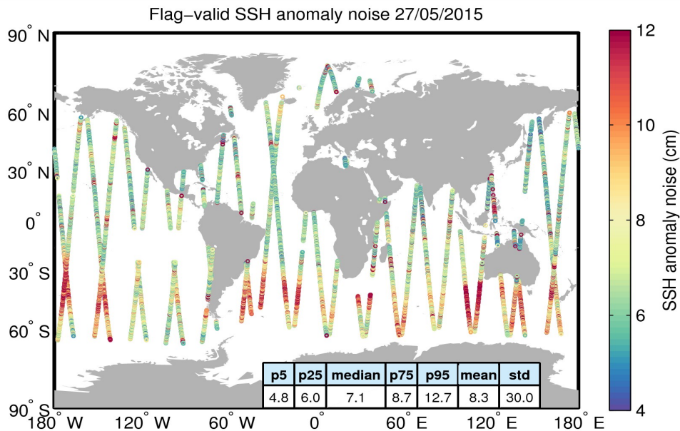
Figure 8. Geographical distribution of flag-valid 20-Hz SSH anomaly measurement noise over oceans and lakes for 27/05/2015. The statistical values shown in the table refer to the SSH anomaly noise and are calculated over all measurements shown in the figure.
