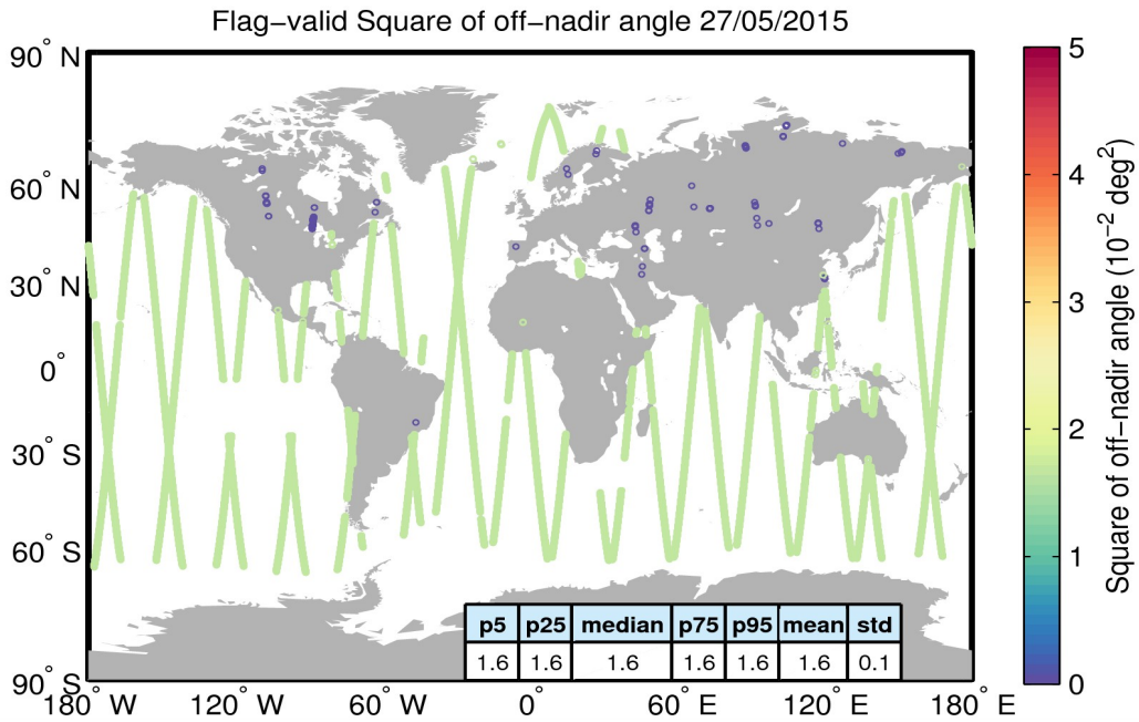
Figure 37. Geographical distribution of flag-valid mispointing data over oceans and lakes for 27/05/2015. The statistical values shown in the table refer to the mispointing in 10^{-2} \text{ deg}^2 and are calculated over all measurements shown in the figure.
