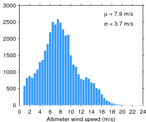
Figure 35. Histogram of science-valid wind over oceans and lakes for 27/05/2015. The mean ( \mu ) and standard deviation ( \sigma ) are also shown. Note that values larger than 24 m/s are excluded from the histogram for the sake of readability but not from the computation of \mu and \sigma .
