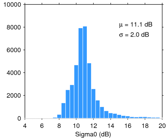
Figure 25. Histogram of flag-valid sigma0 over oceans and lakes for 27/05/2015. The mean ( \mu ) and standard deviation ( \sigma ) are also shown. Note that values outside [4 20] dB are excluded from the histogram for the sake of readability but not from the computation of \mu and \sigma .
