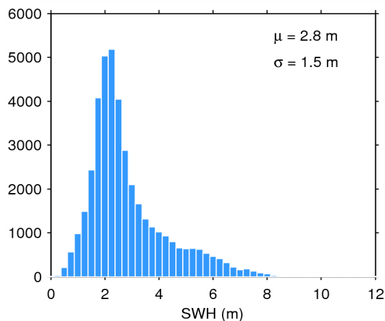
Figure 17. Histogram of flag-valid SWH over oceans and lakes for 27/05/2015. The mean ( \mu ) and standard deviation ( \sigma ) are also shown. Note that values larger than 12 m are excluded from the histogram for the sake of readability but not from the computation of \mu and \sigma .
