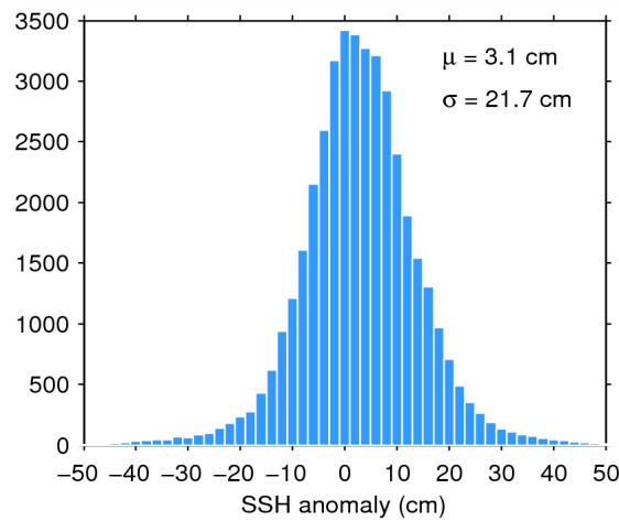
Figure 7. Histogram of flag-valid SSH anomaly over oceans and lakes for 27/05/2015. The mean ( \mu ) and standard deviation ( \sigma ) are also shown. Note that values outside [-50\ 50] cm are excluded from the histogram for the sake of readability but not from the computation of \mu and \sigma .
