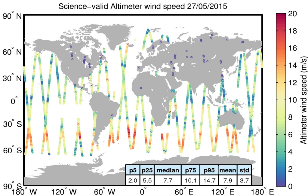
Figure 34. Geographical distribution of science-valid wind data over oceans and lakes for 27/05/2015. The statistical values shown in the table refer to the wind in m/s and are calculated over all measurements shown in the figure. Gray circles denote records that have been rejected based on the editing criteria described in Table 5.
