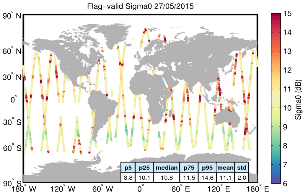
Figure 23. Geographical distribution of flag-valid sigma0 data over oceans and lakes for 27/05/2015. The statistical values shown in the table refer to the sigma0 in dB and are calculated over all measurements shown in the figure.
