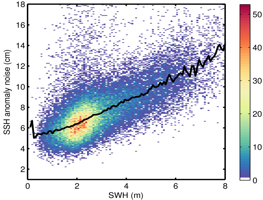
Figure 9. 2D histogram showing flag-valid SSH anomaly noise as a function of SWH for 27/05/2015. The black line denotes the median SSH anomaly as a function of SWH.
