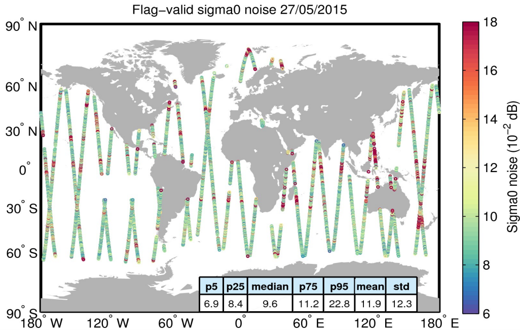
Figure 26. Geographical distribution of flag-valid 20-Hz sigma0 measurement noise over oceans and lakes for 27/05/2015. The statistical values shown in the table refer to the sigma0 noise and are calculated over all measurements shown in the figure.
