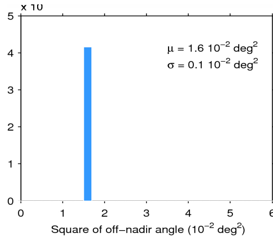
Figure 39. Histogram of flag-valid mispointing over oceans and lakes for 27/05/2015. The mean ( \mu ) and standard deviation ( \sigma ) are also shown. Note that values larger than 6 \cdot 10^{-2} \text{ deg}^2 are excluded from the histogram for the sake of readability but not from the computation of \mu and \sigma .
