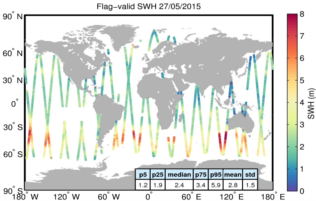
Figure 15. Geographical distribution of flag-valid SWH data over oceans and lakes for 27/05/2015. The statistical values shown in the table refer to the SWH in m and are calculated over all measurements shown in the figure.
