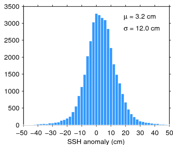
Figure 11. Histogram of science-valid SSH anomaly over oceans and lakes for 27/05/2015. The mean ( \mu ) and standard deviation ( \sigma ) are also shown. Note that values outside [-50 50] cm are excluded from the histogram for the sake of readability but not from the computation of \mu and \sigma .
