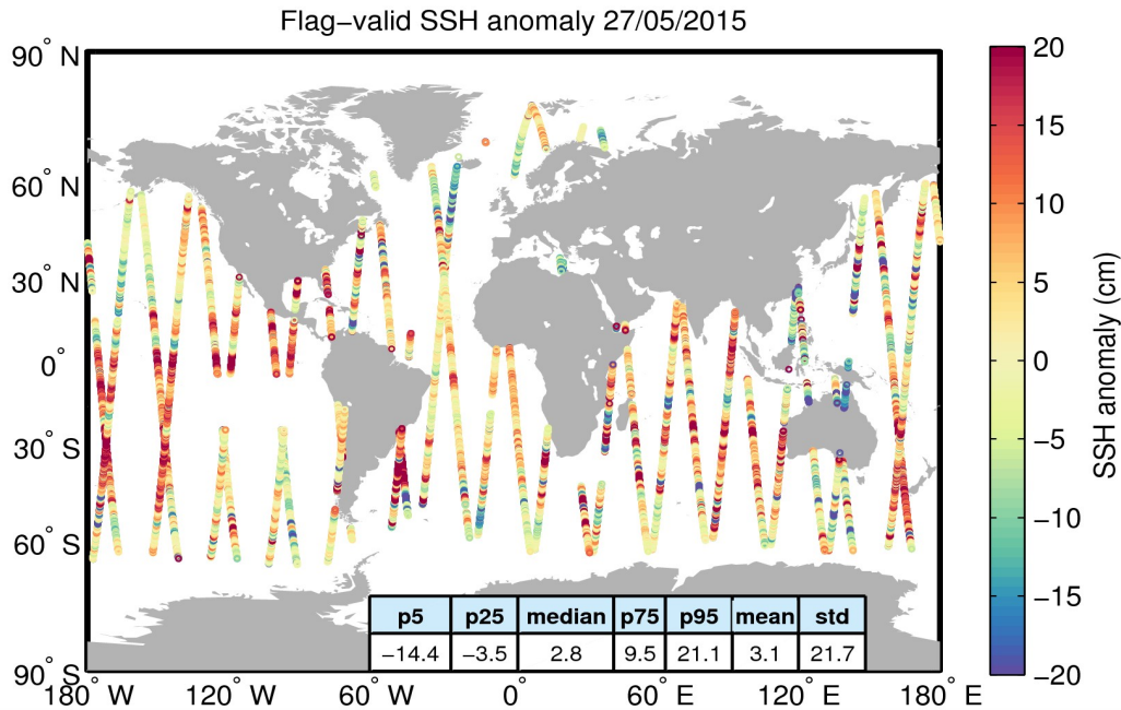
Figure 5. Geographical distribution of flag-valid 1-Hz SSH anomaly data over oceans and lakes for 27/05/2015. The statistical values shown in the table refer to the SSH anomaly in cm and are calculated over all measurements shown in the figure.
