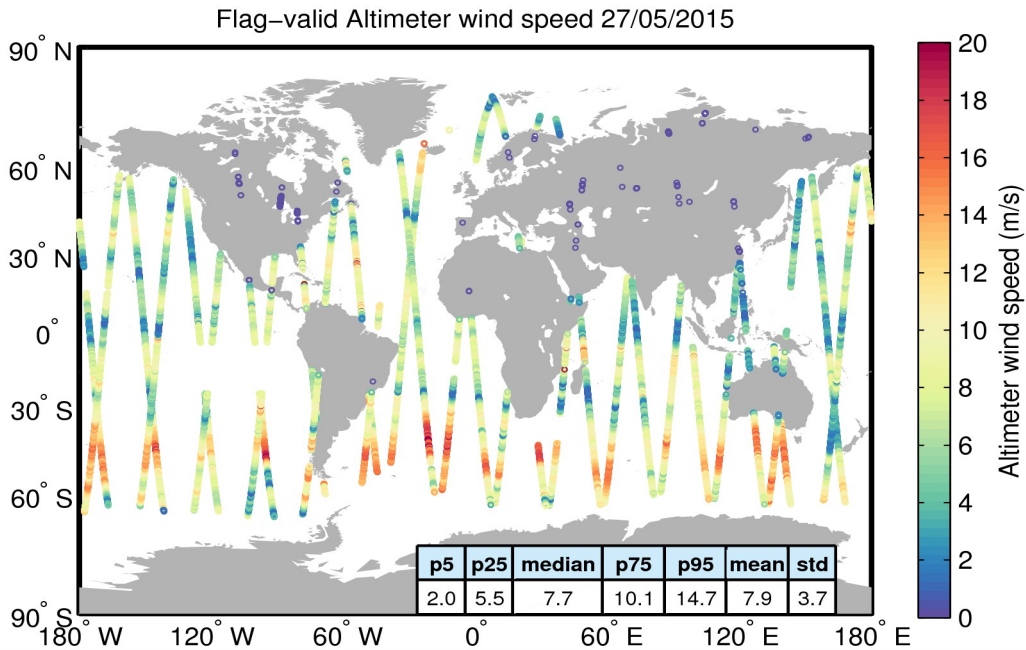
Figure 31. Geographical distribution of flag-valid wind data over oceans and lakes for 27/05/2015. The statistical values shown in the table refer to the wind in m/s and are calculated over all measurements shown in the figure.
