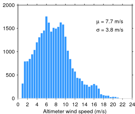
Figure 35. Histogram of science-valid wind over oceans and lakes for 26/05/2015. The mean ( \mu ) and standard deviation ( \sigma ) are also shown. Note that values larger than 24 m/s are excluded from the histogram for the sake of readability but not from the computation of \mu and \sigma .
