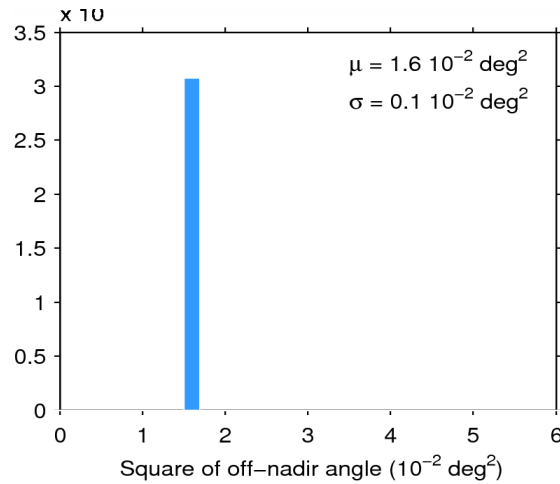
Figure 39. Histogram of flag-valid mispointing over oceans and lakes for 26/05/2015. The mean ( \mu ) and standard deviation ( \sigma ) are also shown. Note that values larger than 6 \cdot 10^{-2} \text{ deg}^2 are excluded from the histogram for the sake of readability but not from the computation of \mu and \sigma .
