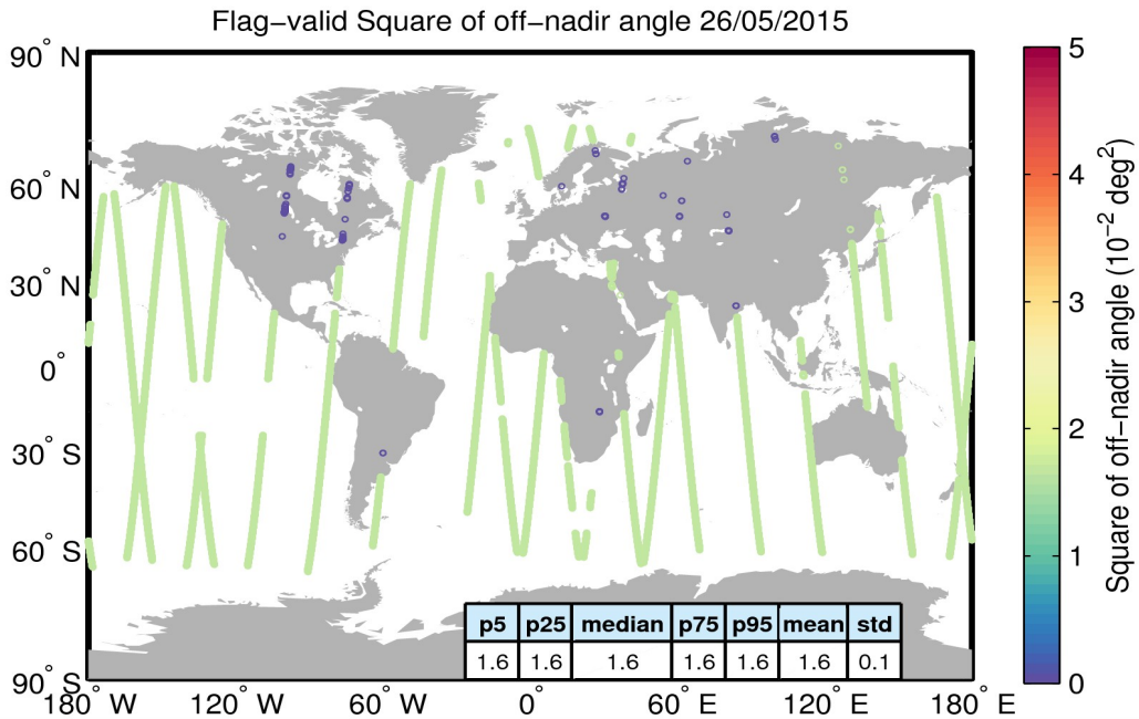
Figure 37. Geographical distribution of flag-valid mispointing data over oceans and lakes for 26/05/2015. The statistical values shown in the table refer to the mispointing in 10^{-2} deg 2 and are calculated over all measurements shown in the figure.
