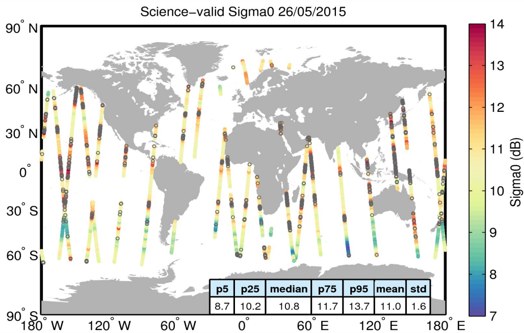
Figure 27. Geographical distribution of science-valid sigma0 data over oceans and lakes for 26/05/2015. The statistical values shown in the table refer to the sigma0 in dB and are calculated over all measurements shown in the figure. Gray circles denote records that have been rejected based on the editing criteria described in Table 4.
