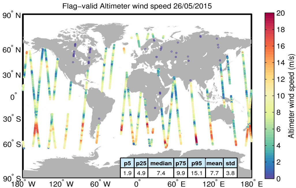
Figure 31. Geographical distribution of flag-valid wind data over oceans and lakes for 26/05/2015. The statistical values shown in the table refer to the wind in m/s and are calculated over all measurements shown in the figure.
