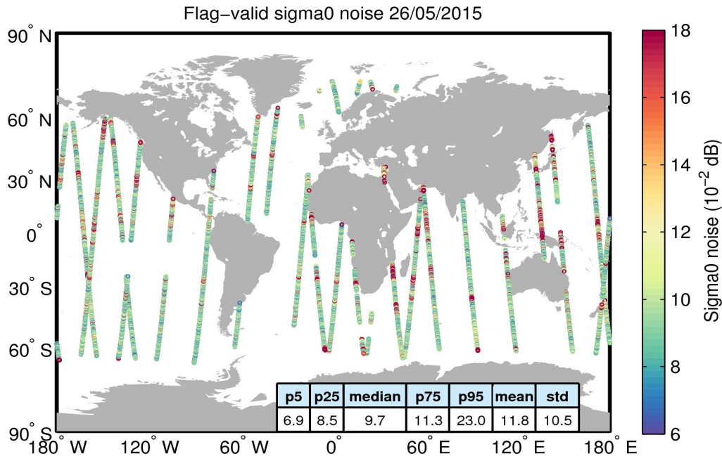
Figure 26. Geographical distribution of flag-valid 20-Hz sigma0 measurement noise over oceans and lakes for 26/05/2015. The statistical values shown in the table refer to the sigma0 noise and are calculated over all measurements shown in the figure.
