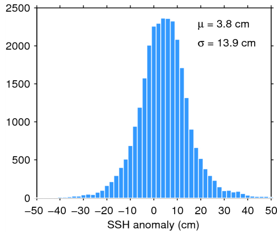
Figure 11. Histogram of science-valid SSH anomaly over oceans and lakes for 26/05/2015. The mean ( \mu ) and standard deviation ( \sigma ) are also shown. Note that values outside [-50 50] cm are excluded from the histogram for the sake of readability but not from the computation of \mu and \sigma .
