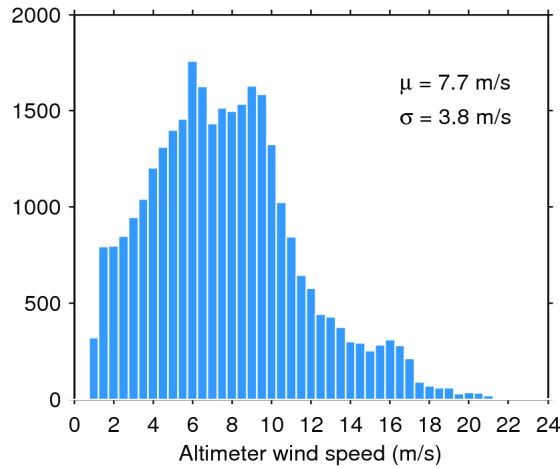
Figure 33. Histogram of flag-valid wind over oceans and lakes for 26/05/2015. The mean ( \mu ) and standard deviation ( \sigma ) are also shown. Note that values larger than 24 m/s are excluded from the histogram for the sake of readability but not from the computation of \mu and \sigma .
