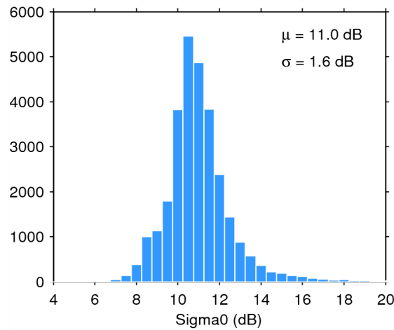
Figure 28. Histogram of science-valid sigma0 over oceans and lakes for 26/05/2015. The mean ( \mu ) and standard deviation ( \sigma ) are also shown. Note that values outside [4 20] dB are excluded from the histogram for the sake of readability but not from the computation of \mu and \sigma .
