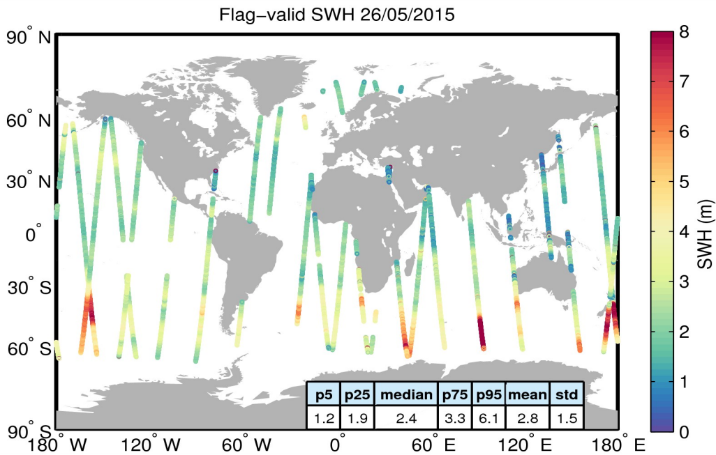
Figure 15. Geographical distribution of flag-valid SWH data over oceans and lakes for 26/05/2015. The statistical values shown in the table refer to the SWH in m and are calculated over all measurements shown in the figure.
