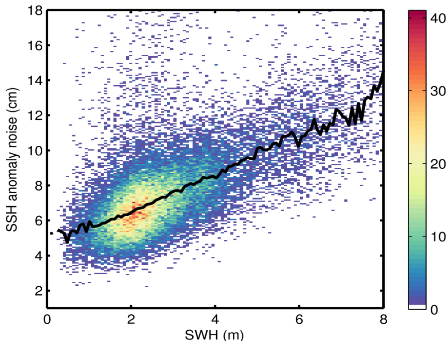
Figure 9. 2D histogram showing flag-valid SSH anomaly noise as a function of SWH for 26/05/2015. The black line denotes the median SSH anomaly as a function of SWH.
