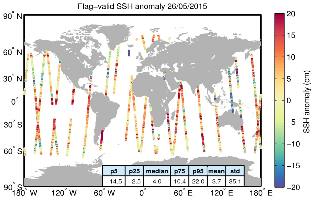
Figure 5. Geographical distribution of flag-valid 1-Hz SSH anomaly data over oceans and lakes for 26/05/2015. The statistical values shown in the table refer to the SSH anomaly in cm and are calculated over all measurements shown in the figure.
