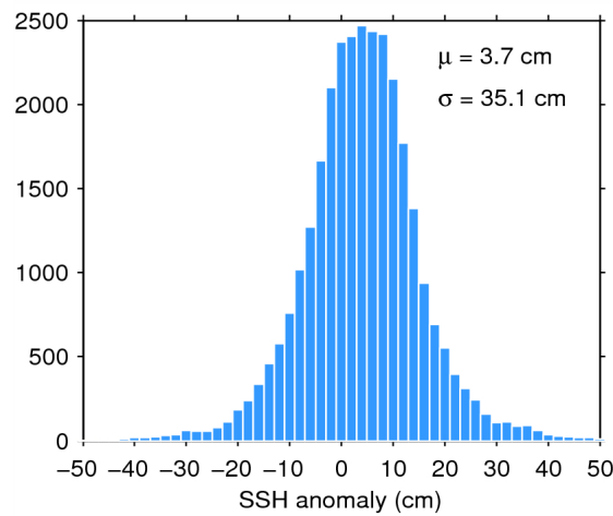
Figure 7. Histogram of flag-valid SSH anomaly over oceans and lakes for 26/05/2015. The mean ( \mu ) and standard deviation ( \sigma ) are also shown. Note that values outside [-50\ 50] cm are excluded from the histogram for the sake of readability but not from the computation of \mu and \sigma .
