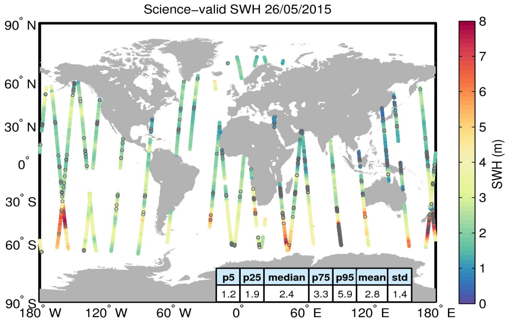
Figure 19. Geographical distribution of science-valid SWH data over oceans and lakes for 26/05/2015. The statistical values shown in the table refer to the SWH in m and are calculated over all measurements shown in the figure. Gray circles denote records that have been rejected based on the editing criteria described in Table 3.
