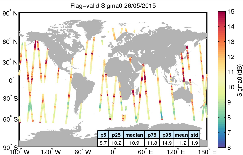
Figure 23. Geographical distribution of flag-valid sigma0 data over oceans and lakes for 26/05/2015. The statistical values shown in the table refer to the sigma0 in dB and are calculated over all measurements shown in the figure.
