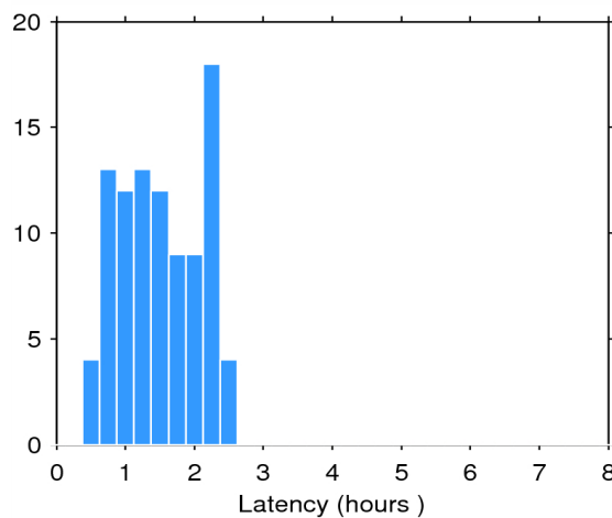
Figure 2. Histogram of the data latency for 26/05/2015. The y-axis denotes the number of files that are made available with a delay of x-hours with respect to the mean time of the records stored in the file.
