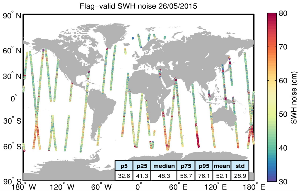
Figure 18. Geographical distribution of flag-valid 20-Hz SWH measurement noise over oceans and lakes for 26/05/2015. The statistical values shown in the figure refer to the SWH noise and are calculated over all measurements shown in the figure.
