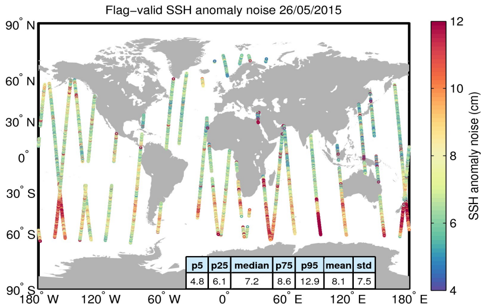
Figure 8. Geographical distribution of flag-valid 20-Hz SSH anomaly measurement noise over oceans and lakes for 26/05/2015. The statistical values shown in the table refer to the SSH anomaly noise and are calculated over all measurements shown in the figure.
