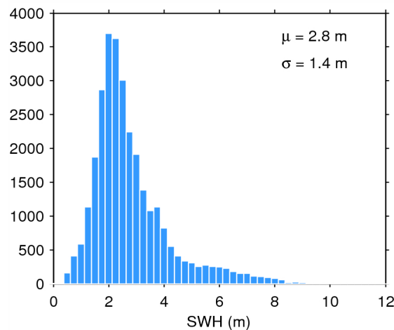
Figure 20. Histogram of science-valid SWH over oceans and lakes for 26/05/2015. The mean ( \mu ) and standard deviation ( \sigma ) are also shown. Note that values larger than 12 m are excluded from the histogram for the sake of readability but not from the computation of \mu and \sigma .
