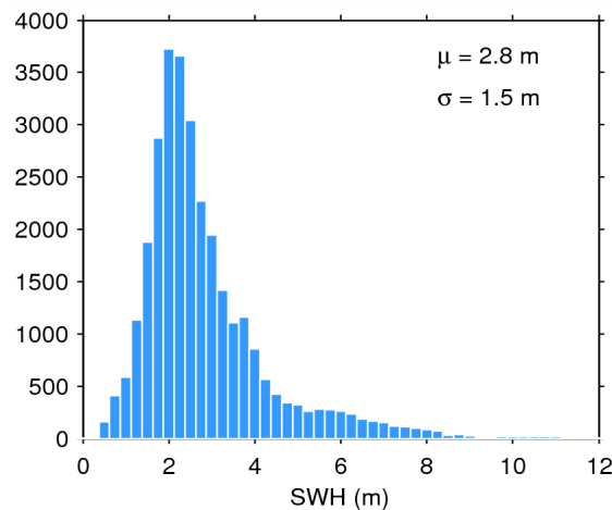
Figure 17. Histogram of flag-valid SWH over oceans and lakes for 26/05/2015. The mean ( \mu ) and standard deviation ( \sigma ) are also shown. Note that values larger than 12 m are excluded from the histogram for the sake of readability but not from the computation of \mu and \sigma .
