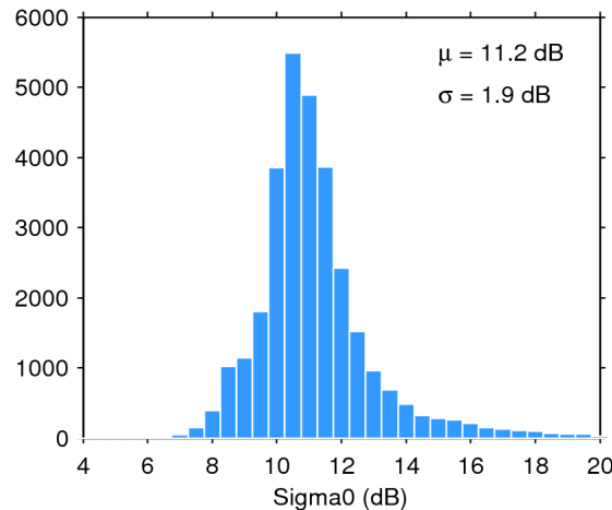
Figure 25. Histogram of flag-valid sigma0 over oceans and lakes for 26/05/2015. The mean ( \mu ) and standard deviation ( \sigma ) are also shown. Note that values outside [4 20] dB are excluded from the histogram for the sake of readability but not from the computation of \mu and \sigma .
