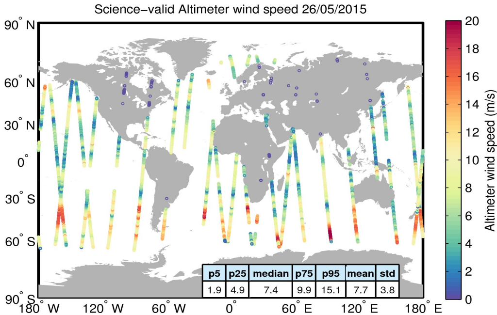
Figure 34. Geographical distribution of science-valid wind data over oceans and lakes for 26/05/2015. The statistical values shown in the table refer to the wind in m/s and are calculated over all measurements shown in the figure. Gray circles denote records that have been rejected based on the editing criteria described in Table 5.
