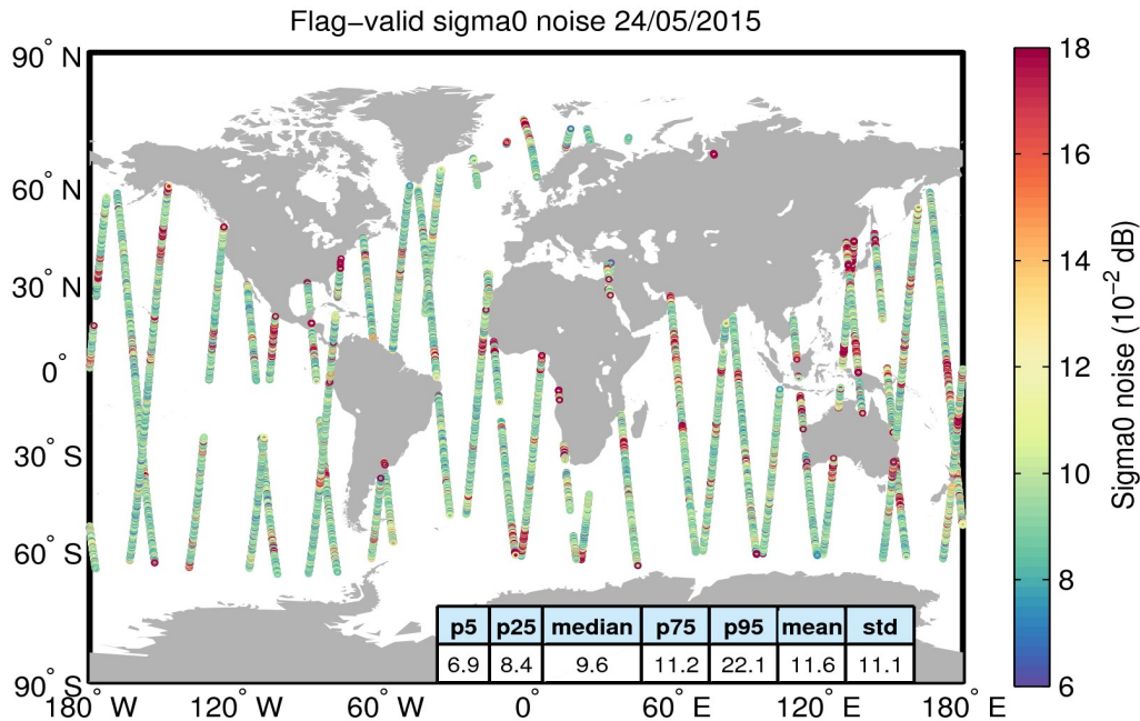
Figure 26. Geographical distribution of flag-valid 20-Hz sigma0 measurement noise over oceans and lakes for 24/05/2015. The statistical values shown in the table refer to the sigma0 noise and are calculated over all measurements shown in the figure.
