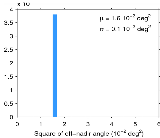
Figure 39. Histogram of flag-valid mispointing over oceans and lakes for 24/05/2015. The mean ( \mu ) and standard deviation ( \sigma ) are also shown. Note that values larger than 6 \cdot 10^{-2} \text{ deg}^2 are excluded from the histogram for the sake of readability but not from the computation of \mu and \sigma .
