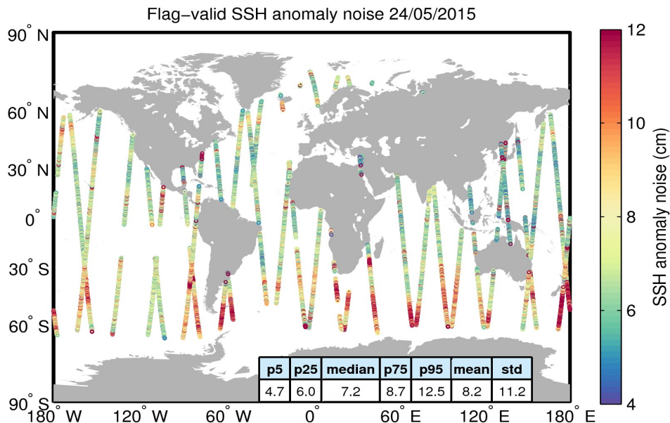
Figure 8. Geographical distribution of flag-valid 20-Hz SSH anomaly measurement noise over oceans and lakes for 24/05/2015. The statistical values shown in the table refer to the SSH anomaly noise and are calculated over all measurements shown in the figure.
