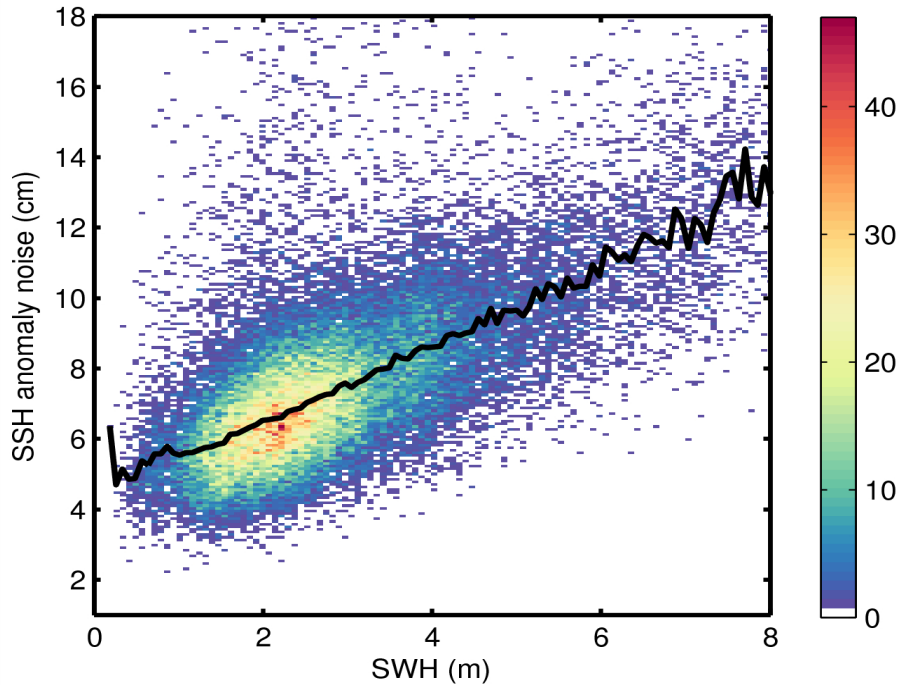
Figure 9. 2D histogram showing flag-valid SSH anomaly noise as a function of SWH for 24/05/2015. The black line denotes the median SSH anomaly as a function of SWH.
