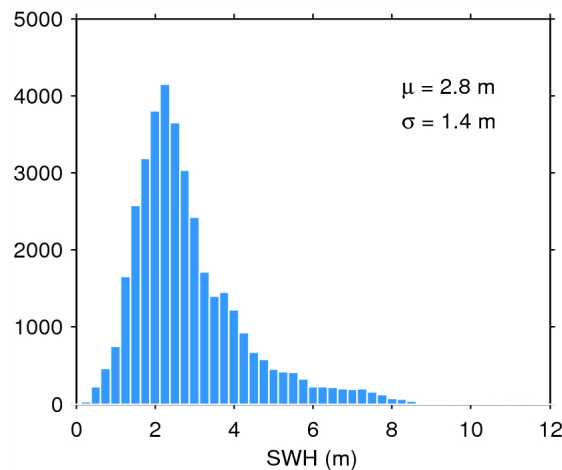
Figure 20. Histogram of science-valid SWH over oceans and lakes for 24/05/2015. The mean ( \mu ) and standard deviation ( \sigma ) are also shown. Note that values larger than 12 m are excluded from the histogram for the sake of readability but not from the computation of \mu and \sigma .
