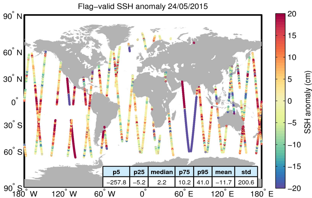
Figure 5. Geographical distribution of flag-valid 1-Hz SSH anomaly data over oceans and lakes for 24/05/2015. The statistical values shown in the table refer to the SSH anomaly in cm and are calculated over all measurements shown in the figure.
