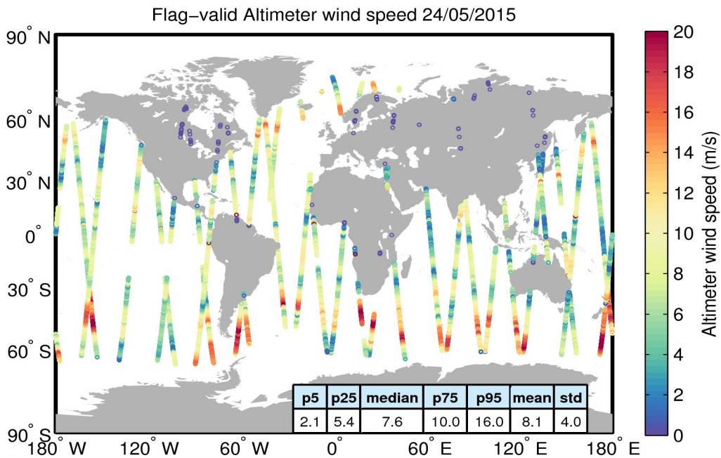
Figure 31. Geographical distribution of flag-valid wind data over oceans and lakes for 24/05/2015. The statistical values shown in the table refer to the wind in m/s and are calculated over all measurements shown in the figure.
