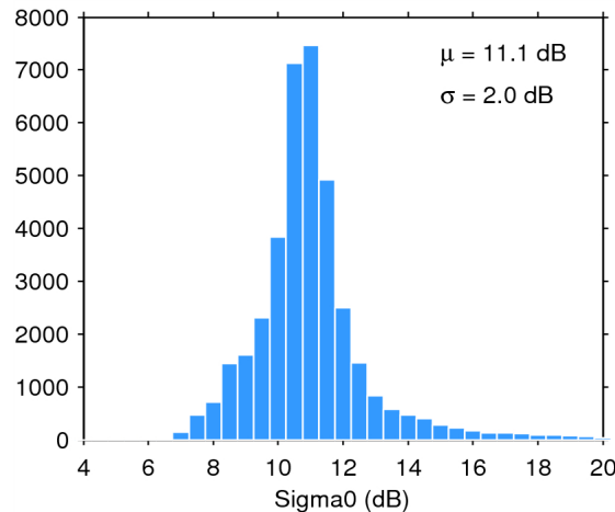
Figure 25. Histogram of flag-valid sigma0 over oceans and lakes for 24/05/2015. The mean ( \mu ) and standard deviation ( \sigma ) are also shown. Note that values outside [4 20] dB are excluded from the histogram for the sake of readability but not from the computation of \mu and \sigma .
