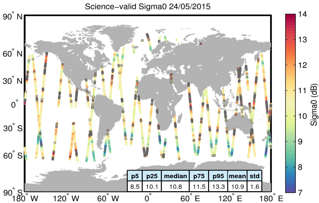
Figure 27. Geographical distribution of science-valid sigma0 data over oceans and lakes for 24/05/2015. The statistical values shown in the table refer to the sigma0 in dB and are calculated over all measurements shown in the figure. Gray circles denote records that have been rejected based on the editing criteria described in Table 4.
