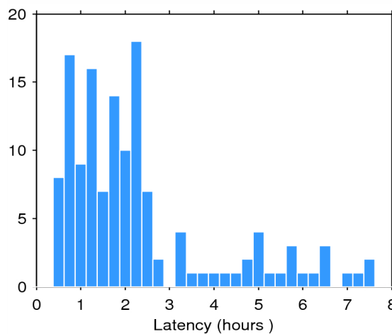
Figure 2. Histogram of the data latency for 24/05/2015. The y-axis denotes the number of files that are made available with a delay of x-hours with respect to the mean time of the records stored in the file.
