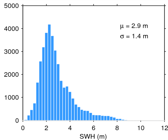
Figure 17. Histogram of flag-valid SWH over oceans and lakes for 24/05/2015. The mean ( \mu ) and standard deviation ( \sigma ) are also shown. Note that values larger than 12 m are excluded from the histogram for the sake of readability but not from the computation of \mu and \sigma .
