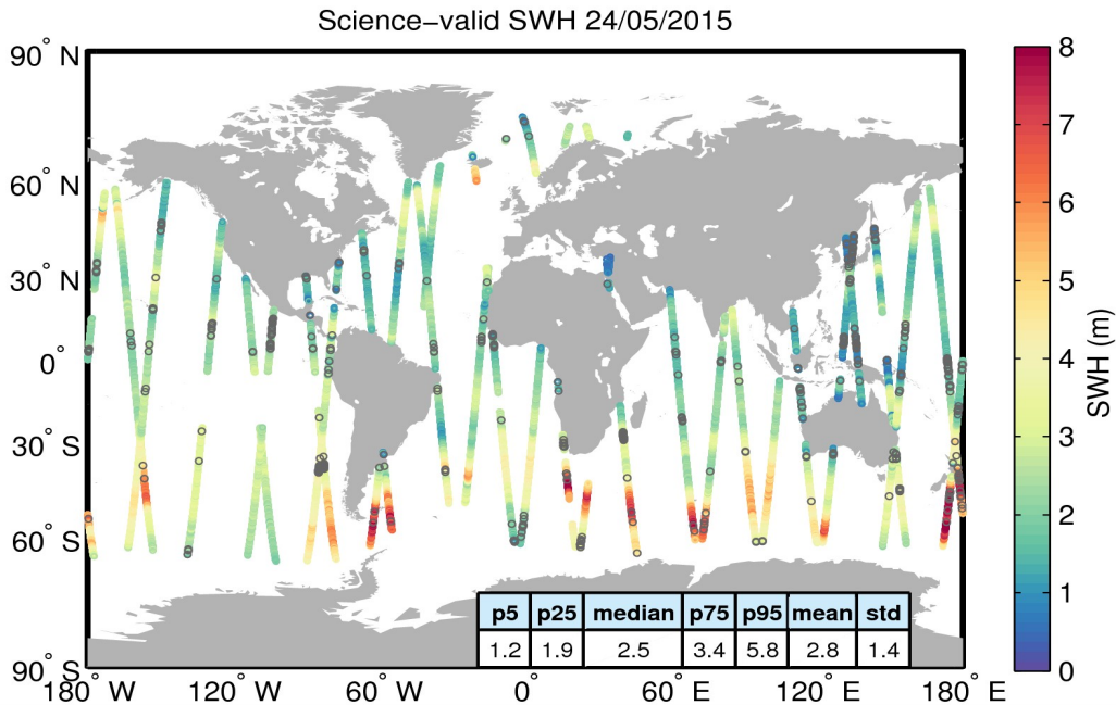
Figure 19. Geographical distribution of science-valid SWH data over oceans and lakes for 24/05/2015. The statistical values shown in the table refer to the SWH in m and are calculated over all measurements shown in the figure. Gray circles denote records that have been rejected based on the editing criteria described in Table 3.
