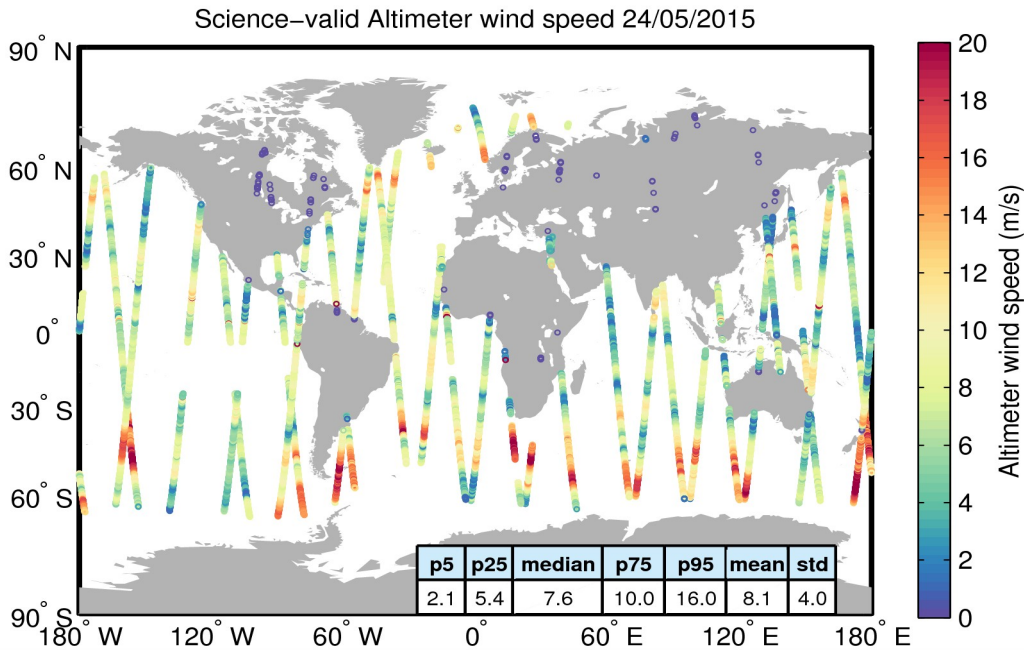
Figure 34. Geographical distribution of science-valid wind data over oceans and lakes for 24/05/2015. The statistical values shown in the table refer to the wind in m/s and are calculated over all measurements shown in the figure. Gray circles denote records that have been rejected based on the editing criteria described in Table 5.
