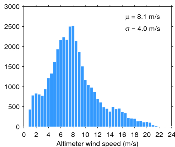
Figure 35. Histogram of science-valid wind over oceans and lakes for 24/05/2015. The mean ( \mu ) and standard deviation ( \sigma ) are also shown. Note that values larger than 24 m/s are excluded from the histogram for the sake of readability but not from the computation of \mu and \sigma .
