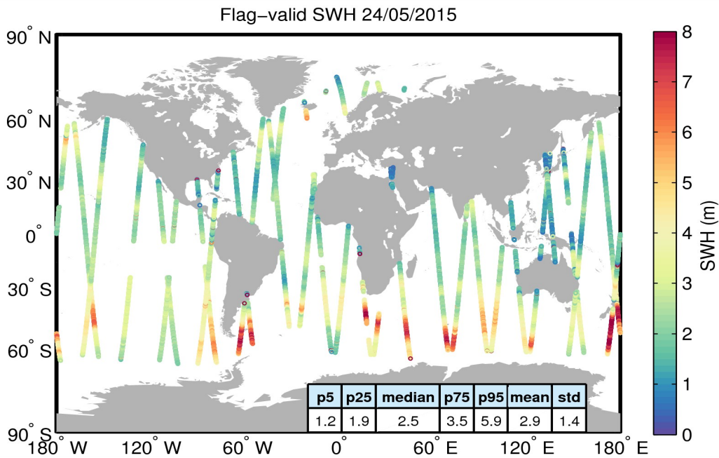
Figure 15. Geographical distribution of flag-valid SWH data over oceans and lakes for 24/05/2015. The statistical values shown in the table refer to the SWH in m and are calculated over all measurements shown in the figure.
