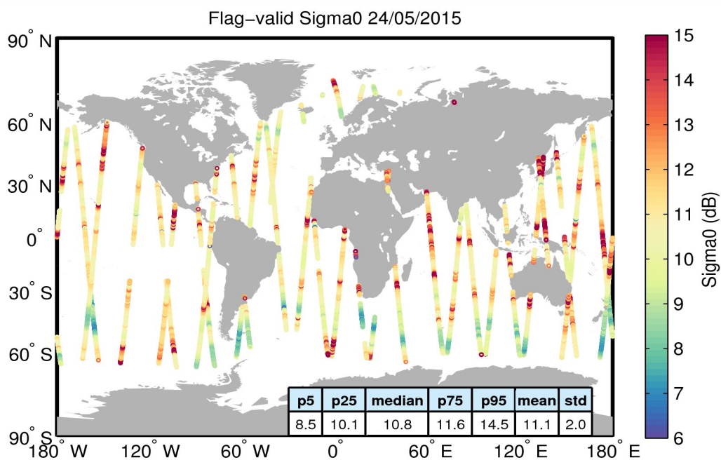
Figure 23. Geographical distribution of flag-valid sigma0 data over oceans and lakes for 24/05/2015. The statistical values shown in the table refer to the sigma0 in dB and are calculated over all measurements shown in the figure.
