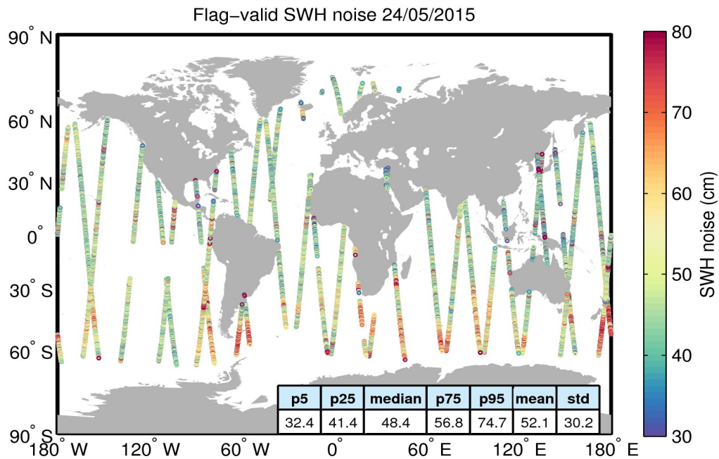
Figure 18. Geographical distribution of flag-valid 20-Hz SWH measurement noise over oceans and lakes for 24/05/2015. The statistical values shown in the figure refer to the SWH noise and are calculated over all measurements shown in the figure.
