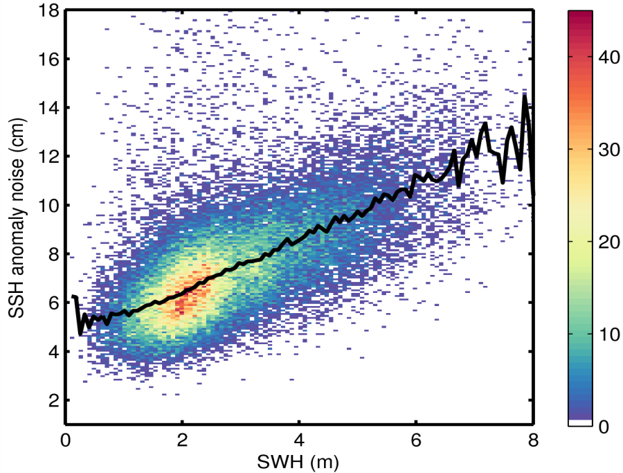
Figure 9. 2D histogram showing flag-valid SSH anomaly noise as a function of SWH for 23/05/2015. The black line denotes the median SSH anomaly as a function of SWH.
