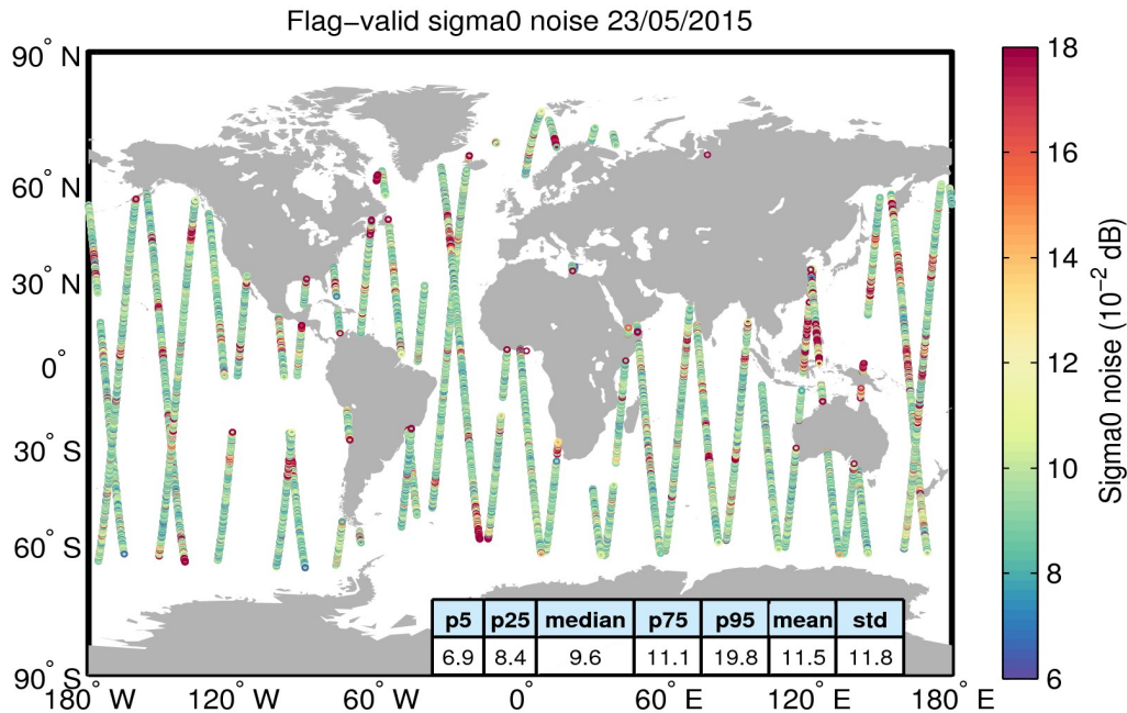
Figure 26. Geographical distribution of flag-valid 20-Hz sigma0 measurement noise over oceans and lakes for 23/05/2015. The statistical values shown in the table refer to the sigma0 noise and are calculated over all measurements shown in the figure.
