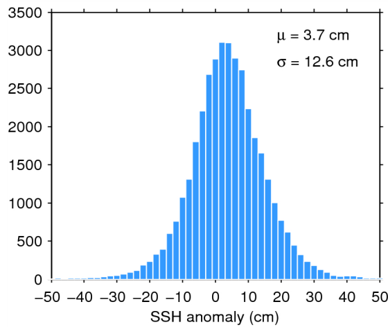
Figure 11. Histogram of science-valid SSH anomaly over oceans and lakes for 23/05/2015. The mean ( \mu ) and standard deviation ( \sigma ) are also shown. Note that values outside [-50 50] cm are excluded from the histogram for the sake of readability but not from the computation of \mu and \sigma .
