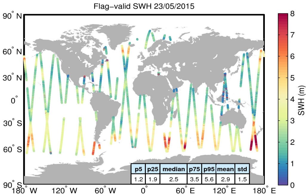
Figure 15. Geographical distribution of flag-valid SWH data over oceans and lakes for 23/05/2015. The statistical values shown in the table refer to the SWH in m and are calculated over all measurements shown in the figure.
