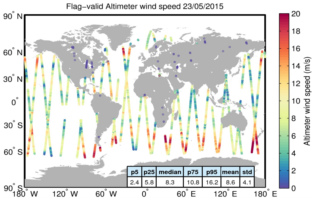
Figure 31. Geographical distribution of flag-valid wind data over oceans and lakes for 23/05/2015. The statistical values shown in the table refer to the wind in m/s and are calculated over all measurements shown in the figure.
