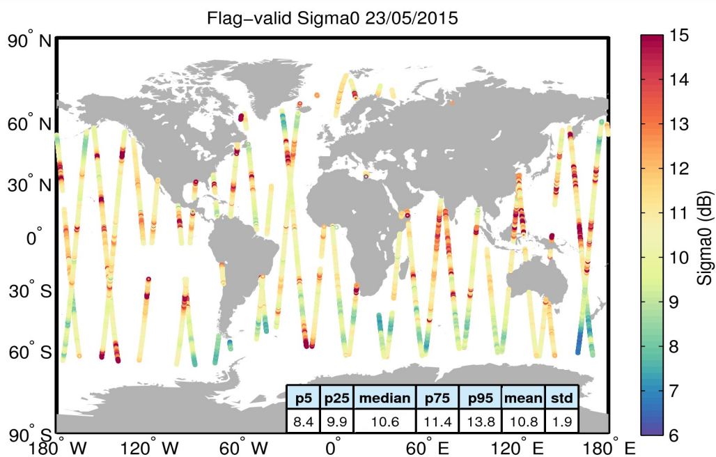
Figure 23. Geographical distribution of flag-valid sigma0 data over oceans and lakes for 23/05/2015. The statistical values shown in the table refer to the sigma0 in dB and are calculated over all measurements shown in the figure.
