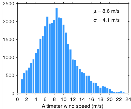
Figure 33. Histogram of flag-valid wind over oceans and lakes for 23/05/2015. The mean ( \mu ) and standard deviation ( \sigma ) are also shown. Note that values larger than 24 m/s are excluded from the histogram for the sake of readability but not from the computation of \mu and \sigma .
