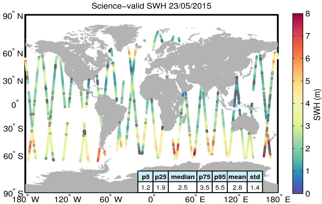
Figure 19. Geographical distribution of science-valid SWH data over oceans and lakes for 23/05/2015. The statistical values shown in the table refer to the SWH in m and are calculated over all measurements shown in the figure. Gray circles denote records that have been rejected based on the editing criteria described in Table 3.
