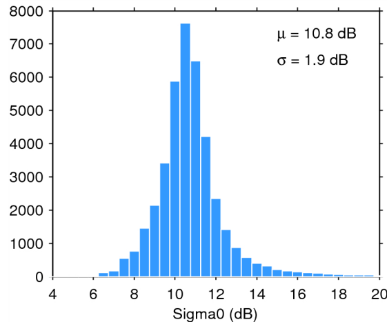
Figure 25. Histogram of flag-valid sigma0 over oceans and lakes for 23/05/2015. The mean ( \mu ) and standard deviation ( \sigma ) are also shown. Note that values outside [4 20] dB are excluded from the histogram for the sake of readability but not from the computation of \mu and \sigma .
