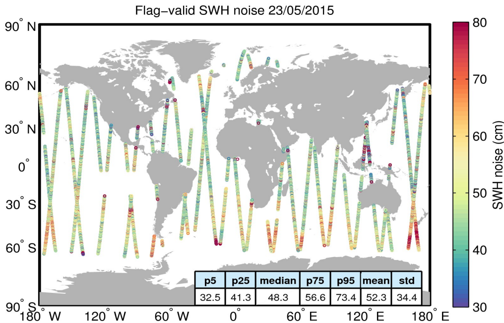
Figure 18. Geographical distribution of flag-valid 20-Hz SWH measurement noise over oceans and lakes for 23/05/2015. The statistical values shown in the figure refer to the SWH noise and are calculated over all measurements shown in the figure.
