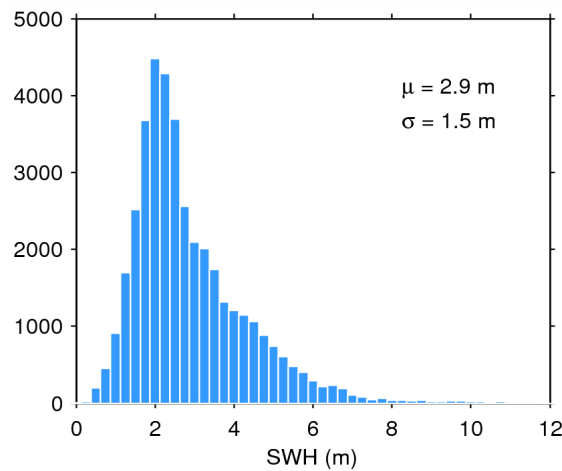
Figure 17. Histogram of flag-valid SWH over oceans and lakes for 23/05/2015. The mean ( \mu ) and standard deviation ( \sigma ) are also shown. Note that values larger than 12 m are excluded from the histogram for the sake of readability but not from the computation of \mu and \sigma .
