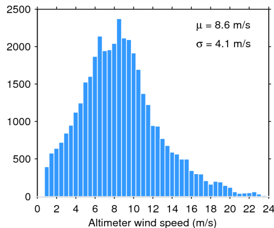
Figure 35. Histogram of science-valid wind over oceans and lakes for 23/05/2015. The mean ( \mu ) and standard deviation ( \sigma ) are also shown. Note that values larger than 24 m/s are excluded from the histogram for the sake of readability but not from the computation of \mu and \sigma .
