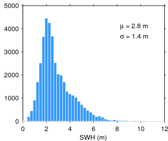
Figure 20. Histogram of science-valid SWH over oceans and lakes for 23/05/2015. The mean ( \mu ) and standard deviation ( \sigma ) are also shown. Note that values larger than 12 m are excluded from the histogram for the sake of readability but not from the computation of \mu and \sigma .
