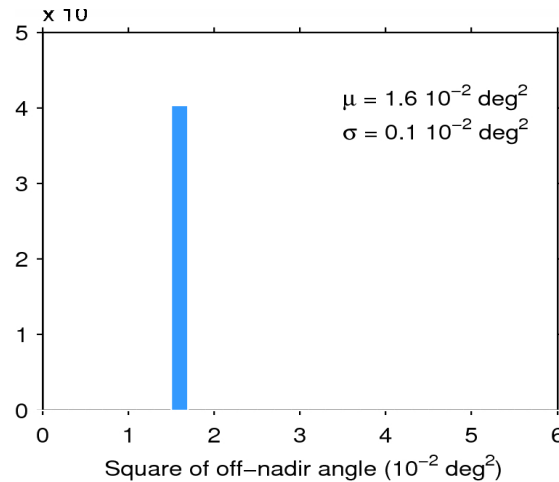
Figure 39. Histogram of flag-valid mispointing over oceans and lakes for 23/05/2015. The mean ( \mu ) and standard deviation ( \sigma ) are also shown. Note that values larger than 6 \cdot 10^{-2} \text{ deg}^2 are excluded from the histogram for the sake of readability but not from the computation of \mu and \sigma .
