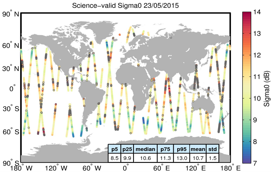
Figure 27. Geographical distribution of science-valid sigma0 data over oceans and lakes for 23/05/2015. The statistical values shown in the table refer to the sigma0 in dB and are calculated over all measurements shown in the figure. Gray circles denote records that have been rejected based on the editing criteria described in Table 4.
