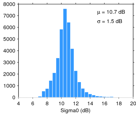
Figure 28. Histogram of science-valid sigma0 over oceans and lakes for 23/05/2015. The mean ( \mu ) and standard deviation ( \sigma ) are also shown. Note that values outside [4 20] dB are excluded from the histogram for the sake of readability but not from the computation of \mu and \sigma .
