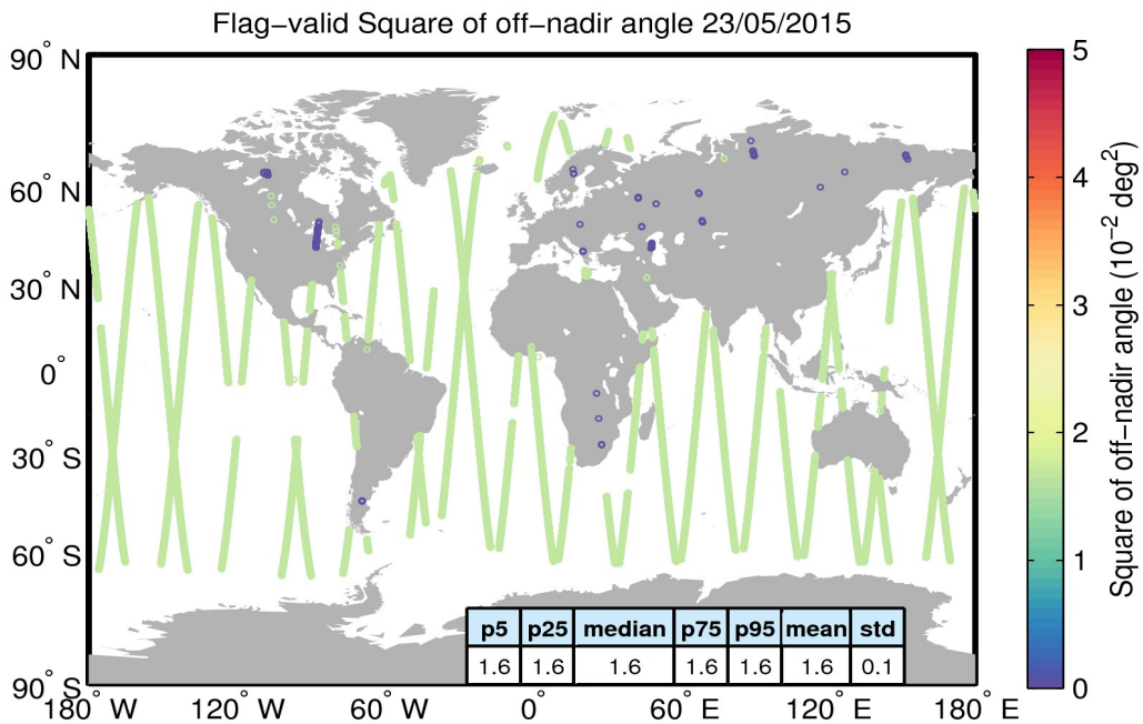
Figure 37. Geographical distribution of flag-valid mispointing data over oceans and lakes for 23/05/2015. The statistical values shown in the table refer to the mispointing in 10^{-2} \text{ deg}^2 and are calculated over all measurements shown in the figure.
