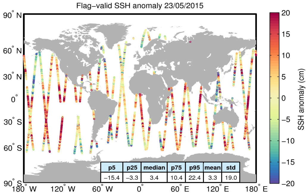
Figure 5. Geographical distribution of flag-valid 1-Hz SSH anomaly data over oceans and lakes for 23/05/2015. The statistical values shown in the table refer to the SSH anomaly in cm and are calculated over all measurements shown in the figure.
