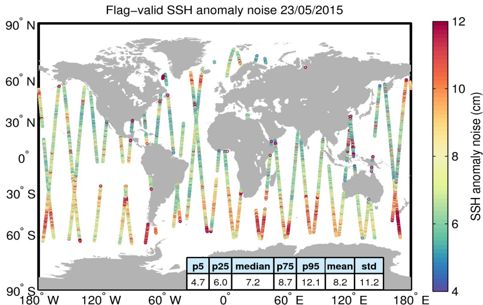
Figure 8. Geographical distribution of flag-valid 20-Hz SSH anomaly measurement noise over oceans and lakes for 23/05/2015. The statistical values shown in the table refer to the SSH anomaly noise and are calculated over all measurements shown in the figure.
