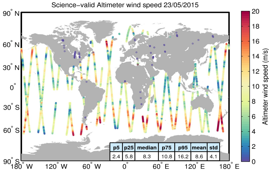
Figure 34. Geographical distribution of science-valid wind data over oceans and lakes for 23/05/2015. The statistical values shown in the table refer to the wind in m/s and are calculated over all measurements shown in the figure. Gray circles denote records that have been rejected based on the editing criteria described in Table 5.
