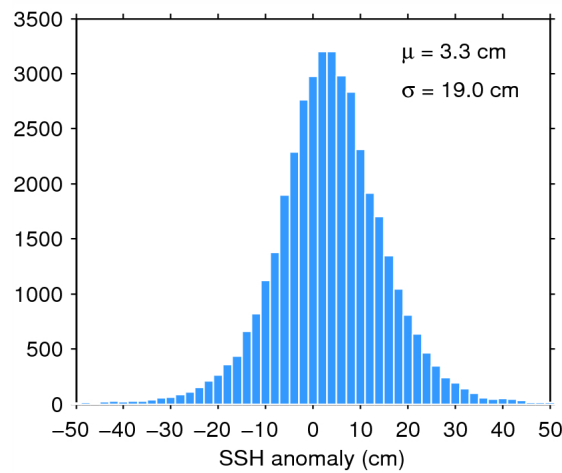
Figure 7. Histogram of flag-valid SSH anomaly over oceans and lakes for 23/05/2015. The mean ( \mu ) and standard deviation ( \sigma ) are also shown. Note that values outside [-50\ 50] cm are excluded from the histogram for the sake of readability but not from the computation of \mu and \sigma .
