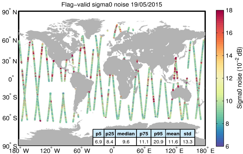
Figure 26. Geographical distribution of flag-valid 20-Hz sigma0 measurement noise over oceans and lakes for 19/05/2015. The statistical values shown in the table refer to the sigma0 noise and are calculated over all measurements shown in the figure.
