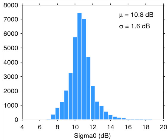
Figure 28. Histogram of science-valid sigma0 over oceans and lakes for 19/05/2015. The mean ( \mu ) and standard deviation ( \sigma ) are also shown. Note that values outside [4 20] dB are excluded from the histogram for the sake of readability but not from the computation of \mu and \sigma .
