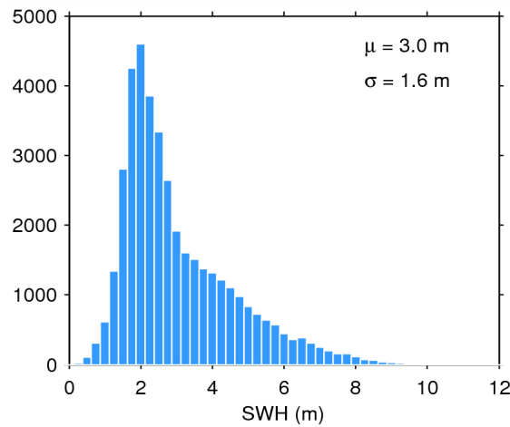
Figure 17. Histogram of flag-valid SWH over oceans and lakes for 19/05/2015. The mean ( \mu ) and standard deviation ( \sigma ) are also shown. Note that values larger than 12 m are excluded from the histogram for the sake of readability but not from the computation of \mu and \sigma .
