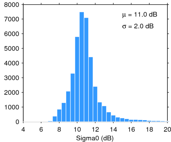
Figure 25. Histogram of flag-valid sigma0 over oceans and lakes for 19/05/2015. The mean ( \mu ) and standard deviation ( \sigma ) are also shown. Note that values outside [4 20] dB are excluded from the histogram for the sake of readability but not from the computation of \mu and \sigma .
