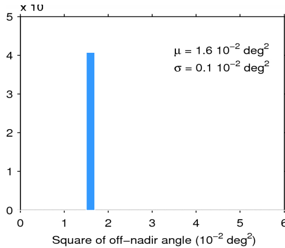
Figure 39. Histogram of flag-valid mispointing over oceans and lakes for 19/05/2015. The mean ( \mu ) and standard deviation ( \sigma ) are also shown. Note that values larger than 6 \cdot 10^{-2} \text{ deg}^2 are excluded from the histogram for the sake of readability but not from the computation of \mu and \sigma .
