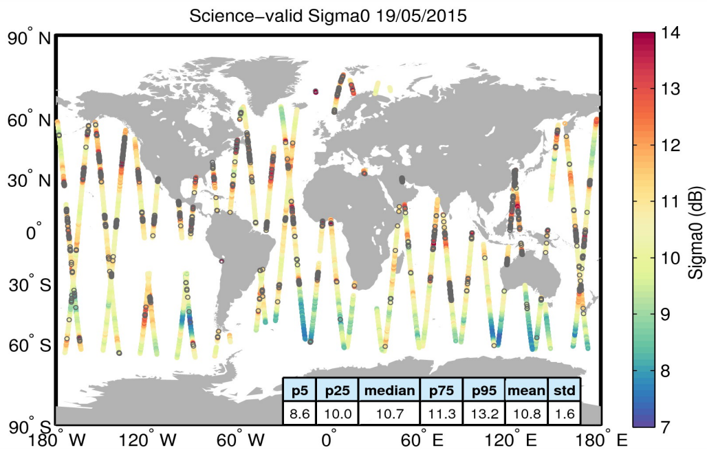
Figure 27. Geographical distribution of science-valid sigma0 data over oceans and lakes for 19/05/2015. The statistical values shown in the table refer to the sigma0 in dB and are calculated over all measurements shown in the figure. Gray circles denote records that have been rejected based on the editing criteria described in Table 4.
