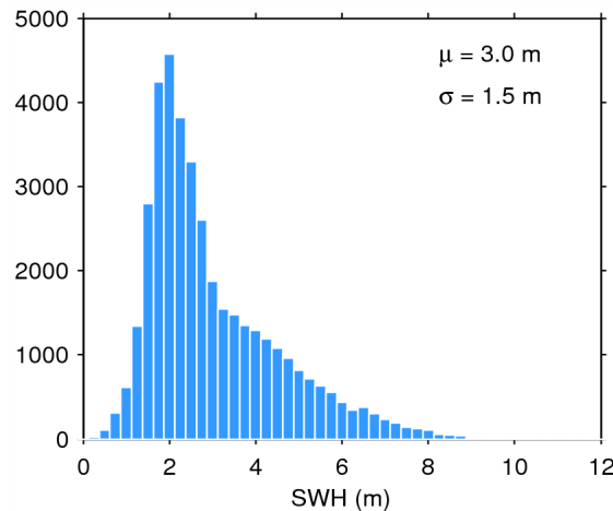
Figure 20. Histogram of science-valid SWH over oceans and lakes for 19/05/2015. The mean ( \mu ) and standard deviation ( \sigma ) are also shown. Note that values larger than 12 m are excluded from the histogram for the sake of readability but not from the computation of \mu and \sigma .
