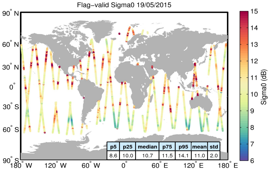
Figure 23. Geographical distribution of flag-valid sigma0 data over oceans and lakes for 19/05/2015. The statistical values shown in the table refer to the sigma0 in dB and are calculated over all measurements shown in the figure.
