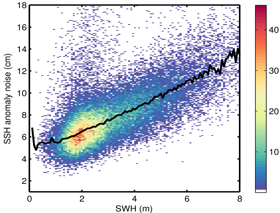
Figure 9. 2D histogram showing flag-valid SSH anomaly noise as a function of SWH for 19/05/2015. The black line denotes the median SSH anomaly as a function of SWH.
