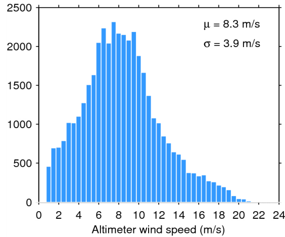
Figure 33. Histogram of flag-valid wind over oceans and lakes for 19/05/2015. The mean ( \mu ) and standard deviation ( \sigma ) are also shown. Note that values larger than 24 m/s are excluded from the histogram for the sake of readability but not from the computation of \mu and \sigma .
