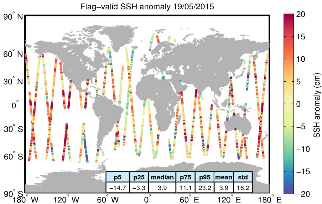
Figure 5. Geographical distribution of flag-valid 1-Hz SSH anomaly data over oceans and lakes for 19/05/2015. The statistical values shown in the table refer to the SSH anomaly in cm and are calculated over all measurements shown in the figure.
