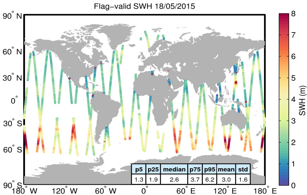
Figure 15. Geographical distribution of flag-valid SWH data over oceans and lakes for 18/05/2015. The statistical values shown in the table refer to the SWH in m and are calculated over all measurements shown in the figure.
