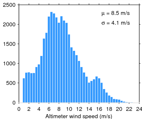
Figure 35. Histogram of science-valid wind over oceans and lakes for 18/05/2015. The mean ( \mu ) and standard deviation ( \sigma ) are also shown. Note that values larger than 24 m/s are excluded from the histogram for the sake of readability but not from the computation of \mu and \sigma .
