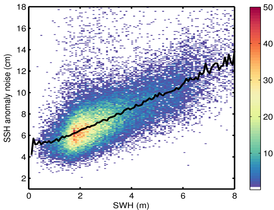
Figure 9. 2D histogram showing flag-valid SSH anomaly noise as a function of SWH for 18/05/2015. The black line denotes the median SSH anomaly as a function of SWH.
