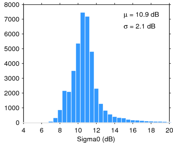
Figure 25. Histogram of flag-valid sigma0 over oceans and lakes for 18/05/2015. The mean ( \mu ) and standard deviation ( \sigma ) are also shown. Note that values outside [4 20] dB are excluded from the histogram for the sake of readability but not from the computation of \mu and \sigma .
