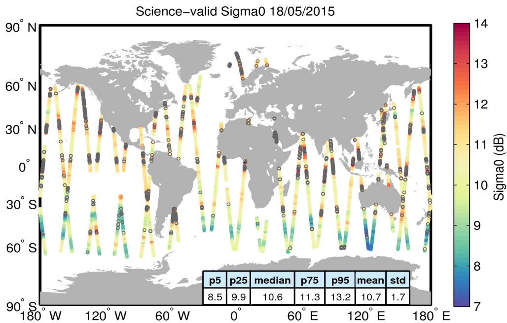
Figure 27. Geographical distribution of science-valid sigma0 data over oceans and lakes for 18/05/2015. The statistical values shown in the table refer to the sigma0 in dB and are calculated over all measurements shown in the figure. Gray circles denote records that have been rejected based on the editing criteria described in Table 4.
