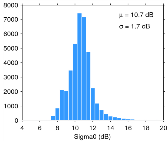
Figure 28. Histogram of science-valid sigma0 over oceans and lakes for 18/05/2015. The mean ( \mu ) and standard deviation ( \sigma ) are also shown. Note that values outside [4 20] dB are excluded from the histogram for the sake of readability but not from the computation of \mu and \sigma .
