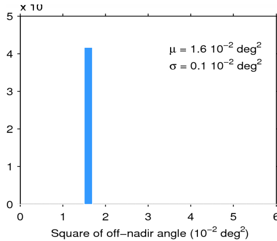
Figure 39. Histogram of flag-valid mispointing over oceans and lakes for 18/05/2015. The mean ( \mu ) and standard deviation ( \sigma ) are also shown. Note that values larger than 6 \cdot 10^{-2} \text{ deg}^2 are excluded from the histogram for the sake of readability but not from the computation of \mu and \sigma .
