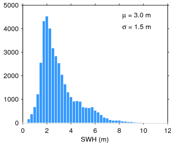
Figure 20. Histogram of science-valid SWH over oceans and lakes for 18/05/2015. The mean ( \mu ) and standard deviation ( \sigma ) are also shown. Note that values larger than 12 m are excluded from the histogram for the sake of readability but not from the computation of \mu and \sigma .
