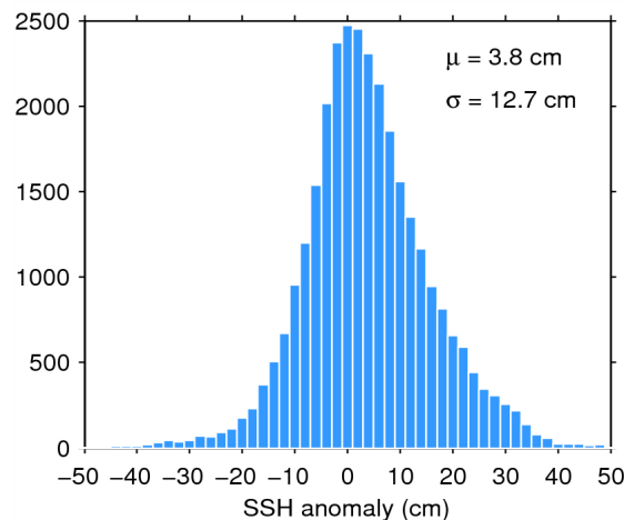
Figure 11. Histogram of science-valid SSH anomaly over oceans and lakes for 18/05/2015. The mean ( \mu ) and standard deviation ( \sigma ) are also shown. Note that values outside [-50 50] cm are excluded from the histogram for the sake of readability but not from the computation of \mu and \sigma .
