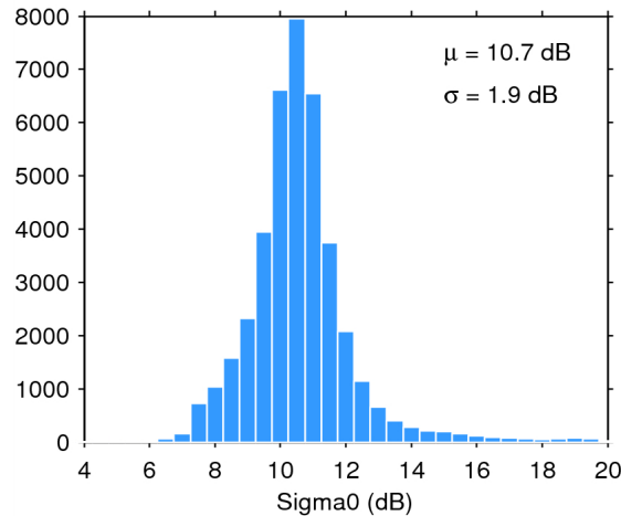
Figure 25. Histogram of flag-valid sigma0 over oceans and lakes for 17/05/2015. The mean ( \mu ) and standard deviation ( \sigma ) are also shown. Note that values outside [4 20] dB are excluded from the histogram for the sake of readability but not from the computation of \mu and \sigma .
