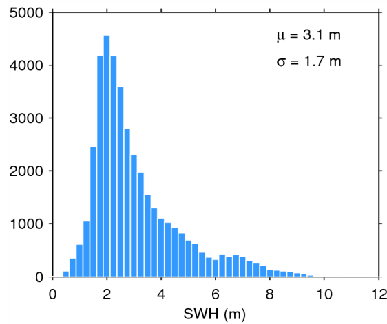
Figure 17. Histogram of flag-valid SWH over oceans and lakes for 17/05/2015. The mean ( \mu ) and standard deviation ( \sigma ) are also shown. Note that values larger than 12 m are excluded from the histogram for the sake of readability but not from the computation of \mu and \sigma .
