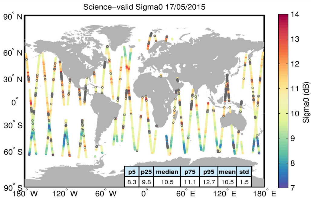
Figure 27. Geographical distribution of science-valid sigma0 data over oceans and lakes for 17/05/2015. The statistical values shown in the table refer to the sigma0 in dB and are calculated over all measurements shown in the figure. Gray circles denote records that have been rejected based on the editing criteria described in Table 4.
