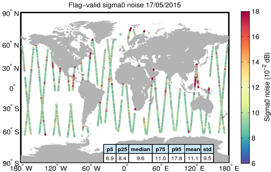
Figure 26. Geographical distribution of flag-valid 20-Hz sigma0 measurement noise over oceans and lakes for 17/05/2015. The statistical values shown in the table refer to the sigma0 noise and are calculated over all measurements shown in the figure.
