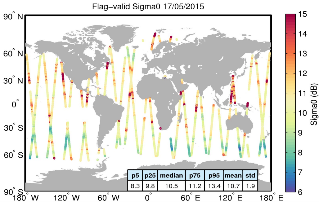
Figure 23. Geographical distribution of flag-valid sigma0 data over oceans and lakes for 17/05/2015. The statistical values shown in the table refer to the sigma0 in dB and are calculated over all measurements shown in the figure.
