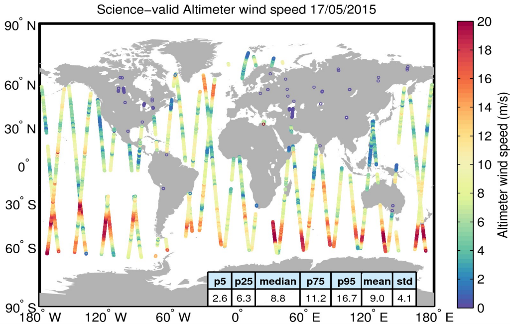
Figure 34. Geographical distribution of science-valid wind data over oceans and lakes for 17/05/2015. The statistical values shown in the table refer to the wind in m/s and are calculated over all measurements shown in the figure. Gray circles denote records that have been rejected based on the editing criteria described in Table 5.
