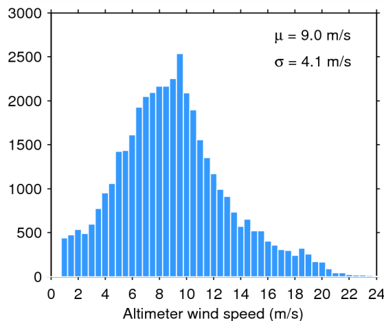
Figure 35. Histogram of science-valid wind over oceans and lakes for 17/05/2015. The mean ( \mu ) and standard deviation ( \sigma ) are also shown. Note that values larger than 24 m/s are excluded from the histogram for the sake of readability but not from the computation of \mu and \sigma .
