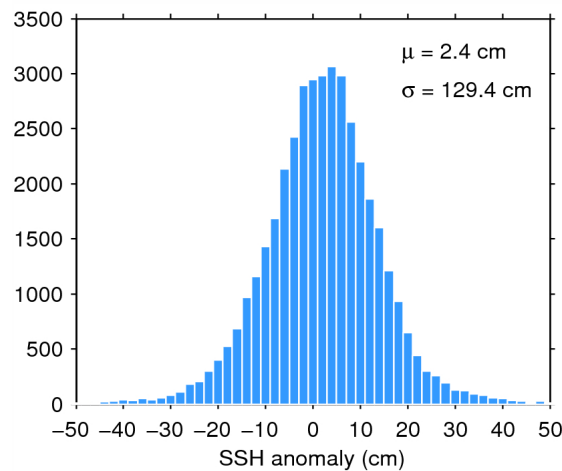
Figure 7. Histogram of flag-valid SSH anomaly over oceans and lakes for 17/05/2015. The mean ( \mu ) and standard deviation ( \sigma ) are also shown. Note that values outside [-50\ 50] cm are excluded from the histogram for the sake of readability but not from the computation of \mu and \sigma .
