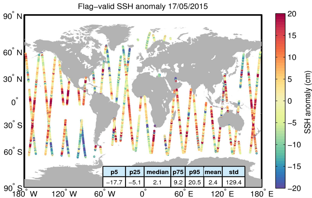
Figure 5. Geographical distribution of flag-valid 1-Hz SSH anomaly data over oceans and lakes for 17/05/2015. The statistical values shown in the table refer to the SSH anomaly in cm and are calculated over all measurements shown in the figure.
