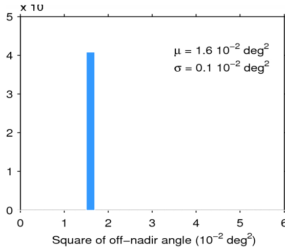
Figure 39. Histogram of flag-valid mispointing over oceans and lakes for 17/05/2015. The mean ( \mu ) and standard deviation ( \sigma ) are also shown. Note that values larger than 6 \cdot 10^{-2} \text{ deg}^2 are excluded from the histogram for the sake of readability but not from the computation of \mu and \sigma .
