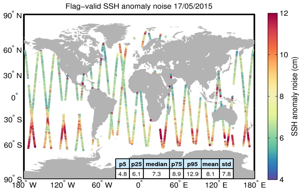
Figure 8. Geographical distribution of flag-valid 20-Hz SSH anomaly measurement noise over oceans and lakes for 17/05/2015. The statistical values shown in the table refer to the SSH anomaly noise and are calculated over all measurements shown in the figure.
