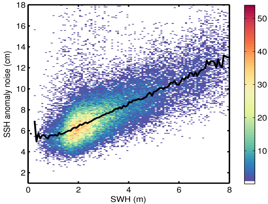
Figure 9. 2D histogram showing flag-valid SSH anomaly noise as a function of SWH for 17/05/2015. The black line denotes the median SSH anomaly as a function of SWH.
