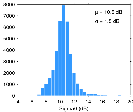
Figure 28. Histogram of science-valid sigma0 over oceans and lakes for 17/05/2015. The mean ( \mu ) and standard deviation ( \sigma ) are also shown. Note that values outside [4 20] dB are excluded from the histogram for the sake of readability but not from the computation of \mu and \sigma .
