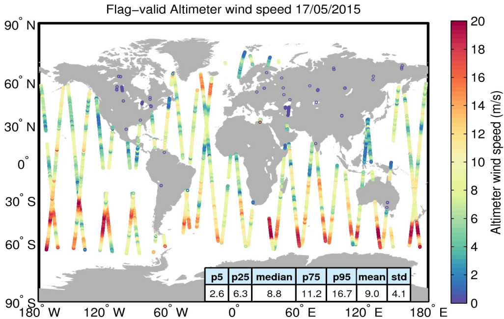
Figure 31. Geographical distribution of flag-valid wind data over oceans and lakes for 17/05/2015. The statistical values shown in the table refer to the wind in m/s and are calculated over all measurements shown in the figure.
