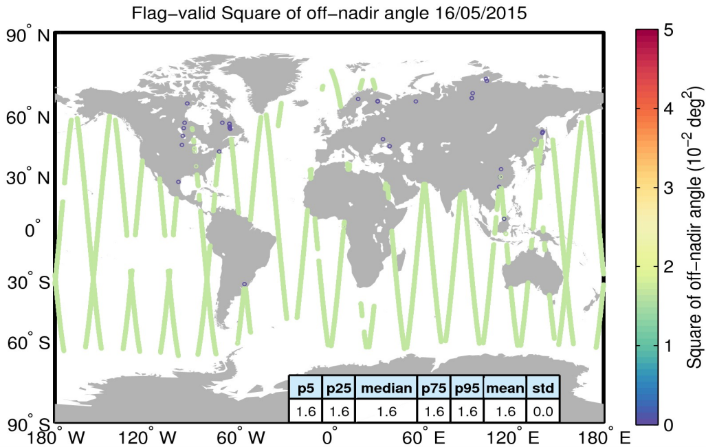
Figure 37. Geographical distribution of flag-valid mispointing data over oceans and lakes for 16/05/2015. The statistical values shown in the table refer to the mispointing in 10^{-2} \text{ deg}^2 and are calculated over all measurements shown in the figure.
