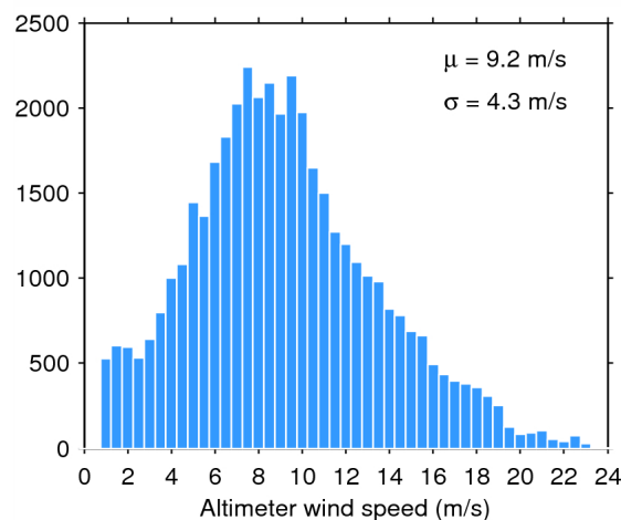
Figure 35. Histogram of science-valid wind over oceans and lakes for 16/05/2015. The mean ( \mu ) and standard deviation ( \sigma ) are also shown. Note that values larger than 24 m/s are excluded from the histogram for the sake of readability but not from the computation of \mu and \sigma .
