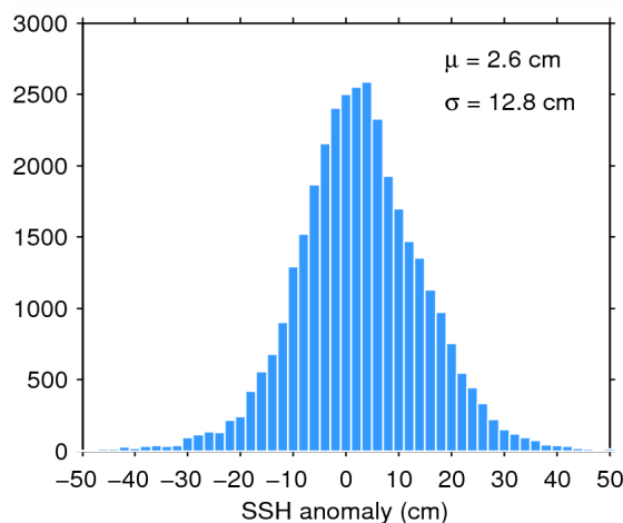
Figure 11. Histogram of science-valid SSH anomaly over oceans and lakes for 16/05/2015. The mean ( \mu ) and standard deviation ( \sigma ) are also shown. Note that values outside [-50 50] cm are excluded from the histogram for the sake of readability but not from the computation of \mu and \sigma .
