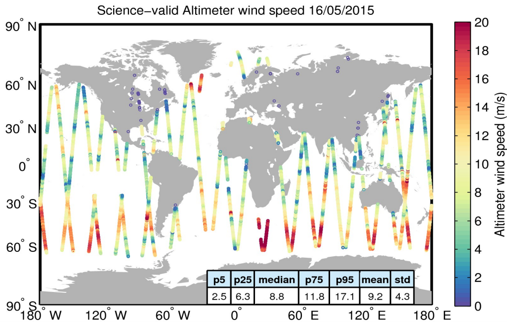
Figure 34. Geographical distribution of science-valid wind data over oceans and lakes for 16/05/2015. The statistical values shown in the table refer to the wind in m/s and are calculated over all measurements shown in the figure. Gray circles denote records that have been rejected based on the editing criteria described in Table 5.
