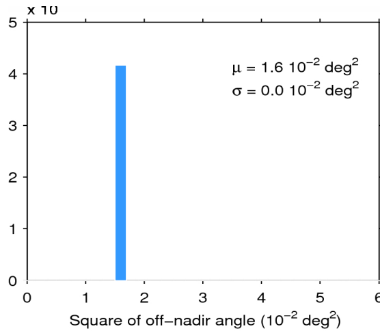
Figure 39. Histogram of flag-valid mispointing over oceans and lakes for 16/05/2015. The mean ( \mu ) and standard deviation ( \sigma ) are also shown. Note that values larger than 6 \cdot 10^{-2} \text{ deg}^2 are excluded from the histogram for the sake of readability but not from the computation of \mu and \sigma .
