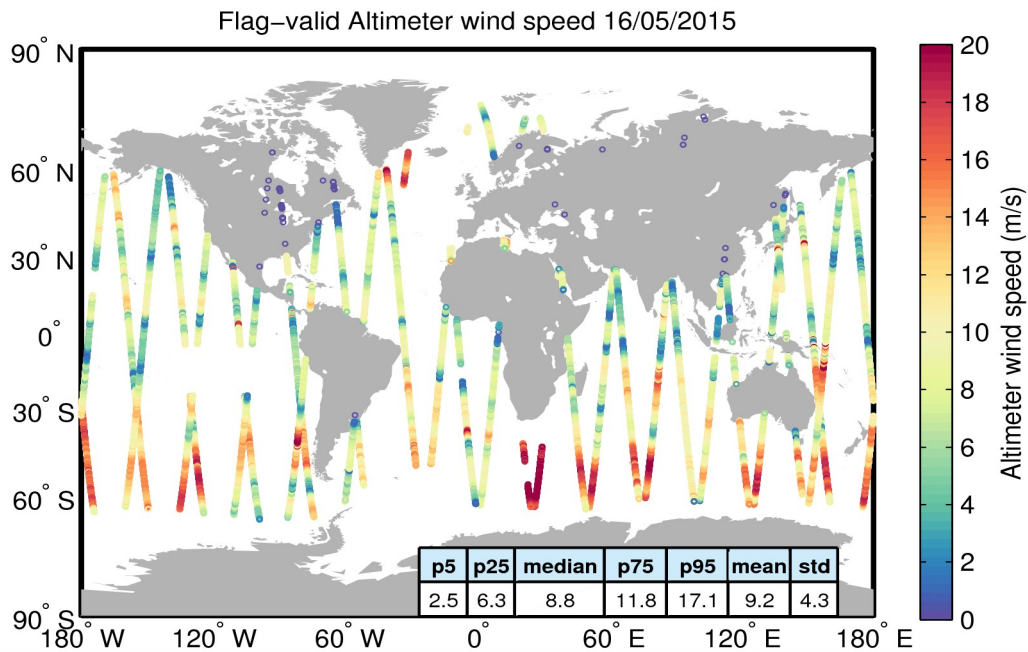
Figure 31. Geographical distribution of flag-valid wind data over oceans and lakes for 16/05/2015. The statistical values shown in the table refer to the wind in m/s and are calculated over all measurements shown in the figure.
