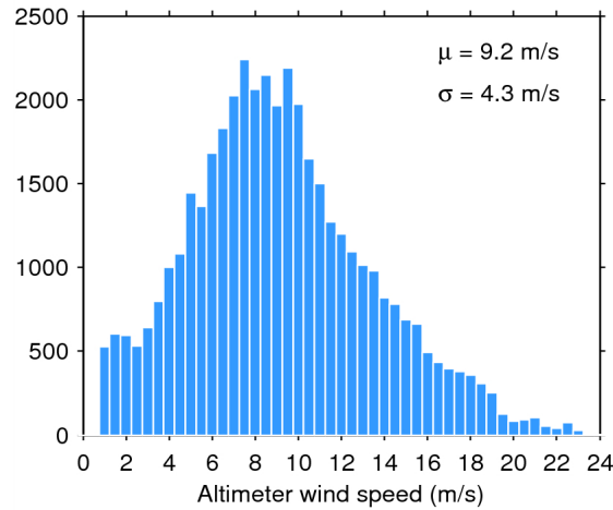
Figure 33. Histogram of flag-valid wind over oceans and lakes for 16/05/2015. The mean ( \mu ) and standard deviation ( \sigma ) are also shown. Note that values larger than 24 m/s are excluded from the histogram for the sake of readability but not from the computation of \mu and \sigma .
