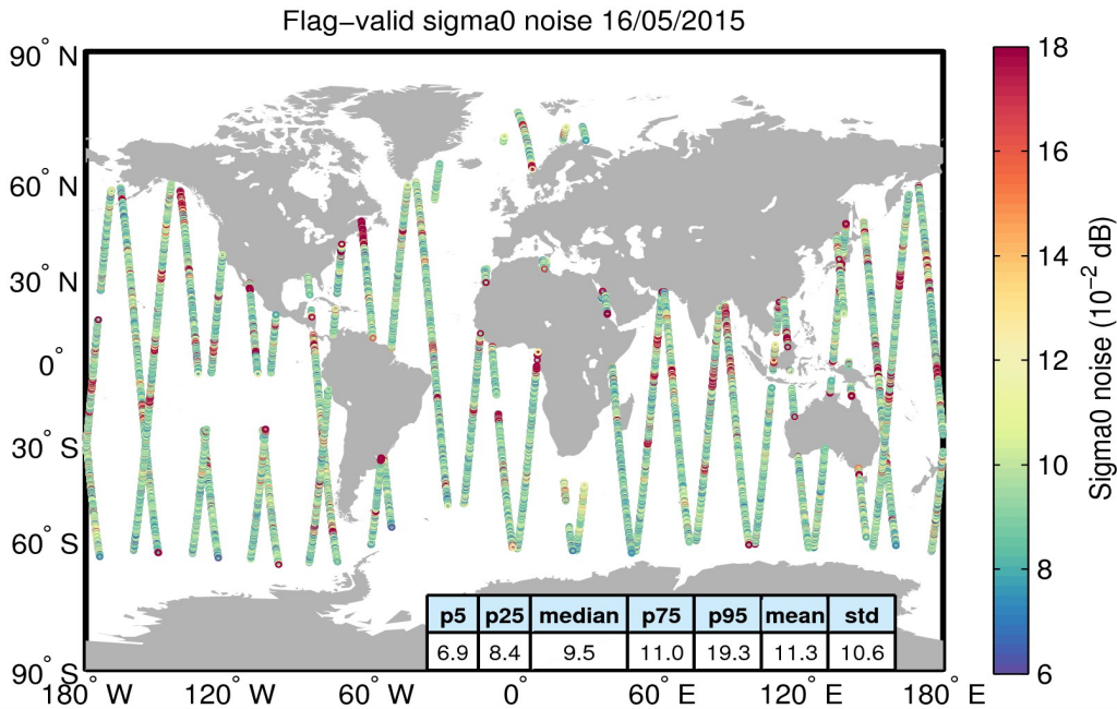
Figure 26. Geographical distribution of flag-valid 20-Hz sigma0 measurement noise over oceans and lakes for 16/05/2015. The statistical values shown in the table refer to the sigma0 noise and are calculated over all measurements shown in the figure.
