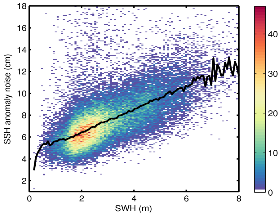
Figure 9. 2D histogram showing flag-valid SSH anomaly noise as a function of SWH for 16/05/2015. The black line denotes the median SSH anomaly as a function of SWH.
