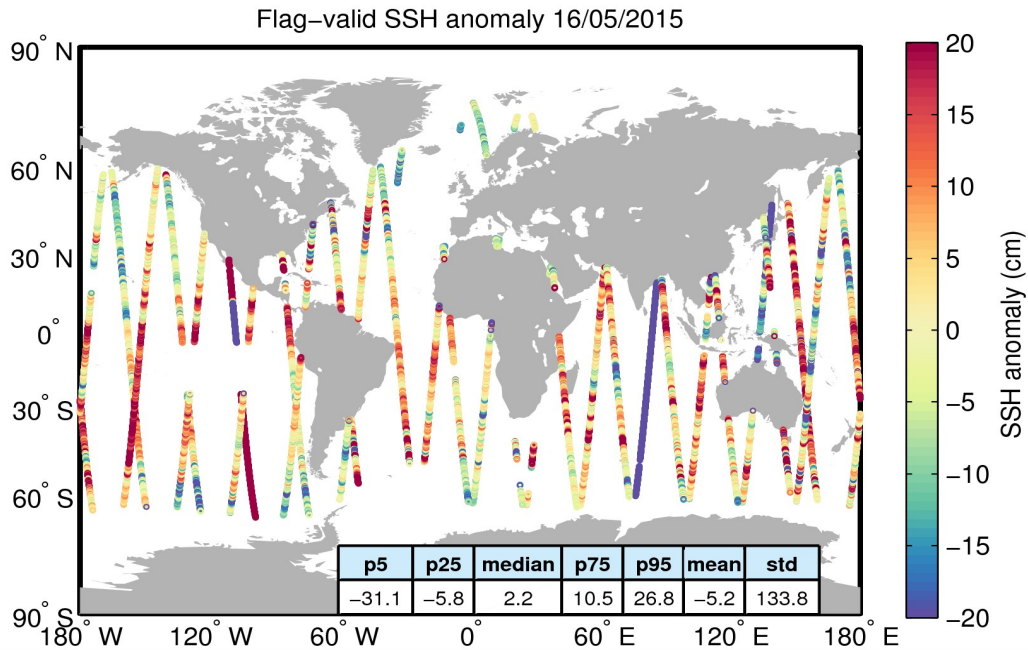
Figure 5. Geographical distribution of flag-valid 1-Hz SSH anomaly data over oceans and lakes for 16/05/2015. The statistical values shown in the table refer to the SSH anomaly in cm and are calculated over all measurements shown in the figure.
