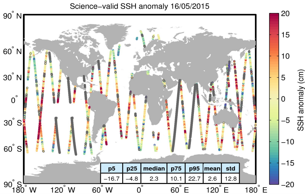
Figure 10. Geographical distribution of science-valid SSH anomaly data over oceans and lakes for 16/05/2015. The statistical values shown in the table refer to the SSH anomaly in cm and are calculated over all measurements shown in the figure. Gray circles denote records that have been rejected based on the editing criteria described in Table 2.
