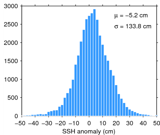
Figure 7. Histogram of flag-valid SSH anomaly over oceans and lakes for 16/05/2015. The mean ( \mu ) and standard deviation ( \sigma ) are also shown. Note that values outside [-50 50] cm are excluded from the histogram for the sake of readability but not from the computation of \mu and \sigma .
