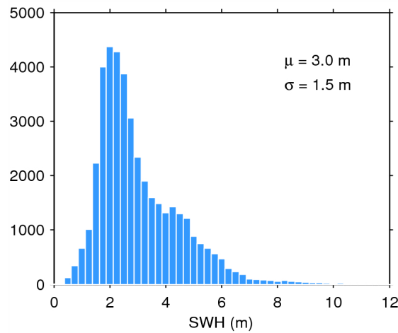
Figure 17. Histogram of flag-valid SWH over oceans and lakes for 16/05/2015. The mean ( \mu ) and standard deviation ( \sigma ) are also shown. Note that values larger than 12 m are excluded from the histogram for the sake of readability but not from the computation of \mu and \sigma .
