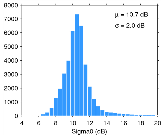
Figure 25. Histogram of flag-valid sigma0 over oceans and lakes for 16/05/2015. The mean ( \mu ) and standard deviation ( \sigma ) are also shown. Note that values outside [4 20] dB are excluded from the histogram for the sake of readability but not from the computation of \mu and \sigma .
