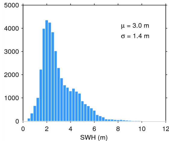
Figure 20. Histogram of science-valid SWH over oceans and lakes for 16/05/2015. The mean ( \mu ) and standard deviation ( \sigma ) are also shown. Note that values larger than 12 m are excluded from the histogram for the sake of readability but not from the computation of \mu and \sigma .
