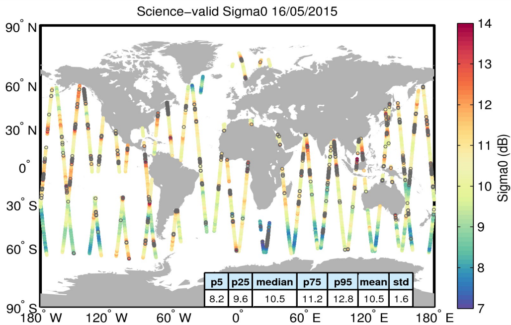
Figure 27. Geographical distribution of science-valid sigma0 data over oceans and lakes for 16/05/2015. The statistical values shown in the table refer to the sigma0 in dB and are calculated over all measurements shown in the figure. Gray circles denote records that have been rejected based on the editing criteria described in Table 4.
