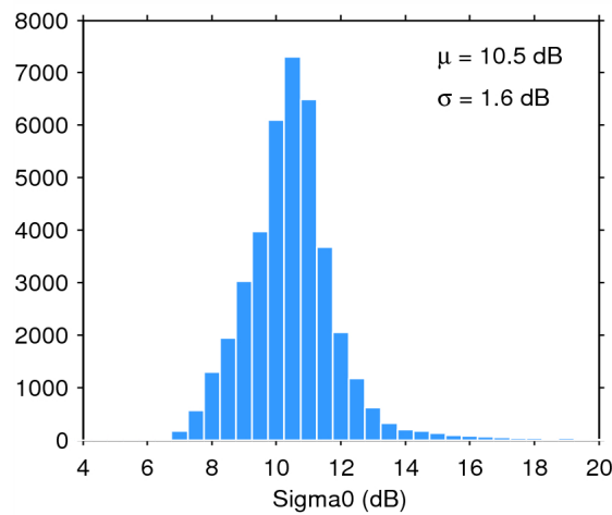
Figure 28. Histogram of science-valid sigma0 over oceans and lakes for 16/05/2015. The mean ( \mu ) and standard deviation ( \sigma ) are also shown. Note that values outside [4 20] dB are excluded from the histogram for the sake of readability but not from the computation of \mu and \sigma .
