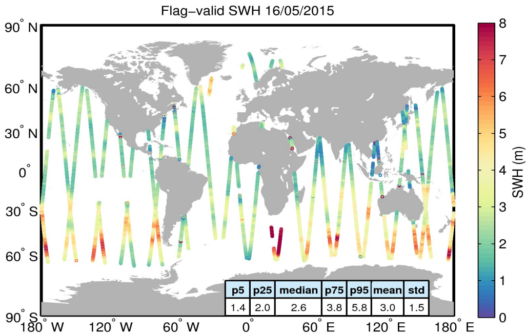
Figure 15. Geographical distribution of flag-valid SWH data over oceans and lakes for 16/05/2015. The statistical values shown in the table refer to the SWH in m and are calculated over all measurements shown in the figure.
