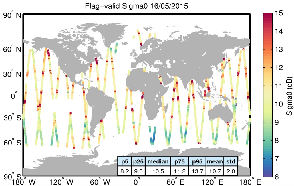
Figure 23. Geographical distribution of flag-valid sigma0 data over oceans and lakes for 16/05/2015. The statistical values shown in the table refer to the sigma0 in dB and are calculated over all measurements shown in the figure.
