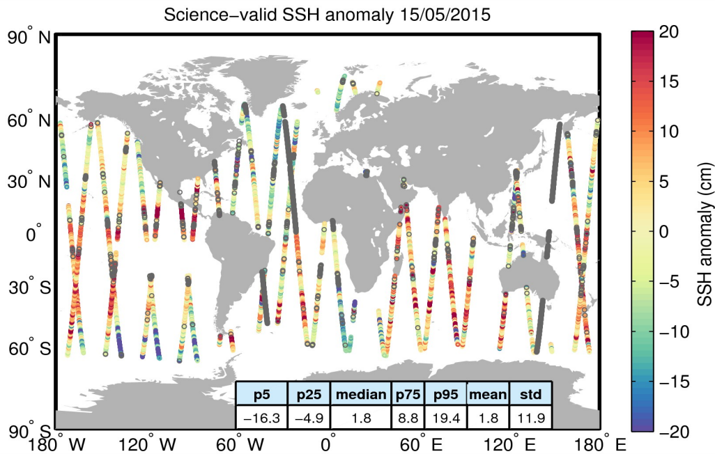
Figure 10. Geographical distribution of science-valid SSH anomaly data over oceans and lakes for 15/05/2015. The statistical values shown in the table refer to the SSH anomaly in cm and are calculated over all measurements shown in the figure. Gray circles denote records that have been rejected based on the editing criteria described in Table 2.
