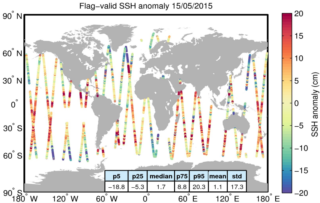
Figure 5. Geographical distribution of flag-valid 1-Hz SSH anomaly data over oceans and lakes for 15/05/2015. The statistical values shown in the table refer to the SSH anomaly in cm and are calculated over all measurements shown in the figure.
