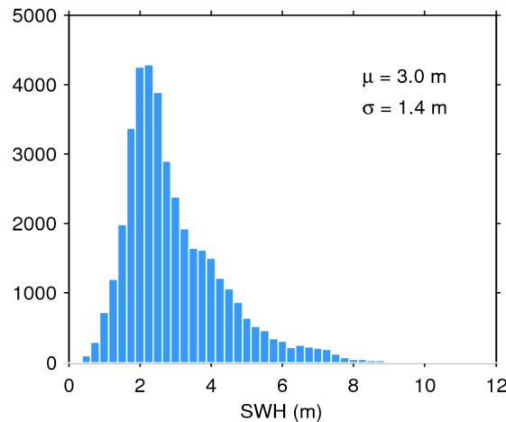
Figure 20. Histogram of science-valid SWH over oceans and lakes for 15/05/2015. The mean ( \mu ) and standard deviation ( \sigma ) are also shown. Note that values larger than 12 m are excluded from the histogram for the sake of readability but not from the computation of \mu and \sigma .
