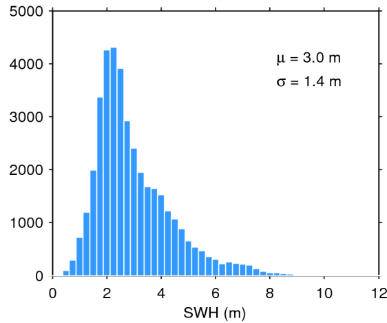
Figure 17. Histogram of flag-valid SWH over oceans and lakes for 15/05/2015. The mean ( \mu ) and standard deviation ( \sigma ) are also shown. Note that values larger than 12 m are excluded from the histogram for the sake of readability but not from the computation of \mu and \sigma .
