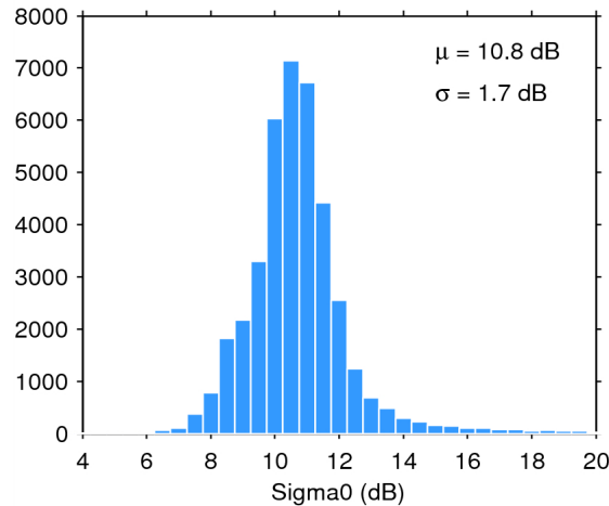
Figure 25. Histogram of flag-valid sigma0 over oceans and lakes for 15/05/2015. The mean ( \mu ) and standard deviation ( \sigma ) are also shown. Note that values outside [4 20] dB are excluded from the histogram for the sake of readability but not from the computation of \mu and \sigma .
