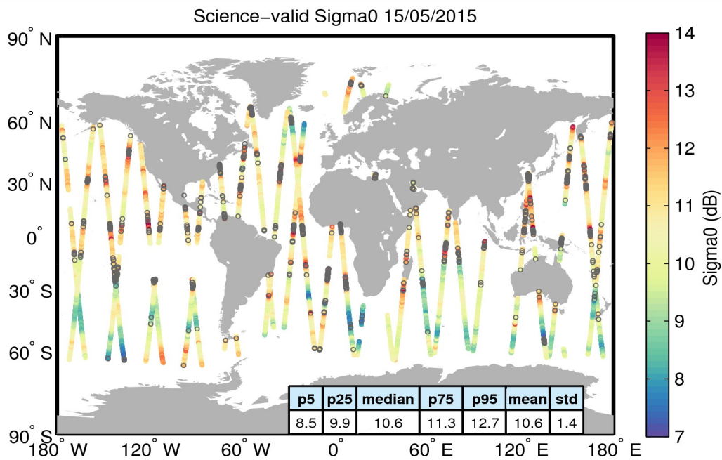
Figure 27. Geographical distribution of science-valid sigma0 data over oceans and lakes for 15/05/2015. The statistical values shown in the table refer to the sigma0 in dB and are calculated over all measurements shown in the figure. Gray circles denote records that have been rejected based on the editing criteria described in Table 4.
