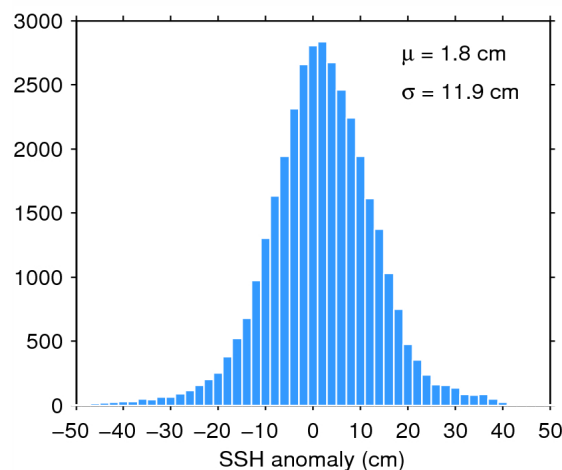
Figure 11. Histogram of science-valid SSH anomaly over oceans and lakes for 15/05/2015. The mean ( \mu ) and standard deviation ( \sigma ) are also shown. Note that values outside [-50 50] cm are excluded from the histogram for the sake of readability but not from the computation of \mu and \sigma .
