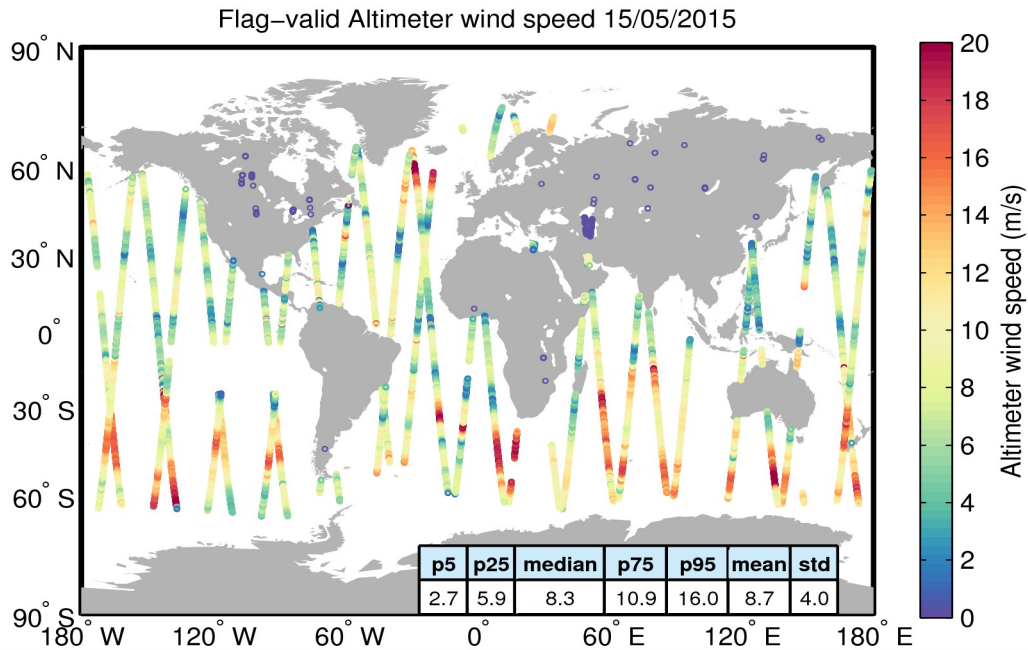
Figure 31. Geographical distribution of flag-valid wind data over oceans and lakes for 15/05/2015. The statistical values shown in the table refer to the wind in m/s and are calculated over all measurements shown in the figure.
