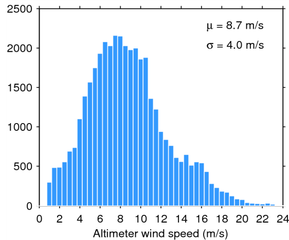
Figure 33. Histogram of flag-valid wind over oceans and lakes for 15/05/2015. The mean ( \mu ) and standard deviation ( \sigma ) are also shown. Note that values larger than 24 m/s are excluded from the histogram for the sake of readability but not from the computation of \mu and \sigma .
