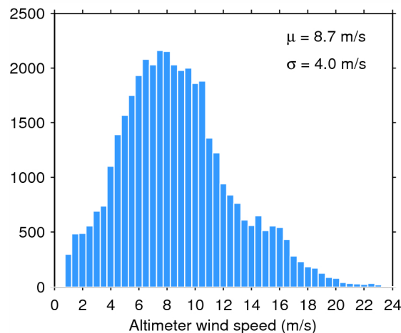
Figure 35. Histogram of science-valid wind over oceans and lakes for 15/05/2015. The mean ( \mu ) and standard deviation ( \sigma ) are also shown. Note that values larger than 24 m/s are excluded from the histogram for the sake of readability but not from the computation of \mu and \sigma .
