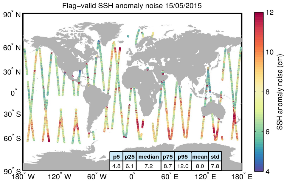
Figure 8. Geographical distribution of flag-valid 20-Hz SSH anomaly measurement noise over oceans and lakes for 15/05/2015. The statistical values shown in the table refer to the SSH anomaly noise and are calculated over all measurements shown in the figure.
