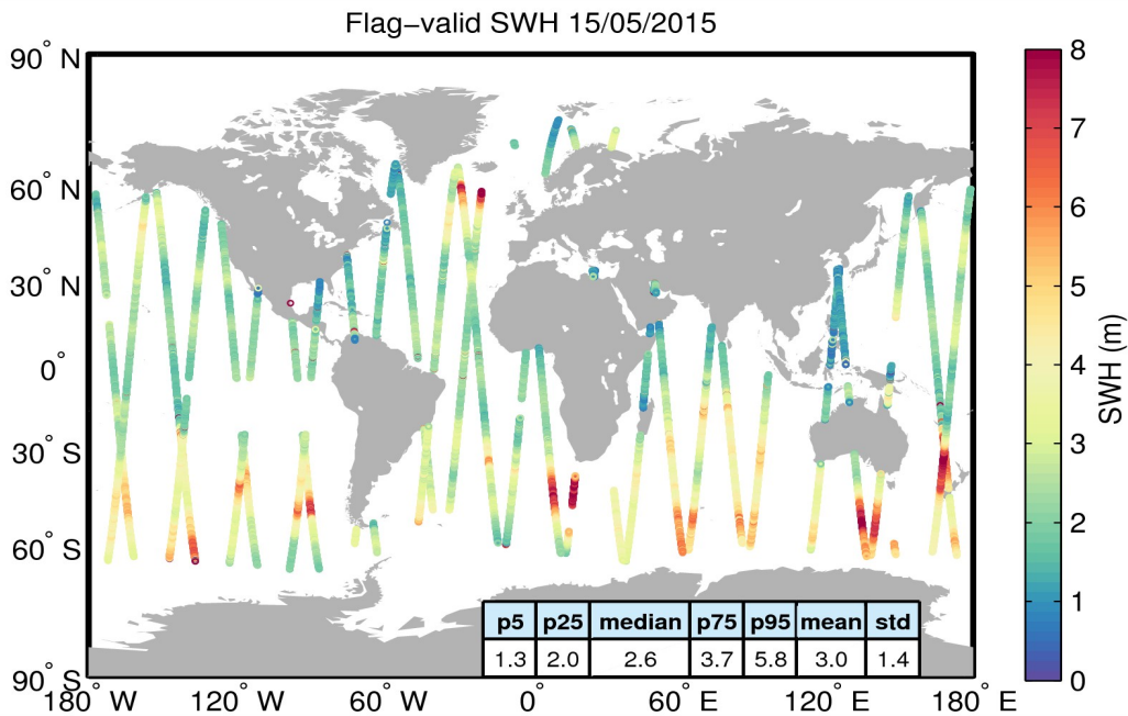
Figure 15. Geographical distribution of flag-valid SWH data over oceans and lakes for 15/05/2015. The statistical values shown in the table refer to the SWH in m and are calculated over all measurements shown in the figure.
