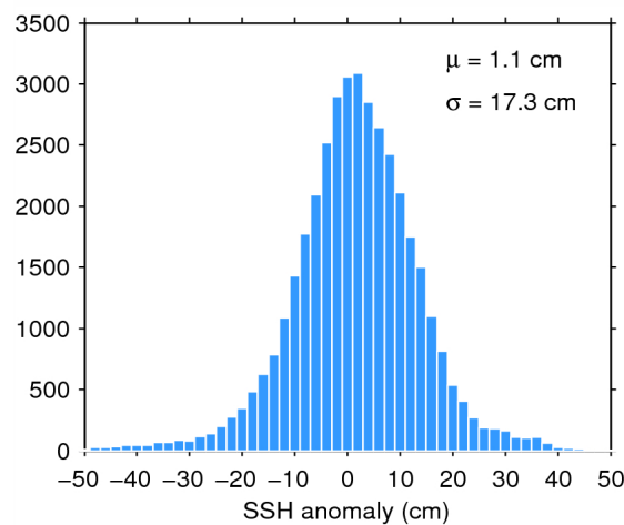
Figure 7. Histogram of flag-valid SSH anomaly over oceans and lakes for 15/05/2015. The mean ( \mu ) and standard deviation ( \sigma ) are also shown. Note that values outside [-50\ 50] cm are excluded from the histogram for the sake of readability but not from the computation of \mu and \sigma .
