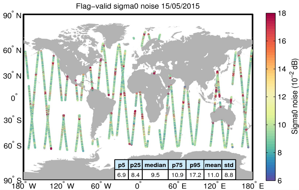
Figure 26. Geographical distribution of flag-valid 20-Hz sigma0 measurement noise over oceans and lakes for 15/05/2015. The statistical values shown in the table refer to the sigma0 noise and are calculated over all measurements shown in the figure.
