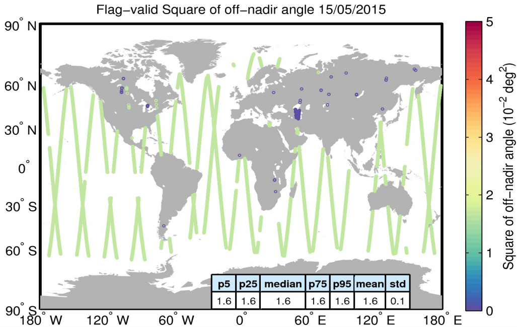
Figure 37. Geographical distribution of flag-valid mispointing data over oceans and lakes for 15/05/2015. The statistical values shown in the table refer to the mispointing in 10^{-2} deg 2 and are calculated over all measurements shown in the figure.
