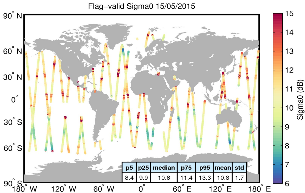
Figure 23. Geographical distribution of flag-valid sigma0 data over oceans and lakes for 15/05/2015. The statistical values shown in the table refer to the sigma0 in dB and are calculated over all measurements shown in the figure.
