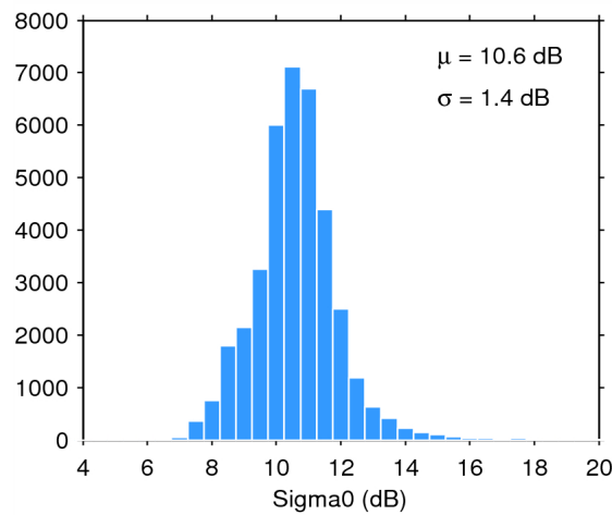
Figure 28. Histogram of science-valid sigma0 over oceans and lakes for 15/05/2015. The mean ( \mu ) and standard deviation ( \sigma ) are also shown. Note that values outside [4 20] dB are excluded from the histogram for the sake of readability but not from the computation of \mu and \sigma .
