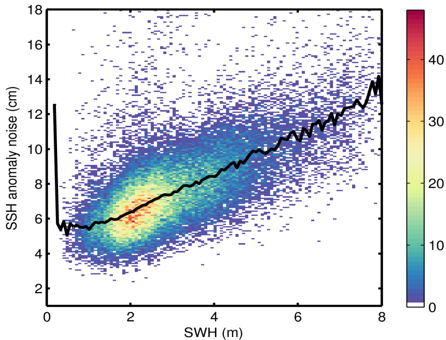
Figure 9. 2D histogram showing flag-valid SSH anomaly noise as a function of SWH for 15/05/2015. The black line denotes the median SSH anomaly as a function of SWH.
