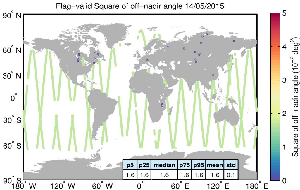
Figure 37. Geographical distribution of flag-valid mispointing data over oceans and lakes for 14/05/2015. The statistical values shown in the table refer to the mispointing in 10^{-2} deg 2 and are calculated over all measurements shown in the figure.
