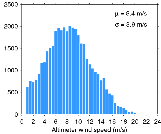
Figure 33. Histogram of flag-valid wind over oceans and lakes for 14/05/2015. The mean ( \mu ) and standard deviation ( \sigma ) are also shown. Note that values larger than 24 m/s are excluded from the histogram for the sake of readability but not from the computation of \mu and \sigma .
