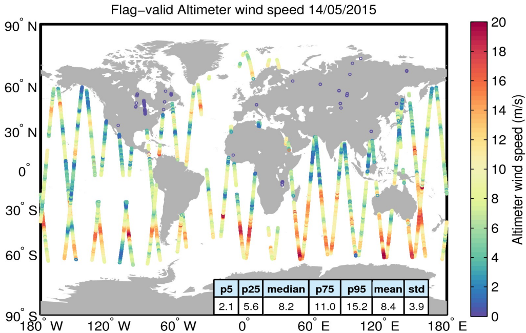
Figure 31. Geographical distribution of flag-valid wind data over oceans and lakes for 14/05/2015. The statistical values shown in the table refer to the wind in m/s and are calculated over all measurements shown in the figure.
