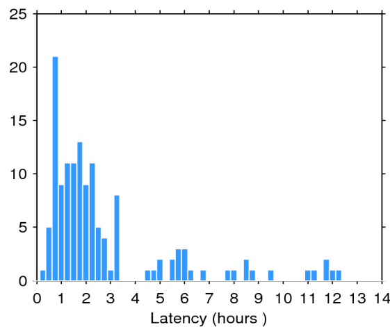
Figure 2. Histogram of the data latency for 14/05/2015. The y-axis denotes the number of files that are made available with a delay of x-hours with respect to the mean time of the records stored in the file.
