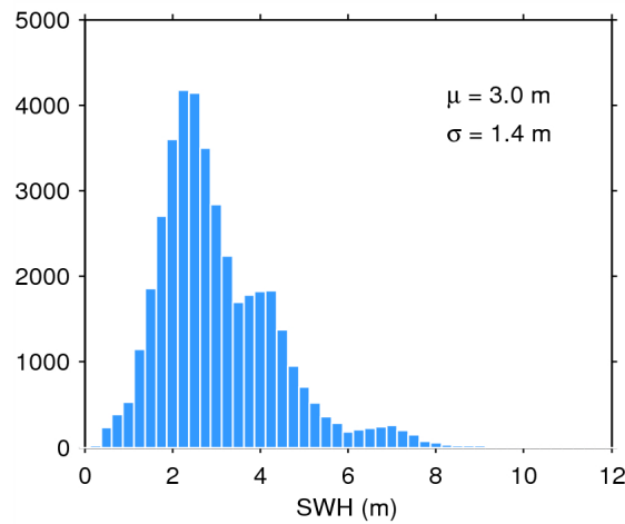
Figure 17. Histogram of flag-valid SWH over oceans and lakes for 14/05/2015. The mean ( \mu ) and standard deviation ( \sigma ) are also shown. Note that values larger than 12 m are excluded from the histogram for the sake of readability but not from the computation of \mu and \sigma .
