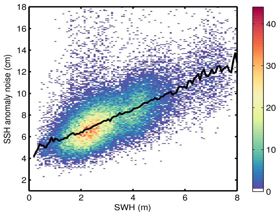
Figure 9. 2D histogram showing flag-valid SSH anomaly noise as a function of SWH for 14/05/2015. The black line denotes the median SSH anomaly as a function of SWH.
