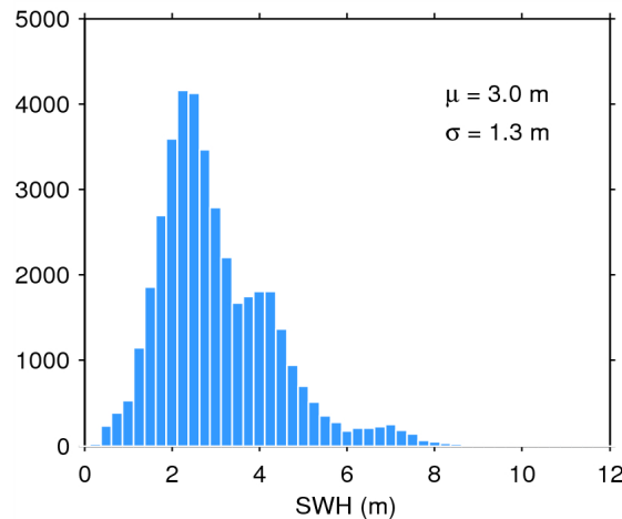
Figure 20. Histogram of science-valid SWH over oceans and lakes for 14/05/2015. The mean ( \mu ) and standard deviation ( \sigma ) are also shown. Note that values larger than 12 m are excluded from the histogram for the sake of readability but not from the computation of \mu and \sigma .
