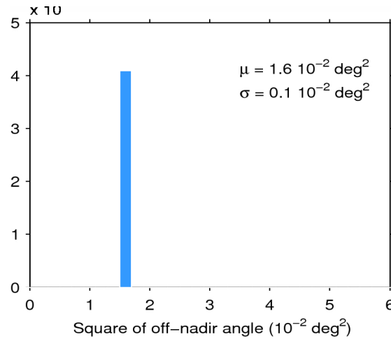
Figure 39. Histogram of flag-valid mispointing over oceans and lakes for 14/05/2015. The mean ( \mu ) and standard deviation ( \sigma ) are also shown. Note that values than 6 \times 10^{-2} \text{ deg}^2 are excluded from the histogram for the sake of readability but not from the computation of \mu and \sigma .
