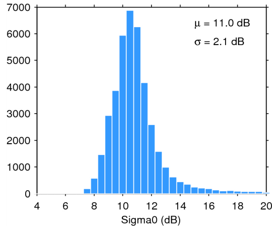
Figure 25. Histogram of flag-valid sigma0 over oceans and lakes for 14/05/2015. The mean ( \mu ) and standard deviation ( \sigma ) are also shown. Note that values outside [4 20] dB are excluded from the histogram for the sake of readability but not from the computation of \mu and \sigma .
