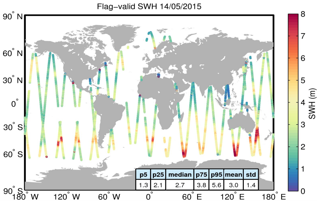
Figure 15. Geographical distribution of flag-valid SWH data over oceans and lakes for 14/05/2015. The statistical values shown in the table refer to the SWH in m and are calculated over all measurements shown in the figure.
