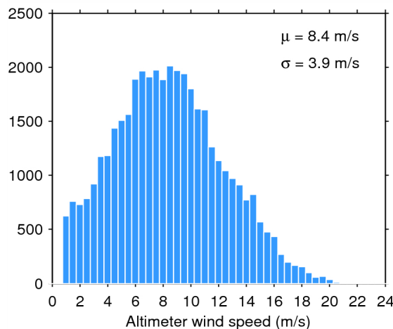
Figure 35. Histogram of science-valid wind over oceans and lakes for 14/05/2015. The mean ( \mu ) and standard deviation ( \sigma ) are also shown. Note that values larger than 24 m/s are excluded from the histogram for the sake of readability but not from the computation of \mu and \sigma .
