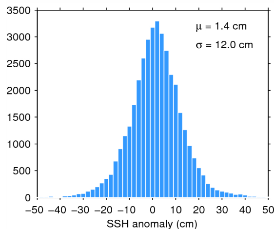
Figure 11. Histogram of science-valid SSH anomaly over oceans and lakes for 14/05/2015. The mean ( \mu ) and standard deviation ( \sigma ) are also shown. Note that values outside [-50 50] cm are excluded from the histogram for the sake of readability but not from the computation of \mu and \sigma .
