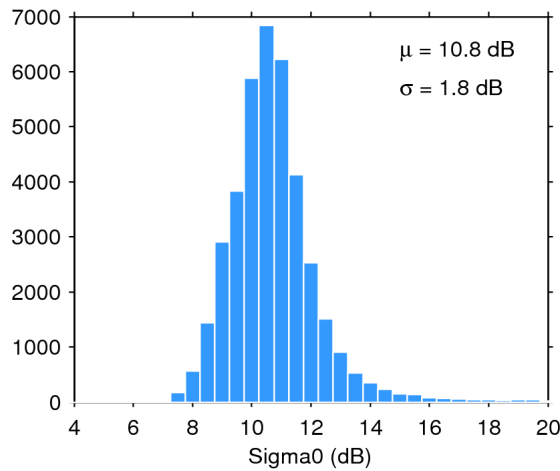
Figure 28. Histogram of science-valid sigma0 over oceans and lakes for 14/05/2015. The mean ( \mu ) and standard deviation ( \sigma ) are also shown. Note that values outside [4 20] dB are excluded from the histogram for the sake of readability but not from the computation of \mu and \sigma .
