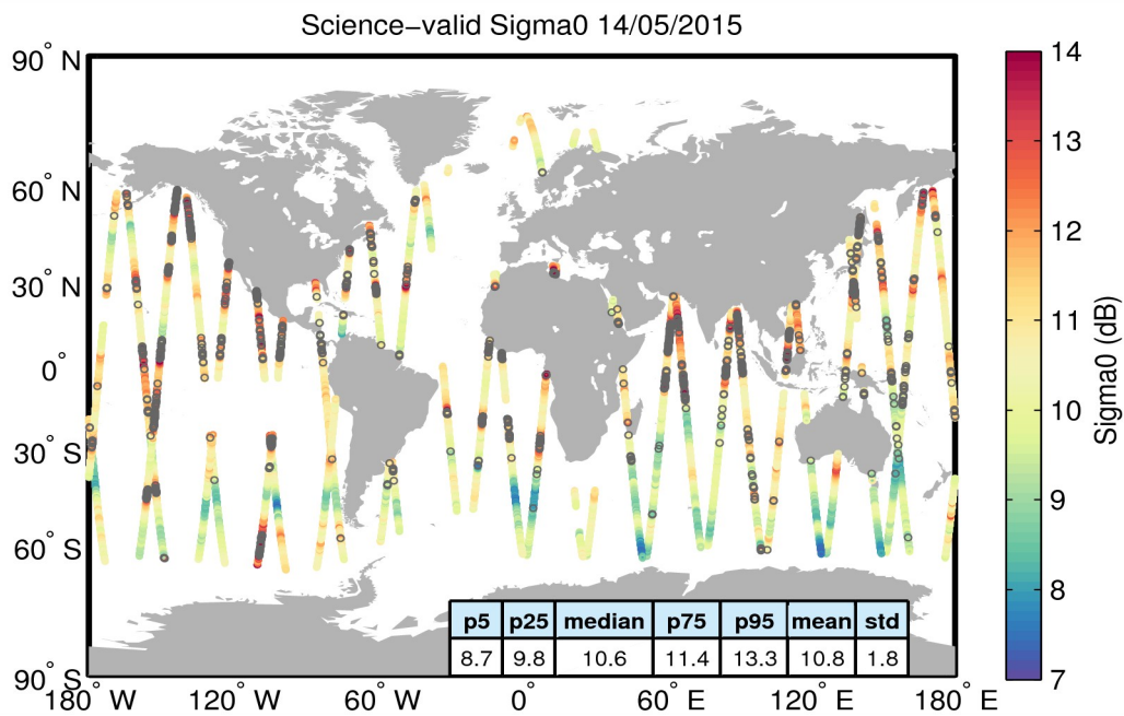
Figure 27. Geographical distribution of science-valid sigma0 data over oceans and lakes for 14/05/2015. The statistical values shown in the table refer to the sigma0 in dB and are calculated over all measurements shown in the figure. Gray circles denote records that have been rejected based on the editing criteria described in Table 4.
