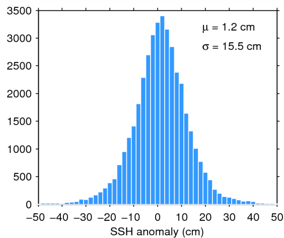
Figure 7. Histogram of flag-valid SSH anomaly over oceans and lakes for 14/05/2015. The mean ( \mu ) and standard deviation ( \sigma ) are also shown. Note that values outside [-50 50] cm are excluded from the histogram for the sake of readability but not from the computation of \mu and \sigma .
