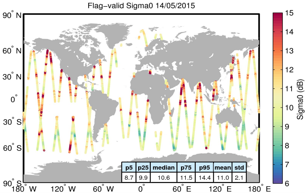
Figure 23. Geographical distribution of flag-valid sigma0 data over oceans and lakes for 14/05/2015. The statistical values shown in the table refer to the sigma0 in dB and are calculated over all measurements shown in the figure.
