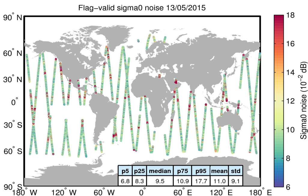
Figure 26. Geographical distribution of flag-valid 20-Hz sigma0 measurement noise over oceans and lakes for 13/05/2015. The statistical values shown in the table refer to the sigma0 noise and are calculated over all measurements shown in the figure.
