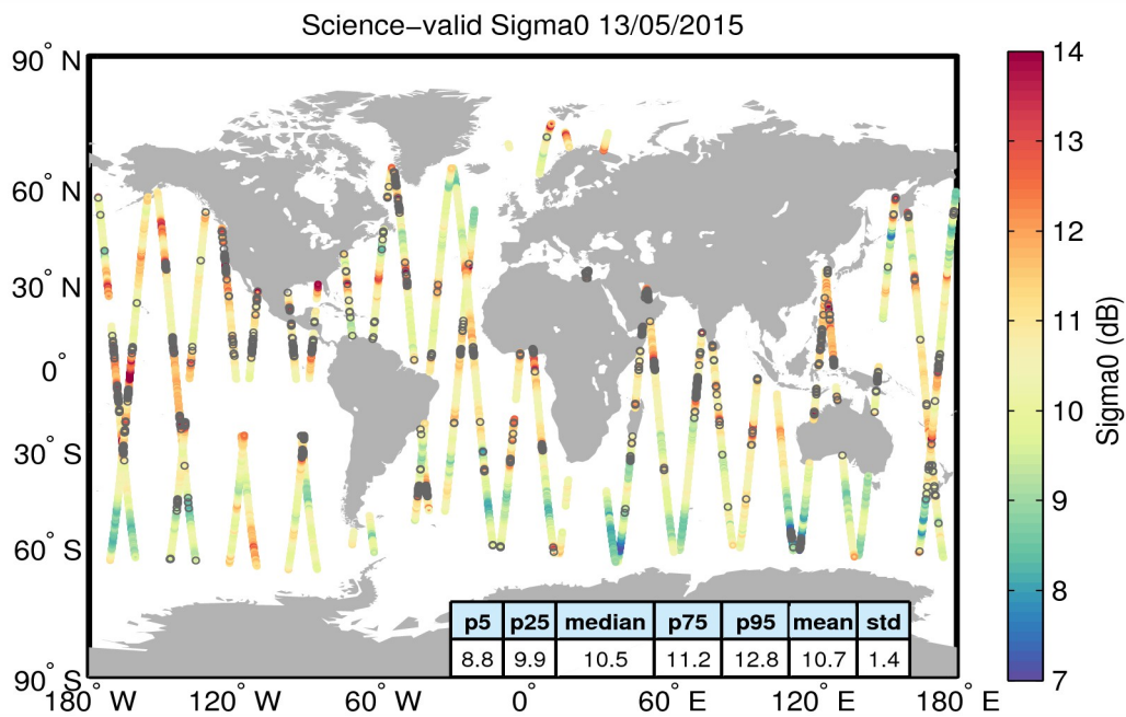
Figure 27. Geographical distribution of science-valid sigma0 data over oceans and lakes for 13/05/2015. The statistical values shown in the table refer to the sigma0 in dB and are calculated over all measurements shown in the figure. Gray circles denote records that have been rejected based on the editing criteria described in Table 4.
