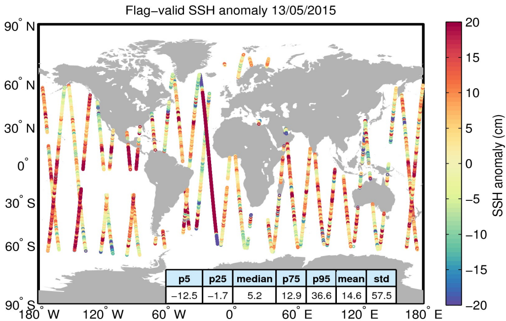
Figure 5. Geographical distribution of flag-valid 1-Hz SSH anomaly data over oceans and lakes for 13/05/2015. The statistical values shown in the table refer to the SSH anomaly in cm and are calculated over all measurements shown in the figure.
