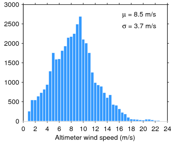
Figure 33. Histogram of flag-valid wind over oceans and lakes for 13/05/2015. The mean ( \mu ) and standard deviation ( \sigma ) are also shown. Note that values larger than 24 m/s are excluded from the histogram for the sake of readability but not from the computation of \mu and \sigma .
