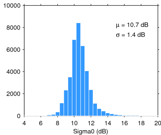
Figure 28. Histogram of science-valid sigma0 over oceans and lakes for 13/05/2015. The mean ( \mu ) and standard deviation ( \sigma ) are also shown. Note that values outside [4 20] dB are excluded from the histogram for the sake of readability but not from the computation of \mu and \sigma .
