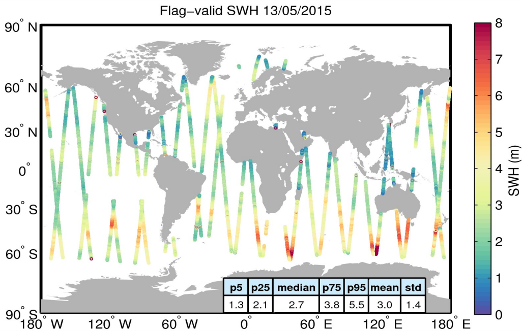
Figure 15. Geographical distribution of flag-valid SWH data over oceans and lakes for 13/05/2015. The statistical values shown in the table refer to the SWH in m and are calculated over all measurements shown in the figure.
