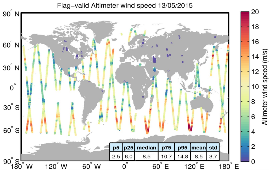
Figure 31. Geographical distribution of flag-valid wind data over oceans and lakes for 13/05/2015. The statistical values shown in the table refer to the wind in m/s and are calculated over all measurements shown in the figure.
