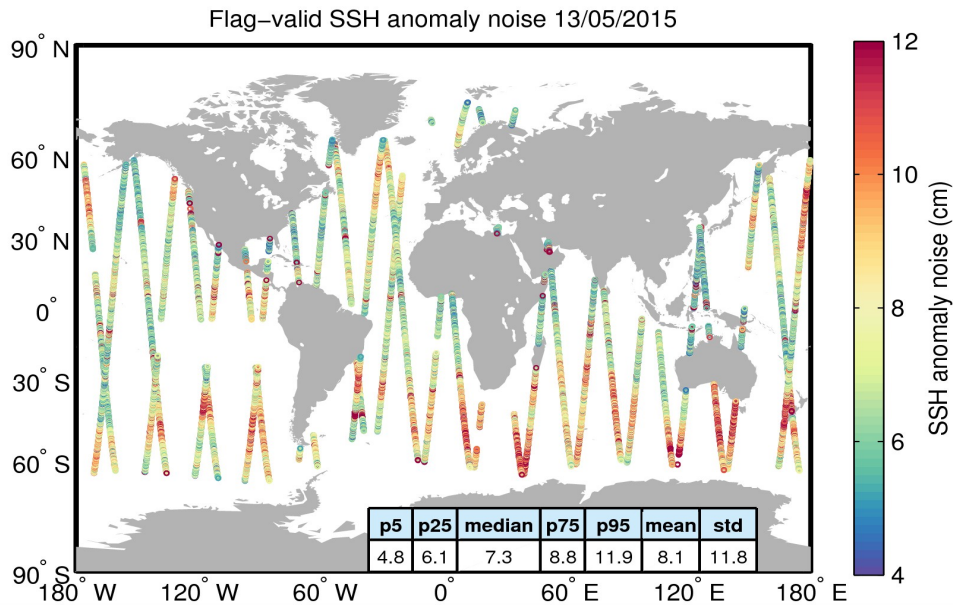
Figure 8. Geographical distribution of flag-valid 20-Hz SSH anomaly measurement noise over oceans and lakes for 13/05/2015. The statistical values shown in the table refer to the SSH anomaly noise and are calculated over all measurements shown in the figure.
