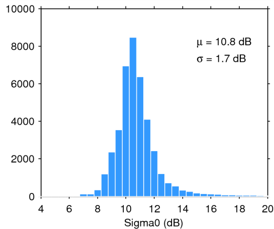
Figure 25. Histogram of flag-valid sigma0 over oceans and lakes for 13/05/2015. The mean ( \mu ) and standard deviation ( \sigma ) are also shown. Note that values outside [4 20] dB are excluded from the histogram for the sake of readability but not from the computation of \mu and \sigma .
