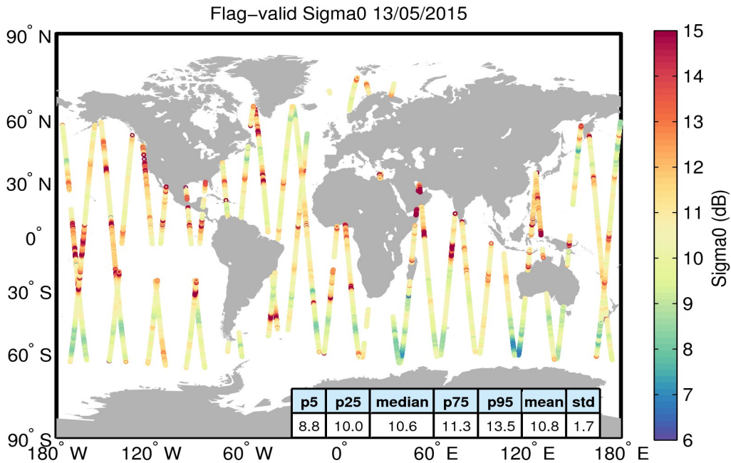
Figure 23. Geographical distribution of flag-valid sigma0 data over oceans and lakes for 13/05/2015. The statistical values shown in the table refer to the sigma0 in dB and are calculated over all measurements shown in the figure.
