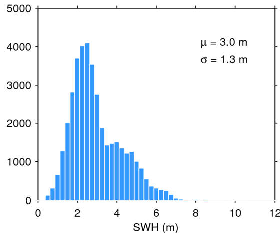
Figure 20. Histogram of science-valid SWH over oceans and lakes for 13/05/2015. The mean ( \mu ) and standard deviation ( \sigma ) are also shown. Note that values larger than 12 m are excluded from the histogram for the sake of readability but not from the computation of \mu and \sigma .
