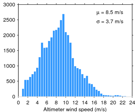
Figure 35. Histogram of science-valid wind over oceans and lakes for 13/05/2015. The mean ( \mu ) and standard deviation ( \sigma ) are also shown. Note that values larger than 24 m/s are excluded from the histogram for the sake of readability but not from the computation of \mu and \sigma .
