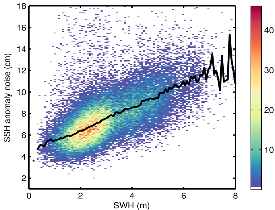
Figure 9. 2D histogram showing flag-valid SSH anomaly noise as a function of SWH for 13/05/2015. The black line denotes the median SSH anomaly as a function of SWH.
