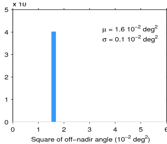
Figure 39. Histogram of flag-valid mispointing over oceans and lakes for 13/05/2015. The mean ( \mu ) and standard deviation ( \sigma ) are also shown. Note that values than 6 \cdot 10^{-2} \text{ deg}^2 are excluded from the histogram for the sake of readability but not from the computation of \mu and \sigma .
