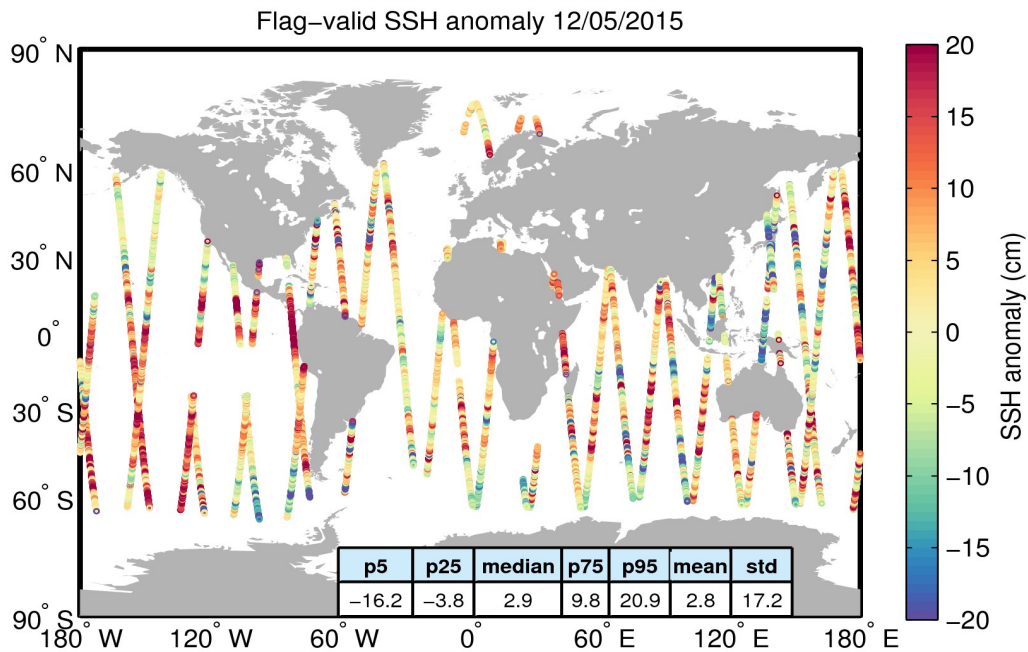
Figure 5. Geographical distribution of flag-valid 1-Hz SSH anomaly data over oceans and lakes for 12/05/2015. The statistical values shown in the table refer to the SSH anomaly in cm and are calculated over all measurements shown in the figure.
