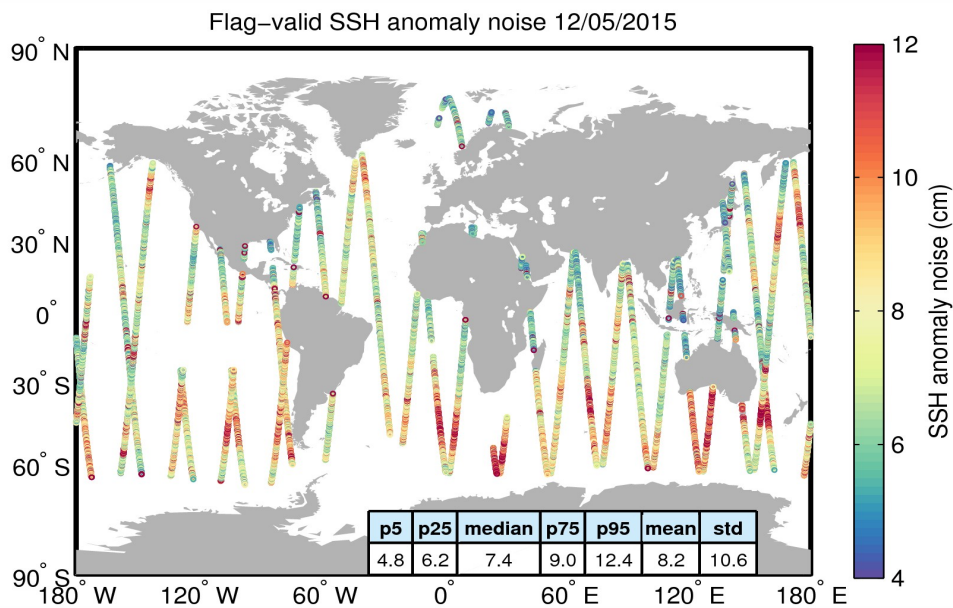
Figure 8. Geographical distribution of flag-valid 20-Hz SSH anomaly measurement noise over oceans and lakes for 12/05/2015. The statistical values shown in the table refer to the SSH anomaly noise and are calculated over all measurements shown in the figure.
