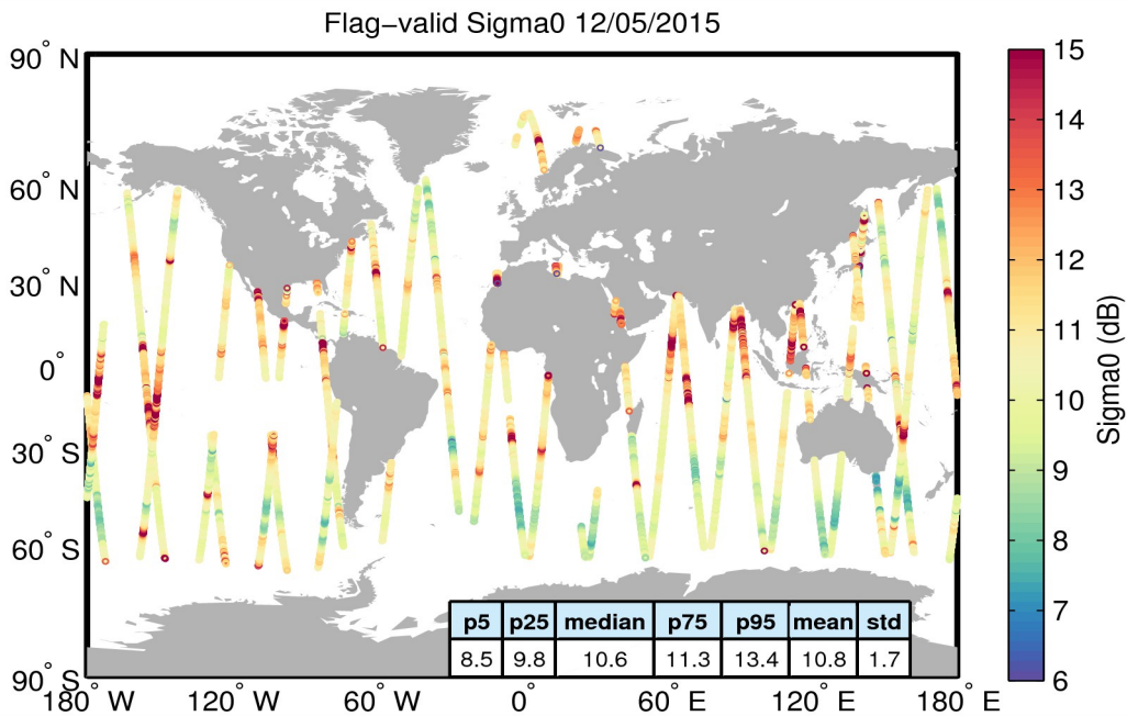
Figure 23. Geographical distribution of flag-valid sigma0 data over oceans and lakes for 12/05/2015. The statistical values shown in the table refer to the sigma0 in dB and are calculated over all measurements shown in the figure.
