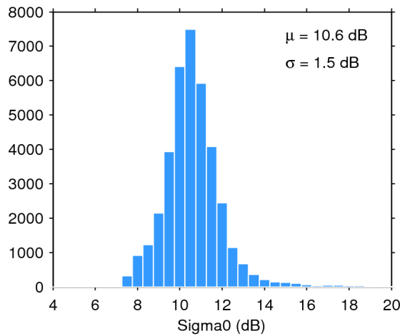
Figure 28. Histogram of science-valid sigma0 over oceans and lakes for 12/05/2015. The mean ( \mu ) and standard deviation ( \sigma ) are also shown. Note that values outside [4 20] dB are excluded from the histogram for the sake of readability but not from the computation of \mu and \sigma .
