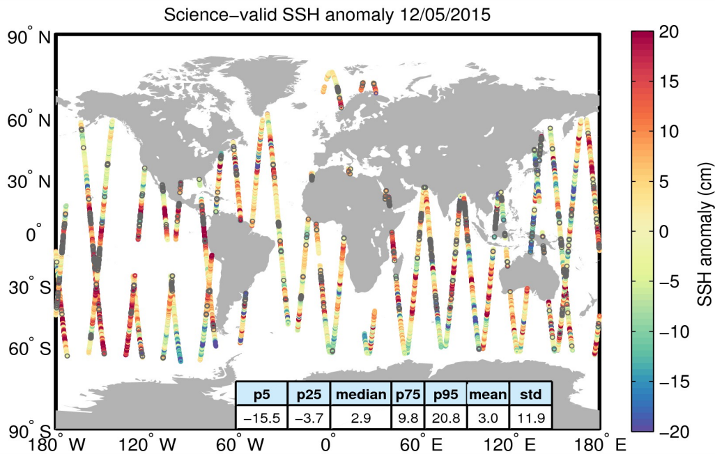
Figure 10. Geographical distribution of science-valid SSH anomaly data over oceans and lakes for 12/05/2015. The statistical values shown in the table refer to the SSH anomaly in cm and are calculated over all measurements shown in the figure. Gray circles denote records that have been rejected based on the editing criteria described in Table 2.
