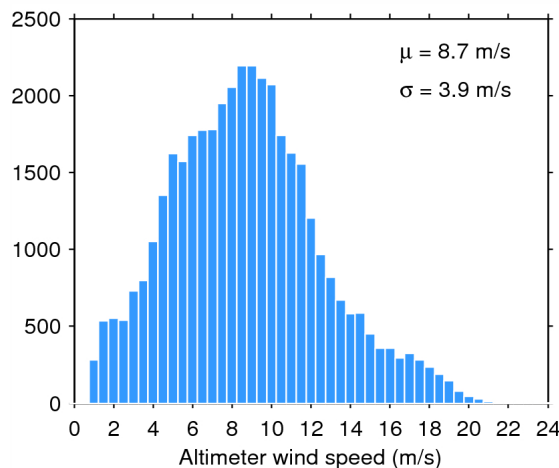
Figure 35. Histogram of science-valid wind over oceans and lakes for 12/05/2015. The mean ( \mu ) and standard deviation ( \sigma ) are also shown. Note that values larger than 24 m/s are excluded from the histogram for the sake of readability but not from the computation of \mu and \sigma .
