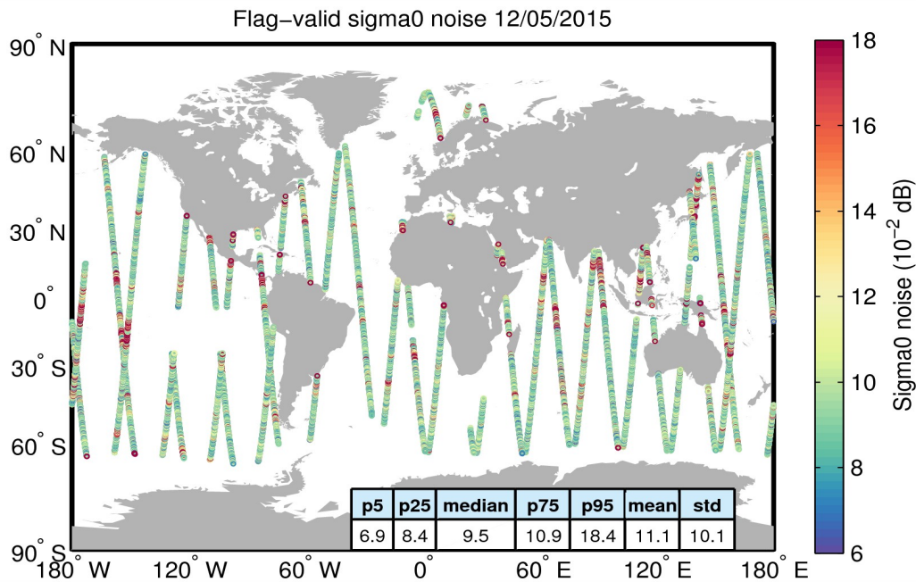
Figure 26. Geographical distribution of flag-valid 20-Hz sigma0 measurement noise over oceans and lakes for 12/05/2015. The statistical values shown in the table refer to the sigma0 noise and are calculated over all measurements shown in the figure.
