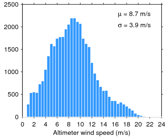
Figure 33. Histogram of flag-valid wind over oceans and lakes for 12/05/2015. The mean ( \mu ) and standard deviation ( \sigma ) are also shown. Note that values larger than 24 m/s are excluded from the histogram for the sake of readability but not from the computation of \mu and \sigma .
