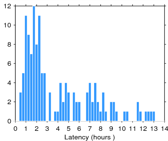
Figure 2. Histogram of the data latency for 12/05/2015. The y-axis denotes the number of files that are made available with a delay of x-hours with respect to the mean time of the records stored in the file.
