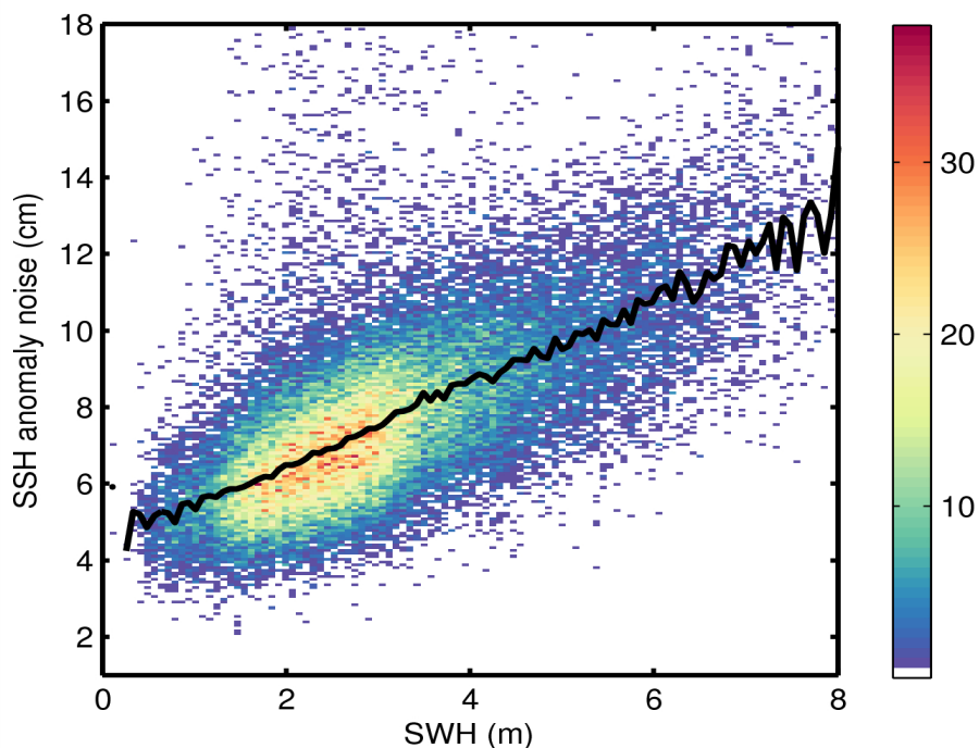
Figure 9. 2D histogram showing flag-valid SSH anomaly noise as a function of SWH for 12/05/2015. The black line denotes the median SSH anomaly as a function of SWH.
