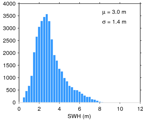
Figure 20. Histogram of science-valid SWH over oceans and lakes for 12/05/2015. The mean ( \mu ) and standard deviation ( \sigma ) are also shown. Note that values larger than 12 m are excluded from the histogram for the sake of readability but not from the computation of \mu and \sigma .
