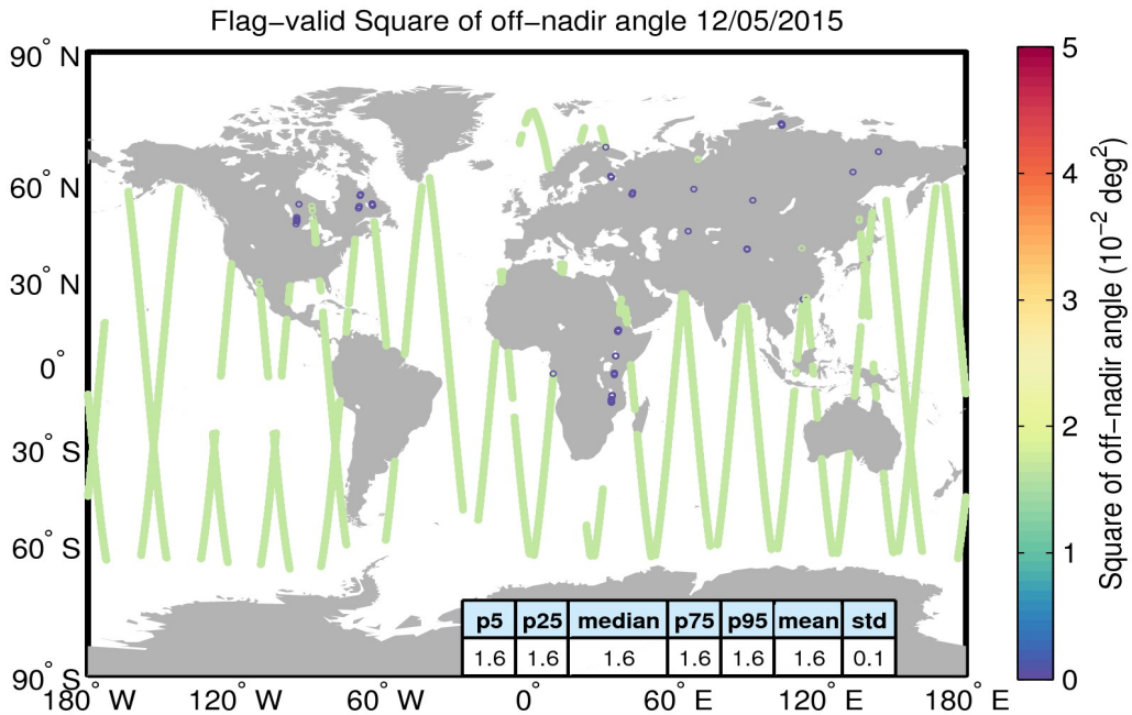
Figure 37. Geographical distribution of flag-valid mispointing data over oceans and lakes for 12/05/2015. The statistical values shown in the table refer to the mispointing in 10^{-2} \text{deg}^2 and are calculated over all measurements shown in the figure.
