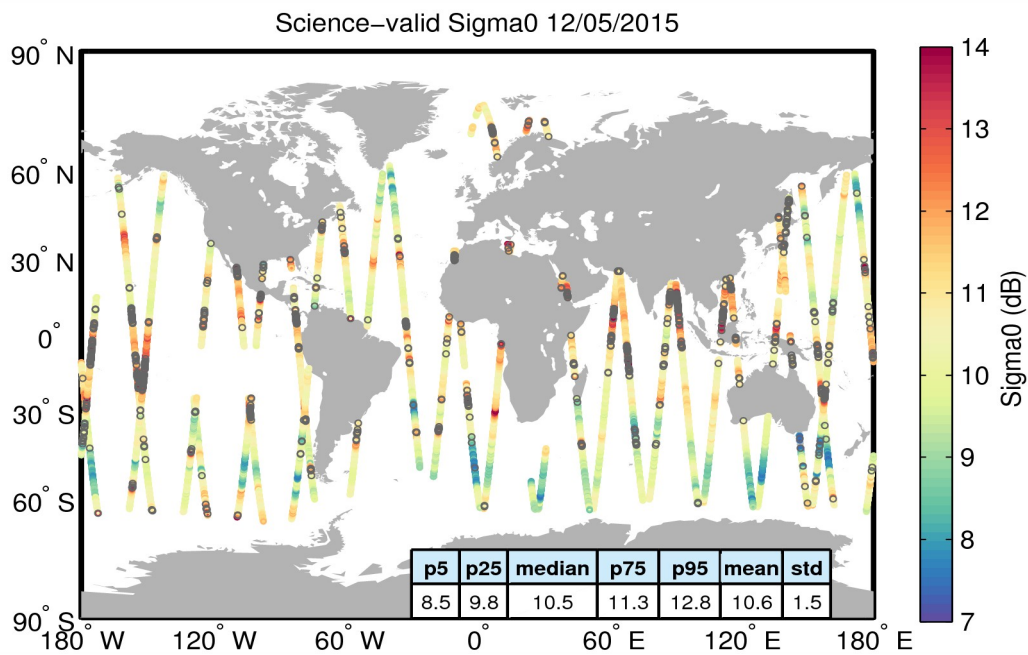
Figure 27. Geographical distribution of science-valid sigma0 data over oceans and lakes for 12/05/2015. The statistical values shown in the table refer to the sigma0 in dB and are calculated over all measurements shown in the figure. Gray circles denote records that have been rejected based on the editing criteria described in Table 4.
