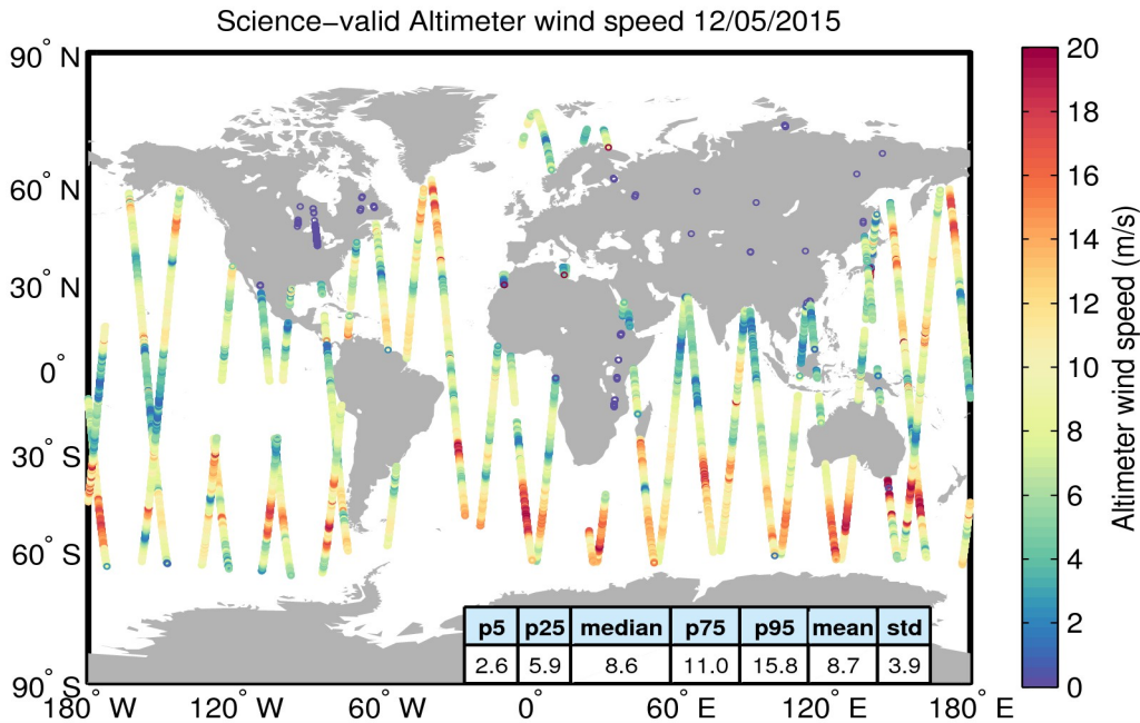
Figure 34. Geographical distribution of science-valid wind data over oceans and lakes for 12/05/2015. The statistical values shown in the table refer to the wind in m/s and are calculated over all measurements shown in the figure. Gray circles denote records that have been rejected based on the editing criteria described in Table 5.
