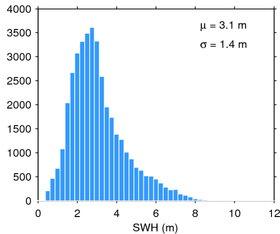
Figure 17. Histogram of flag-valid SWH over oceans and lakes for 12/05/2015. The mean ( \mu ) and standard deviation ( \sigma ) are also shown. Note that values larger than 12 m are excluded from the histogram for the sake of readability but not from the computation of \mu and \sigma .
