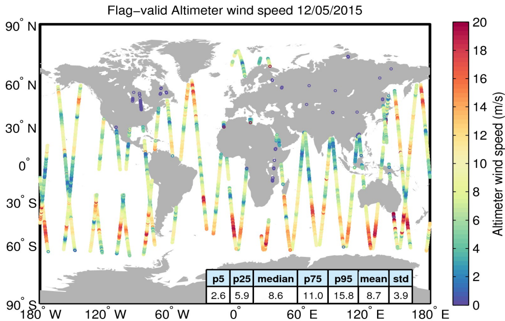
Figure 31. Geographical distribution of flag-valid wind data over oceans and lakes for 12/05/2015. The statistical values shown in the table refer to the wind in m/s and are calculated over all measurements shown in the figure.
