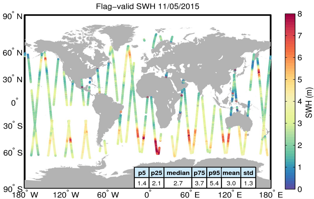
Figure 15. Geographical distribution of flag-valid SWH data over oceans and lakes for 11/05/2015. The statistical values shown in the table refer to the SWH in m and are calculated over all measurements shown in the figure.
