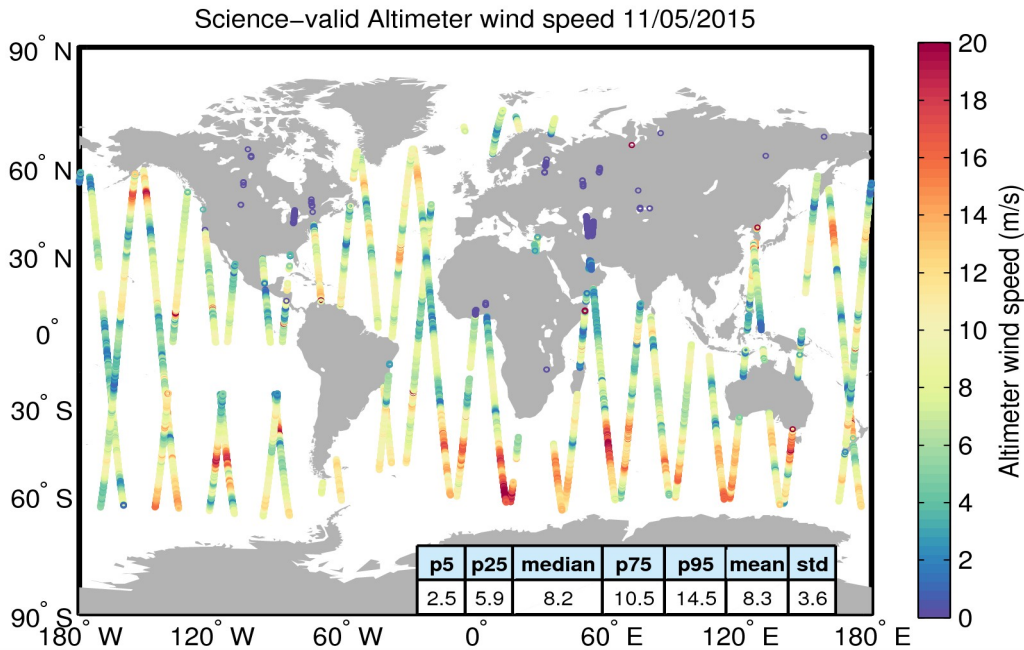
Figure 34. Geographical distribution of science-valid wind data over oceans and lakes for 11/05/2015. The statistical values shown in the table refer to the wind in m/s and are calculated over all measurements shown in the figure. Gray circles denote records that have been rejected based on the editing criteria described in Table 5.
