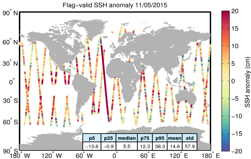
Figure 5. Geographical distribution of flag-valid 1-Hz SSH anomaly data over oceans and lakes for 11/05/2015. The statistical values shown in the table refer to the SSH anomaly in cm and are calculated over all measurements shown in the figure.
