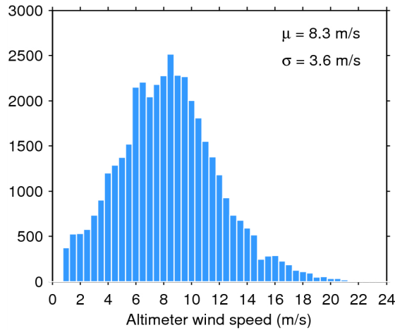
Figure 33. Histogram of flag-valid wind over oceans and lakes for 11/05/2015. The mean ( \mu ) and standard deviation ( \sigma ) are also shown. Note that values larger than 24 m/s are excluded from the histogram for the sake of readability but not from the computation of \mu and \sigma .
