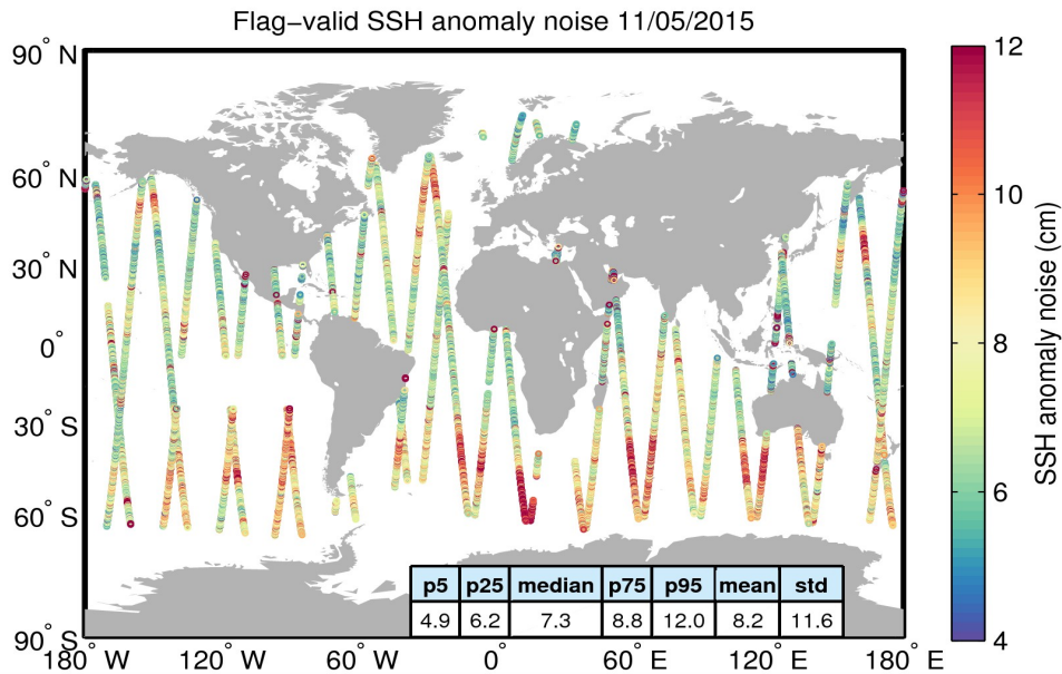
Figure 8. Geographical distribution of flag-valid 20-Hz SSH anomaly measurement noise over oceans and lakes for 11/05/2015. The statistical values shown in the table refer to the SSH anomaly noise and are calculated over all measurements shown in the figure.
