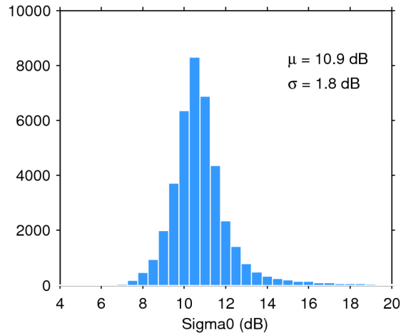
Figure 25. Histogram of flag-valid sigma0 over oceans and lakes for 11/05/2015. The mean ( \mu ) and standard deviation ( \sigma ) are also shown. Note that values outside [4 20] dB are excluded from the histogram for the sake of readability but not from the computation of \mu and \sigma .
