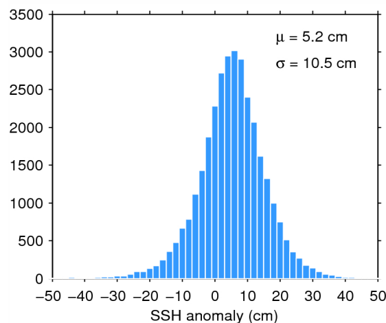
Figure 11. Histogram of science-valid SSH anomaly over oceans and lakes for 11/05/2015. The mean ( \mu ) and standard deviation ( \sigma ) are also shown. Note that values outside [-50 50] cm are excluded from the histogram for the sake of readability but not from the computation of \mu and \sigma .
