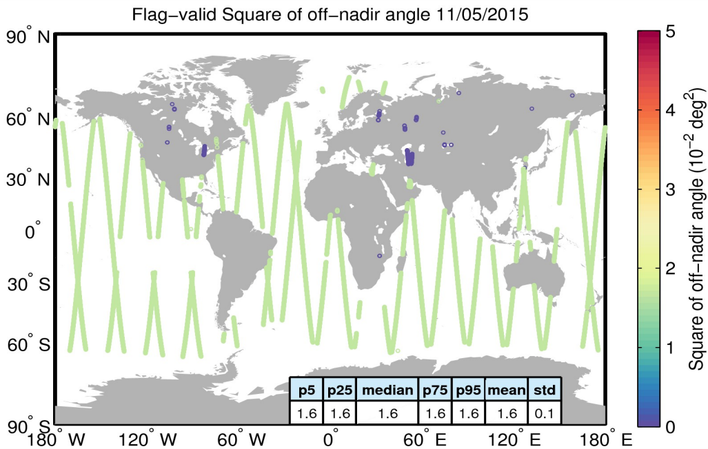
Figure 37. Geographical distribution of flag-valid mispointing data over oceans and lakes for 11/05/2015. The statistical values shown in the table refer to the mispointing in 10^{-2} deg 2 and are calculated over all measurements shown in the figure.
