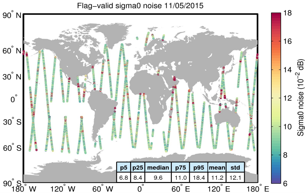
Figure 26. Geographical distribution of flag-valid 20-Hz sigma0 measurement noise over oceans and lakes for 11/05/2015. The statistical values shown in the table refer to the sigma0 noise and are calculated over all measurements shown in the figure.
