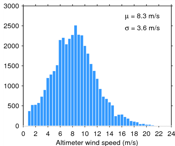
Figure 35. Histogram of science-valid wind over oceans and lakes for 11/05/2015. The mean ( \mu ) and standard deviation ( \sigma ) are also shown. Note that values larger than 24 m/s are excluded from the histogram for the sake of readability but not from the computation of \mu and \sigma .
