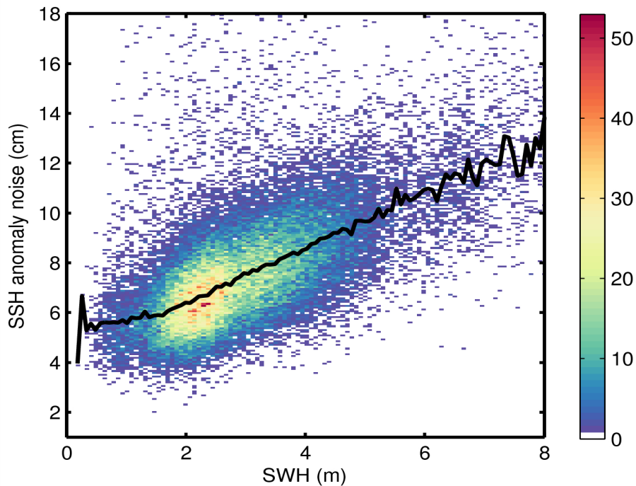
Figure 9. 2D histogram showing flag-valid SSH anomaly noise as a function of SWH for 11/05/2015. The black line denotes the median SSH anomaly as a function of SWH.
