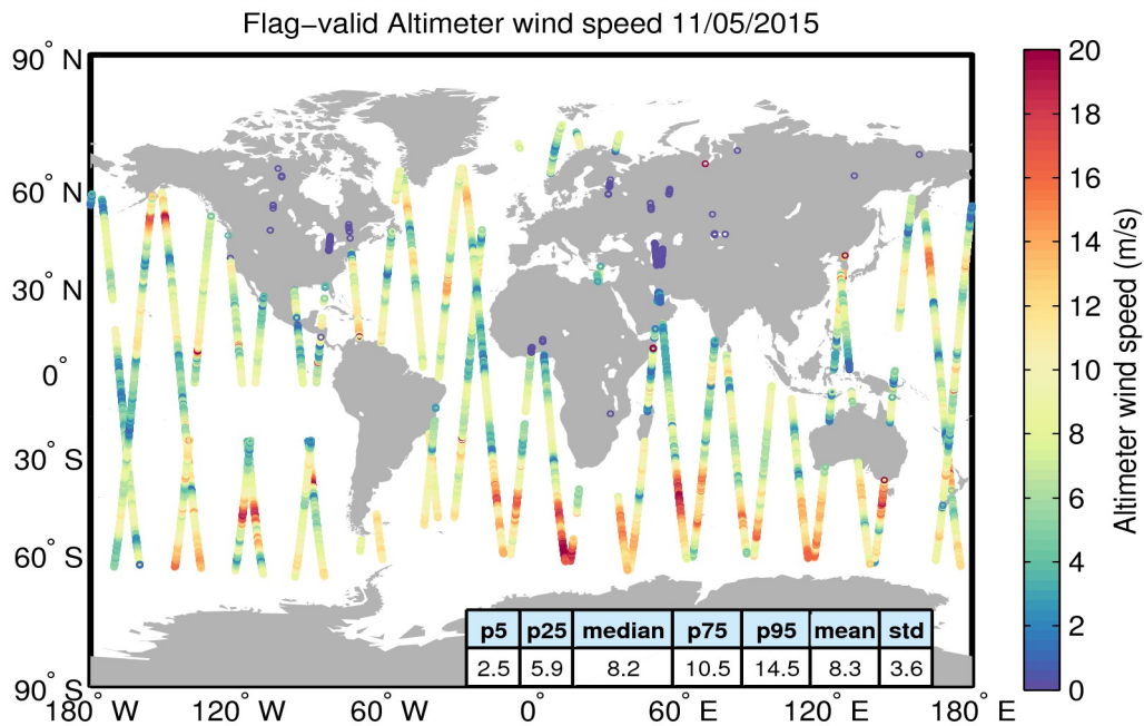
Figure 31. Geographical distribution of flag-valid wind data over oceans and lakes for 11/05/2015. The statistical values shown in the table refer to the wind in m/s and are calculated over all measurements shown in the figure.
