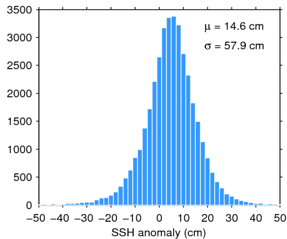
Figure 7. Histogram of flag-valid SSH anomaly over oceans and lakes for 11/05/2015. The mean ( \mu ) and standard deviation ( \sigma ) are also shown. Note that values outside [-50\ 50] cm are excluded from the histogram for the sake of readability but not from the computation of \mu and \sigma .
