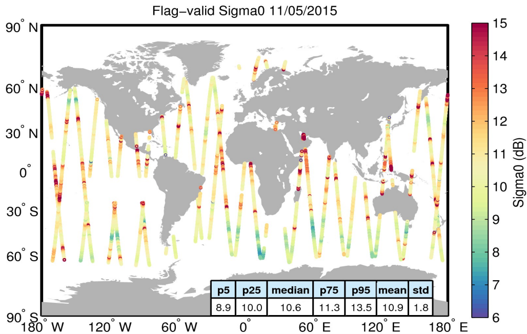
Figure 23. Geographical distribution of flag-valid sigma0 data over oceans and lakes for 11/05/2015. The statistical values shown in the table refer to the sigma0 in dB and are calculated over all measurements shown in the figure.
