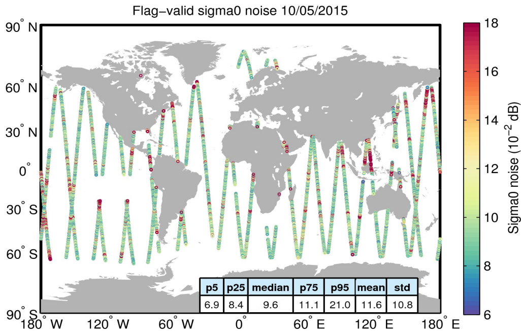
Figure 26. Geographical distribution of flag-valid 20-Hz sigma0 measurement noise over oceans and lakes for 10/05/2015. The statistical values shown in the table refer to the sigma0 noise and are calculated over all measurements shown in the figure.
