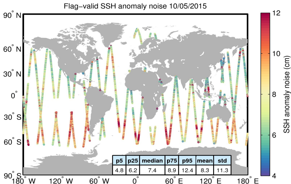
Figure 8. Geographical distribution of flag-valid 20-Hz SSH anomaly measurement noise over oceans and lakes for 10/05/2015. The statistical values shown in the table refer to the SSH anomaly noise and are calculated over all measurements shown in the figure.
