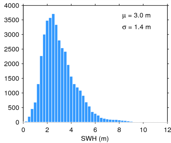
Figure 17. Histogram of flag-valid SWH over oceans and lakes for 10/05/2015. The mean ( \mu ) and standard deviation ( \sigma ) are also shown. Note that values larger than 12 m are excluded from the histogram for the sake of readability but not from the computation of \mu and \sigma .
