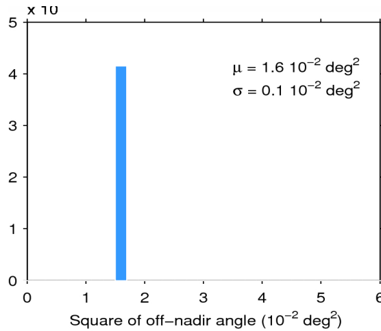
Figure 39. Histogram of flag-valid mispointing over oceans and lakes for 10/05/2015. The mean ( \mu ) and standard deviation ( \sigma ) are also shown. Note that values than 6 \cdot 10^{-2} \text{ deg}^2 are excluded from the histogram for the sake of readability but not from the computation of \mu and \sigma .
