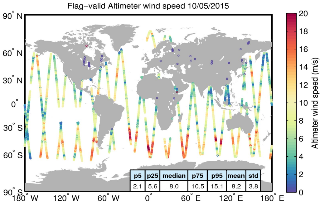
Figure 31. Geographical distribution of flag-valid wind data over oceans and lakes for 10/05/2015. The statistical values shown in the table refer to the wind in m/s and are calculated over all measurements shown in the figure.
