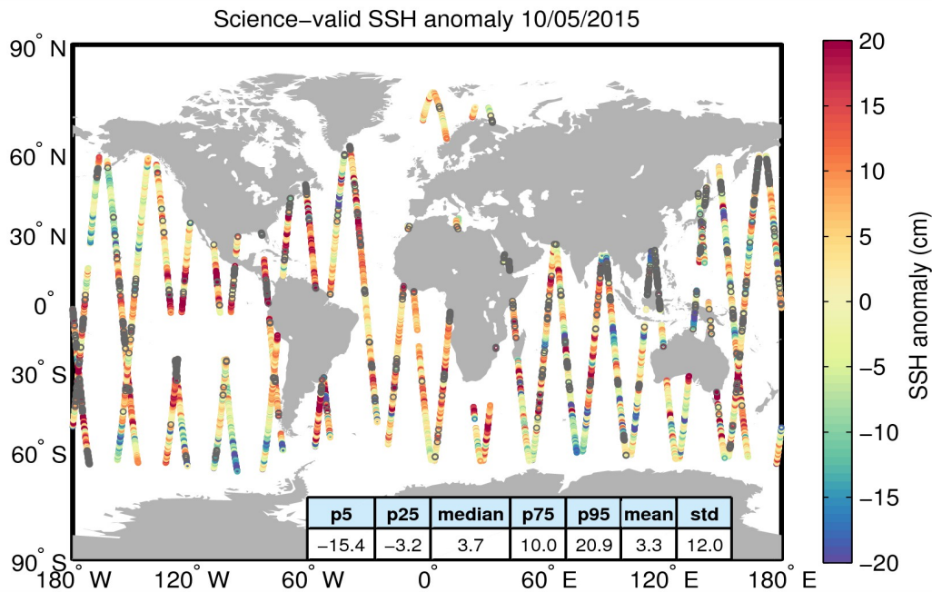
Figure 10. Geographical distribution of science-valid SSH anomaly data over oceans and lakes for 10/05/2015. The statistical values shown in the table refer to the SSH anomaly in cm and are calculated over all measurements shown in the figure. Gray circles denote records that have been rejected based on the editing criteria described in Table 2.
