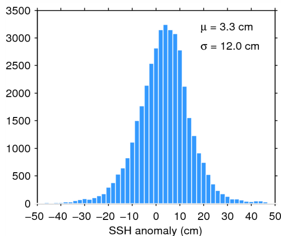
Figure 11. Histogram of science-valid SSH anomaly over oceans and lakes for 10/05/2015. The mean ( \mu ) and standard deviation ( \sigma ) are also shown. Note that values outside [-50 50] cm are excluded from the histogram for the sake of readability but not from the computation of \mu and \sigma .
