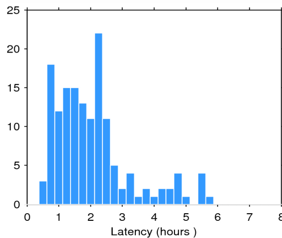
Figure 2. Histogram of the data latency for 10/05/2015. The y-axis denotes the number of files that are made available with a delay of x-hours with respect to the mean time of the records stored in the file.
