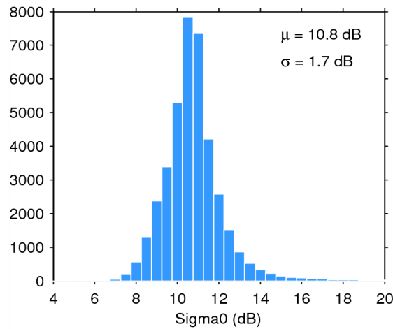
Figure 28. Histogram of science-valid sigma0 over oceans and lakes for 10/05/2015. The mean ( \mu ) and standard deviation ( \sigma ) are also shown. Note that values outside [4 20] dB are excluded from the histogram for the sake of readability but not from the computation of \mu and \sigma .
