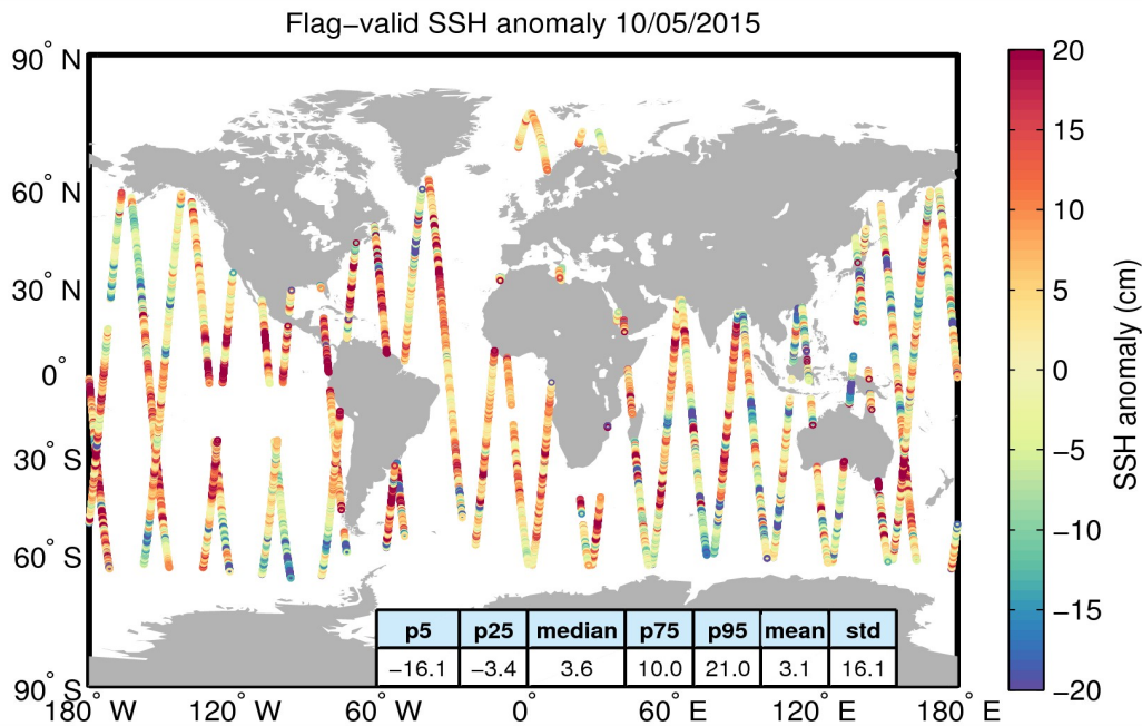
Figure 5. Geographical distribution of flag-valid 1-Hz SSH anomaly data over oceans and lakes for 10/05/2015. The statistical values shown in the table refer to the SSH anomaly in cm and are calculated over all measurements shown in the figure.
