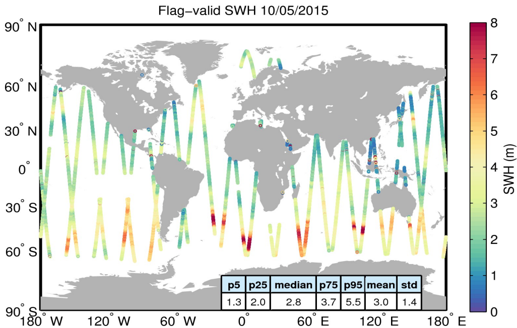
Figure 15. Geographical distribution of flag-valid SWH data over oceans and lakes for 10/05/2015. The statistical values shown in the table refer to the SWH in m and are calculated over all measurements shown in the figure.
