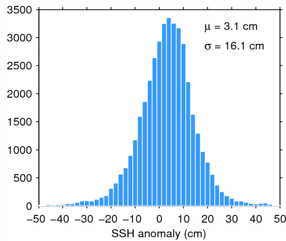
Figure 7. Histogram of flag-valid SSH anomaly over oceans and lakes for 10/05/2015. The mean ( \mu ) and standard deviation ( \sigma ) are also shown. Note that values outside [-50\ 50] cm are excluded from the histogram for the sake of readability but not from the computation of \mu and \sigma .
