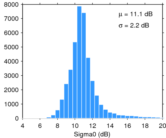
Figure 25. Histogram of flag-valid sigma0 over oceans and lakes for 10/05/2015. The mean ( \mu ) and standard deviation ( \sigma ) are also shown. Note that values outside [4 20] dB are excluded from the histogram for the sake of readability but not from the computation of \mu and \sigma .
