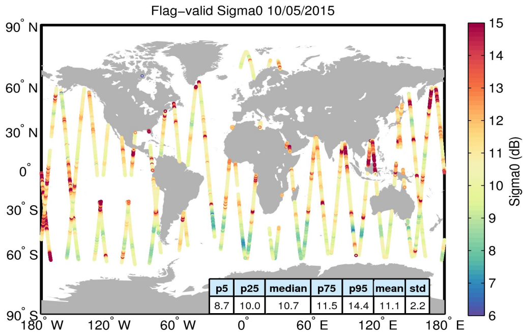
Figure 23. Geographical distribution of flag-valid sigma0 data over oceans and lakes for 10/05/2015. The statistical values shown in the table refer to the sigma0 in dB and are calculated over all measurements shown in the figure.
