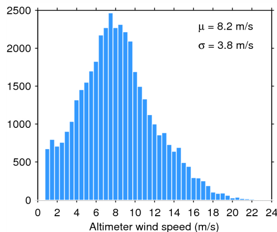
Figure 35. Histogram of science-valid wind over oceans and lakes for 10/05/2015. The mean ( \mu ) and standard deviation ( \sigma ) are also shown. Note that values larger than 24 m/s are excluded from the histogram for the sake of readability but not from the computation of \mu and \sigma .
