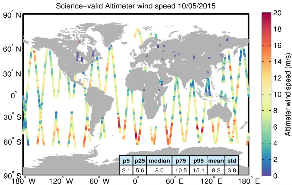
Figure 34. Geographical distribution of science-valid wind data over oceans and lakes for 10/05/2015. The statistical values shown in the table refer to the wind in m/s and are calculated over all measurements shown in the figure. Gray circles denote records that have been rejected based on the editing criteria described in Table 5.
