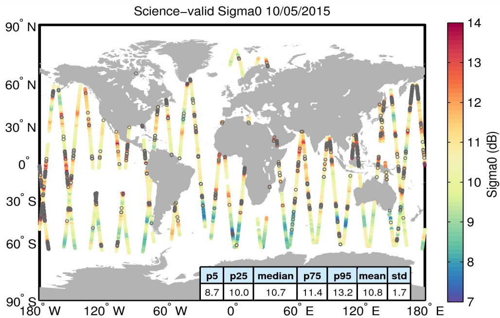
Figure 27. Geographical distribution of science-valid sigma0 data over oceans and lakes for 10/05/2015. The statistical values shown in the table refer to the sigma0 in dB and are calculated over all measurements shown in the figure. Gray circles denote records that have been rejected based on the editing criteria described in Table 4.
