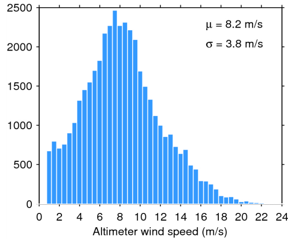
Figure 33. Histogram of flag-valid wind over oceans and lakes for 10/05/2015. The mean ( \mu ) and standard deviation ( \sigma ) are also shown. Note that values larger than 24 m/s are excluded from the histogram for the sake of readability but not from the computation of \mu and \sigma .
