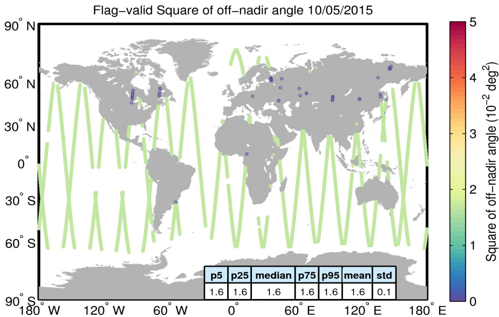
Figure 37. Geographical distribution of flag-valid mispointing data over oceans and lakes for 10/05/2015. The statistical values shown in the table refer to the mispointing in 10^{-2} deg 2 and are calculated over all measurements shown in the figure.
