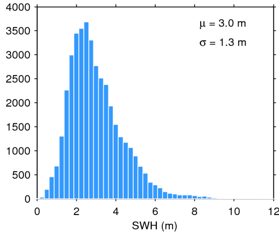
Figure 20. Histogram of science-valid SWH over oceans and lakes for 10/05/2015. The mean ( \mu ) and standard deviation ( \sigma ) are also shown. Note that values larger than 12 m are excluded from the histogram for the sake of readability but not from the computation of \mu and \sigma .
