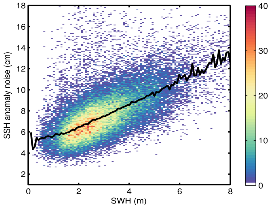
Figure 9. 2D histogram showing flag-valid SSH anomaly noise as a function of SWH for 10/05/2015. The black line denotes the median SSH anomaly as a function of SWH.
