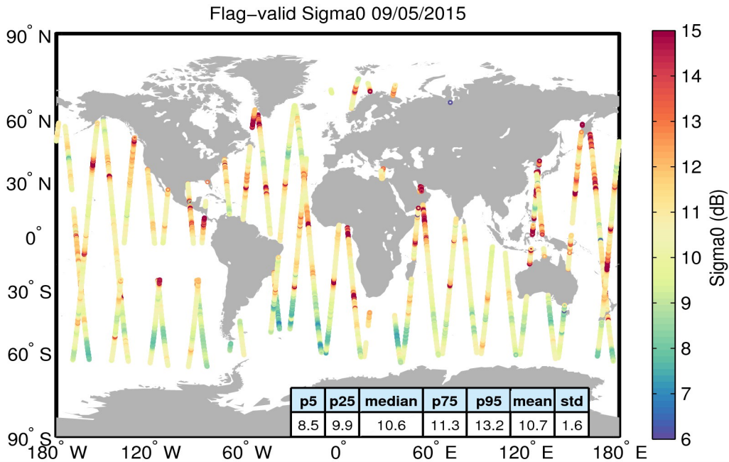
Figure 23. Geographical distribution of flag-valid sigma0 data over oceans and lakes for 09/05/2015. The statistical values shown in the table refer to the sigma0 in dB and are calculated over all measurements shown in the figure.
