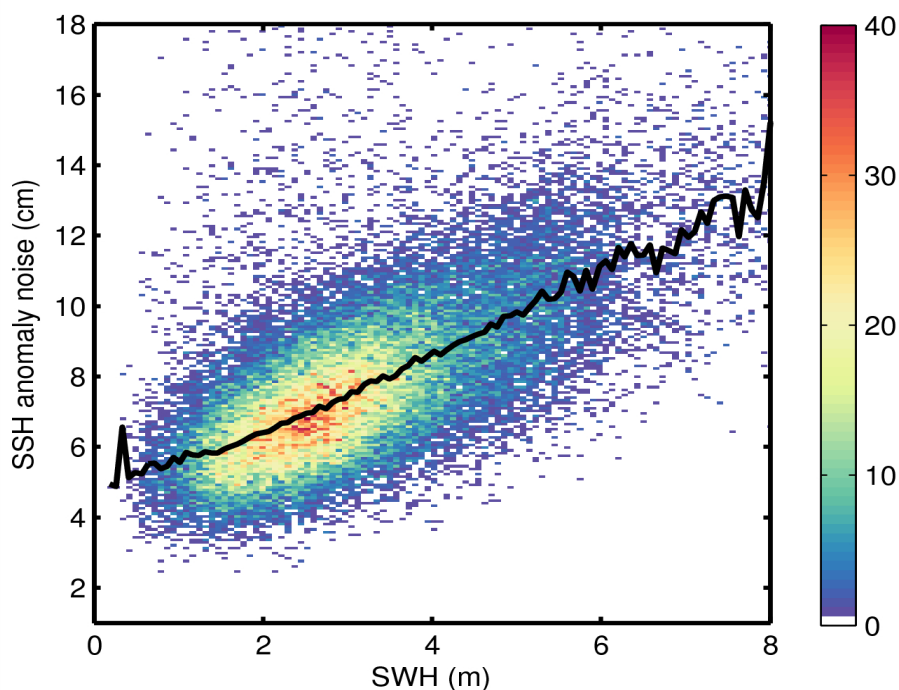
Figure 9. 2D histogram showing flag-valid SSH anomaly noise as a function of SWH for 09/05/2015. The black line denotes the median SSH anomaly as a function of SWH.
