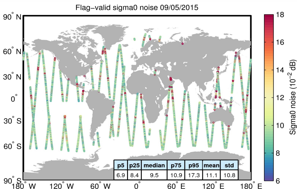
Figure 26. Geographical distribution of flag-valid 20-Hz sigma0 measurement noise over oceans and lakes for 09/05/2015. The statistical values shown in the table refer to the sigma0 noise and are calculated over all measurements shown in the figure.
