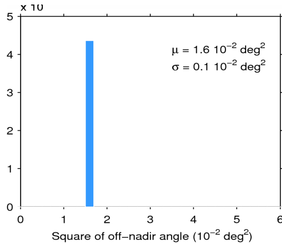
Figure 39. Histogram of flag-valid mispointing over oceans and lakes for 09/05/2015. The mean ( \mu ) and standard deviation ( \sigma ) are also shown. Note that values than 6 \cdot 10^{-2} \text{ deg}^2 are excluded from the histogram for the sake of readability but not from the computation of \mu and \sigma .
