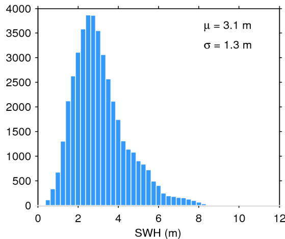
Figure 20. Histogram of science-valid SWH over oceans and lakes for 09/05/2015. The mean ( \mu ) and standard deviation ( \sigma ) are also shown. Note that values larger than 12 m are excluded from the histogram for the sake of readability but not from the computation of \mu and \sigma .
