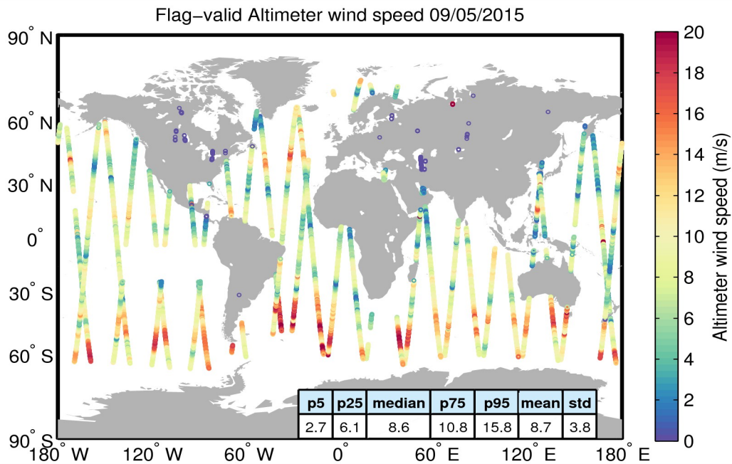
Figure 31. Geographical distribution of flag-valid wind data over oceans and lakes for 09/05/2015. The statistical values shown in the table refer to the wind in m/s and are calculated over all measurements shown in the figure.
