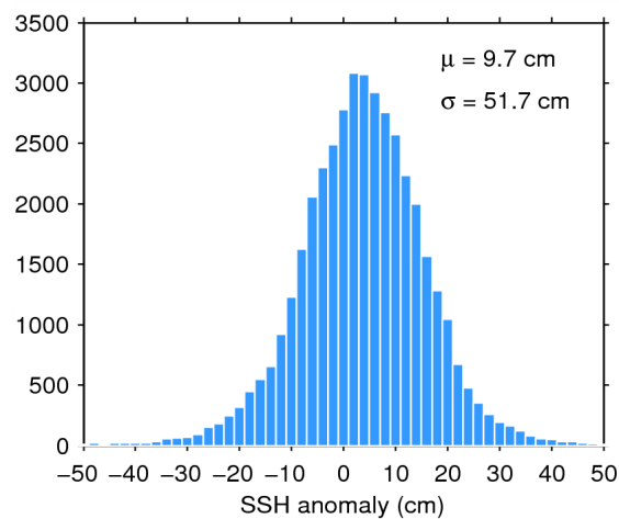
Figure 7. Histogram of flag-valid SSH anomaly over oceans and lakes for 09/05/2015. The mean ( \mu ) and standard deviation ( \sigma ) are also shown. Note that values outside [-50 50] cm are excluded from the histogram for the sake of readability but not from the computation of \mu and \sigma .
