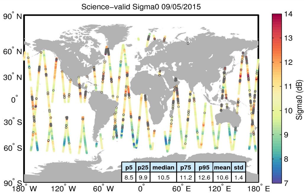
Figure 27. Geographical distribution of science-valid sigma0 data over oceans and lakes for 09/05/2015. The statistical values shown in the table refer to the sigma0 in dB and are calculated over all measurements shown in the figure. Gray circles denote records that have been rejected based on the editing criteria described in Table 4.
