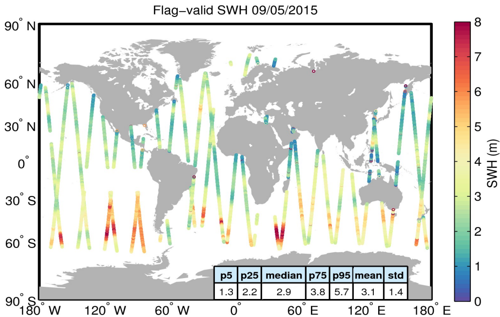
Figure 15. Geographical distribution of flag-valid SWH data over oceans and lakes for 09/05/2015. The statistical values shown in the table refer to the SWH in m and are calculated over all measurements shown in the figure.
