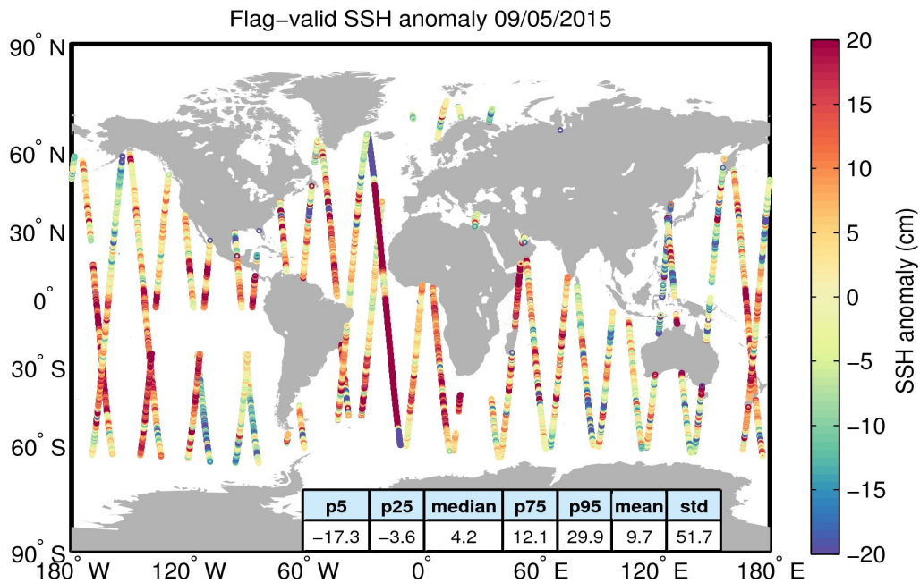
Figure 5. Geographical distribution of flag-valid 1-Hz SSH anomaly data over oceans and lakes for 09/05/2015. The statistical values shown in the table refer to the SSH anomaly in cm and are calculated over all measurements shown in the figure.
