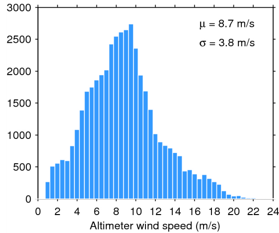
Figure 33. Histogram of flag-valid wind over oceans and lakes for 09/05/2015. The mean ( \mu ) and standard deviation ( \sigma ) are also shown. Note that values larger than 24 m/s are excluded from the histogram for the sake of readability but not from the computation of \mu and \sigma .
