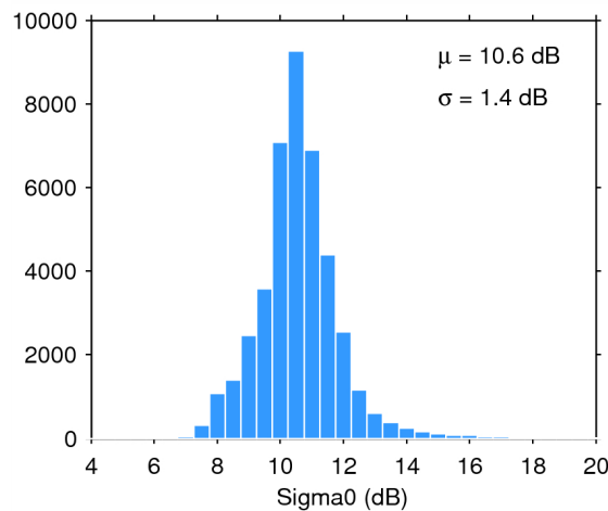
Figure 28. Histogram of science-valid sigma0 over oceans and lakes for 09/05/2015. The mean ( \mu ) and standard deviation ( \sigma ) are also shown. Note that values outside [4 20] dB are excluded from the histogram for the sake of readability but not from the computation of \mu and \sigma .
