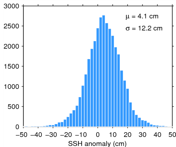
Figure 11. Histogram of science-valid SSH anomaly over oceans and lakes for 09/05/2015. The mean ( \mu ) and standard deviation ( \sigma ) are also shown. Note that values outside [-50 50] cm are excluded from the histogram for the sake of readability but not from the computation of \mu and \sigma .
