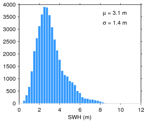
Figure 17. Histogram of flag-valid SWH over oceans and lakes for 09/05/2015. The mean ( \mu ) and standard deviation ( \sigma ) are also shown. Note that values larger than 12 m are excluded from the histogram for the sake of readability but not from the computation of \mu and \sigma .
