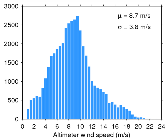
Figure 35. Histogram of science-valid wind over oceans and lakes for 09/05/2015. The mean ( \mu ) and standard deviation ( \sigma ) are also shown. Note that values larger than 24 m/s are excluded from the histogram for the sake of readability but not from the computation of \mu and \sigma .
