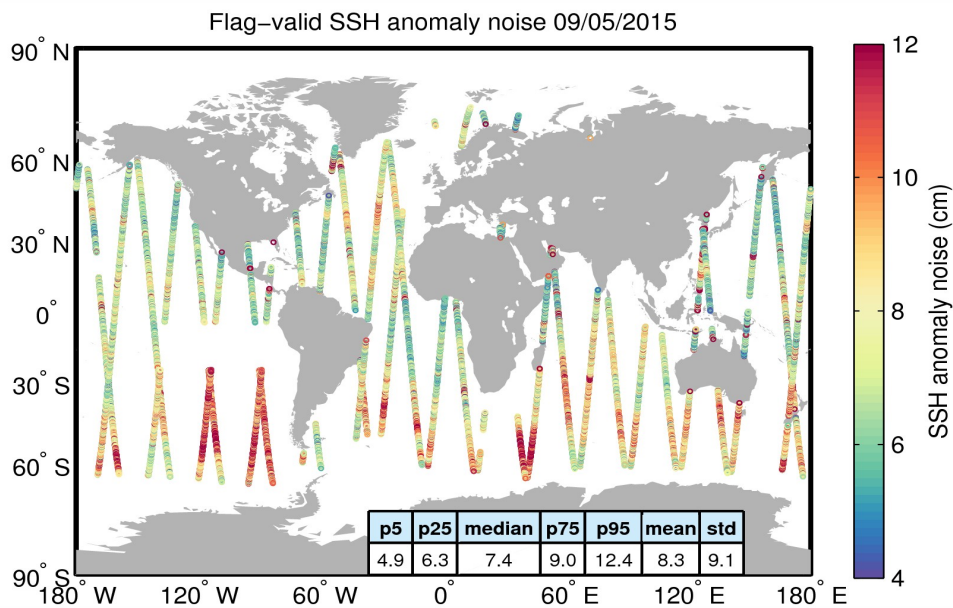
Figure 8. Geographical distribution of flag-valid 20-Hz SSH anomaly measurement noise over oceans and lakes for 09/05/2015. The statistical values shown in the table refer to the SSH anomaly noise and are calculated over all measurements shown in the figure.
