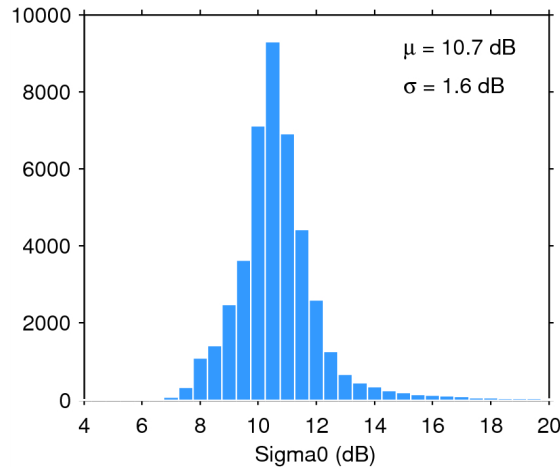
Figure 25. Histogram of flag-valid sigma0 over oceans and lakes for 09/05/2015. The mean ( \mu ) and standard deviation ( \sigma ) are also shown. Note that values outside [4 20] dB are excluded from the histogram for the sake of readability but not from the computation of \mu and \sigma .
