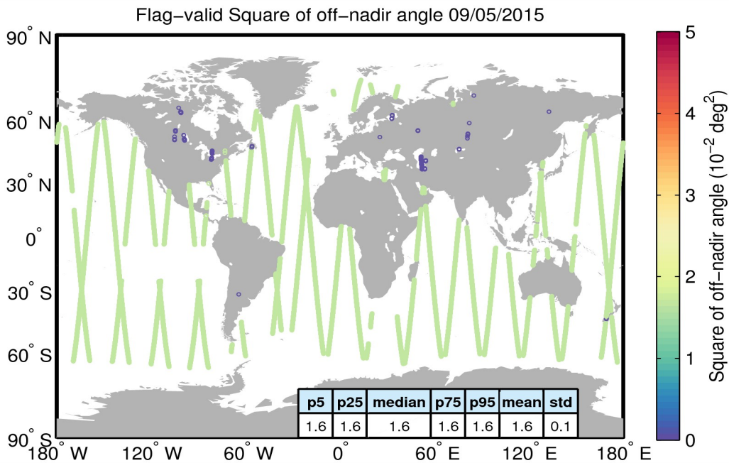
Figure 37. Geographical distribution of flag-valid mispointing data over oceans and lakes for 09/05/2015. The statistical values shown in the table refer to the mispointing in 10^{-2} \text{deg}^2 and are calculated over all measurements shown in the figure.
