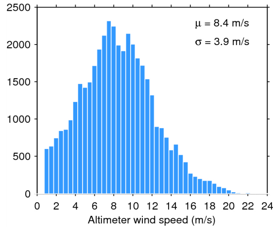
Figure 33. Histogram of flag-valid wind over oceans and lakes for 08/05/2015. The mean ( \mu ) and standard deviation ( \sigma ) are also shown. Note that values larger than 24 m/s are excluded from the histogram for the sake of readability but not from the computation of \mu and \sigma .
