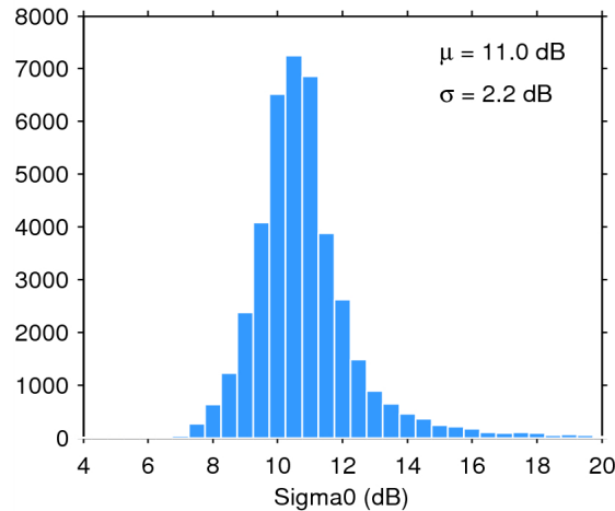
Figure 25. Histogram of flag-valid sigma0 over oceans and lakes for 08/05/2015. The mean ( \mu ) and standard deviation ( \sigma ) are also shown. Note that values outside [4 20] dB are excluded from the histogram for the sake of readability but not from the computation of \mu and \sigma .
