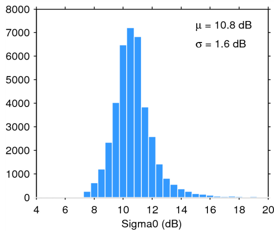
Figure 28. Histogram of science-valid sigma0 over oceans and lakes for 08/05/2015. The mean ( \mu ) and standard deviation ( \sigma ) are also shown. Note that values outside [4 20] dB are excluded from the histogram for the sake of readability but not from the computation of \mu and \sigma .
