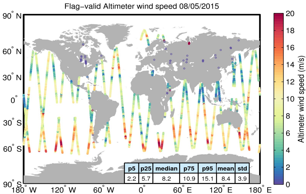
Figure 31. Geographical distribution of flag-valid wind data over oceans and lakes for 08/05/2015. The statistical values shown in the table refer to the wind in m/s and are calculated over all measurements shown in the figure.
