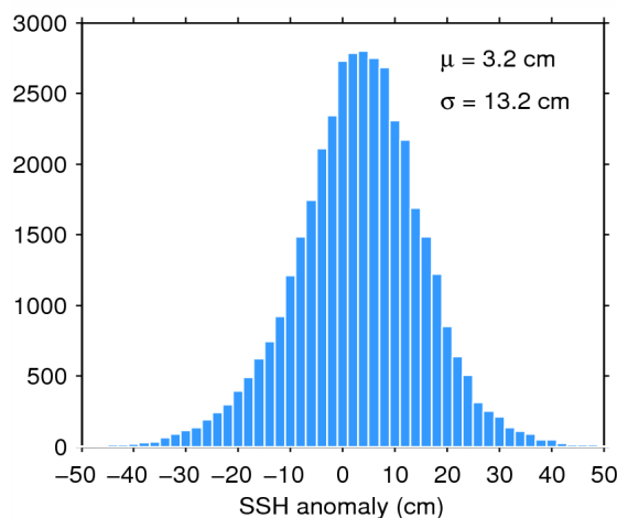
Figure 11. Histogram of science-valid SSH anomaly over oceans and lakes for 08/05/2015. The mean ( \mu ) and standard deviation ( \sigma ) are also shown. Note that values outside [-50 50] cm are excluded from the histogram for the sake of readability but not from the computation of \mu and \sigma .
