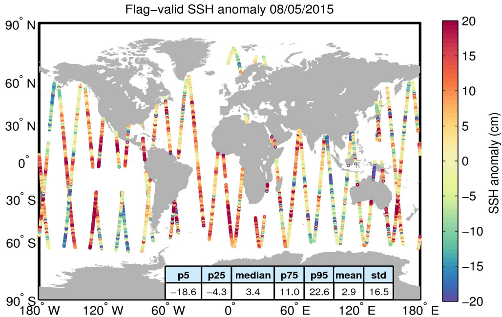
Figure 5. Geographical distribution of flag-valid 1-Hz SSH anomaly data over oceans and lakes for 08/05/2015. The statistical values shown in the table refer to the SSH anomaly in cm and are calculated over all measurements shown in the figure.
