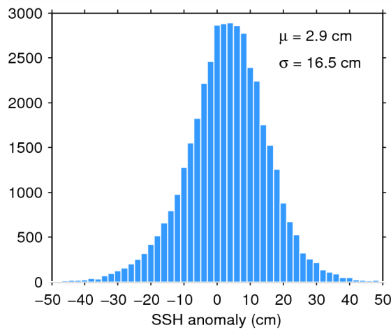
Figure 7. Histogram of flag-valid SSH anomaly over oceans and lakes for 08/05/2015. The mean ( \mu ) and standard deviation ( \sigma ) are also shown. Note that values outside [-50\ 50] cm are excluded from the histogram for the sake of readability but not from the computation of \mu and \sigma .
