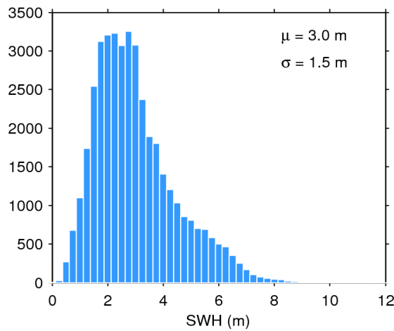
Figure 17. Histogram of flag-valid SWH over oceans and lakes for 08/05/2015. The mean ( \mu ) and standard deviation ( \sigma ) are also shown. Note that values larger than 12 m are excluded from the histogram for the sake of readability but not from the computation of \mu and \sigma .
