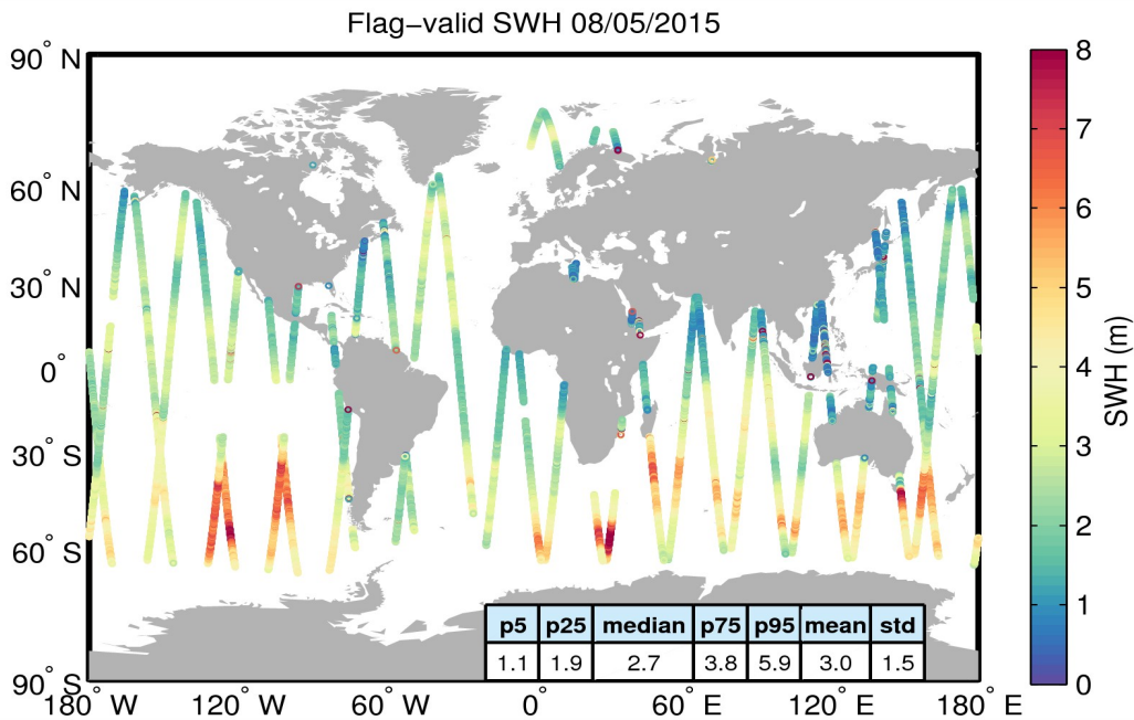
Figure 15. Geographical distribution of flag-valid SWH data over oceans and lakes for 08/05/2015. The statistical values shown in the table refer to the SWH in m and are calculated over all measurements shown in the figure.
