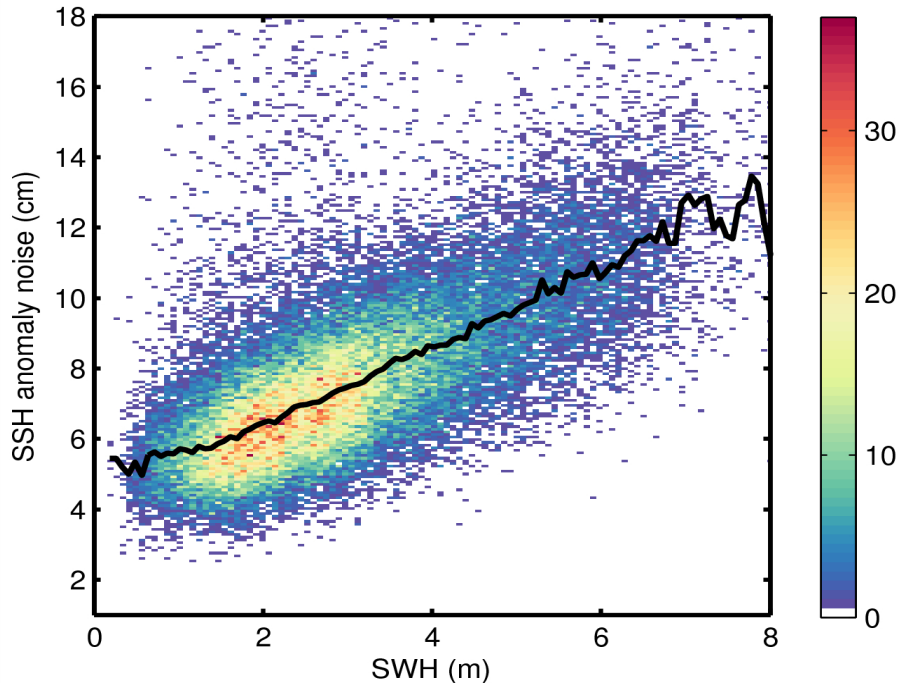
Figure 9. 2D histogram showing flag-valid SSH anomaly noise as a function of SWH for 08/05/2015. The black line denotes the median SSH anomaly as a function of SWH.
