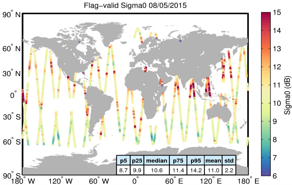
Figure 23. Geographical distribution of flag-valid sigma0 data over oceans and lakes for 08/05/2015. The statistical values shown in the table refer to the sigma0 in dB and are calculated over all measurements shown in the figure.
