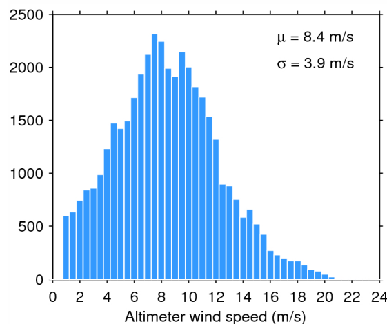
Figure 35. Histogram of science-valid wind over oceans and lakes for 08/05/2015. The mean ( \mu ) and standard deviation ( \sigma ) are also shown. Note that values larger than 24 m/s are excluded from the histogram for the sake of readability but not from the computation of \mu and \sigma .
