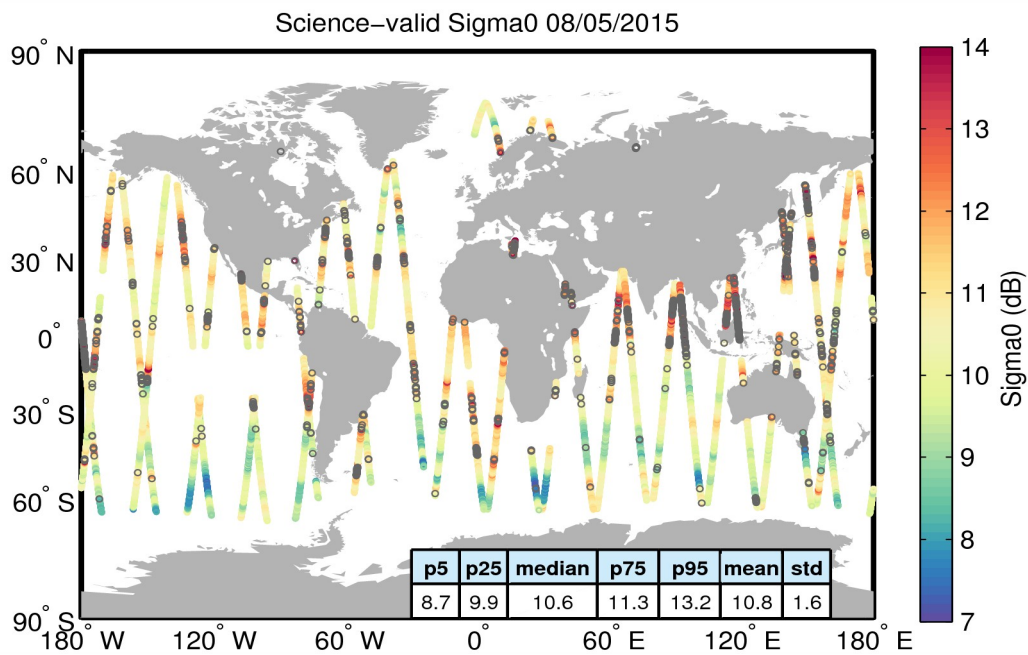
Figure 27. Geographical distribution of science-valid sigma0 data over oceans and lakes for 08/05/2015. The statistical values shown in the table refer to the sigma0 in dB and are calculated over all measurements shown in the figure. Gray circles denote records that have been rejected based on the editing criteria described in Table 4.
