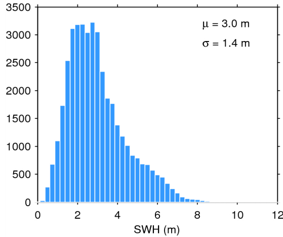
Figure 20. Histogram of science-valid SWH over oceans and lakes for 08/05/2015. The mean ( \mu ) and standard deviation ( \sigma ) are also shown. Note that values larger than 12 m are excluded from the histogram for the sake of readability but not from the computation of \mu and \sigma .
