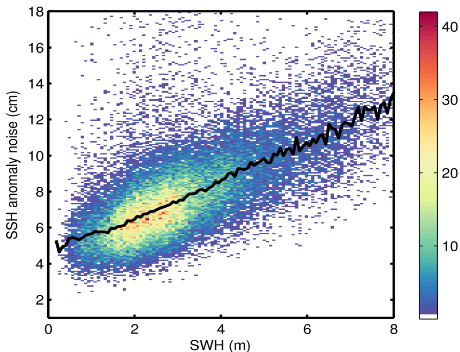
Figure 9. 2D histogram showing flag-valid SSH anomaly noise as a function of SWH for 07/05/2015. The black line denotes the median SSH anomaly as a function of SWH.
