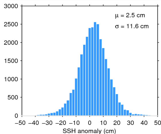
Figure 11. Histogram of science-valid SSH anomaly over oceans and lakes for 07/05/2015. The mean ( \mu ) and standard deviation ( \sigma ) are also shown. Note that values outside [-50 50] cm are excluded from the histogram for the sake of readability but not from the computation of \mu and \sigma .
