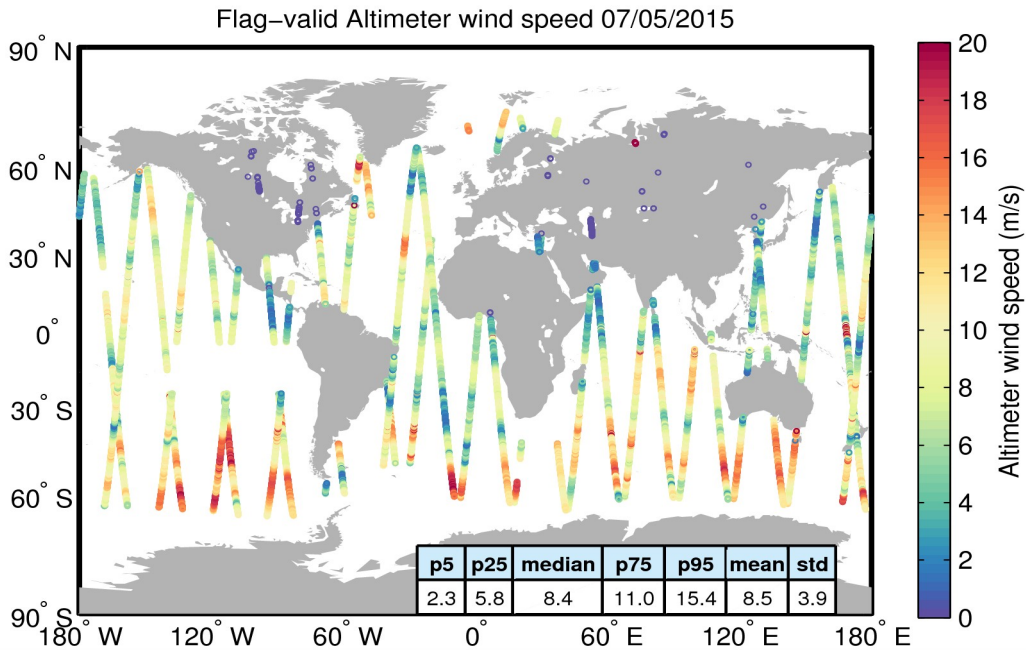
Figure 31. Geographical distribution of flag-valid wind data over oceans and lakes for 07/05/2015. The statistical values shown in the table refer to the wind in m/s and are calculated over all measurements shown in the figure.
