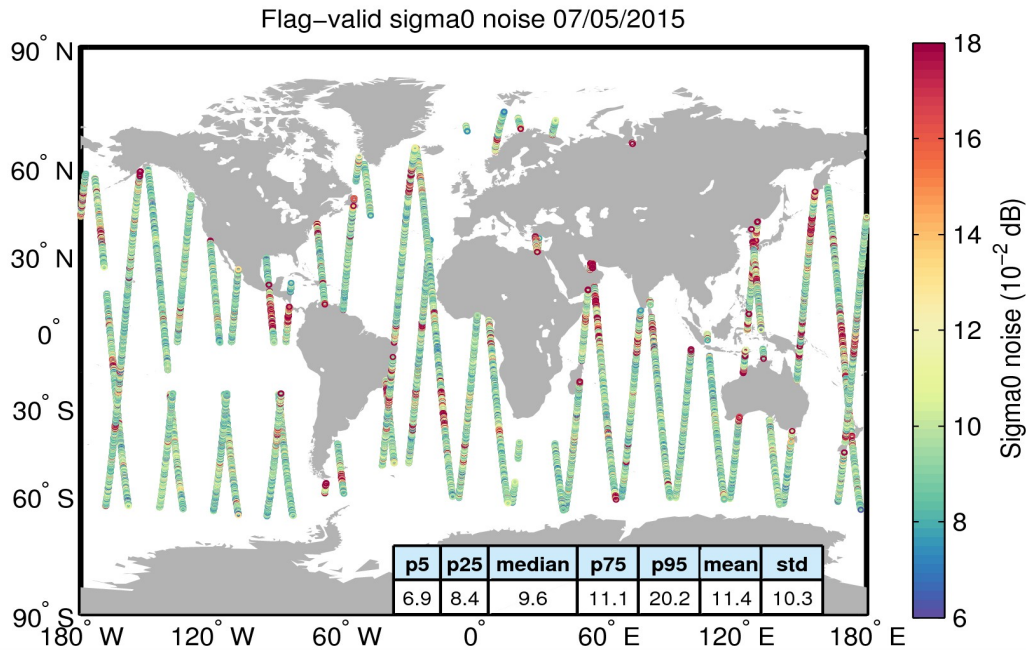
Figure 26. Geographical distribution of flag-valid 20-Hz sigma0 measurement noise over oceans and lakes for 07/05/2015. The statistical values shown in the table refer to the sigma0 noise and are calculated over all measurements shown in the figure.
