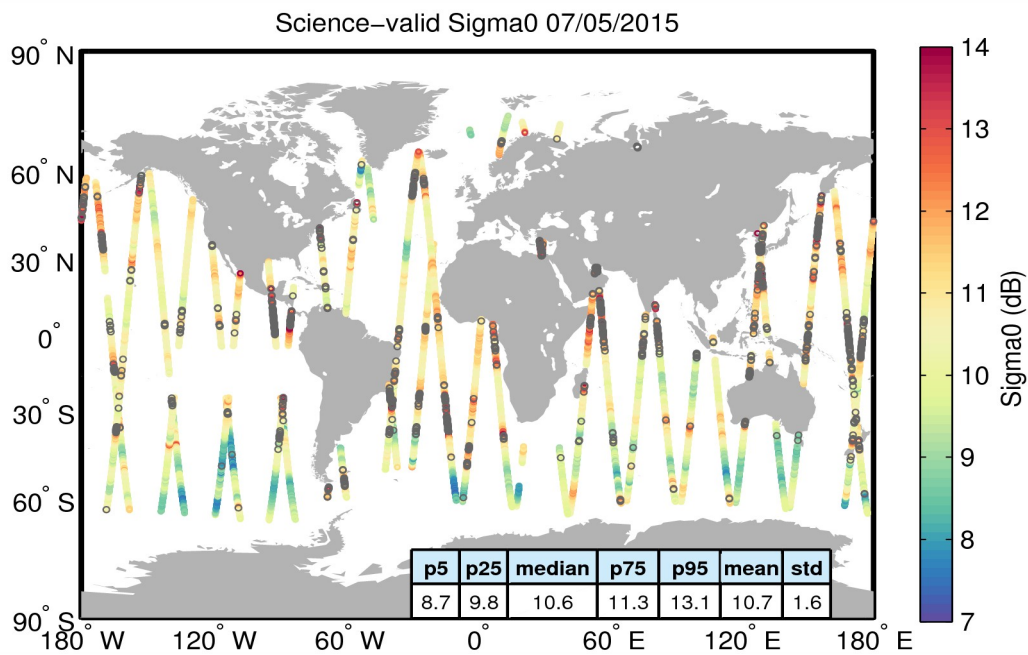
Figure 27. Geographical distribution of science-valid sigma0 data over oceans and lakes for 07/05/2015. The statistical values shown in the table refer to the sigma0 in dB and are calculated over all measurements shown in the figure. Gray circles denote records that have been rejected based on the editing criteria described in Table 4.
