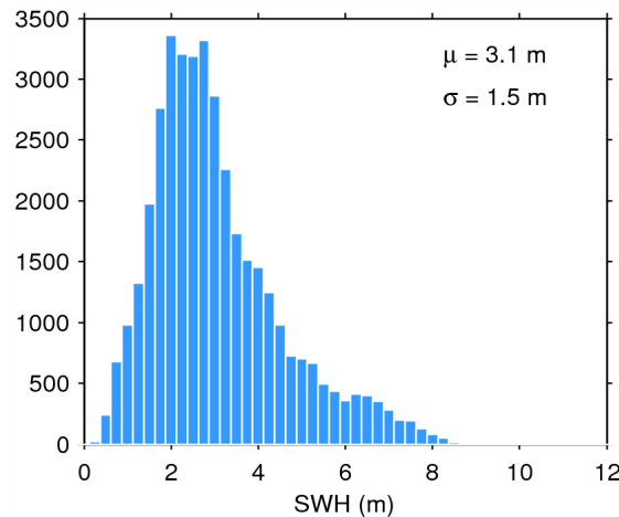
Figure 20. Histogram of science-valid SWH over oceans and lakes for 07/05/2015. The mean ( \mu ) and standard deviation ( \sigma ) are also shown. Note that values larger than 12 m are excluded from the histogram for the sake of readability but not from the computation of \mu and \sigma .
