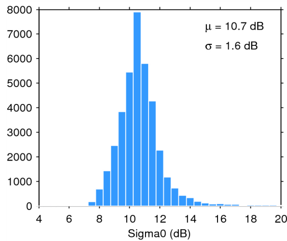
Figure 28. Histogram of science-valid sigma0 over oceans and lakes for 07/05/2015. The mean ( \mu ) and standard deviation ( \sigma ) are also shown. Note that values outside [4 20] dB are excluded from the histogram for the sake of readability but not from the computation of \mu and \sigma .
