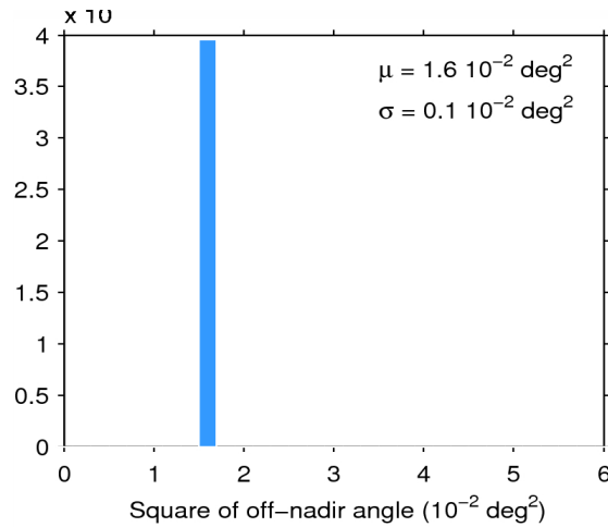
Figure 39. Histogram of flag-valid mispointing over oceans and lakes for 07/05/2015. The mean ( \mu ) and standard deviation ( \sigma ) are also shown. Note that values than 6 \cdot 10^{-2} \text{ deg}^2 are excluded from the histogram for the sake of readability but not from the computation of \mu and \sigma .
