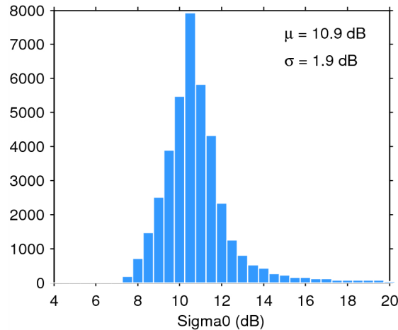
Figure 25. Histogram of flag-valid sigma0 over oceans and lakes for 07/05/2015. The mean ( \mu ) and standard deviation ( \sigma ) are also shown. Note that values outside [4 20] dB are excluded from the histogram for the sake of readability but not from the computation of \mu and \sigma .
