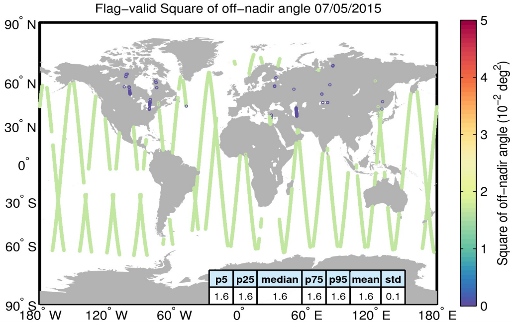
Figure 37. Geographical distribution of flag-valid mispointing data over oceans and lakes for 07/05/2015. The statistical values shown in the table refer to the mispointing in 10^{-2} \text{ deg}^2 and are calculated over all measurements shown in the figure.
