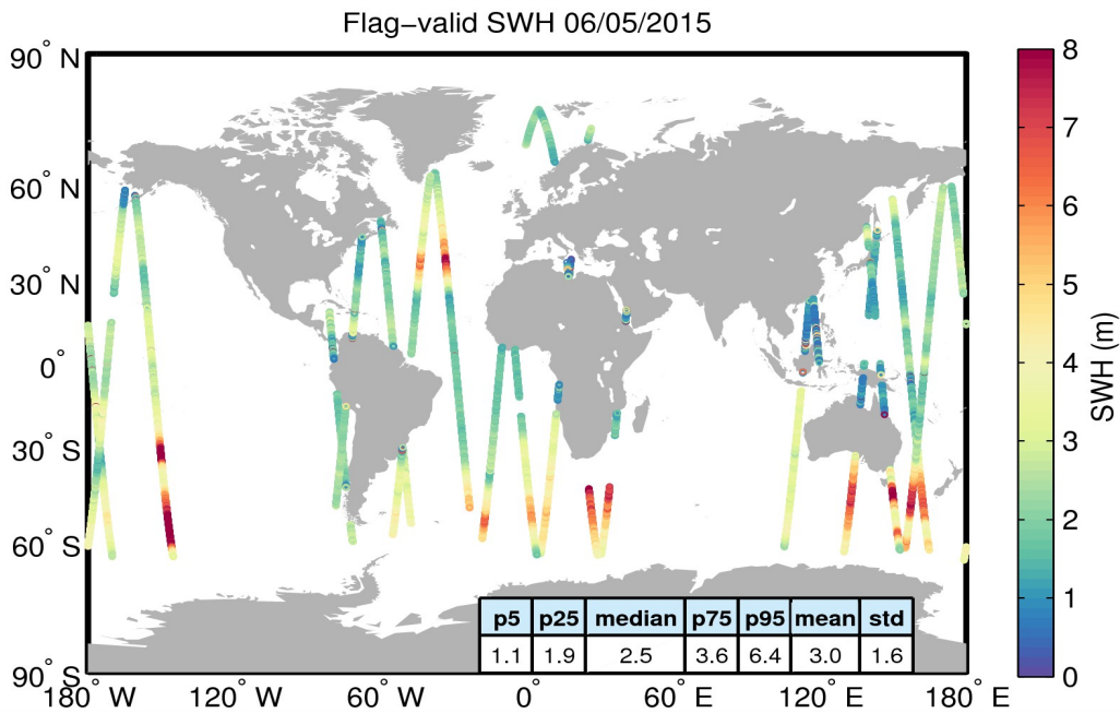
Figure 15. Geographical distribution of flag-valid SWH data over oceans and lakes for 06/05/2015. The statistical values shown in the table refer to the SWH in m and are calculated over all measurements shown in the figure.
