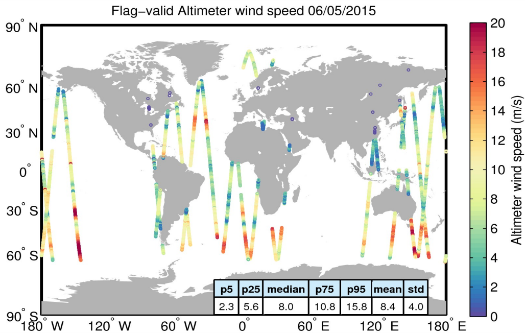
Figure 31. Geographical distribution of flag-valid wind data over oceans and lakes for 06/05/2015. The statistical values shown in the table refer to the wind in m/s and are calculated over all measurements shown in the figure.
