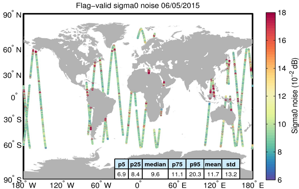
Figure 26. Geographical distribution of flag-valid 20-Hz sigma0 measurement noise over oceans and lakes for 06/05/2015. The statistical values shown in the table refer to the sigma0 noise and are calculated over all measurements shown in the figure.
