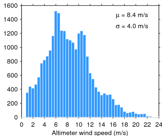
Figure 35. Histogram of science-valid wind over oceans and lakes for 06/05/2015. The mean ( \mu ) and standard deviation ( \sigma ) are also shown. Note that values larger than 24 m/s are excluded from the histogram for the sake of readability but not from the computation of \mu and \sigma .
