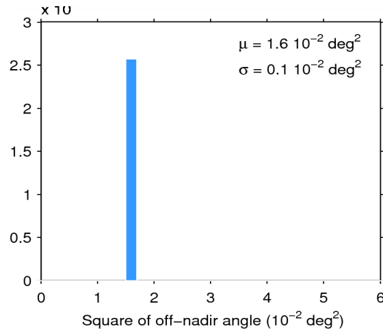
Figure 39. Histogram of flag-valid mispointing over oceans and lakes for 06/05/2015. The mean ( \mu ) and standard deviation ( \sigma ) are also shown. Note that values than 6 \cdot 10^{-2} \text{ deg}^2 are excluded from the histogram for the sake of readability but not from the computation of \mu and \sigma .
