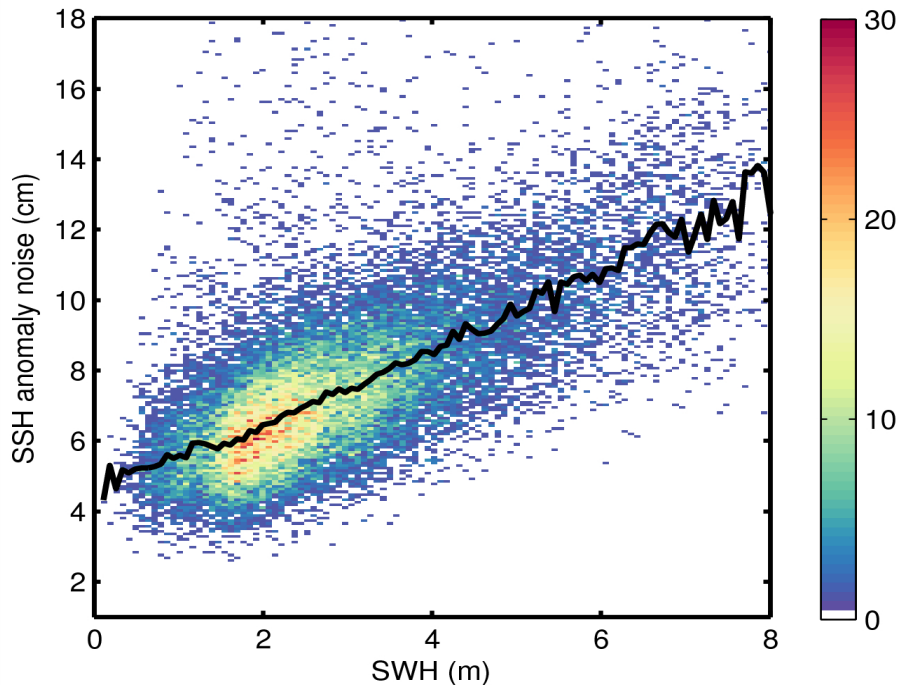
Figure 9. 2D histogram showing flag-valid SSH anomaly noise as a function of SWH for 06/05/2015. The black line denotes the median SSH anomaly as a function of SWH.
