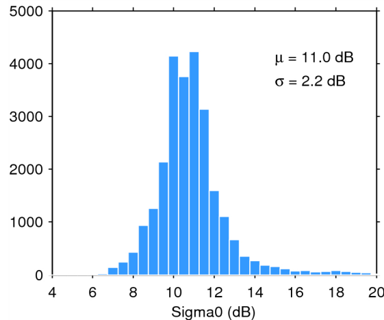
Figure 25. Histogram of flag-valid sigma0 over oceans and lakes for 06/05/2015. The mean ( \mu ) and standard deviation ( \sigma ) are also shown. Note that values outside [4 20] dB are excluded from the histogram for the sake of readability but not from the computation of \mu and \sigma .
