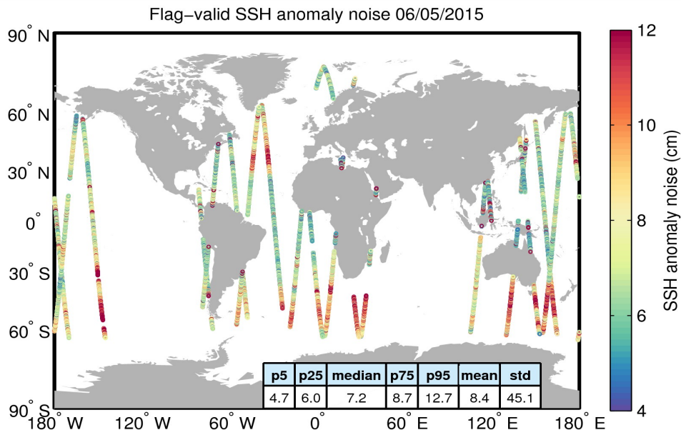
Figure 8. Geographical distribution of flag-valid 20-Hz SSH anomaly measurement noise over oceans and lakes for 06/05/2015. The statistical values shown in the table refer to the SSH anomaly noise and are calculated over all measurements shown in the figure.
