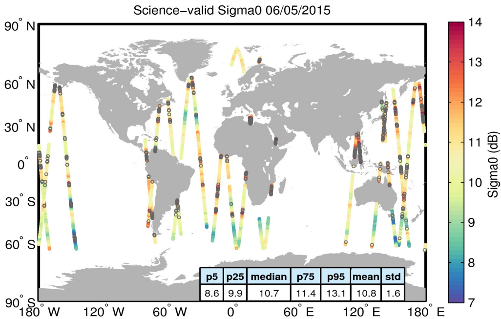
Figure 27. Geographical distribution of science-valid sigma0 data over oceans and lakes for 06/05/2015. The statistical values shown in the table refer to the sigma0 in dB and are calculated over all measurements shown in the figure. Gray circles denote records that have been rejected based on the editing criteria described in Table 4.
