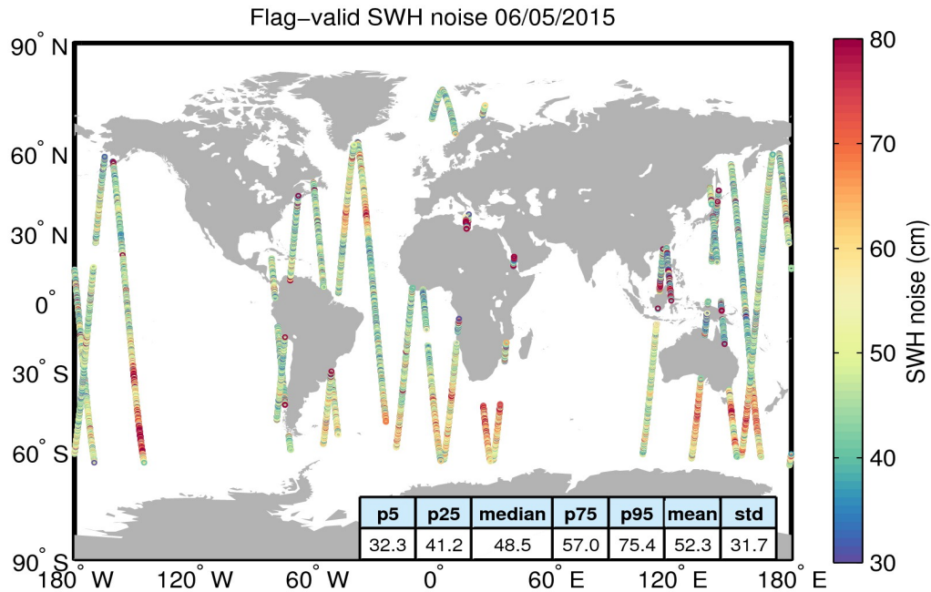
Figure 18. Geographical distribution of flag-valid 20-Hz SWH measurement noise over oceans and lakes for 06/05/2015. The statistical values shown in the figure refer to the SWH noise and are calculated over all measurements shown in the figure.
