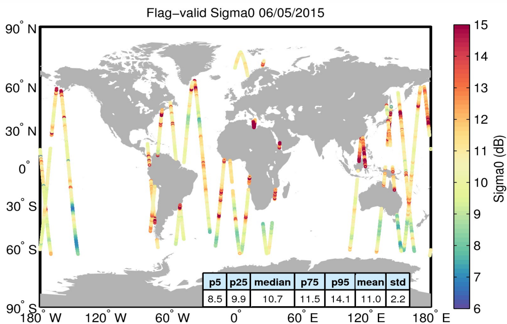
Figure 23. Geographical distribution of flag-valid sigma0 data over oceans and lakes for 06/05/2015. The statistical values shown in the table refer to the sigma0 in dB and are calculated over all measurements shown in the figure.
