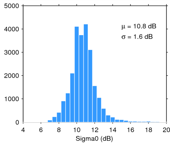
Figure 28. Histogram of science-valid sigma0 over oceans and lakes for 06/05/2015. The mean ( \mu ) and standard deviation ( \sigma ) are also shown. Note that values outside [4 20] dB are excluded from the histogram for the sake of readability but not from the computation of \mu and \sigma .
