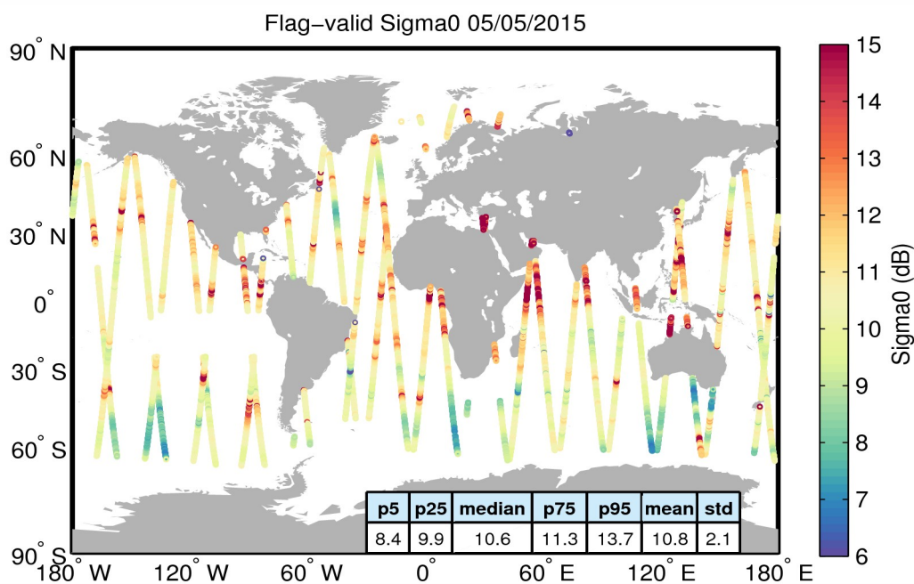
Figure 23. Geographical distribution of flag-valid sigma0 data over oceans and lakes for 05/05/2015. The statistical values shown in the table refer to the sigma0 in dB and are calculated over all measurements shown in the figure.
