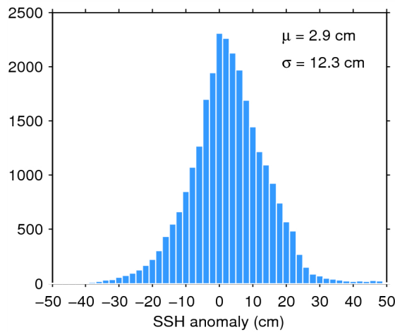
Figure 11. Histogram of science-valid SSH anomaly over oceans and lakes for 05/05/2015. The mean ( \mu ) and standard deviation ( \sigma ) are also shown. Note that values outside [-50 50] cm are excluded from the histogram for the sake of readability but not from the computation of \mu and \sigma .
