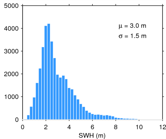
Figure 20. Histogram of science-valid SWH over oceans and lakes for 05/05/2015. The mean ( \mu ) and standard deviation ( \sigma ) are also shown. Note that values larger than 12 m are excluded from the histogram for the sake of readability but not from the computation of \mu and \sigma .
