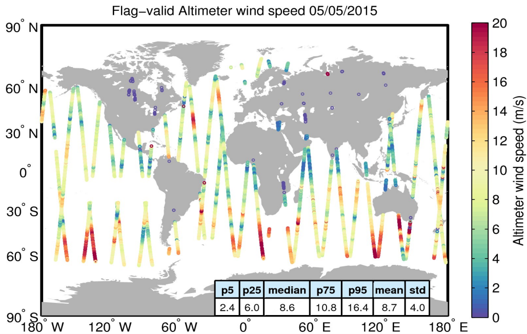
Figure 31. Geographical distribution of flag-valid wind data over oceans and lakes for 05/05/2015. The statistical values shown in the table refer to the wind in m/s and are calculated over all measurements shown in the figure.
