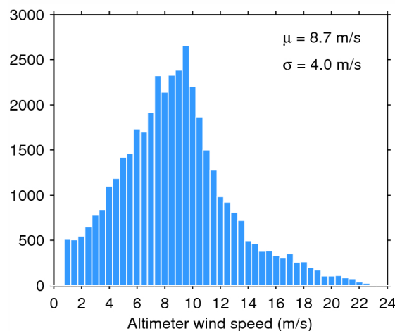
Figure 35. Histogram of science-valid wind over oceans and lakes for 05/05/2015. The mean ( \mu ) and standard deviation ( \sigma ) are also shown. Note that values larger than 24 m/s are excluded from the histogram for the sake of readability but not from the computation of \mu and \sigma .
