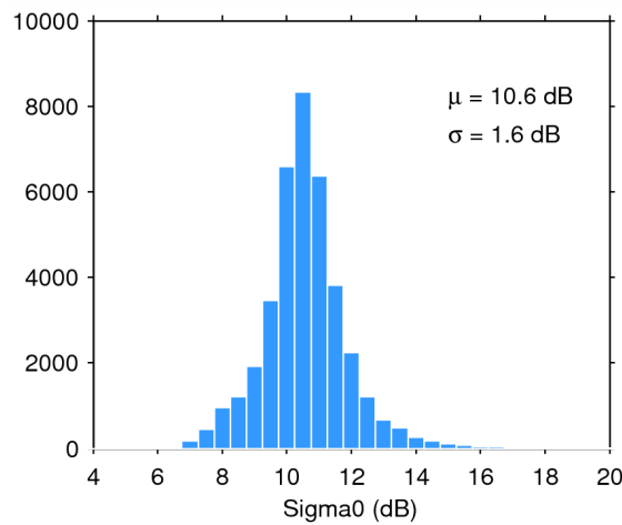
Figure 28. Histogram of science-valid sigma0 over oceans and lakes for 05/05/2015. The mean ( \mu ) and standard deviation ( \sigma ) are also shown. Note that values outside [4 20] dB are excluded from the histogram for the sake of readability but not from the computation of \mu and \sigma .
