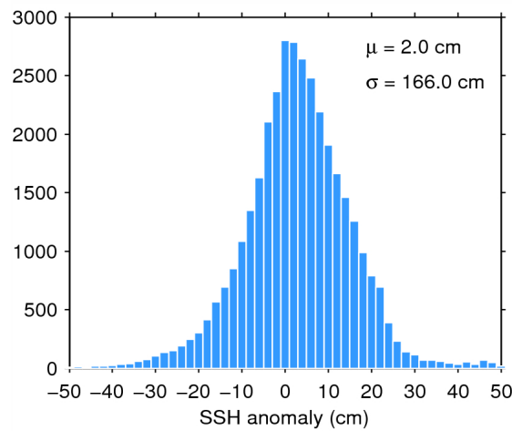
Figure 7. Histogram of flag-valid SSH anomaly over oceans and lakes for 05/05/2015. The mean ( \mu ) and standard deviation ( \sigma ) are also shown. Note that values outside [-50 50] cm are excluded from the histogram for the sake of readability but not from the computation of \mu and \sigma .
