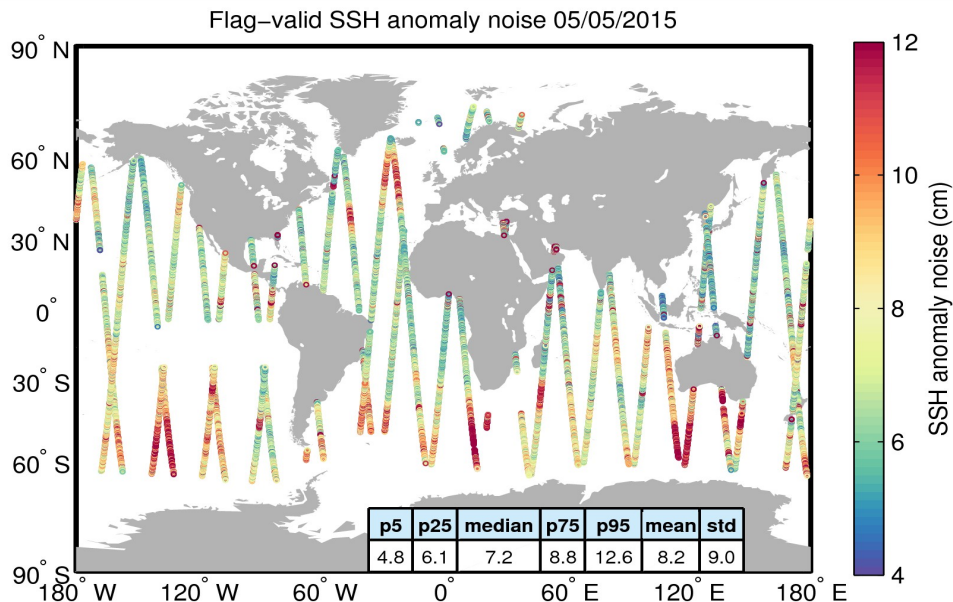
Figure 8. Geographical distribution of flag-valid 20-Hz SSH anomaly measurement noise over oceans and lakes for 05/05/2015. The statistical values shown in the table refer to the SSH anomaly noise and are calculated over all measurements shown in the figure.
