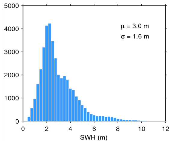
Figure 17. Histogram of flag-valid SWH over oceans and lakes for 05/05/2015. The mean ( \mu ) and standard deviation ( \sigma ) are also shown. Note that values larger than 12 m are excluded from the histogram for the sake of readability but not from the computation of \mu and \sigma .
