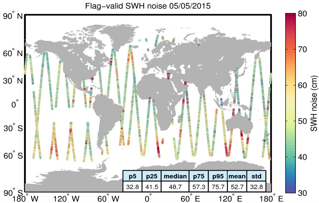
Figure 18. Geographical distribution of flag-valid 20-Hz SWH measurement noise over oceans and lakes for 05/05/2015. The statistical values shown in the figure refer to the SWH noise and are calculated over all measurements shown in the figure.
