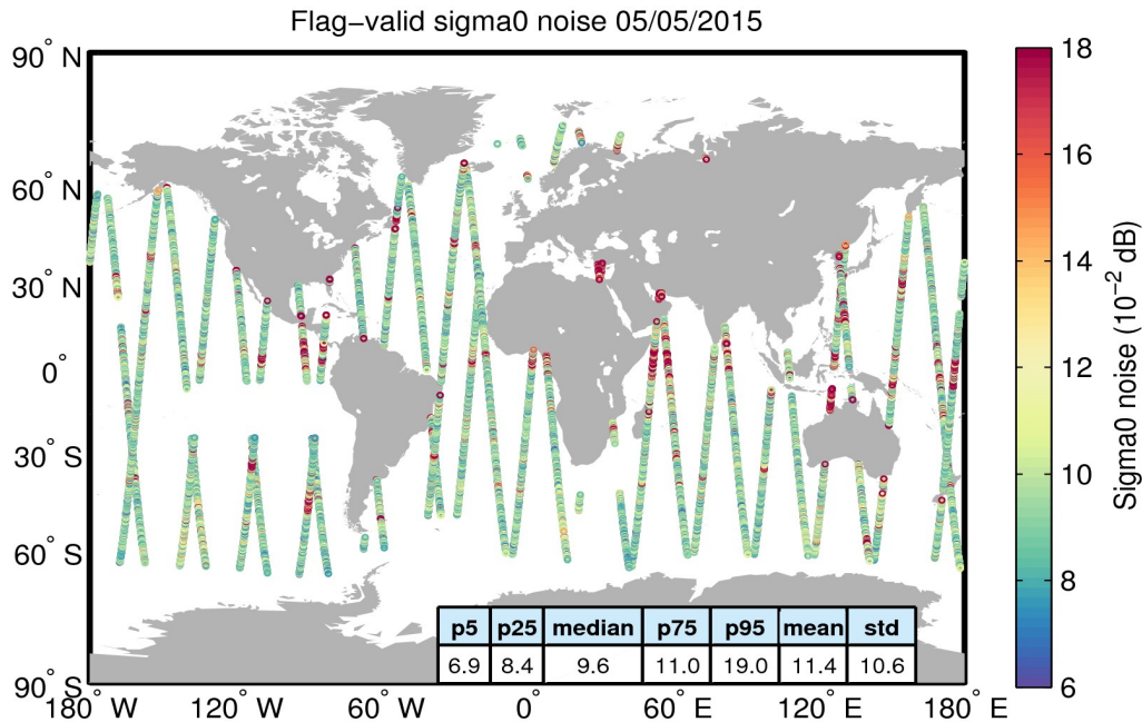
Figure 26. Geographical distribution of flag-valid 20-Hz sigma0 measurement noise over oceans and lakes for 05/05/2015. The statistical values shown in the table refer to the sigma0 noise and are calculated over all measurements shown in the figure.
