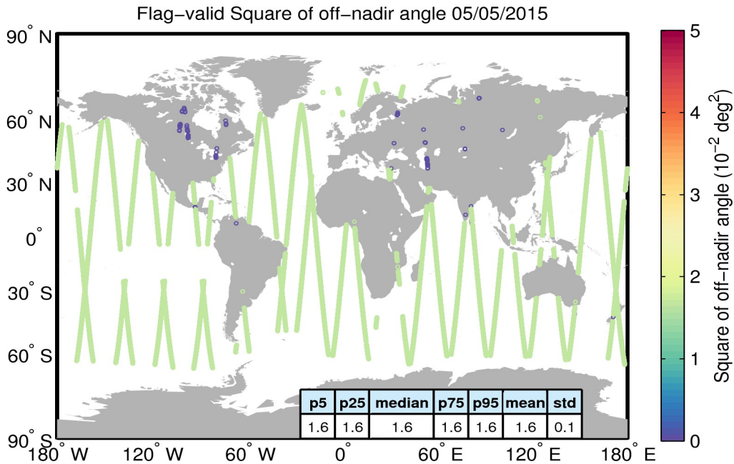
Figure 37. Geographical distribution of flag-valid mispointing data over oceans and lakes for 05/05/2015. The statistical values shown in the table refer to the mispointing in 10^{-2} \text{ deg}^2 and are calculated over all measurements shown in the figure.
