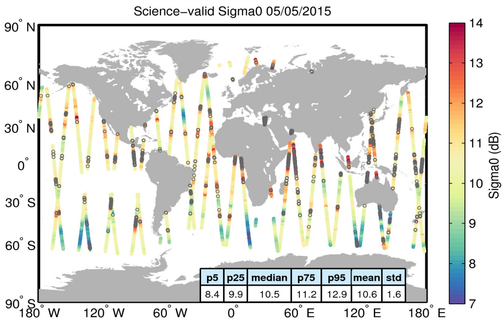
Figure 27. Geographical distribution of science-valid sigma0 data over oceans and lakes for 05/05/2015. The statistical values shown in the table refer to the sigma0 in dB and are calculated over all measurements shown in the figure. Gray circles denote records that have been rejected based on the editing criteria described in Table 4.
