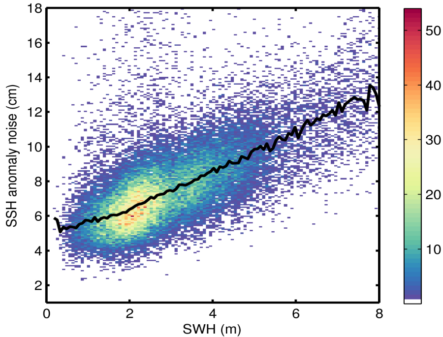
Figure 9. 2D histogram showing flag-valid SSH anomaly noise as a function of SWH for 05/05/2015. The black line denotes the median SSH anomaly as a function of SWH.
