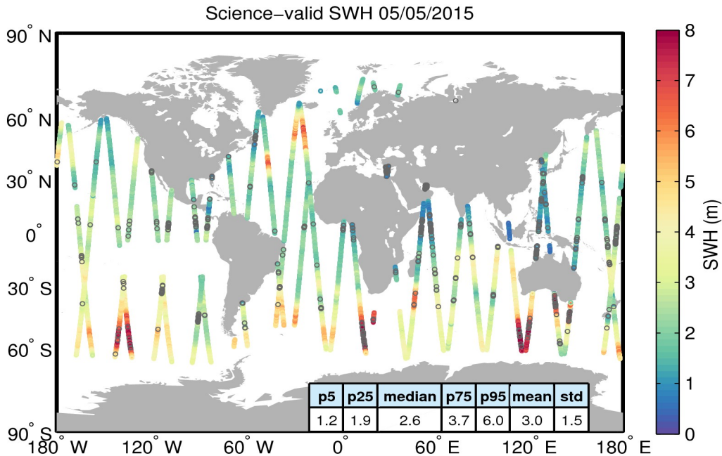
Figure 19. Geographical distribution of science-valid SWH data over oceans and lakes for 05/05/2015. The statistical values shown in the table refer to the SWH in m and are calculated over all measurements shown in the figure. Gray circles denote records that have been rejected based on the editing criteria described in Table 3.
