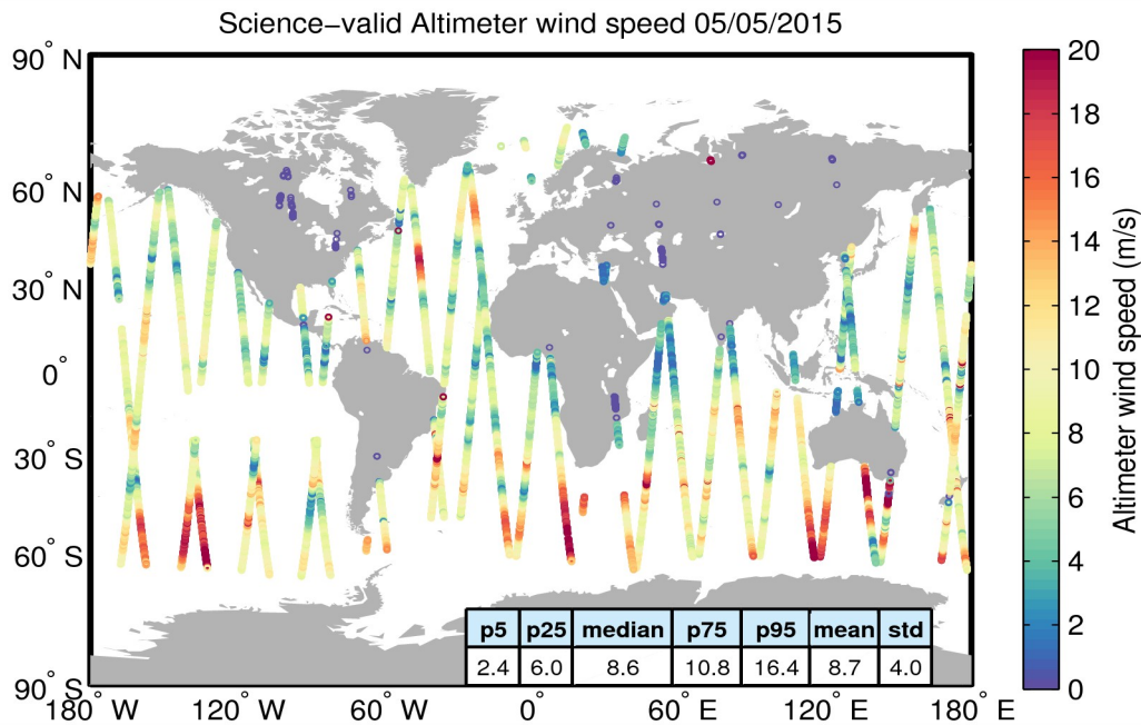
Figure 34. Geographical distribution of science-valid wind data over oceans and lakes for 05/05/2015. The statistical values shown in the table refer to the wind in m/s and are calculated over all measurements shown in the figure. Gray circles denote records that have been rejected based on the editing criteria described in Table 5.
