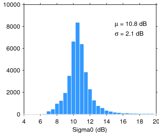
Figure 25. Histogram of flag-valid sigma0 over oceans and lakes for 05/05/2015. The mean ( \mu ) and standard deviation ( \sigma ) are also shown. Note that values outside [4 20] dB are excluded from the histogram for the sake of readability but not from the computation of \mu and \sigma .
