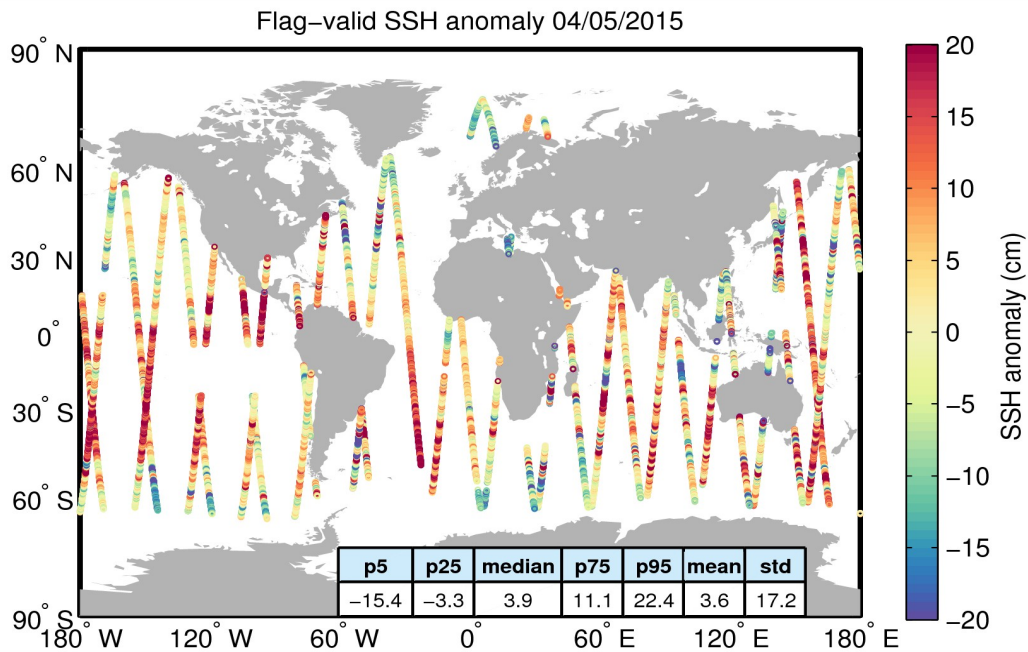
Figure 5. Geographical distribution of flag-valid 1-Hz SSH anomaly data over oceans and lakes for 04/05/2015. The statistical values shown in the table refer to the SSH anomaly in cm and are calculated over all measurements shown in the figure.
