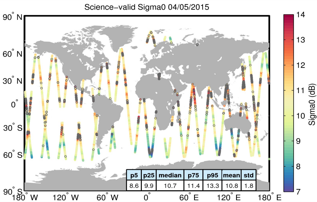
Figure 27. Geographical distribution of science-valid sigma0 data over oceans and lakes for 04/05/2015. The statistical values shown in the table refer to the sigma0 in dB and are calculated over all measurements shown in the figure. Gray circles denote records that have been rejected based on the editing criteria described in Table 4.
