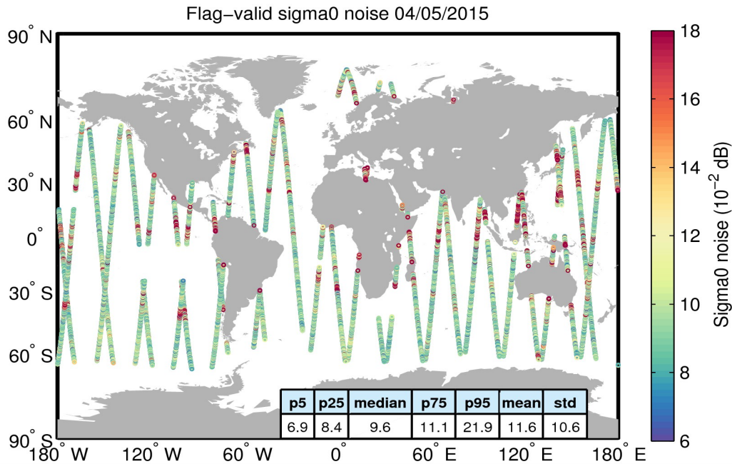
Figure 26. Geographical distribution of flag-valid 20-Hz sigma0 measurement noise over oceans and lakes for 04/05/2015. The statistical values shown in the table refer to the sigma0 noise and are calculated over all measurements shown in the figure.
