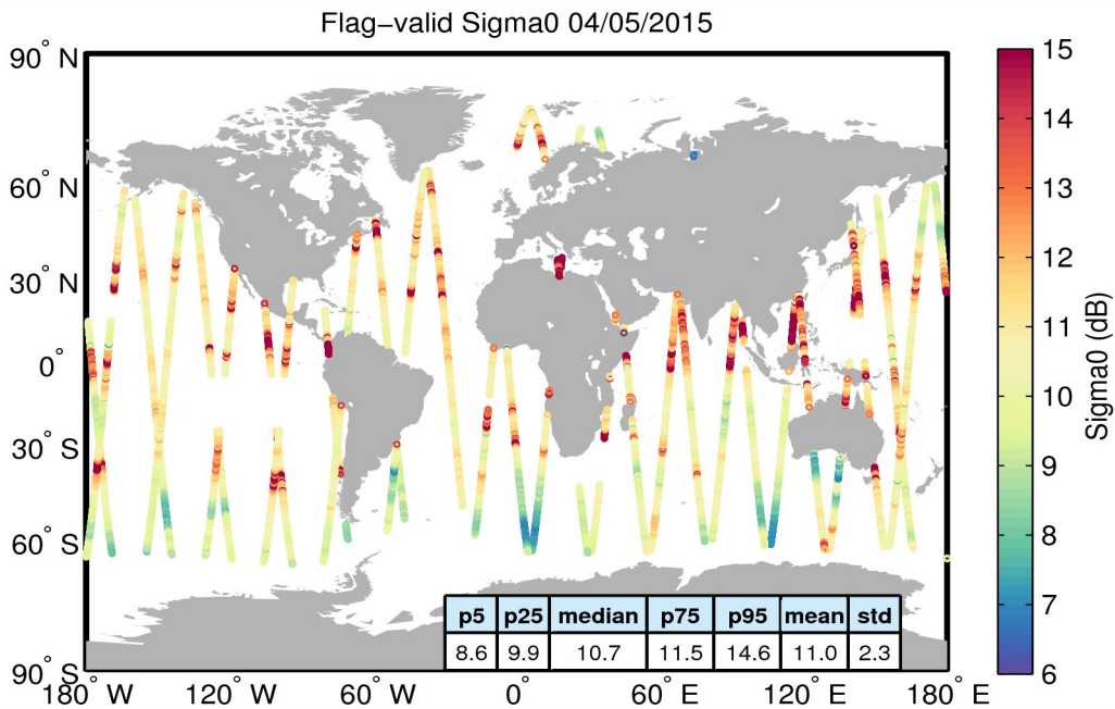
Figure 23. Geographical distribution of flag-valid sigma0 data over oceans and lakes for 04/05/2015. The statistical values shown in the table refer to the sigma0 in dB and are calculated over all measurements shown in the figure.
