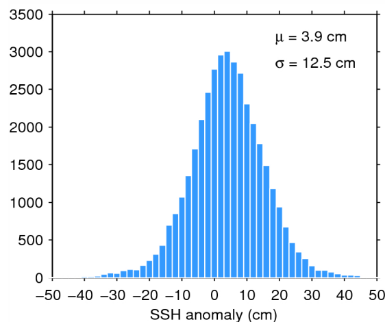
Figure 11. Histogram of science-valid SSH anomaly over oceans and lakes for 04/05/2015. The mean ( \mu ) and standard deviation ( \sigma ) are also shown. Note that values outside [-50 50] cm are excluded from the histogram for the sake of readability but not from the computation of \mu and \sigma .
