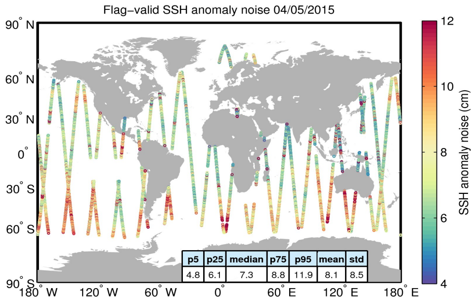
Figure 8. Geographical distribution of flag-valid 20-Hz SSH anomaly measurement noise over oceans and lakes for 04/05/2015. The statistical values shown in the table refer to the SSH anomaly noise and are calculated over all measurements shown in the figure.
