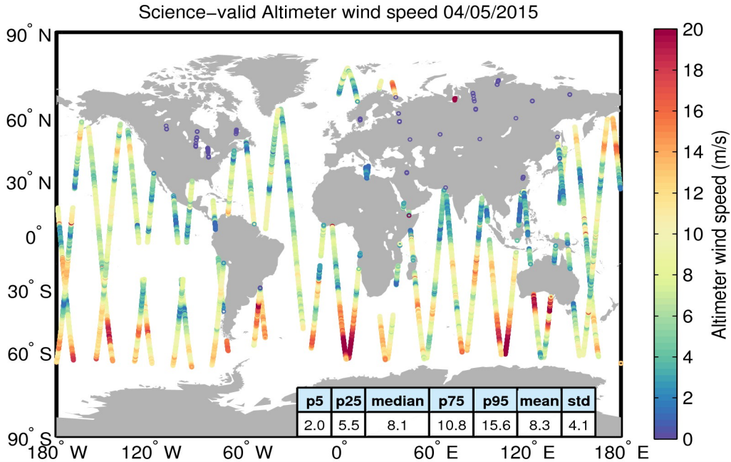
Figure 34. Geographical distribution of science-valid wind data over oceans and lakes for 04/05/2015. The statistical values shown in the table refer to the wind in m/s and are calculated over all measurements shown in the figure. Gray circles denote records that have been rejected based on the editing criteria described in Table 5.
