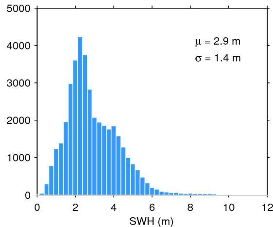
Figure 20. Histogram of science-valid SWH over oceans and lakes for 04/05/2015. The mean ( \mu ) and standard deviation ( \sigma ) are also shown. Note that values larger than 12 m are excluded from the histogram for the sake of readability but not from the computation of \mu and \sigma .
