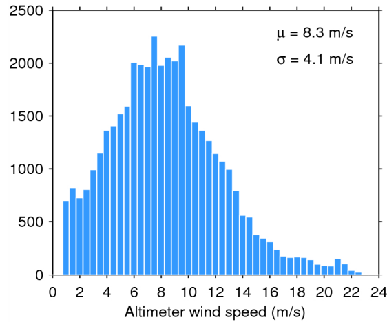
Figure 33. Histogram of flag-valid wind over oceans and lakes for 04/05/2015. The mean ( \mu ) and standard deviation ( \sigma ) are also shown. Note that values larger than 24 m/s are excluded from the histogram for the sake of readability but not from the computation of \mu and \sigma .
