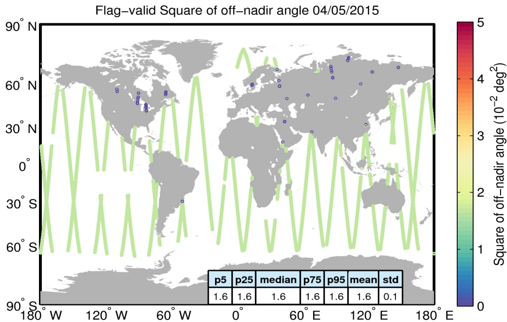
Figure 37. Geographical distribution of flag-valid mispointing data over oceans and lakes for 04/05/2015. The statistical values shown in the table refer to the mispointing in 10^{-2} deg 2 and are calculated over all measurements shown in the figure.
