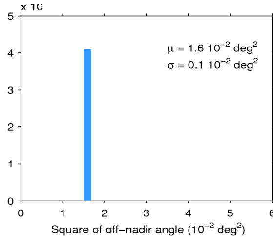
Figure 39. Histogram of flag-valid mispointing over oceans and lakes for 04/05/2015. The mean ( \mu ) and standard deviation ( \sigma ) are also shown. Note that values than 6 \cdot 10^{-2} \text{ deg}^2 are excluded from the histogram for the sake of readability but not from the computation of \mu and \sigma .
