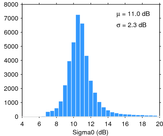
Figure 25. Histogram of flag-valid sigma0 over oceans and lakes for 04/05/2015. The mean ( \mu ) and standard deviation ( \sigma ) are also shown. Note that values outside [4 20] dB are excluded from the histogram for the sake of readability but not from the computation of \mu and \sigma .
