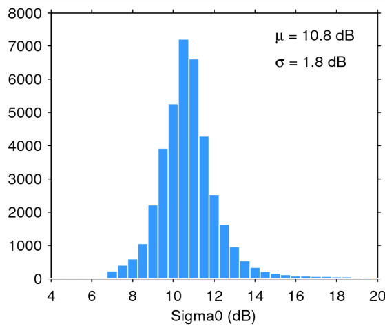
Figure 28. Histogram of science-valid sigma0 over oceans and lakes for 04/05/2015. The mean ( \mu ) and standard deviation ( \sigma ) are also shown. Note that values outside [4 20] dB are excluded from the histogram for the sake of readability but not from the computation of \mu and \sigma .
