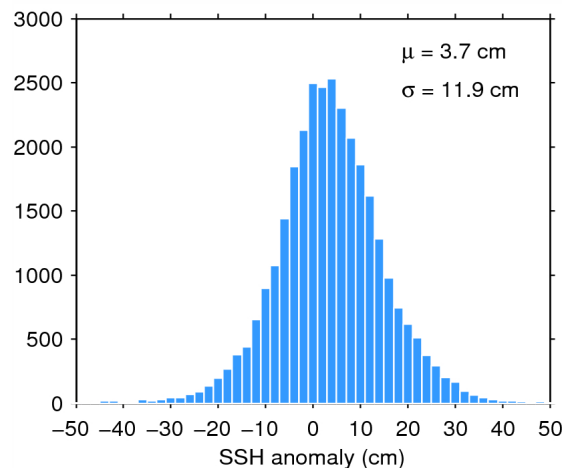
Figure 11. Histogram of science-valid SSH anomaly over oceans and lakes for 03/05/2015. The mean ( \mu ) and standard deviation ( \sigma ) are also shown. Note that values outside [-50 50] cm are excluded from the histogram for the sake of readability but not from the computation of \mu and \sigma .
