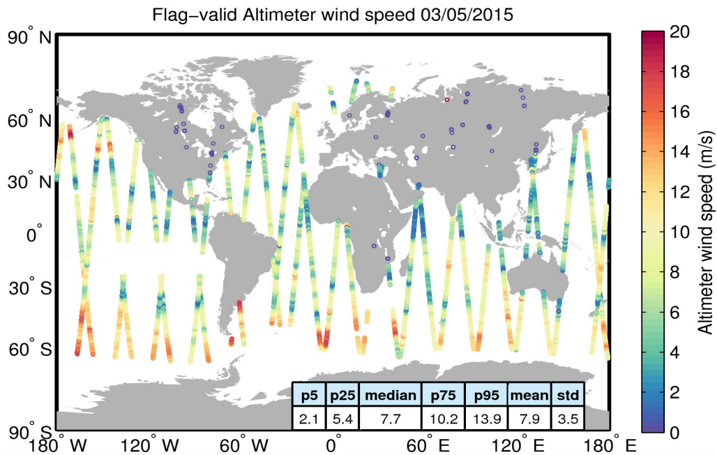
Figure 31. Geographical distribution of flag-valid wind data over oceans and lakes for 03/05/2015. The statistical values shown in the table refer to the wind in m/s and are calculated over all measurements shown in the figure.
