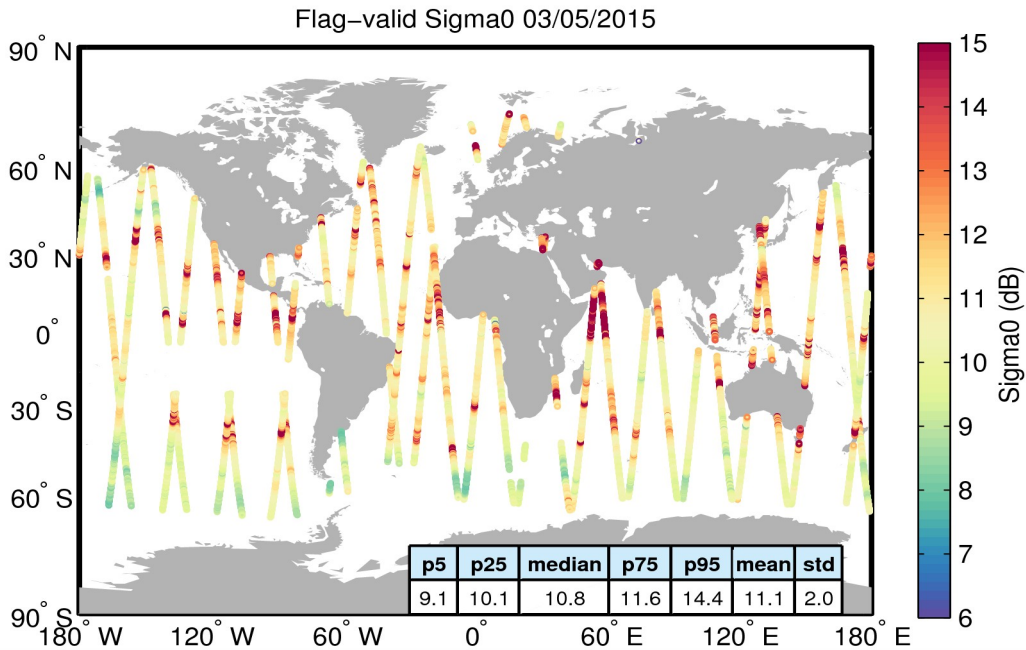
Figure 23. Geographical distribution of flag-valid sigma0 data over oceans and lakes for 03/05/2015. The statistical values shown in the table refer to the sigma0 in dB and are calculated over all measurements shown in the figure.
