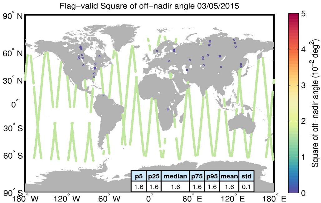
Figure 37. Geographical distribution of flag-valid mispointing data over oceans and lakes for 03/05/2015. The statistical values shown in the table refer to the mispointing in 10^{-2} \text{ deg}^2 and are calculated over all measurements shown in the figure.
