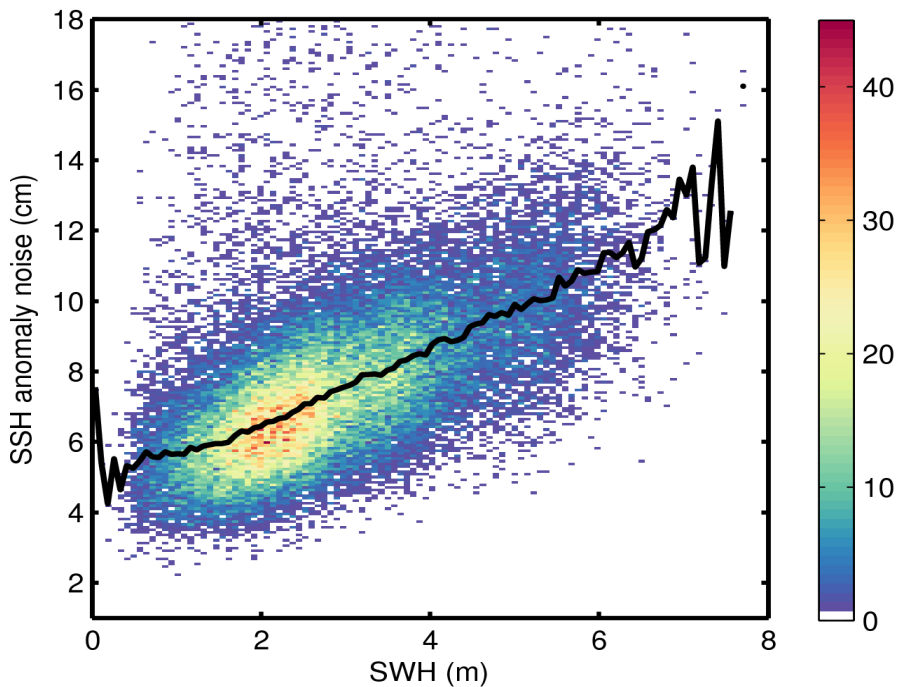
Figure 9. 2D histogram showing flag-valid SSH anomaly noise as a function of SWH for 03/05/2015. The black line denotes the median SSH anomaly as a function of SWH.
