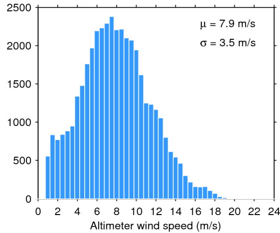
Figure 33. Histogram of flag-valid wind over oceans and lakes for 03/05/2015. The mean ( \mu ) and standard deviation ( \sigma ) are also shown. Note that values larger than 24 m/s are excluded from the histogram for the sake of readability but not from the computation of \mu and \sigma .
