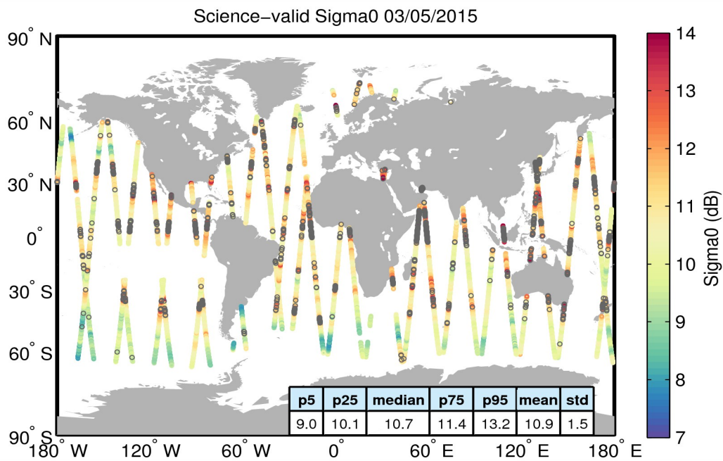
Figure 27. Geographical distribution of science-valid sigma0 data over oceans and lakes for 03/05/2015. The statistical values shown in the table refer to the sigma0 in dB and are calculated over all measurements shown in the figure. Gray circles denote records that have been rejected based on the editing criteria described in Table 4.
