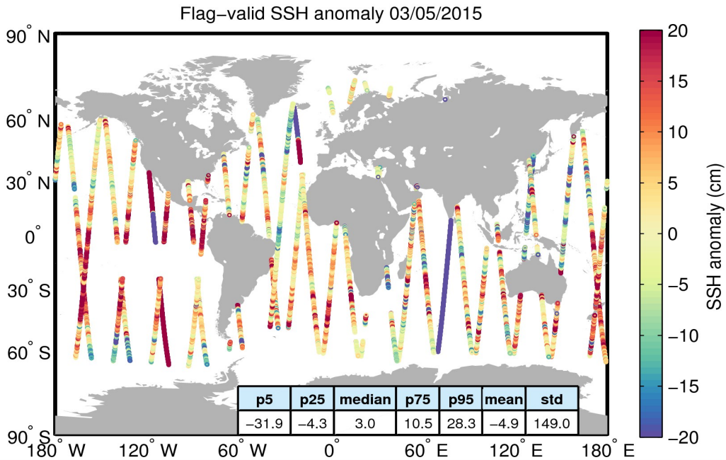
Figure 5. Geographical distribution of flag-valid 1-Hz SSH anomaly data over oceans and lakes for 03/05/2015. The statistical values shown in the table refer to the SSH anomaly in cm and are calculated over all measurements shown in the figure.
