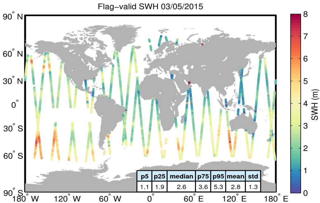
Figure 15. Geographical distribution of flag-valid SWH data over oceans and lakes for 03/05/2015. The statistical values shown in the figure refer to the SWH in m and are calculated over all measurements shown in the figure.
