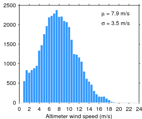
Figure 35. Histogram of science-valid wind over oceans and lakes for 03/05/2015. The mean ( \mu ) and standard deviation ( \sigma ) are also shown. Note that values larger than 24 m/s are excluded from the histogram for the sake of readability but not from the computation of \mu and \sigma .
