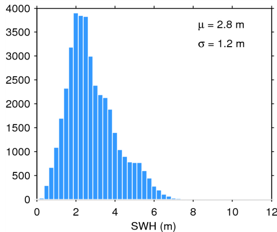
Figure 20. Histogram of science-valid SWH over oceans and lakes for 03/05/2015. The mean ( \mu ) and standard deviation ( \sigma ) are also shown. Note that values larger than 12 m are excluded from the histogram for the sake of readability but not from the computation of \mu and \sigma .
