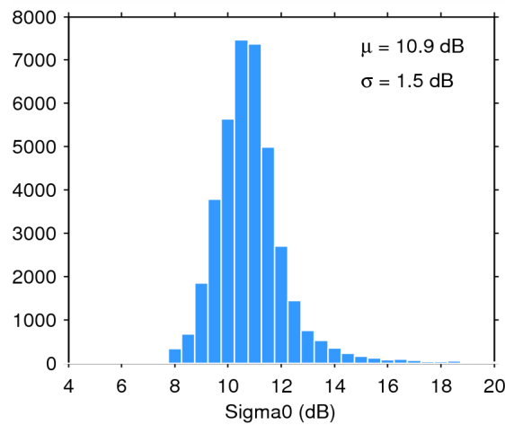
Figure 28. Histogram of science-valid sigma0 over oceans and lakes for 03/05/2015. The mean ( \mu ) and standard deviation ( \sigma ) are also shown. Note that values outside [4 20] dB are excluded from the histogram for the sake of readability but not from the computation of \mu and \sigma .
