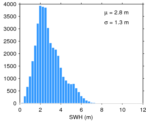
Figure 17. Histogram of flag-valid SWH over oceans and lakes for 03/05/2015. The mean ( \mu ) and standard deviation ( \sigma ) are also shown. Note that values larger than 12 m are excluded from the histogram for the sake of readability but not from the computation of \mu and \sigma .
