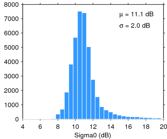
Figure 25. Histogram of flag-valid sigma0 over oceans and lakes for 03/05/2015. The mean ( \mu ) and standard deviation ( \sigma ) are also shown. Note that values outside [4 20] dB are excluded from the histogram for the sake of readability but not from the computation of \mu and \sigma .
