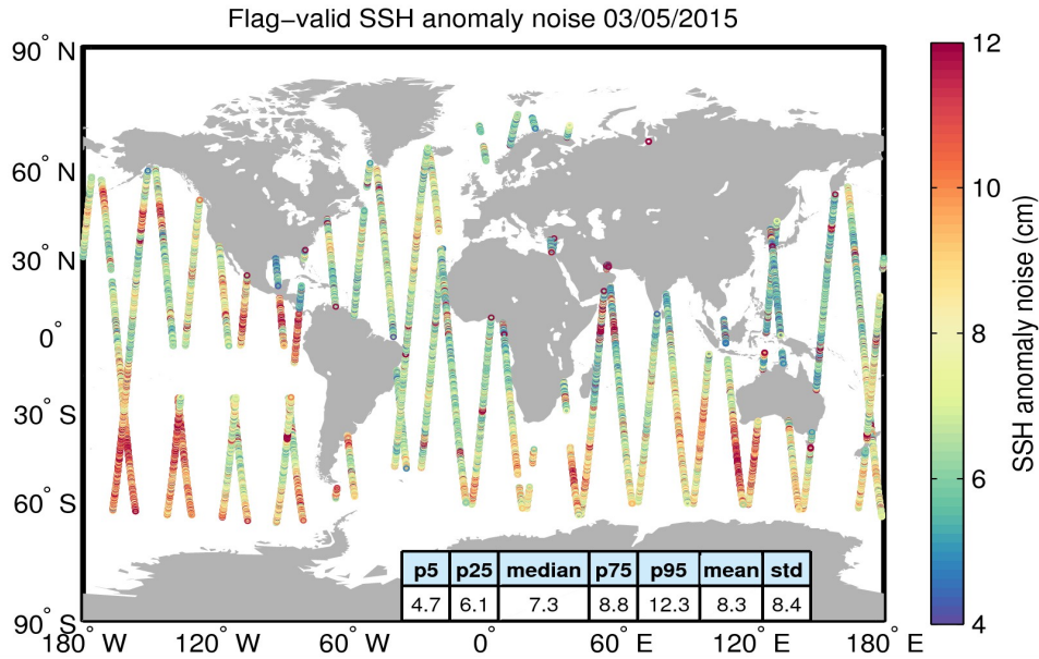
Figure 8. Geographical distribution of flag-valid 20-Hz SSH anomaly measurement noise over oceans and lakes for 03/05/2015. The statistical values shown in the table refer to the SSH anomaly noise and are calculated over all measurements shown in the figure.
