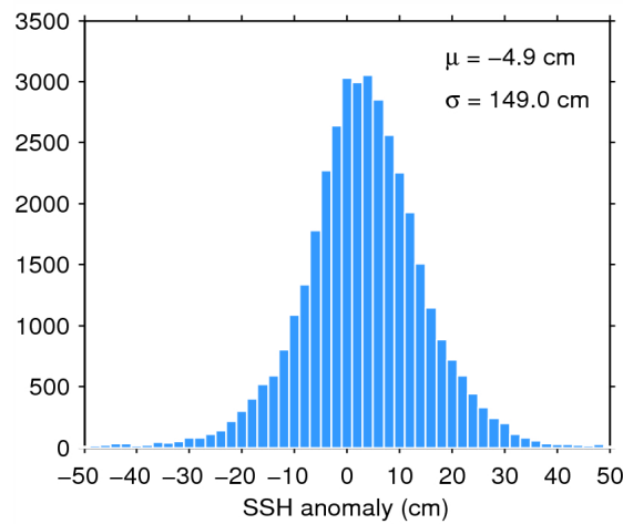
Figure 7. Histogram of flag-valid SSH anomaly over oceans and lakes for 03/05/2015. The mean ( \mu ) and standard deviation ( \sigma ) are also shown. Note that values outside [-50\ 50] cm are excluded from the histogram for the sake of readability but not from the computation of \mu and \sigma .
