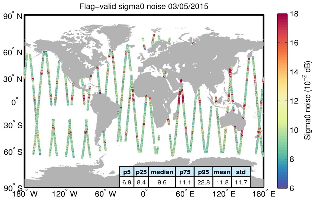
Figure 26. Geographical distribution of flag-valid 20-Hz sigma0 measurement noise over oceans and lakes for 03/05/2015. The statistical values shown in the table refer to the sigma0 noise and are calculated over all measurements shown in the figure.
