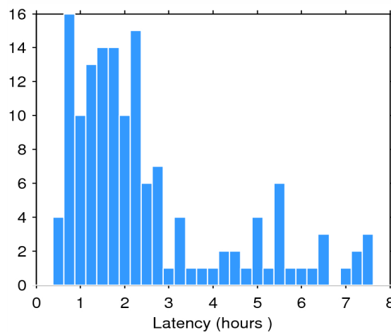
Figure 2. Histogram of the data latency for 03/05/2015. The y-axis denotes the number of files that are made available with a delay of x-hours with respect to the mean time of the records stored in the file.
