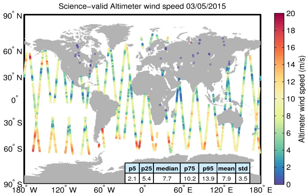
Figure 34. Geographical distribution of science-valid wind data over oceans and lakes for 03/05/2015. The statistical values shown in the table refer to the wind in m/s and are calculated over all measurements shown in the figure. Gray circles denote records that have been rejected based on the editing criteria described in Table 5.
