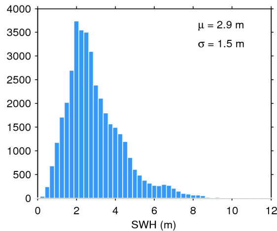
Figure 17. Histogram of flag-valid SWH over oceans and lakes for 02/05/2015. The mean ( \mu ) and standard deviation ( \sigma ) are also shown. Note that values larger than 12 m are excluded from the histogram for the sake of readability but not from the computation of \mu and \sigma .
