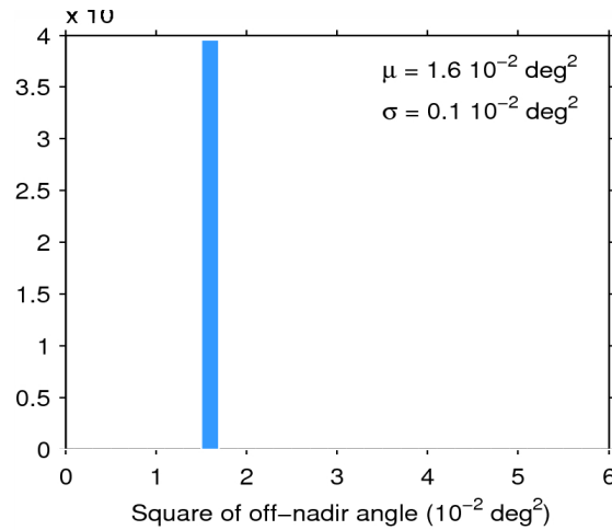
Figure 39. Histogram of flag-valid mispointing over oceans and lakes for 02/05/2015. The mean ( \mu ) and standard deviation ( \sigma ) are also shown. Note that values than 6 \cdot 10^{-2} \text{ deg}^2 are excluded from the histogram for the sake of readability but not from the computation of \mu and \sigma .
