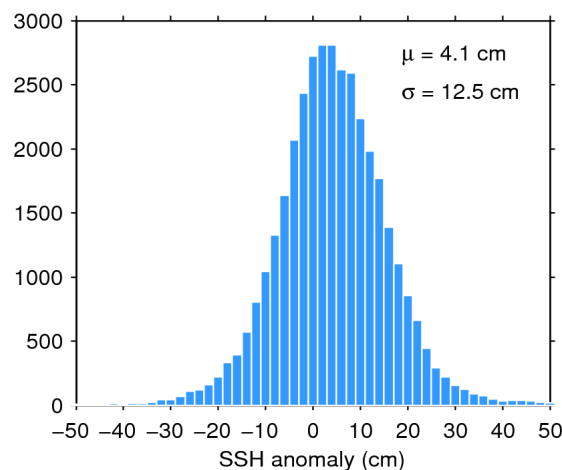
Figure 11. Histogram of science-valid SSH anomaly over oceans and lakes for 02/05/2015. The mean ( \mu ) and standard deviation ( \sigma ) are also shown. Note that values outside [-50 50] cm are excluded from the histogram for the sake of readability but not from the computation of \mu and \sigma .
