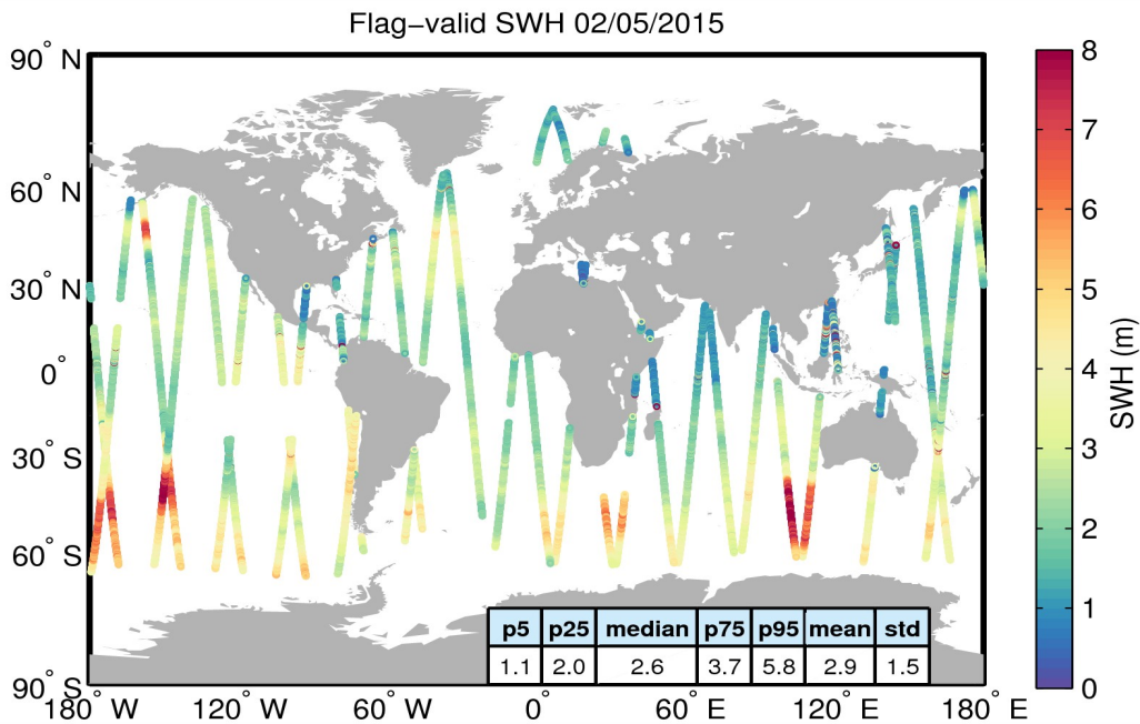
Figure 15. Geographical distribution of flag-valid SWH data over oceans and lakes for 02/05/2015. The statistical values shown in the table refer to the SWH in m and are calculated over all measurements shown in the figure.
