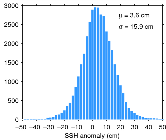
Figure 7. Histogram of flag-valid SSH anomaly over oceans and lakes for 02/05/2015. The mean ( \mu ) and standard deviation ( \sigma ) are also shown. Note that values outside [-50 50] cm are excluded from the histogram for the sake of readability but not from the computation of \mu and \sigma .
