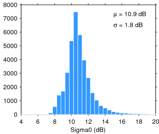
Figure 28. Histogram of science-valid sigma0 over oceans and lakes for 02/05/2015. The mean ( \mu ) and standard deviation ( \sigma ) are also shown. Note that values outside [4 20] dB are excluded from the histogram for the sake of readability but not from the computation of \mu and \sigma .
