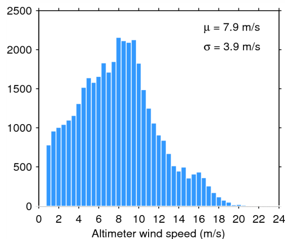
Figure 35. Histogram of science-valid wind over oceans and lakes for 02/05/2015. The mean ( \mu ) and standard deviation ( \sigma ) are also shown. Note that values larger than 24 m/s are excluded from the histogram for the sake of readability but not from the computation of \mu and \sigma .
