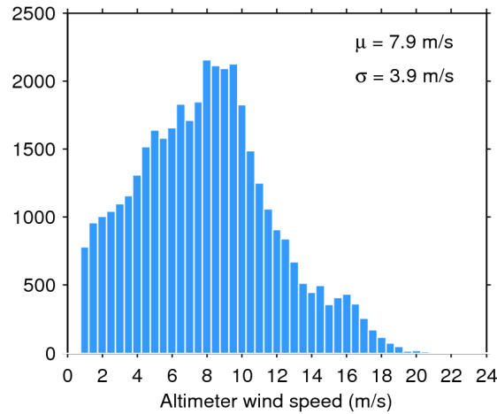
Figure 33. Histogram of flag-valid wind over oceans and lakes for 02/05/2015. The mean ( \mu ) and standard deviation ( \sigma ) are also shown. Note that values larger than 24 m/s are excluded from the histogram for the sake of readability but not from the computation of \mu and \sigma .
