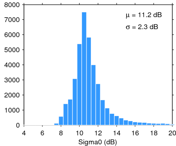
Figure 25. Histogram of flag-valid sigma0 over oceans and lakes for 02/05/2015. The mean ( \mu ) and standard deviation ( \sigma ) are also shown. Note that values outside [4 20] dB are excluded from the histogram for the sake of readability but not from the computation of \mu and \sigma .
