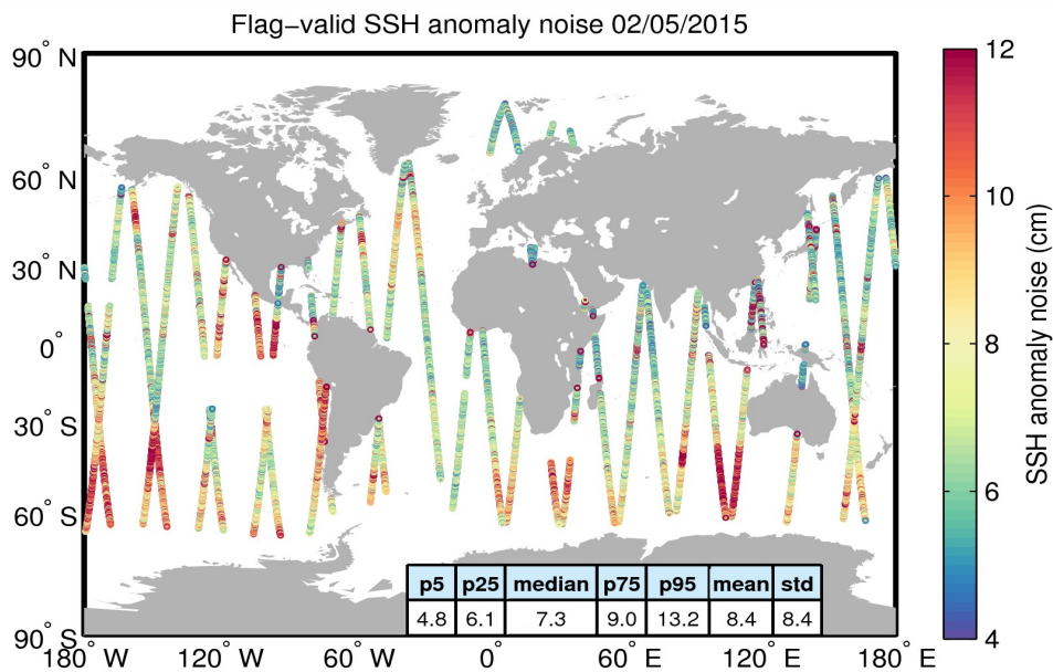
Figure 8. Geographical distribution of flag-valid 20-Hz SSH anomaly measurement noise over oceans and lakes for 02/05/2015. The statistical values shown in the table refer to the SSH anomaly noise and are calculated over all measurements shown in the figure.
