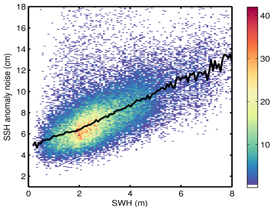
Figure 9. 2D histogram showing flag-valid SSH anomaly noise as a function of SWH for 02/05/2015. The black line denotes the median SSH anomaly as a function of SWH.
