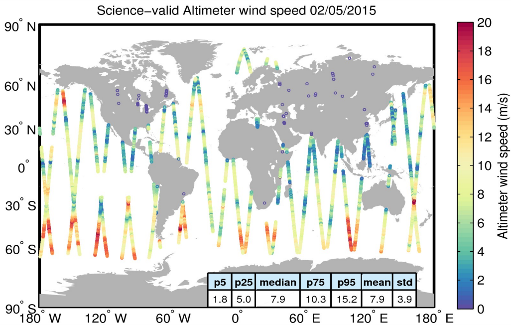
Figure 34. Geographical distribution of science-valid wind data over oceans and lakes for 02/05/2015. The statistical values shown in the table refer to the wind in m/s and are calculated over all measurements shown in the figure. Gray circles denote records that have been rejected based on the editing criteria described in Table 5.
