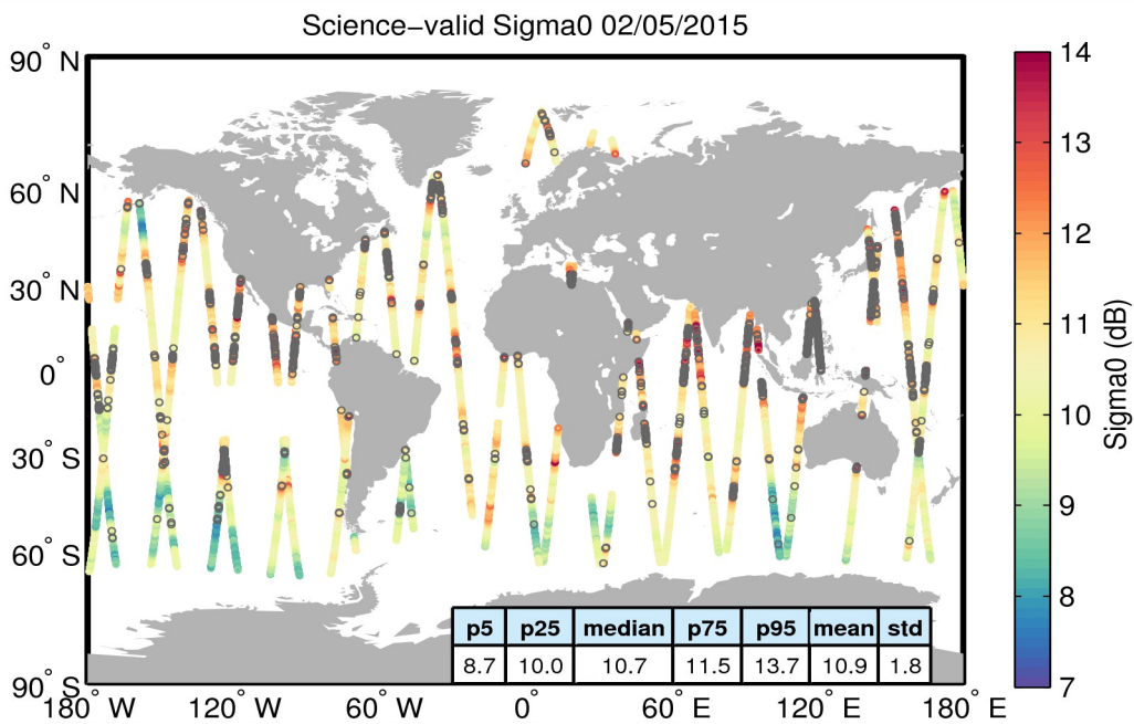
Figure 27. Geographical distribution of science-valid sigma0 data over oceans and lakes for 02/05/2015. The statistical values shown in the table refer to the sigma0 in dB and are calculated over all measurements shown in the figure. Gray circles denote records that have been rejected based on the editing criteria described in Table 4.
