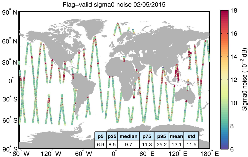
Figure 26. Geographical distribution of flag-valid 20-Hz sigma0 measurement noise over oceans and lakes for 02/05/2015. The statistical values shown in the table refer to the sigma0 noise and are calculated over all measurements shown in the figure.
