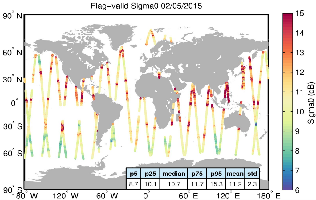
Figure 23. Geographical distribution of flag-valid sigma0 data over oceans and lakes for 02/05/2015. The statistical values shown in the table refer to the sigma0 in dB and are calculated over all measurements shown in the figure.
