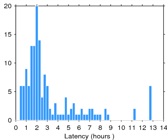
Figure 2. Histogram of the data latency for 02/05/2015. The y-axis denotes the number of files that are made available with a delay of x-hours with respect to the mean time of the records stored in the file.
