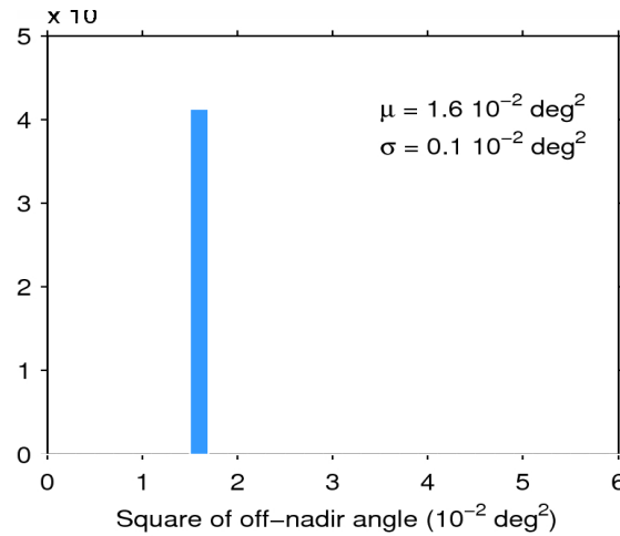
Figure 39. Histogram of flag-valid mispointing over oceans and lakes for 01/05/2015. The mean ( \mu ) and standard deviation ( \sigma ) are also shown. Note that values than 6 \cdot 10^{-2} \text{ deg}^2 are excluded from the histogram for the sake of readability but not from the computation of \mu and \sigma .
