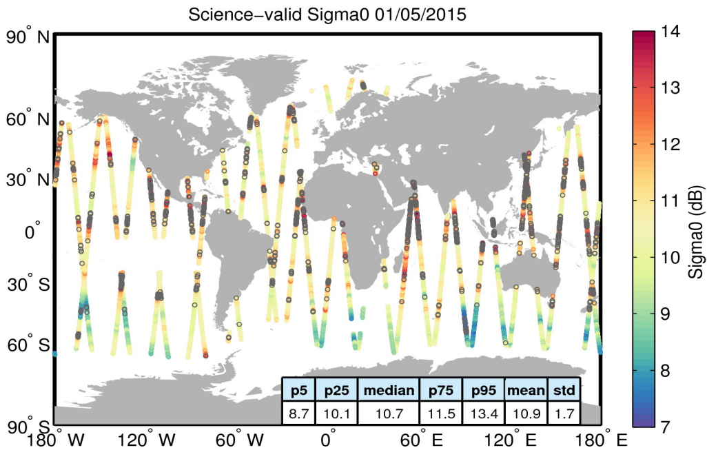
Figure 27. Geographical distribution of science-valid sigma0 data over oceans and lakes for 01/05/2015. The statistical values shown in the table refer to the sigma0 in dB and are calculated over all measurements shown in the figure. Gray circles denote records that have been rejected based on the editing criteria described in Table 4.
