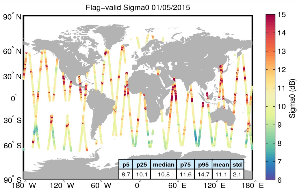
Figure 23. Geographical distribution of flag-valid sigma0 data over oceans and lakes for 01/05/2015. The statistical values shown in the table refer to the sigma0 in dB and are calculated over all measurements shown in the figure.
