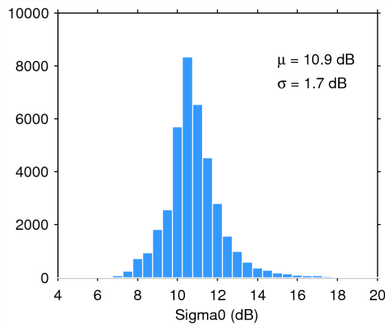
Figure 28. Histogram of science-valid sigma0 over oceans and lakes for 01/05/2015. The mean ( \mu ) and standard deviation ( \sigma ) are also shown. Note that values outside [4 20] dB are excluded from the histogram for the sake of readability but not from the computation of \mu and \sigma .
