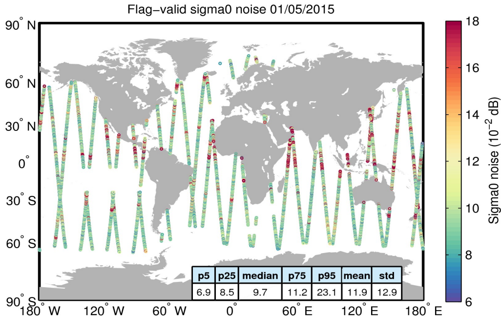
Figure 26. Geographical distribution of flag-valid 20-Hz sigma0 measurement noise over oceans and lakes for 01/05/2015. The statistical values shown in the table refer to the sigma0 noise and are calculated over all measurements shown in the figure.
