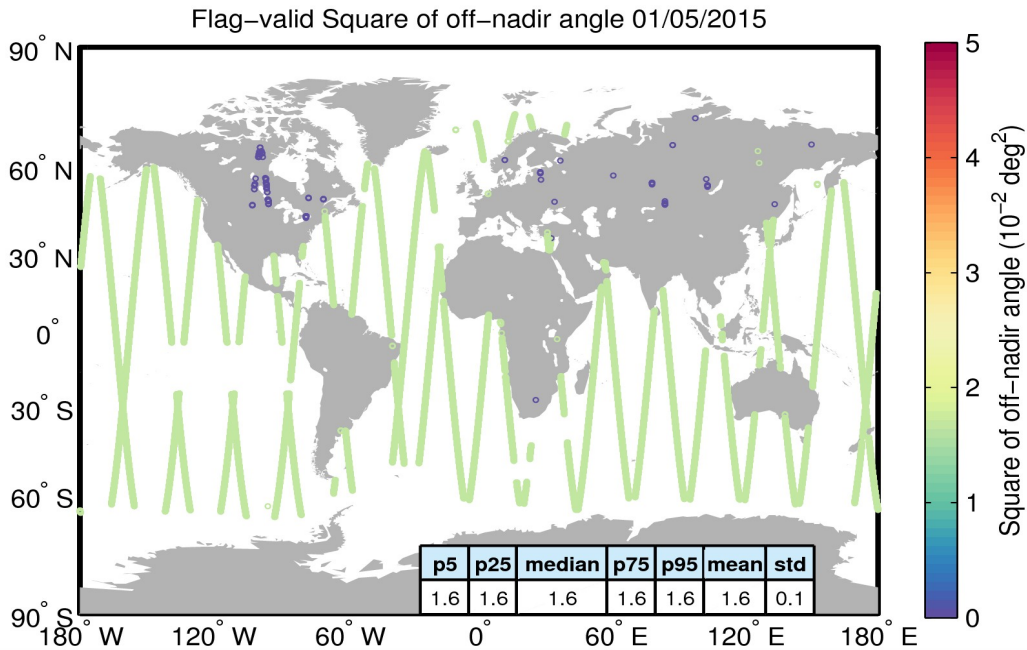
Figure 37. Geographical distribution of flag-valid mispointing data over oceans and lakes for 01/05/2015. The statistical values shown in the table refer to the mispointing in 10^{-2} \text{ deg}^2 and are calculated over all measurements shown in the figure.
