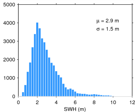
Figure 20. Histogram of science-valid SWH over oceans and lakes for 01/05/2015. The mean ( \mu ) and standard deviation ( \sigma ) are also shown. Note that values larger than 12 m are excluded from the histogram for the sake of readability but not from the computation of \mu and \sigma .
