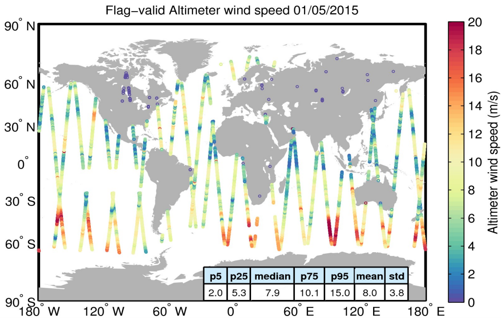
Figure 31. Geographical distribution of flag-valid wind data over oceans and lakes for 01/05/2015. The statistical values shown in the table refer to the wind in m/s and are calculated over all measurements shown in the figure.
