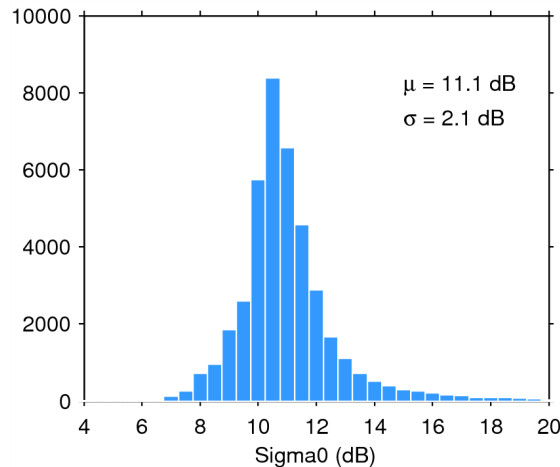
Figure 25. Histogram of flag-valid sigma0 over oceans and lakes for 01/05/2015. The mean ( \mu ) and standard deviation ( \sigma ) are also shown. Note that values outside [4 20] dB are excluded from the histogram for the sake of readability but not from the computation of \mu and \sigma .
