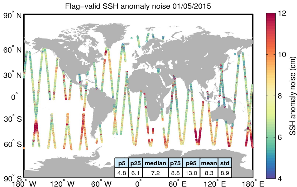
Figure 8. Geographical distribution of flag-valid 20-Hz SSH anomaly measurement noise over oceans and lakes for 01/05/2015. The statistical values shown in the table refer to the SSH anomaly noise and are calculated over all measurements shown in the figure.
