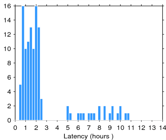
Figure 2. Histogram of the data latency for 01/05/2015. The y-axis denotes the number of files that are made available with a delay of x-hours with respect to the mean time of the records stored in the file.
