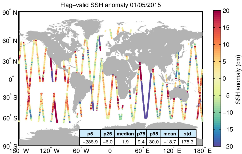
Figure 5. Geographical distribution of flag-valid 1-Hz SSH anomaly data over oceans and lakes for 01/05/2015. The statistical values shown in the table refer to the SSH anomaly in cm and are calculated over all measurements shown in the figure.
