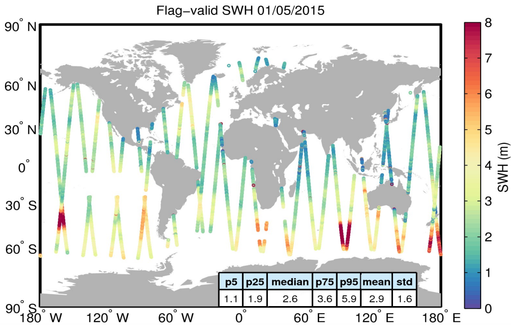
Figure 15. Geographical distribution of flag-valid SWH data over oceans and lakes for 01/05/2015. The statistical values shown in the table refer to the SWH in m and are calculated over all measurements shown in the figure.
