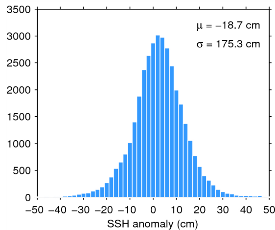
Figure 7. Histogram of flag-valid SSH anomaly over oceans and lakes for 01/05/2015. The mean ( \mu ) and standard deviation ( \sigma ) are also shown. Note that values outside [-50\ 50] cm are excluded from the histogram for the sake of readability but not from the computation of \mu and \sigma .
