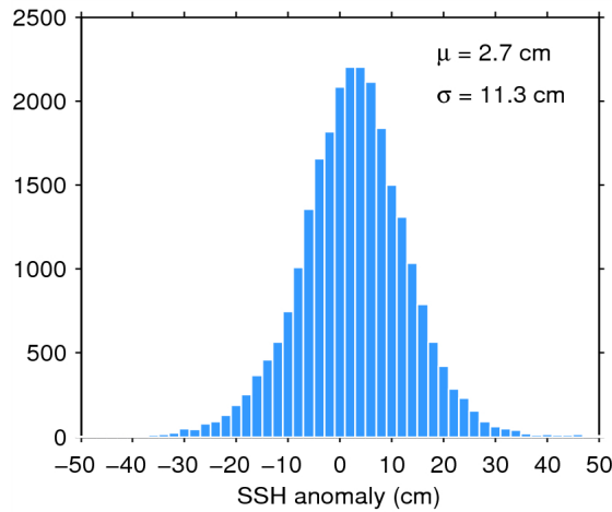
Figure 11. Histogram of science-valid SSH anomaly over oceans and lakes for 01/05/2015. The mean ( \mu ) and standard deviation ( \sigma ) are also shown. Note that values outside [-50 50] cm are excluded from the histogram for the sake of readability but not from the computation of \mu and \sigma .
