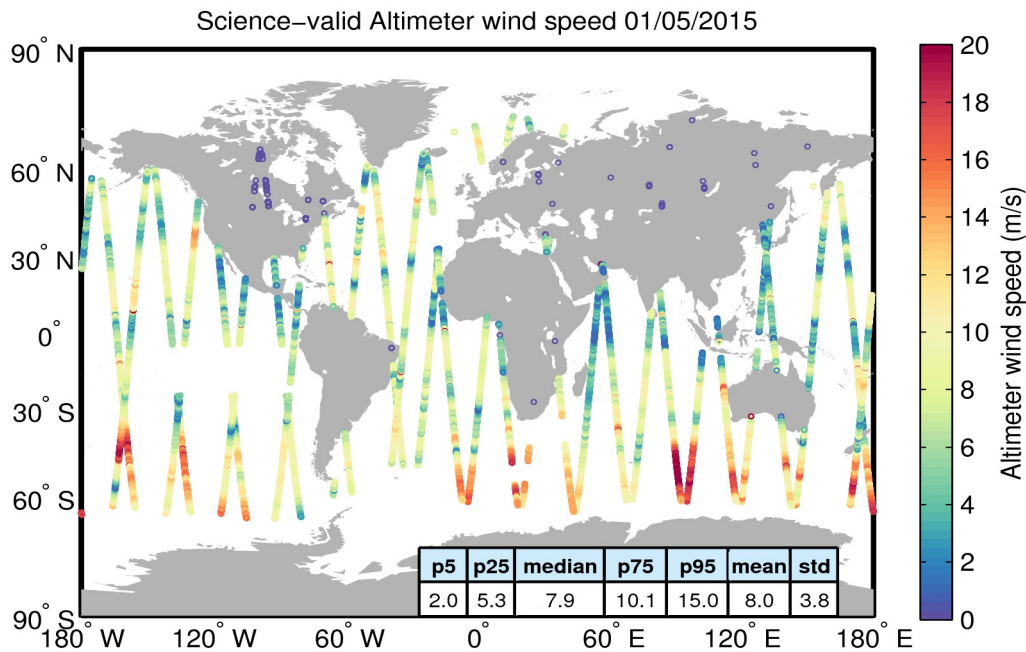
Figure 34. Geographical distribution of science-valid wind data over oceans and lakes for 01/05/2015. The statistical values shown in the table refer to the wind in m/s and are calculated over all measurements shown in the figure. Gray circles denote records that have been rejected based on the editing criteria described in Table 5.
