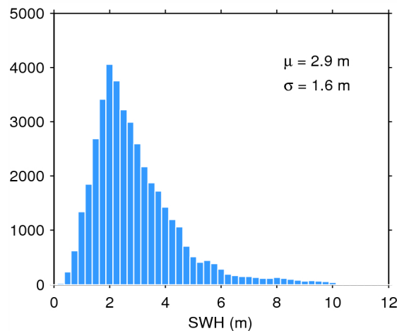
Figure 17. Histogram of flag-valid SWH over oceans and lakes for 01/05/2015. The mean ( \mu ) and standard deviation ( \sigma ) are also shown. Note that values larger than 12 m are excluded from the histogram for the sake of readability but not from the computation of \mu and \sigma .
