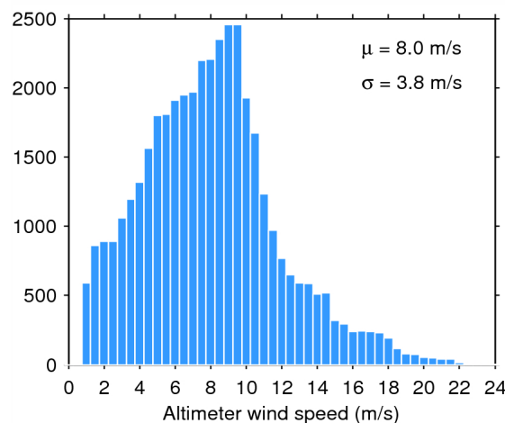
Figure 35. Histogram of science-valid wind over oceans and lakes for 01/05/2015. The mean ( \mu ) and standard deviation ( \sigma ) are also shown. Note that values larger than 24 m/s are excluded from the histogram for the sake of readability but not from the computation of \mu and \sigma .
