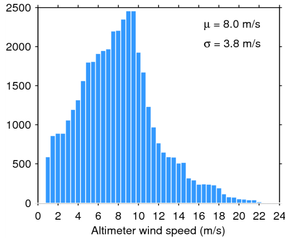
Figure 33. Histogram of flag-valid wind over oceans and lakes for 01/05/2015. The mean ( \mu ) and standard deviation ( \sigma ) are also shown. Note that values larger than 24 m/s are excluded from the histogram for the sake of readability but not from the computation of \mu and \sigma .
