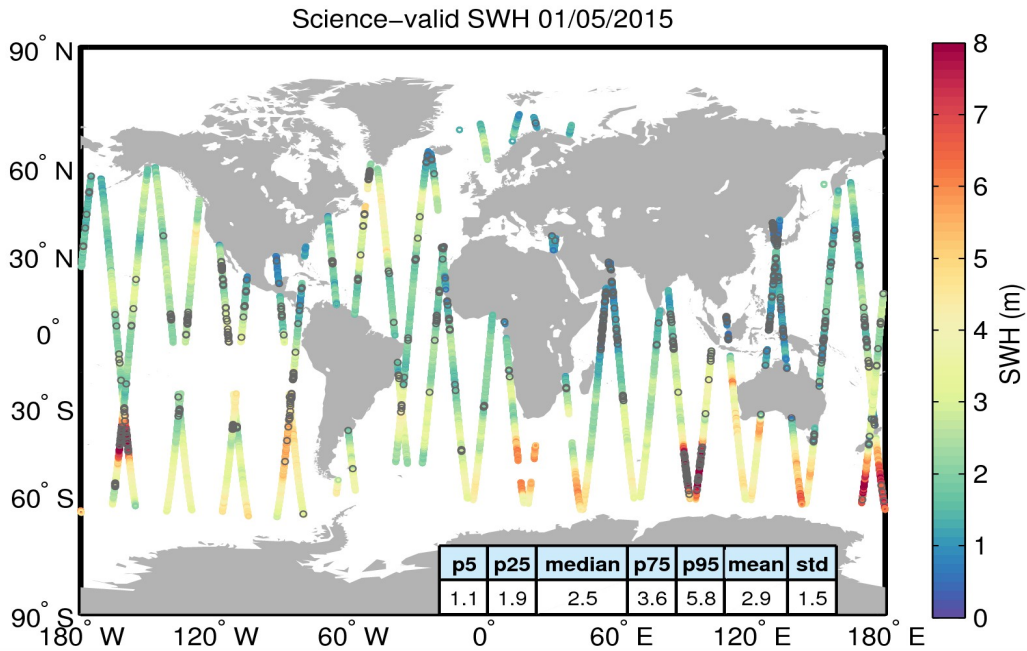
Figure 19. Geographical distribution of science-valid SWH data over oceans and lakes for 01/05/2015. The statistical values shown in the table refer to the SWH in m and are calculated over all measurements shown in the figure. Gray circles denote records that have been rejected based on the editing criteria described in Table 3.
