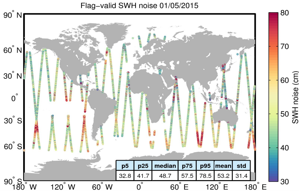
Figure 18. Geographical distribution of flag-valid 20-Hz SWH measurement noise over oceans and lakes for 01/05/2015. The statistical values shown in the figure refer to the SWH noise and are calculated over all measurements shown in the figure.
