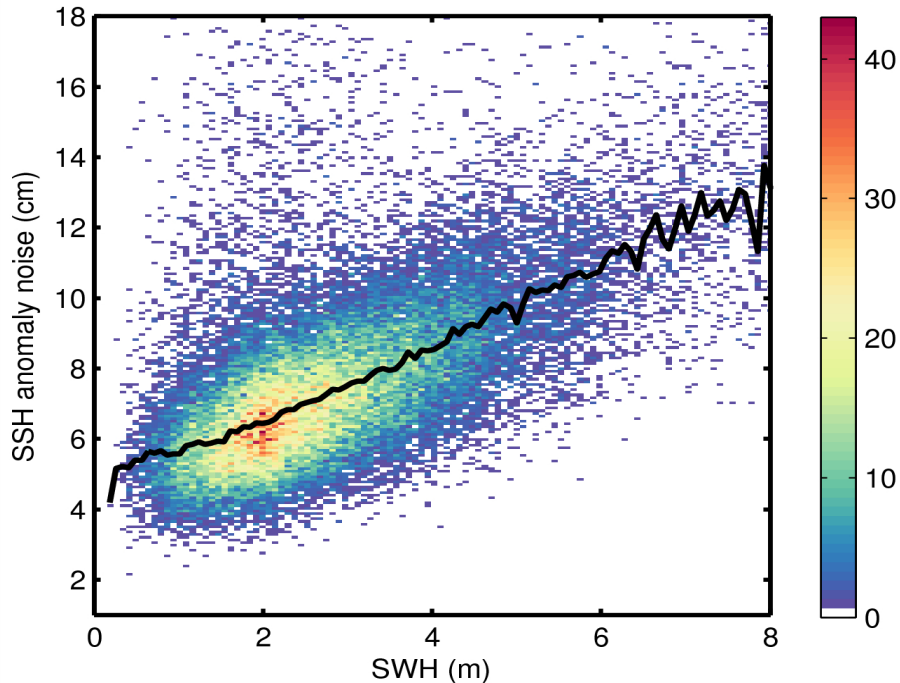
Figure 9. 2D histogram showing flag-valid SSH anomaly noise as a function of SWH for 01/05/2015. The black line denotes the median SSH anomaly as a function of SWH.
