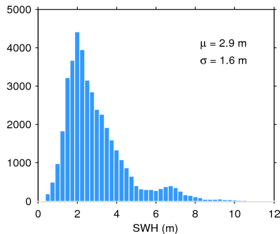
Figure 20. Histogram of science-valid SWH over oceans and lakes for 29/04/2015. The mean ( \mu ) and standard deviation ( \sigma ) are also shown. Note that values larger than 12 m are excluded from the histogram for the sake of readability but not from the computation of \mu and \sigma .
