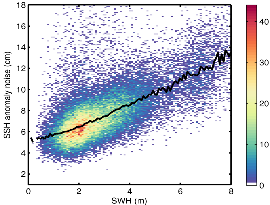
Figure 9. 2D histogram showing flag-valid SSH anomaly noise as a function of SWH for 29/04/2015. The black line denotes the median SSH anomaly as a function of SWH.
