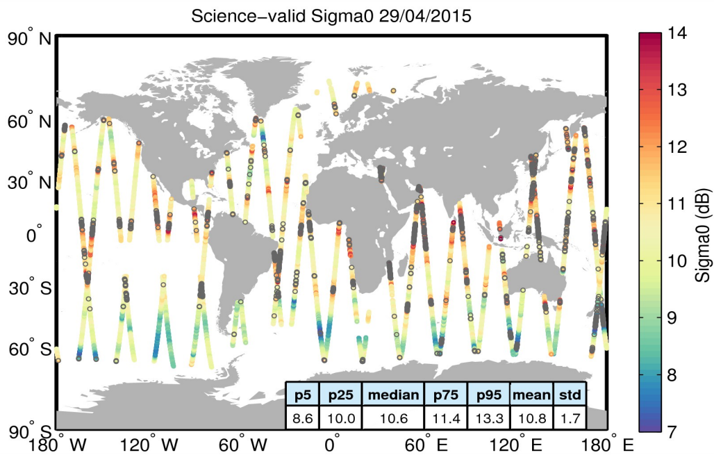
Figure 27. Geographical distribution of science-valid sigma0 data over oceans and lakes for 29/04/2015. The statistical values shown in the table refer to the sigma0 in dB and are calculated over all measurements shown in the figure. Gray circles denote records that have been rejected based on the editing criteria described in Table 4.
