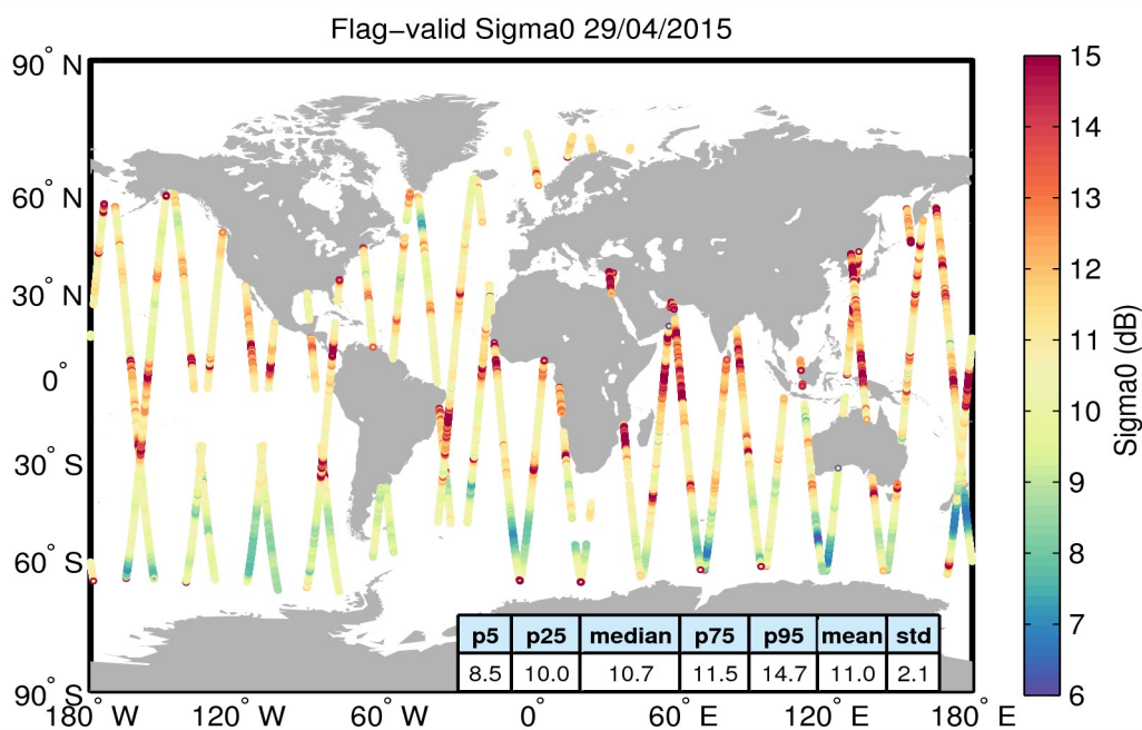
Figure 23. Geographical distribution of flag-valid sigma0 data over oceans and lakes for 29/04/2015. The statistical values shown in the table refer to the sigma0 in dB and are calculated over all measurements shown in the figure.
