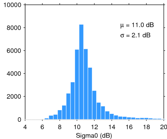
Figure 25. Histogram of flag-valid sigma0 over oceans and lakes for 29/04/2015. The mean ( \mu ) and standard deviation ( \sigma ) are also shown. Note that values outside [4 20] dB are excluded from the histogram for the sake of readability but not from the computation of \mu and \sigma .
