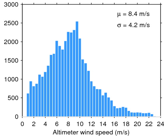
Figure 33. Histogram of flag-valid wind over oceans and lakes for 29/04/2015. The mean ( \mu ) and standard deviation ( \sigma ) are also shown. Note that values larger than 24 m/s are excluded from the histogram for the sake of readability but not from the computation of \mu and \sigma .
