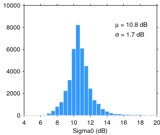
Figure 28. Histogram of science-valid sigma0 over oceans and lakes for 29/04/2015. The mean ( \mu ) and standard deviation ( \sigma ) are also shown. Note that values outside [4 20] dB are excluded from the histogram for the sake of readability but not from the computation of \mu and \sigma .
