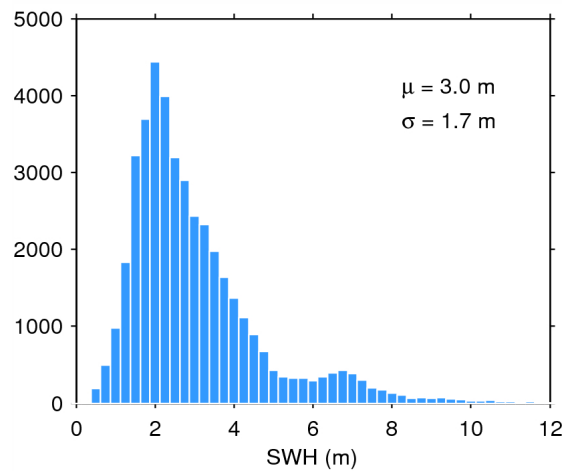
Figure 17. Histogram of flag-valid SWH over oceans and lakes for 29/04/2015. The mean ( \mu ) and standard deviation ( \sigma ) are also shown. Note that values larger than 12 m are excluded from the histogram for the sake of readability but not from the computation of \mu and \sigma .
