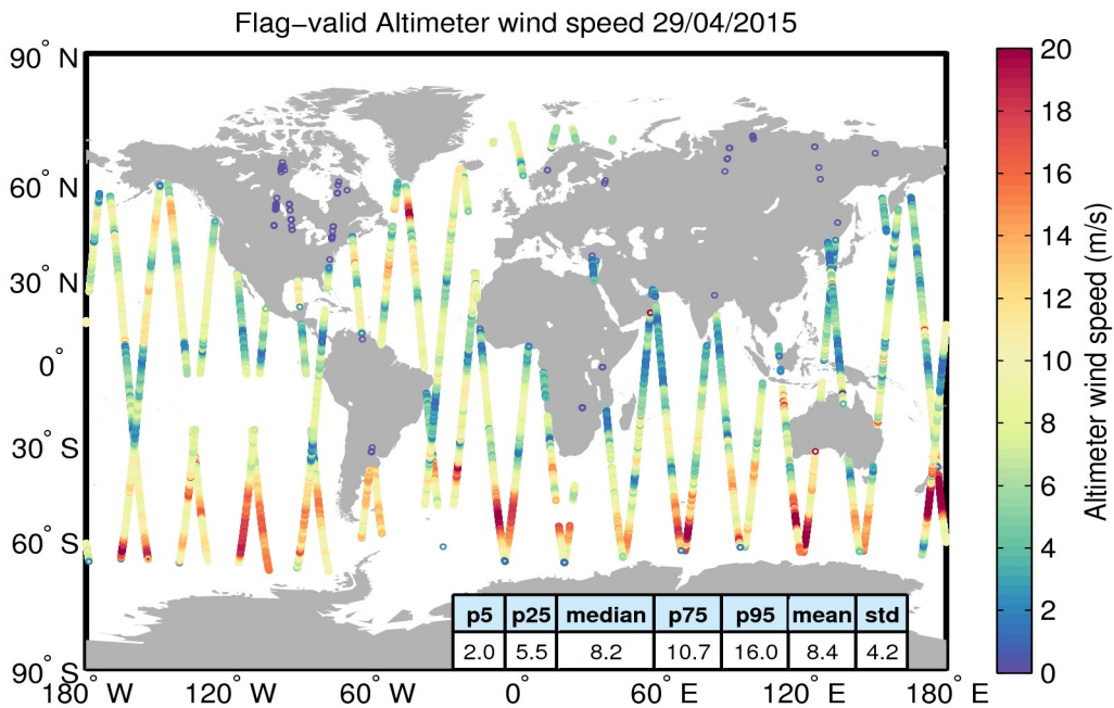
Figure 31. Geographical distribution of flag-valid wind data over oceans and lakes for 29/04/2015. The statistical values shown in the table refer to the wind in m/s and are calculated over all measurements shown in the figure.
