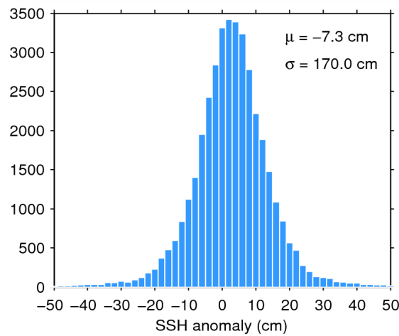
Figure 7. Histogram of flag-valid SSH anomaly over oceans and lakes for 29/04/2015. The mean ( \mu ) and standard deviation ( \sigma ) are also shown. Note that values outside [-50\ 50] cm are excluded from the histogram for the sake of readability but not from the computation of \mu and \sigma .
