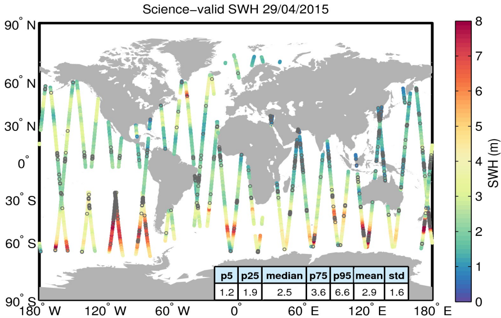
Figure 19. Geographical distribution of science-valid SWH data over oceans and lakes for 29/04/2015. The statistical values shown in the table refer to the SWH in m and are calculated over all measurements shown in the figure. Gray circles denote records that have been rejected based on the editing criteria described in Table 3.
