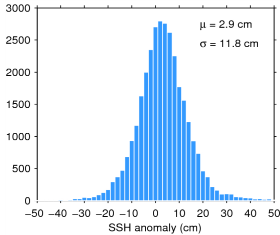
Figure 11. Histogram of science-valid SSH anomaly over oceans and lakes for 29/04/2015. The mean ( \mu ) and standard deviation ( \sigma ) are also shown. Note that values outside [-50 50] cm are excluded from the histogram for the sake of readability but not from the computation of \mu and \sigma .
