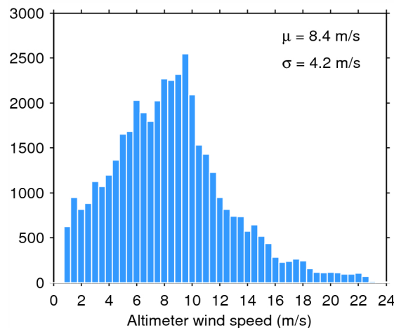
Figure 35. Histogram of science-valid wind over oceans and lakes for 29/04/2015. The mean ( \mu ) and standard deviation ( \sigma ) are also shown. Note that values larger than 24 m/s are excluded from the histogram for the sake of readability but not from the computation of \mu and \sigma .
