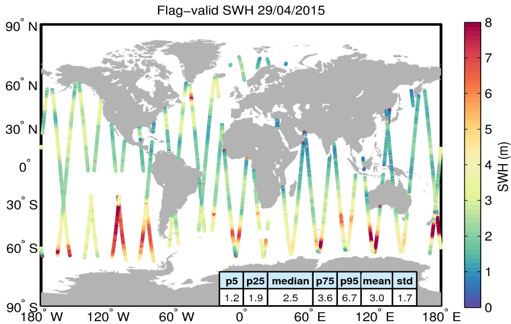
Figure 15. Geographical distribution of flag-valid SWH data over oceans and lakes for 29/04/2015. The statistical values shown in the table refer to the SWH in m and are calculated over all measurements shown in the figure.
