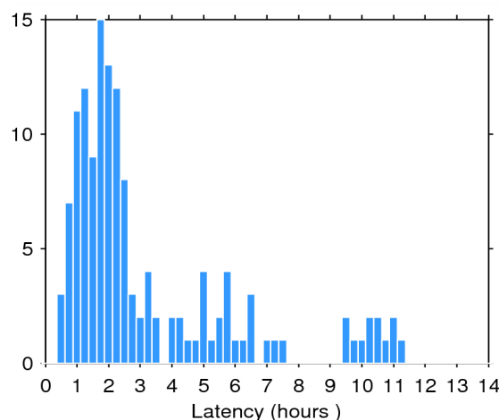
Figure 2. Histogram of the data latency for 29/04/2015. The y-axis denotes the number of files that are made available with a delay of x-hours with respect to the mean time of the records stored in the file.
