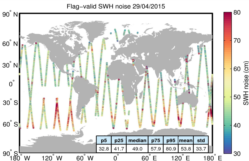
Figure 18. Geographical distribution of flag-valid 20-Hz SWH measurement noise over oceans and lakes for 29/04/2015. The statistical values shown in the figure refer to the SWH noise and are calculated over all measurements shown in the figure.
