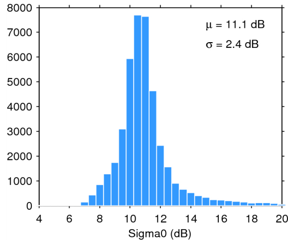
Figure 25. Histogram of flag-valid sigma0 over oceans and lakes for 25/04/2015. The mean ( \mu ) and standard deviation ( \sigma ) are also shown. Note that values outside [4 20] dB are excluded from the histogram for the sake of readability but not from the computation of \mu and \sigma .
