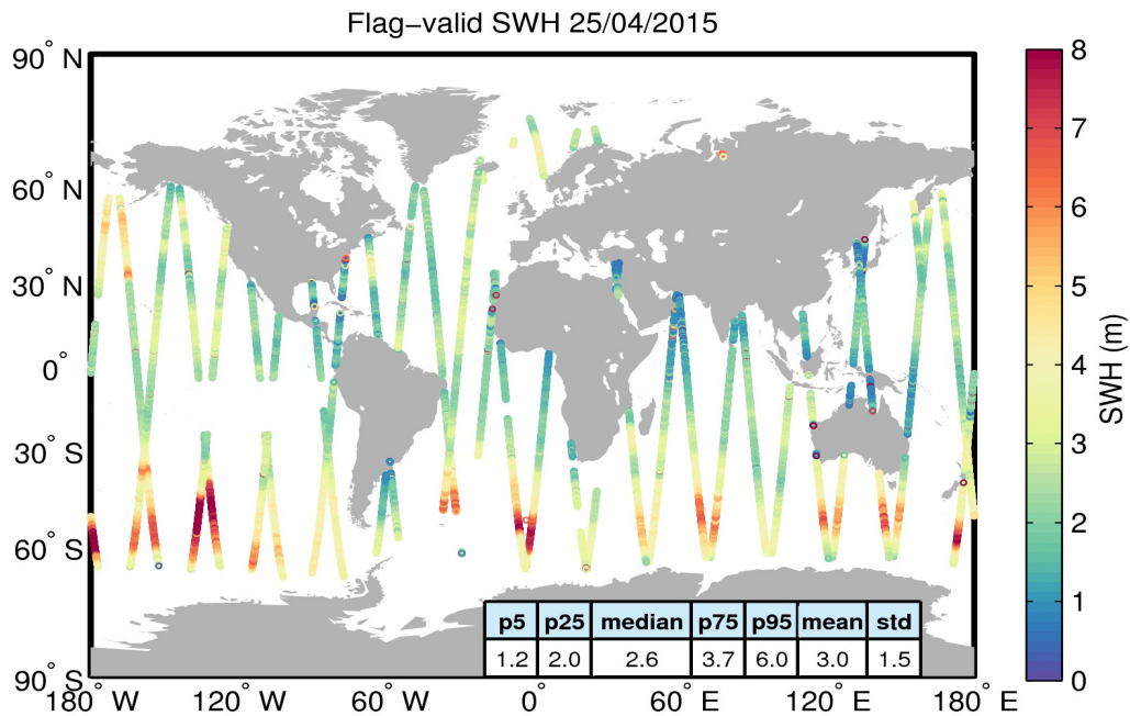
Figure 15. Geographical distribution of flag-valid SWH data over oceans and lakes for 25/04/2015. The statistical values shown in the table refer to the SWH in m and are calculated over all measurements shown in the figure.
