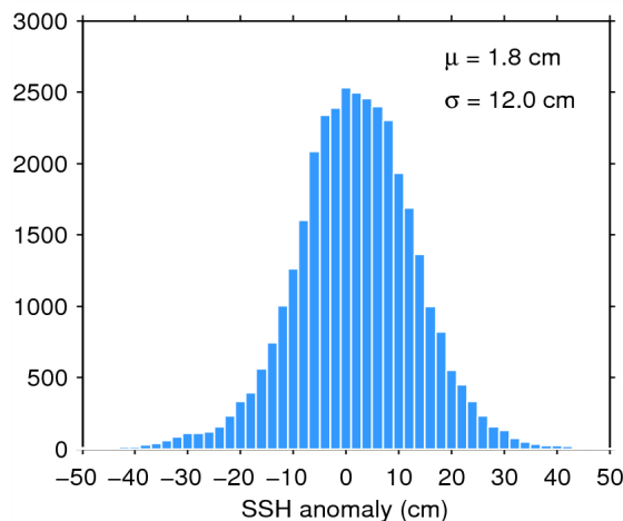
Figure 11. Histogram of science-valid SSH anomaly over oceans and lakes for 25/04/2015. The mean ( \mu ) and standard deviation ( \sigma ) are also shown. Note that values outside [-50 50] cm are excluded from the histogram for the sake of readability but not from the computation of \mu and \sigma .
