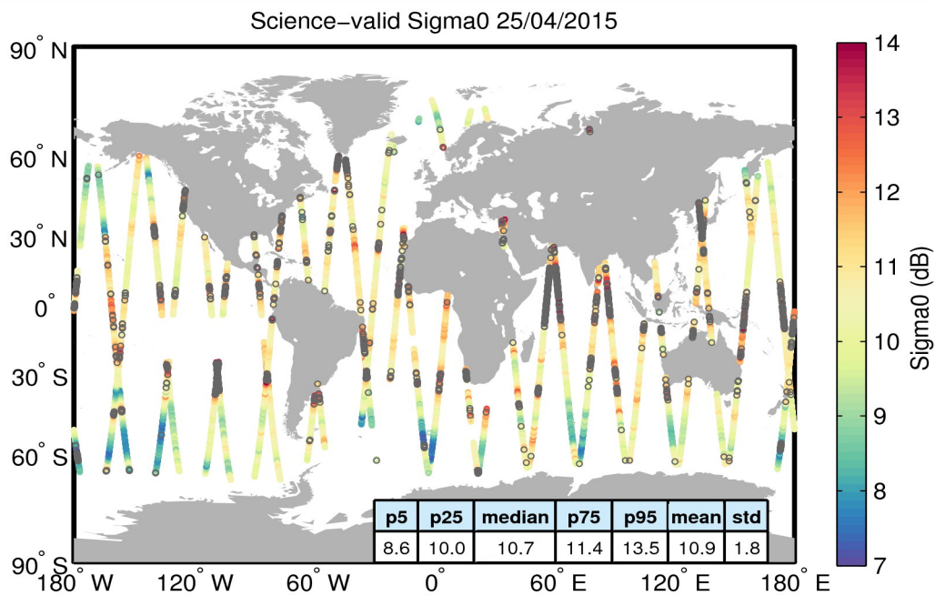
Figure 27. Geographical distribution of science-valid sigma0 data over oceans and lakes for 25/04/2015. The statistical values shown in the table refer to the sigma0 in dB and are calculated over all measurements shown in the figure. Gray circles denote records that have been rejected based on the editing criteria described in Table 4.
