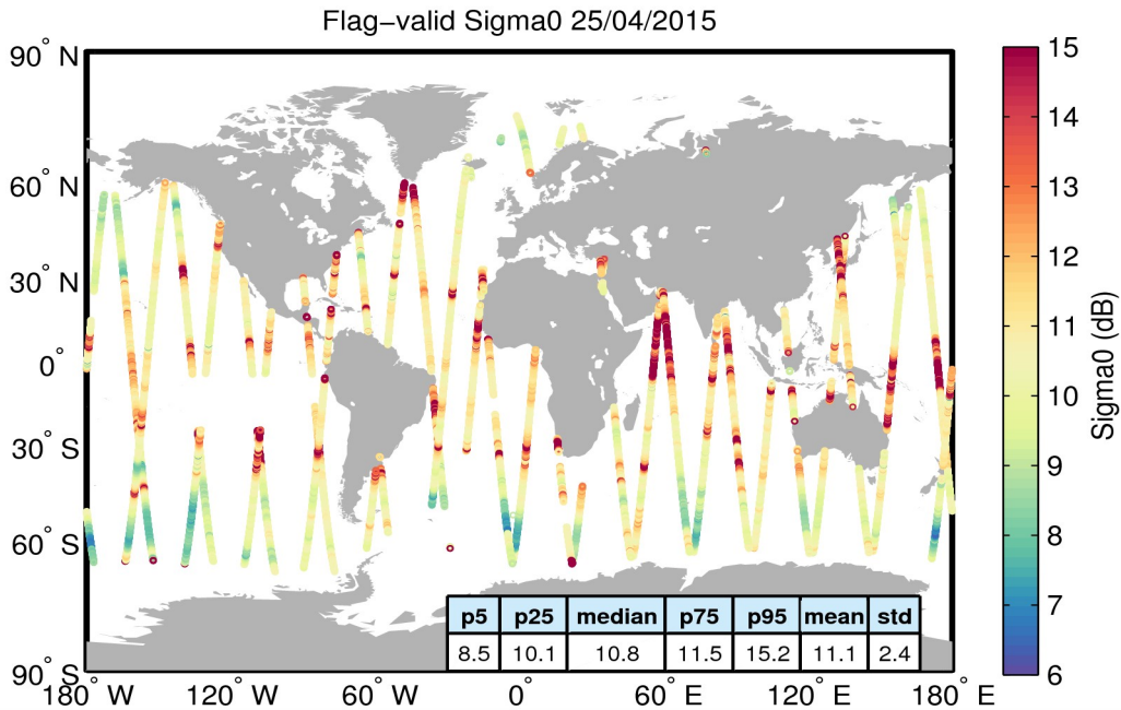
Figure 23. Geographical distribution of flag-valid sigma0 data over oceans and lakes for 25/04/2015. The statistical values shown in the table refer to the sigma0 in dB and are calculated over all measurements shown in the figure.
