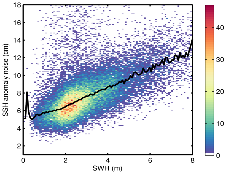
Figure 9. 2D histogram showing flag-valid SSH anomaly noise as a function of SWH for 25/04/2015. The black line denotes the median SSH anomaly as a function of SWH.
