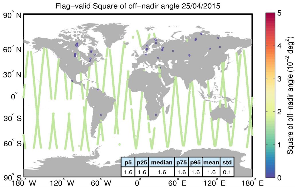
Figure 37. Geographical distribution of flag-valid mispointing data over oceans and lakes for 25/04/2015. The statistical values shown in the table refer to the mispointing in 10^{-2} deg 2 and are calculated over all measurements shown in the figure.
