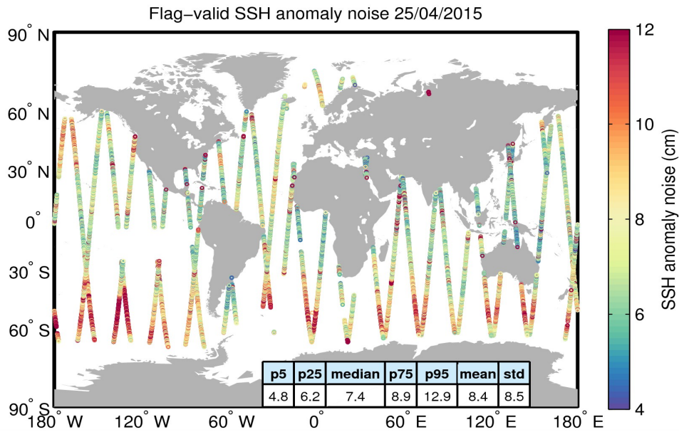
Figure 8. Geographical distribution of flag-valid 20-Hz SSH anomaly measurement noise over oceans and lakes for 25/04/2015. The statistical values shown in the table refer to the SSH anomaly noise and are calculated over all measurements shown in the figure.
