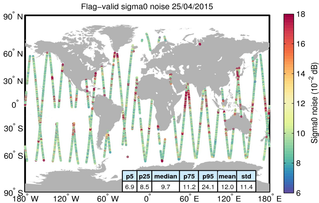
Figure 26. Geographical distribution of flag-valid 20-Hz sigma0 measurement noise over oceans and lakes for 25/04/2015. The statistical values shown in the table refer to the sigma0 noise and are calculated over all measurements shown in the figure.
