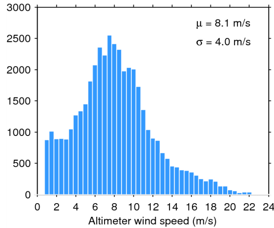
Figure 33. Histogram of flag-valid wind over oceans and lakes for 25/04/2015. The mean ( \mu ) and standard deviation ( \sigma ) are also shown. Note that values larger than 24 m/s are excluded from the histogram for the sake of readability but not from the computation of \mu and \sigma .
