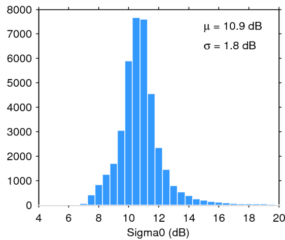
Figure 28. Histogram of science-valid sigma0 over oceans and lakes for 25/04/2015. The mean ( \mu ) and standard deviation ( \sigma ) are also shown. Note that values outside [4 20] dB are excluded from the histogram for the sake of readability but not from the computation of \mu and \sigma .
