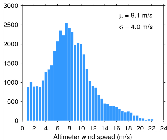
Figure 35. Histogram of science-valid wind over oceans and lakes for 25/04/2015. The mean ( \mu ) and standard deviation ( \sigma ) are also shown. Note that values larger than 24 m/s are excluded from the histogram for the sake of readability but not from the computation of \mu and \sigma .
