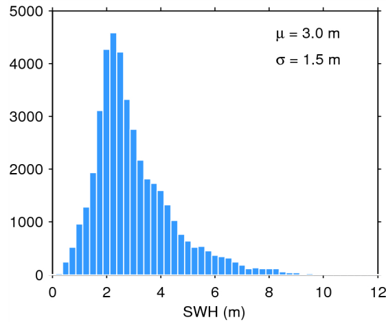
Figure 17. Histogram of flag-valid SWH over oceans and lakes for 25/04/2015. The mean ( \mu ) and standard deviation ( \sigma ) are also shown. Note that values larger than 12 m are excluded from the histogram for the sake of readability but not from the computation of \mu and \sigma .
