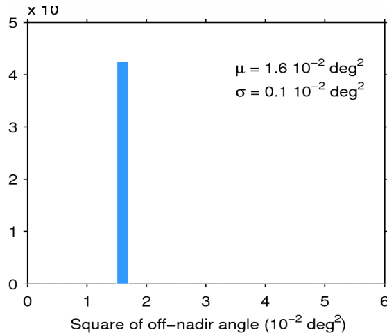
Figure 39. Histogram of flag-valid mispointing over oceans and lakes for 25/04/2015. The mean ( \mu ) and standard deviation ( \sigma ) are also shown. Note that values than 6 \cdot 10^{-2} \text{ deg}^2 are excluded from the histogram for the sake of readability but not from the computation of \mu and \sigma .
