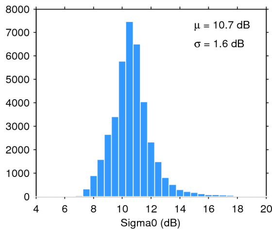
Figure 28. Histogram of science-valid sigma0 over oceans and lakes for 24/04/2015. The mean ( \mu ) and standard deviation ( \sigma ) are also shown. Note that values outside [4 20] dB are excluded from the histogram for the sake of readability but not from the computation of \mu and \sigma .
