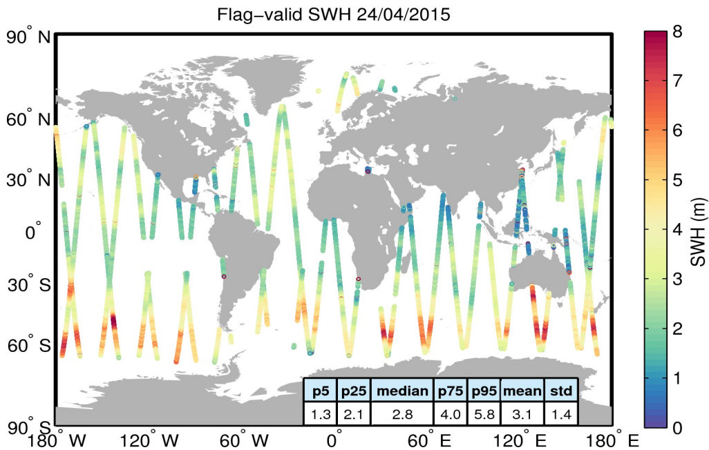
Figure 15. Geographical distribution of flag-valid SWH data over oceans and lakes for 24/04/2015. The statistical values shown in the table refer to the SWH in m and are calculated over all measurements shown in the figure.
