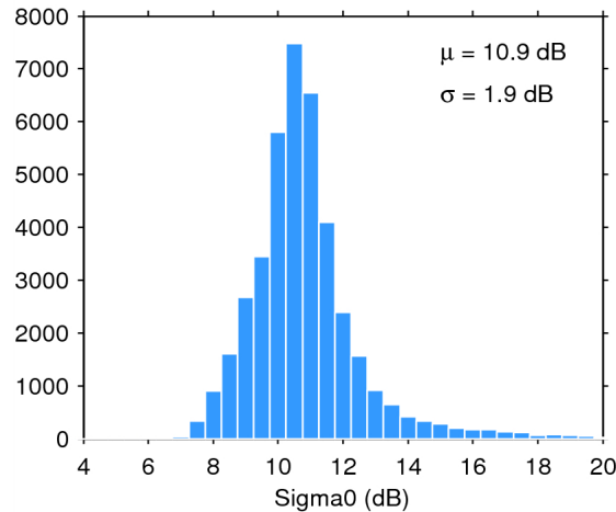
Figure 25. Histogram of flag-valid sigma0 over oceans and lakes for 24/04/2015. The mean ( \mu ) and standard deviation ( \sigma ) are also shown. Note that values outside [4 20] dB are excluded from the histogram for the sake of readability but not from the computation of \mu and \sigma .
