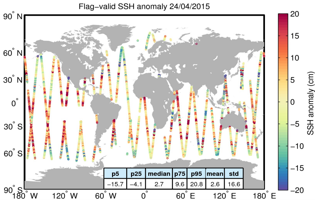
Figure 5. Geographical distribution of flag-valid 1-Hz SSH anomaly data over oceans and lakes for 24/04/2015. The statistical values shown in the table refer to the SSH anomaly in cm and are calculated over all measurements shown in the figure.
