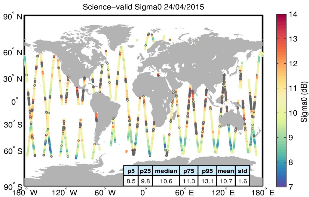
Figure 27. Geographical distribution of science-valid sigma0 data over oceans and lakes for 24/04/2015. The statistical values shown in the table refer to the sigma0 in dB and are calculated over all measurements shown in the figure. Gray circles denote records that have been rejected based on the editing criteria described in Table 4.
