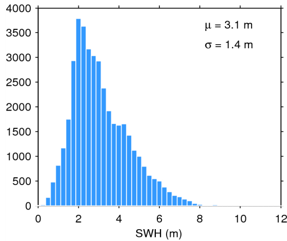
Figure 17. Histogram of flag-valid SWH over oceans and lakes for 24/04/2015. The mean ( \mu ) and standard deviation ( \sigma ) are also shown. Note that values larger than 12 m are excluded from the histogram for the sake of readability but not from the computation of \mu and \sigma .
