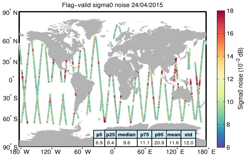
Figure 26. Geographical distribution of flag-valid 20-Hz sigma0 measurement noise over oceans and lakes for 24/04/2015. The statistical values shown in the table refer to the sigma0 noise and are calculated over all measurements shown in the figure.
