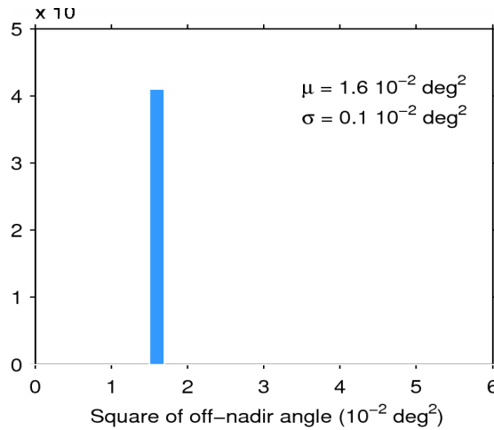
Figure 39. Histogram of flag-valid mispointing over oceans and lakes for 24/04/2015. The mean ( \mu ) and standard deviation ( \sigma ) are also shown. Note that values than 6 \cdot 10^{-2} \text{ deg}^2 are excluded from the histogram for the sake of readability but not from the computation of \mu and \sigma .
