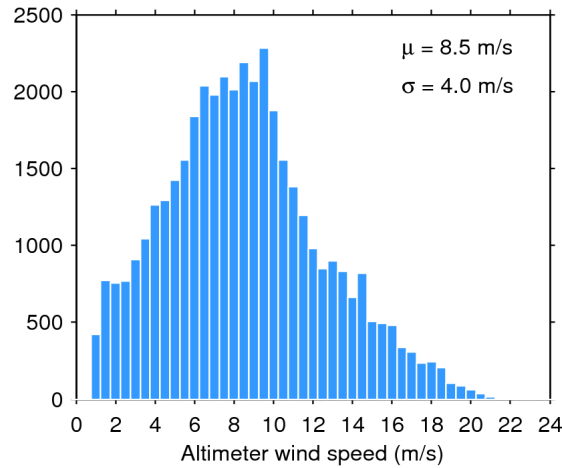
Figure 33. Histogram of flag-valid wind over oceans and lakes for 24/04/2015. The mean ( \mu ) and standard deviation ( \sigma ) are also shown. Note that values larger than 24 m/s are excluded from the histogram for the sake of readability but not from the computation of \mu and \sigma .
