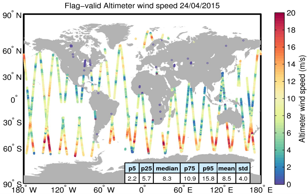
Figure 31. Geographical distribution of flag-valid wind data over oceans and lakes for 24/04/2015. The statistical values shown in the table refer to the wind in m/s and are calculated over all measurements shown in the figure.
