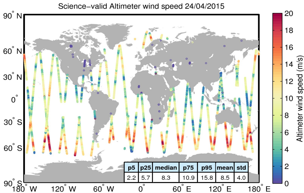
Figure 34. Geographical distribution of science-valid wind data over oceans and lakes for 24/04/2015. The statistical values shown in the table refer to the wind in m/s and are calculated over all measurements shown in the figure. Gray circles denote records that have been rejected based on the editing criteria described in Table 5.
