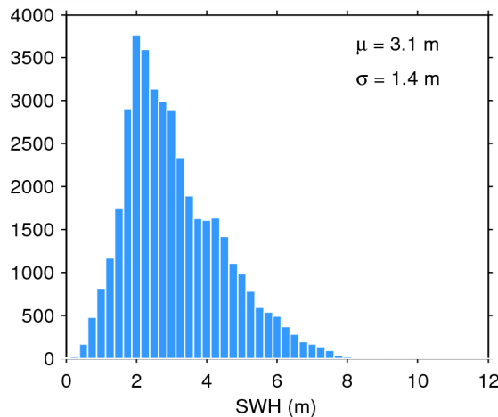
Figure 20. Histogram of science-valid SWH over oceans and lakes for 24/04/2015. The mean ( \mu ) and standard deviation ( \sigma ) are also shown. Note that values larger than 12 m are excluded from the histogram for the sake of readability but not from the computation of \mu and \sigma .
