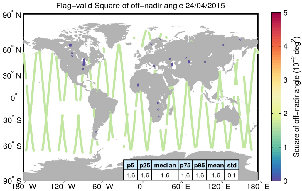
Figure 37. Geographical distribution of flag-valid mispointing data over oceans and lakes for 24/04/2015. The statistical values shown in the table refer to the mispointing in 10^{-2} \text{ deg}^2 and are calculated over all measurements shown in the figure.
