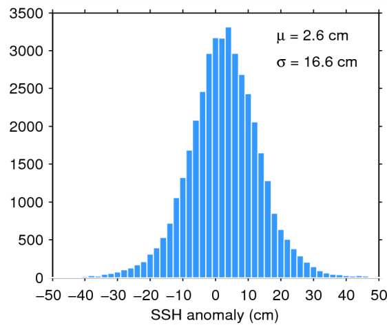
Figure 7. Histogram of flag-valid SSH anomaly over oceans and lakes for 24/04/2015. The mean ( \mu ) and standard deviation ( \sigma ) are also shown. Note that values outside [-50\ 50] cm are excluded from the histogram for the sake of readability but not from the computation of \mu and \sigma .
