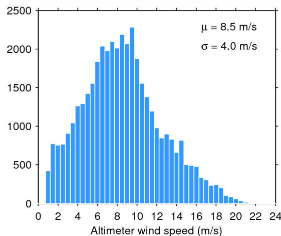
Figure 35. Histogram of science-valid wind over oceans and lakes for 24/04/2015. The mean ( \mu ) and standard deviation ( \sigma ) are also shown. Note that values larger than 24 m/s are excluded from the histogram for the sake of readability but not from the computation of \mu and \sigma .
