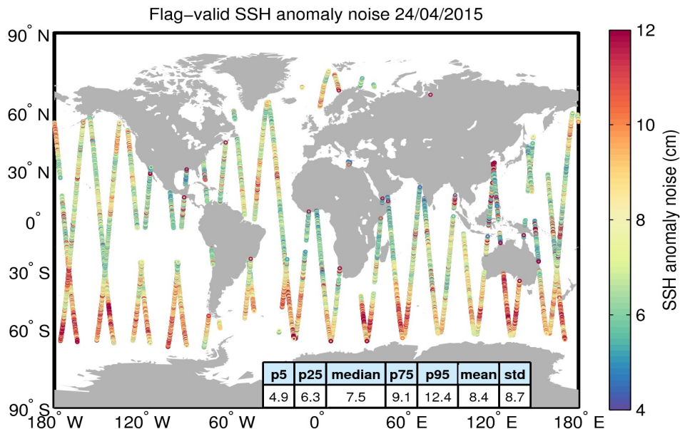
Figure 8. Geographical distribution of flag-valid 20-Hz SSH anomaly measurement noise over oceans and lakes for 24/04/2015. The statistical values shown in the table refer to the SSH anomaly noise and are calculated over all measurements shown in the figure.
