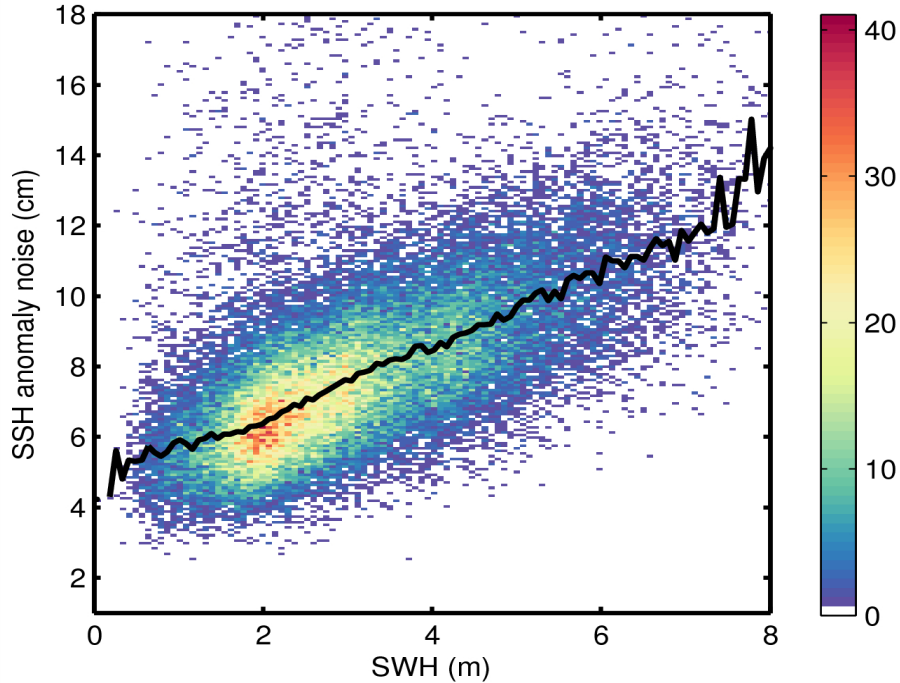
Figure 9. 2D histogram showing flag-valid SSH anomaly noise as a function of SWH for 24/04/2015. The black line denotes the median SSH anomaly as a function of SWH.
