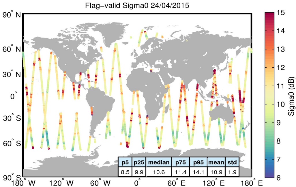
Figure 23. Geographical distribution of flag-valid sigma0 data over oceans and lakes for 24/04/2015. The statistical values shown in the table refer to the sigma0 in dB and are calculated over all measurements shown in the figure.
