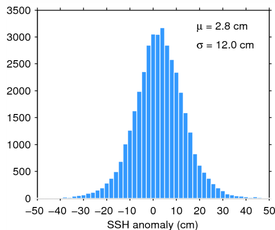
Figure 11. Histogram of science-valid SSH anomaly over oceans and lakes for 24/04/2015. The mean ( \mu ) and standard deviation ( \sigma ) are also shown. Note that values outside [-50 50] cm are excluded from the histogram for the sake of readability but not from the computation of \mu and \sigma .
