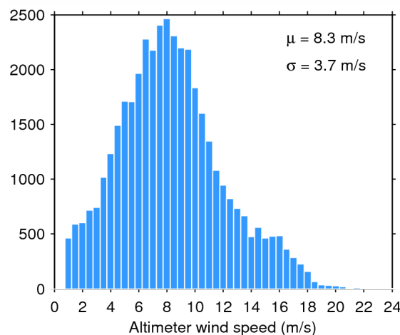
Figure 35. Histogram of science-valid wind over oceans and lakes for 20/04/2015. The mean ( \mu ) and standard deviation ( \sigma ) are also shown. Note that values larger than 24 m/s are excluded from the histogram for the sake of readability but not from the computation of \mu and \sigma .
