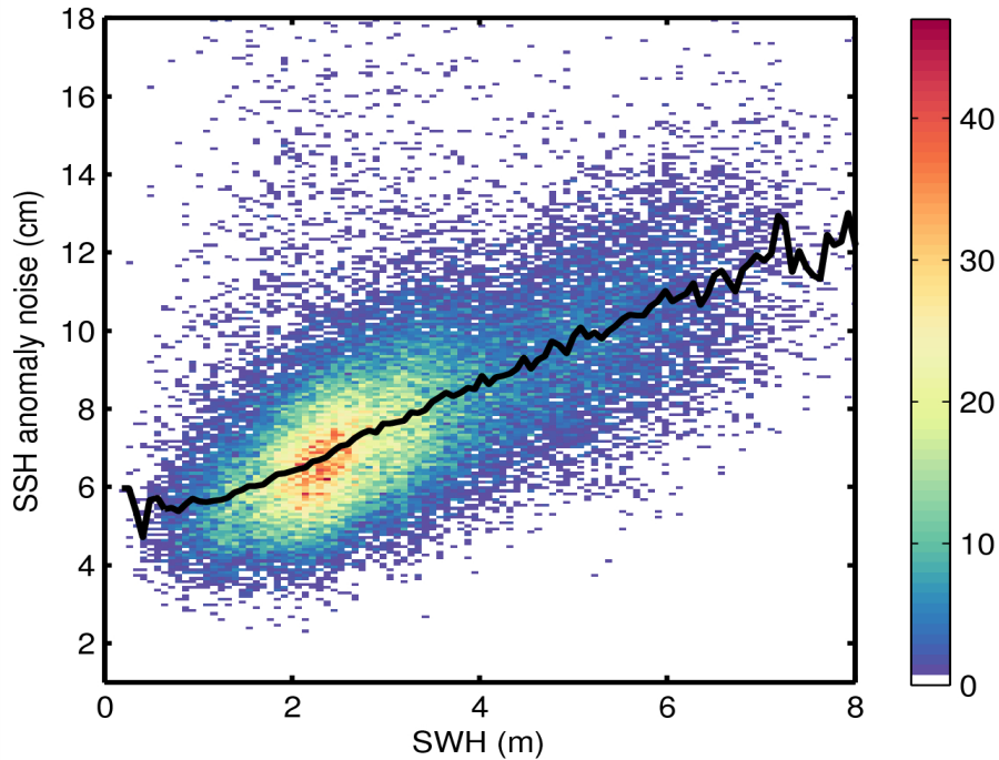
Figure 9. 2D histogram showing flag-valid SSH anomaly noise as a function of SWH for 20/04/2015. The black line denotes the median SSH anomaly as a function of SWH.
