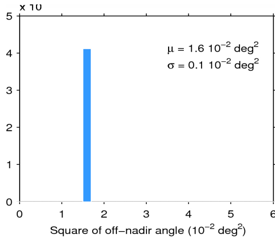
Figure 39. Histogram of flag-valid mispointing over oceans and lakes for 20/04/2015. The mean ( \mu ) and standard deviation ( \sigma ) are also shown. Note that values than 6 \times 10^{-2} \text{ deg}^2 are excluded from the histogram for the sake of readability but not from the computation of \mu and \sigma .
