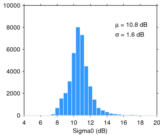
Figure 28. Histogram of science-valid sigma0 over oceans and lakes for 20/04/2015. The mean ( \mu ) and standard deviation ( \sigma ) are also shown. Note that values outside [4 20] dB are excluded from the histogram for the sake of readability but not from the computation of \mu and \sigma .
