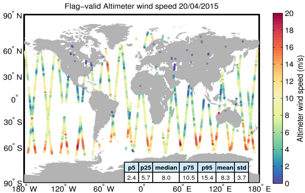
Figure 31. Geographical distribution of flag-valid wind data over oceans and lakes for 20/04/2015. The statistical values shown in the table refer to the wind in m/s and are calculated over all measurements shown in the figure.
