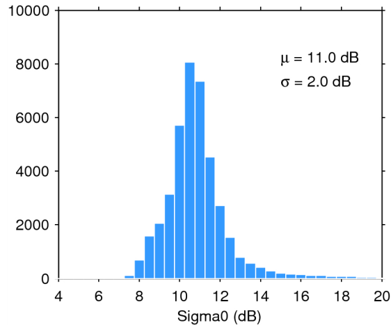
Figure 25. Histogram of flag-valid sigma0 over oceans and lakes for 20/04/2015. The mean ( \mu ) and standard deviation ( \sigma ) are also shown. Note that values outside [4 20] dB are excluded from the histogram for the sake of readability but not from the computation of \mu and \sigma .
