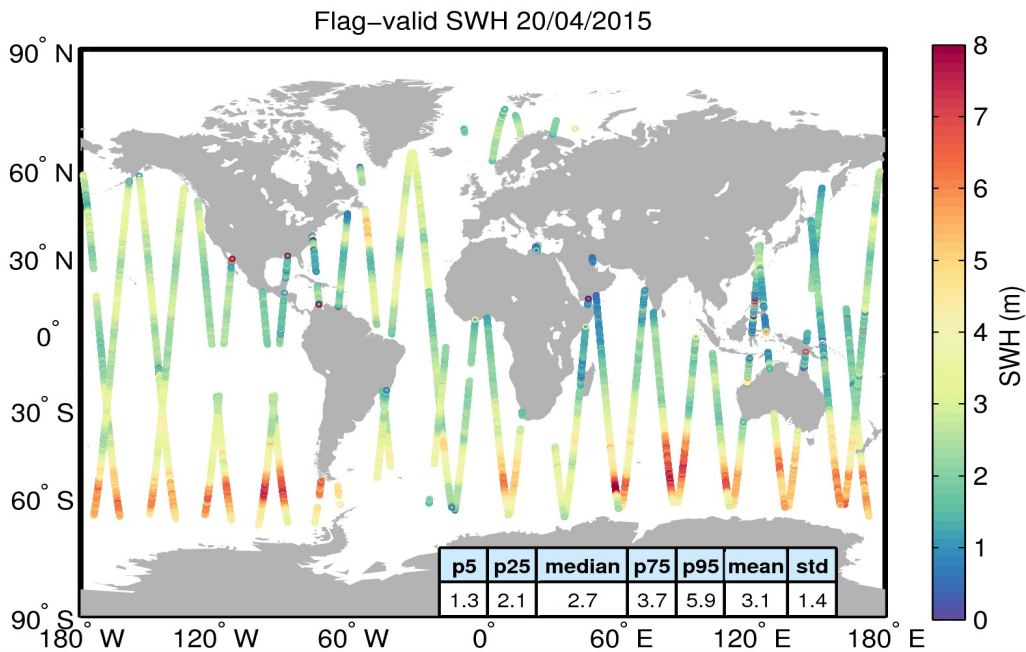
Figure 15. Geographical distribution of flag-valid SWH data over oceans and lakes for 20/04/2015. The statistical values shown in the table refer to the SWH in m and are calculated over all measurements shown in the figure.
