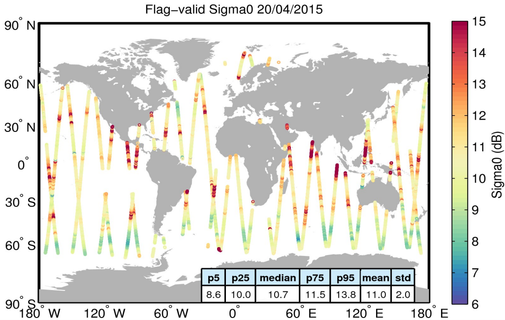
Figure 23. Geographical distribution of flag-valid sigma0 data over oceans and lakes for 20/04/2015. The statistical values shown in the table refer to the sigma0 in dB and are calculated over all measurements shown in the figure.
