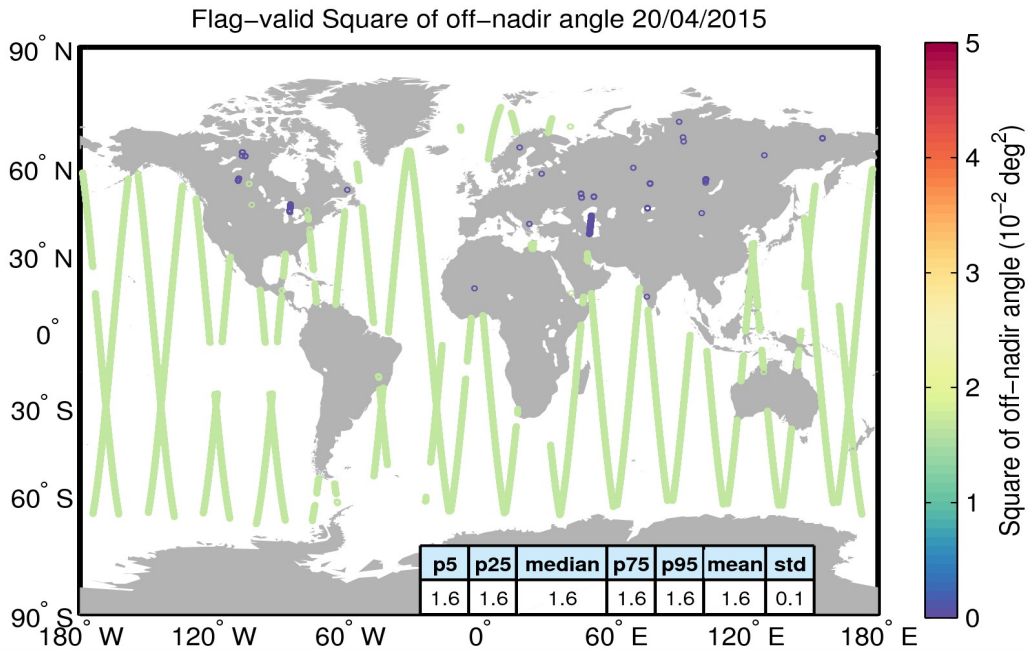
Figure 37. Geographical distribution of flag-valid mispointing data over oceans and lakes for 20/04/2015. The statistical values shown in the table refer to the mispointing in 10^{-2} deg 2 and are calculated over all measurements shown in the figure.
