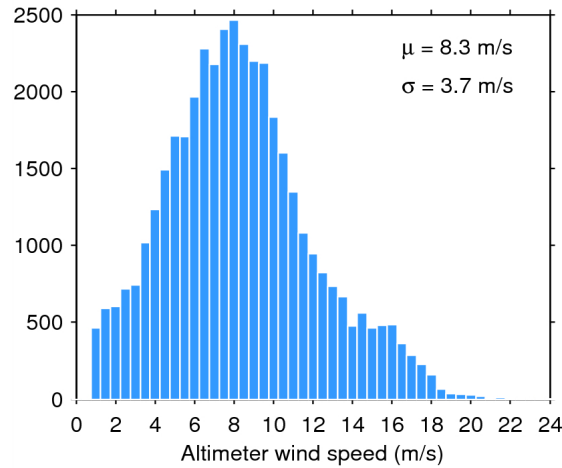
Figure 33. Histogram of flag-valid wind over oceans and lakes for 20/04/2015. The mean ( \mu ) and standard deviation ( \sigma ) are also shown. Note that values larger than 24 m/s are excluded from the histogram for the sake of readability but not from the computation of \mu and \sigma .
