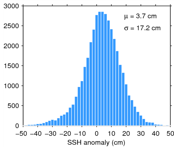
Figure 7. Histogram of flag-valid SSH anomaly over oceans and lakes for 20/04/2015. The mean ( \mu ) and standard deviation ( \sigma ) are also shown. Note that values outside [-50\ 50] cm are excluded from the histogram for the sake of readability but not from the computation of \mu and \sigma .
