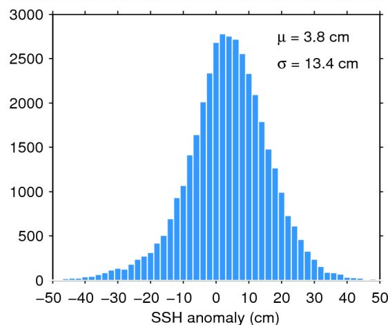
Figure 11. Histogram of science-valid SSH anomaly over oceans and lakes for 20/04/2015. The mean ( \mu ) and standard deviation ( \sigma ) are also shown. Note that values outside [-50 50] cm are excluded from the histogram for the sake of readability but not from the computation of \mu and \sigma .
