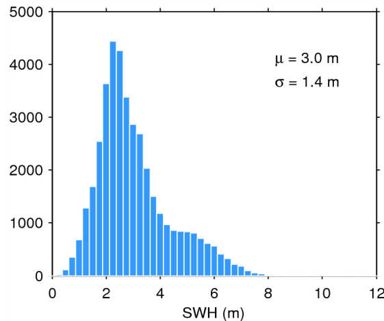
Figure 20. Histogram of science-valid SWH over oceans and lakes for 20/04/2015. The mean ( \mu ) and standard deviation ( \sigma ) are also shown. Note that values larger than 12 m are excluded from the histogram for the sake of readability but not from the computation of \mu and \sigma .
