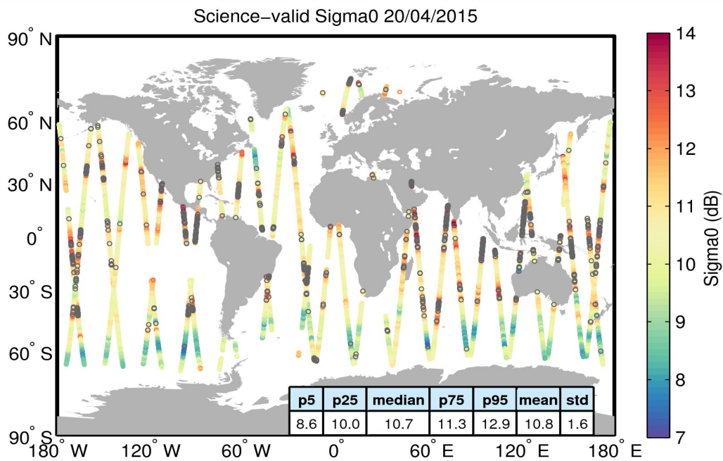
Figure 27. Geographical distribution of science-valid sigma0 data over oceans and lakes for 20/04/2015. The statistical values shown in the table refer to the sigma0 in dB and are calculated over all measurements shown in the figure. Gray circles denote records that have been rejected based on the editing criteria described in Table 4.
