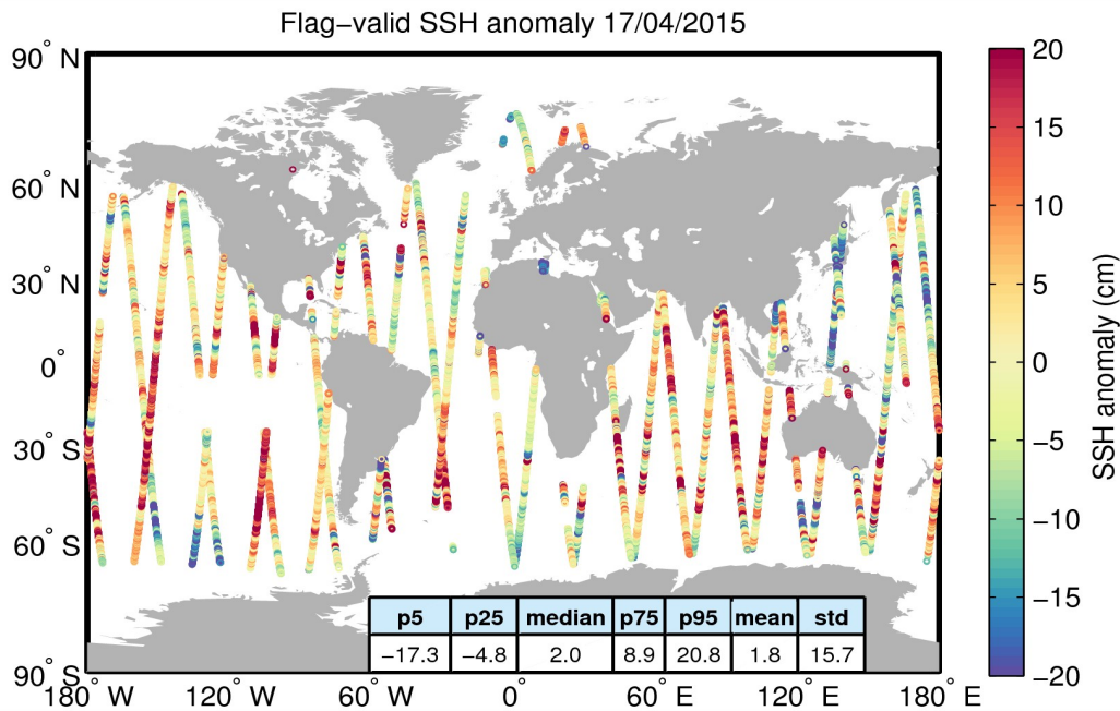
Figure 5. Geographical distribution of flag-valid 1-Hz SSH anomaly data over oceans and lakes for 17/04/2015. The statistical values shown in the table refer to the SSH anomaly in cm and are calculated over all measurements shown in the figure.
