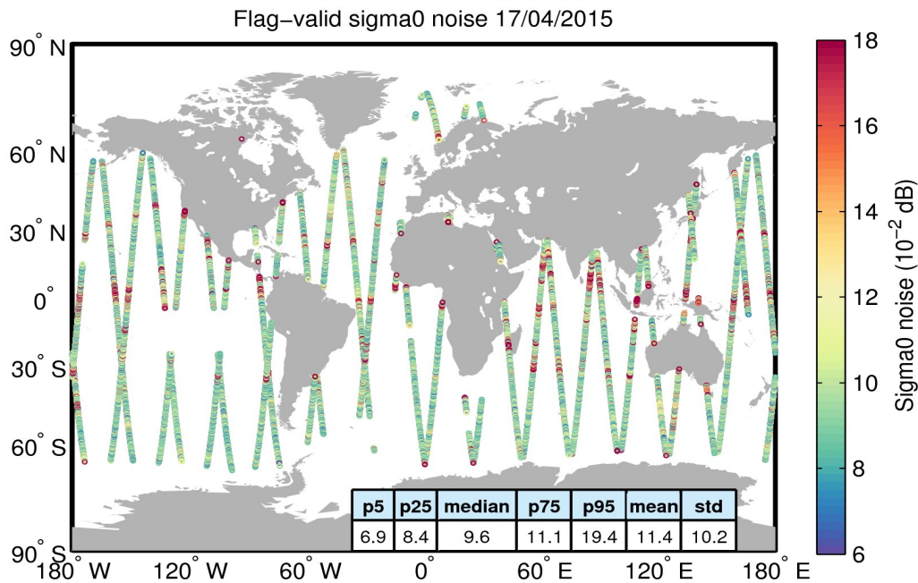
Figure 26. Geographical distribution of flag-valid 20-Hz sigma0 measurement noise over oceans and lakes for 17/04/2015. The statistical values shown in the table refer to the sigma0 noise and are calculated over all measurements shown in the figure.
