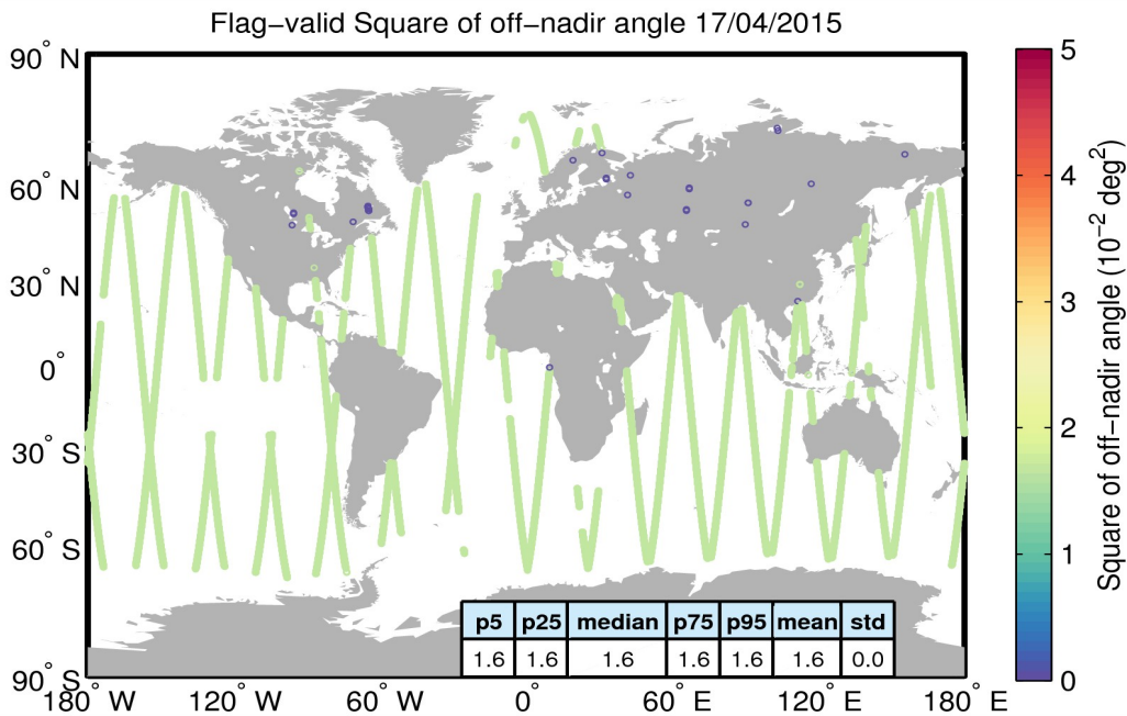
Figure 37. Geographical distribution of flag-valid mispointing data over oceans and lakes for 17/04/2015. The statistical values shown in the table refer to the mispointing in 10^{-2} deg 2 and are calculated over all measurements shown in the figure.
