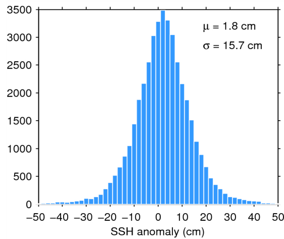
Figure 7. Histogram of flag-valid SSH anomaly over oceans and lakes for 17/04/2015. The mean ( \mu ) and standard deviation ( \sigma ) are also shown. Note that values outside [-50\ 50] cm are excluded from the histogram for the sake of readability but not from the computation of \mu and \sigma .
