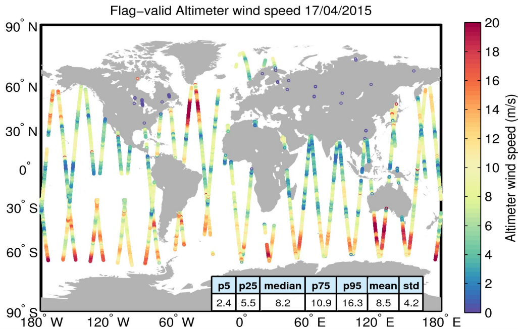
Figure 31. Geographical distribution of flag-valid wind data over oceans and lakes for 17/04/2015. The statistical values shown in the table refer to the wind in m/s and are calculated over all measurements shown in the figure.
