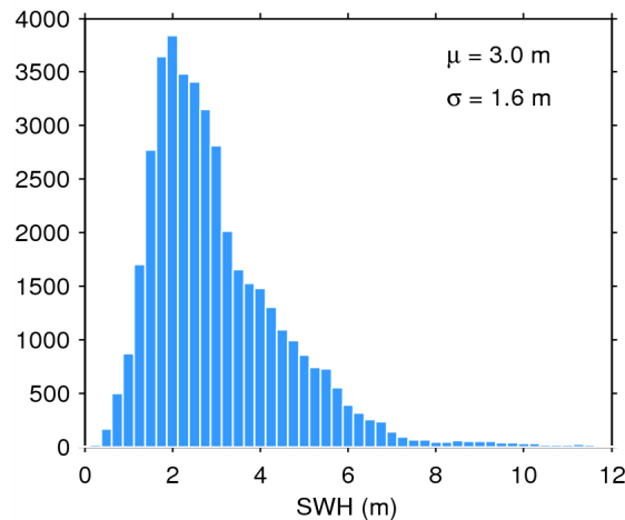
Figure 20. Histogram of science-valid SWH over oceans and lakes for 17/04/2015. The mean ( \mu ) and standard deviation ( \sigma ) are also shown. Note that values larger than 12 m are excluded from the histogram for the sake of readability but not from the computation of \mu and \sigma .
