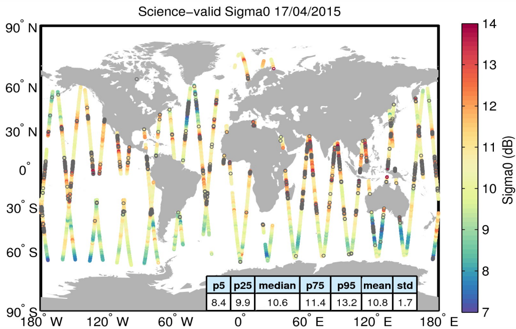
Figure 27. Geographical distribution of science-valid sigma0 data over oceans and lakes for 17/04/2015. The statistical values shown in the table refer to the sigma0 in dB and are calculated over all measurements shown in the figure. Gray circles denote records that have been rejected based on the editing criteria described in Table 4.
