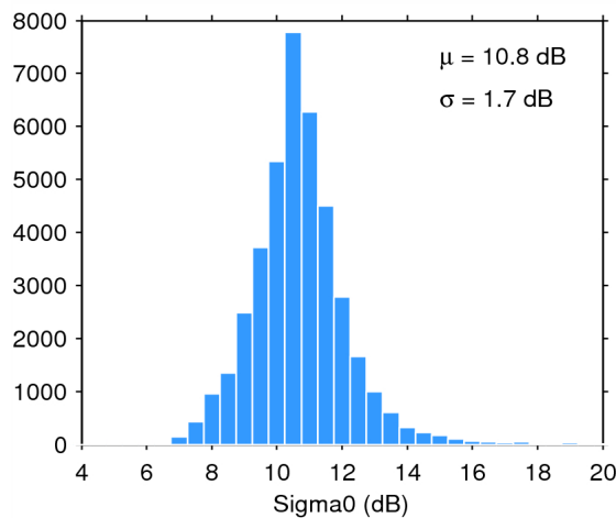
Figure 28. Histogram of science-valid sigma0 over oceans and lakes for 17/04/2015. The mean ( \mu ) and standard deviation ( \sigma ) are also shown. Note that values outside [4 20] dB are excluded from the histogram for the sake of readability but not from the computation of \mu and \sigma .
