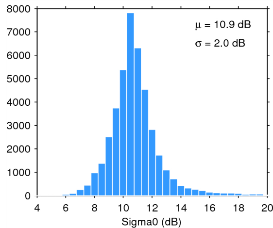
Figure 25. Histogram of flag-valid sigma0 over oceans and lakes for 17/04/2015. The mean ( \mu ) and standard deviation ( \sigma ) are also shown. Note that values outside [4 20] dB are excluded from the histogram for the sake of readability but not from the computation of \mu and \sigma .
