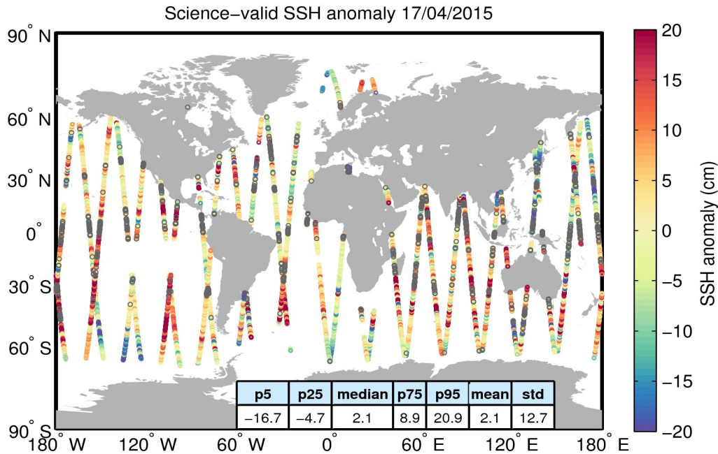
Figure 10. Geographical distribution of science-valid SSH anomaly data over oceans and lakes for 17/04/2015. The statistical values shown in the table refer to the SSH anomaly in cm and are calculated over all measurements shown in the figure. Gray circles denote records that have been rejected based on the editing criteria described in Table 2.
