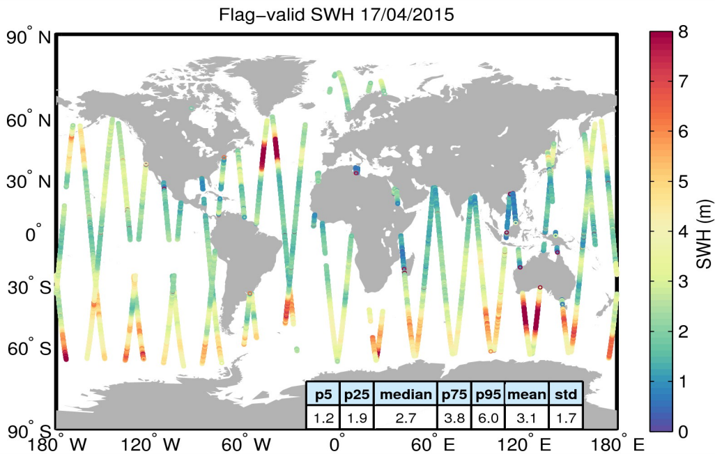
Figure 15. Geographical distribution of flag-valid SWH data over oceans and lakes for 17/04/2015. The statistical values shown in the table refer to the SWH in m and are calculated over all measurements shown in the figure.
