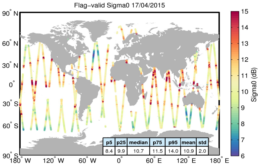
Figure 23. Geographical distribution of flag-valid sigma0 data over oceans and lakes for 17/04/2015. The statistical values shown in the table refer to the sigma0 in dB and are calculated over all measurements shown in the figure.
