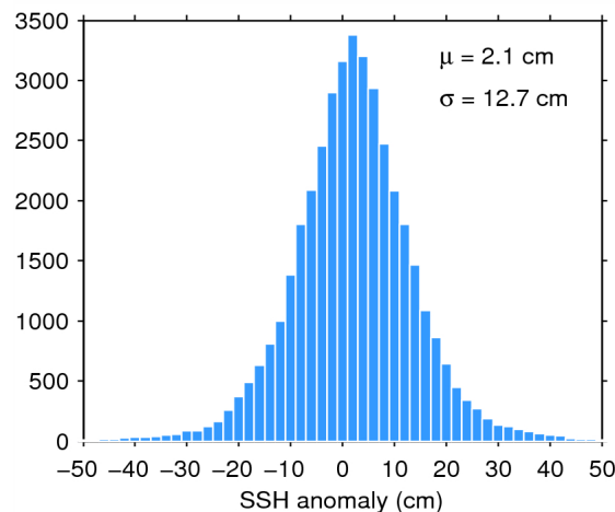
Figure 11. Histogram of science-valid SSH anomaly over oceans and lakes for 17/04/2015. The mean ( \mu ) and standard deviation ( \sigma ) are also shown. Note that values outside [-50 50] cm are excluded from the histogram for the sake of readability but not from the computation of \mu and \sigma .
