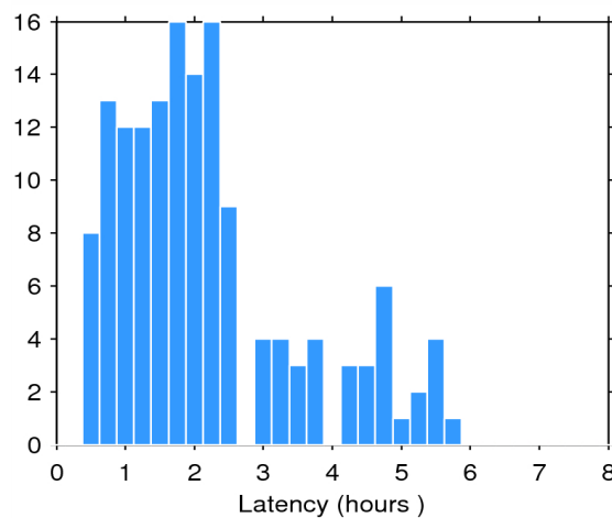
Figure 2. Histogram of the data latency for 17/04/2015. The y-axis denotes the number of files that are made available with a delay of x-hours with respect to the mean time of the records stored in the file.
