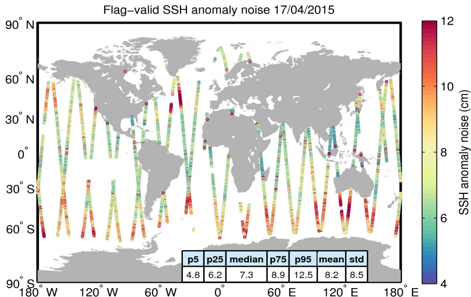
Figure 8. Geographical distribution of flag-valid 20-Hz SSH anomaly measurement noise over oceans and lakes for 17/04/2015. The statistical values shown in the table refer to the SSH anomaly noise and are calculated over all measurements shown in the figure.
