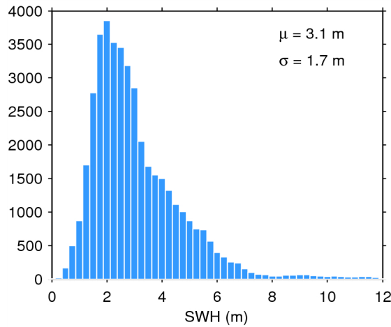
Figure 17. Histogram of flag-valid SWH over oceans and lakes for 17/04/2015. The mean ( \mu ) and standard deviation ( \sigma ) are also shown. Note that values larger than 12 m are excluded from the histogram for the sake of readability but not from the computation of \mu and \sigma .
