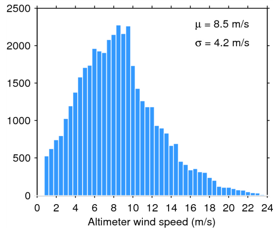
Figure 33. Histogram of flag-valid wind over oceans and lakes for 17/04/2015. The mean ( \mu ) and standard deviation ( \sigma ) are also shown. Note that values larger than 24 m/s are excluded from the histogram for the sake of readability but not from the computation of \mu and \sigma .
