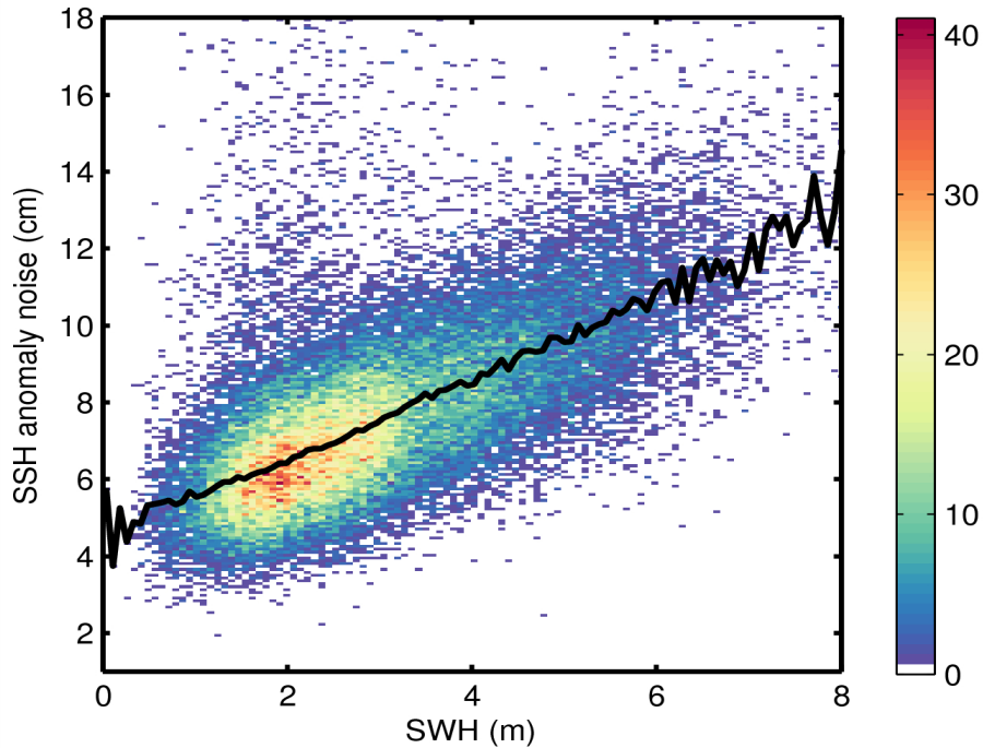
Figure 9. 2D histogram showing flag-valid SSH anomaly noise as a function of SWH for 17/04/2015. The black line denotes the median SSH anomaly as a function of SWH.
