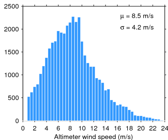
Figure 35. Histogram of science-valid wind over oceans and lakes for 17/04/2015. The mean ( \mu ) and standard deviation ( \sigma ) are also shown. Note that values larger than 24 m/s are excluded from the histogram for the sake of readability but not from the computation of \mu and \sigma .
