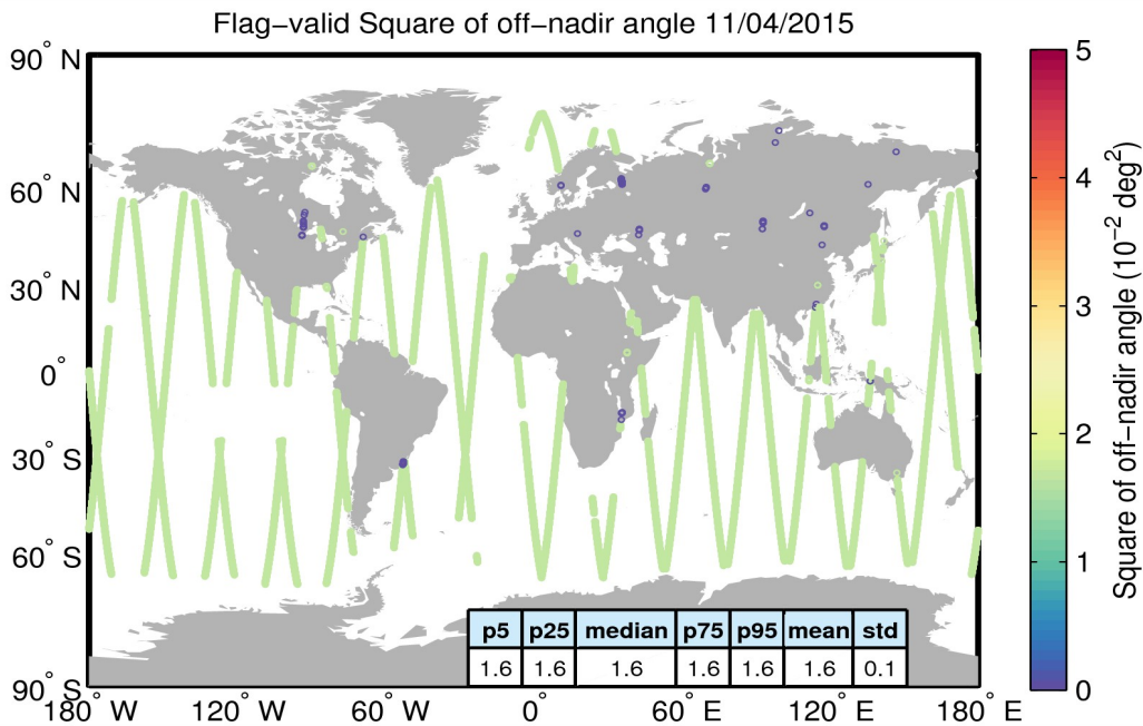
Figure 37. Geographical distribution of flag-valid mispointing data over oceans and lakes for 11/04/2015. The statistical values shown in the table refer to the mispointing in 10^{-2} \text{deg}^2 and are calculated over all measurements shown in the figure.
