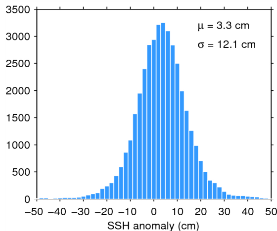
Figure 11. Histogram of science-valid SSH anomaly over oceans and lakes for 11/04/2015. The mean ( \mu ) and standard deviation ( \sigma ) are also shown. Note that values outside [-50 50] cm are excluded from the histogram for the sake of readability but not from the computation of \mu and \sigma .
