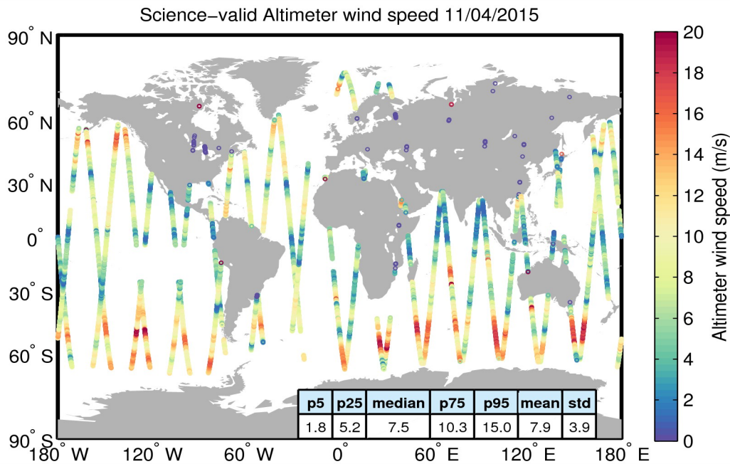
Figure 34. Geographical distribution of science-valid wind data over oceans and lakes for 11/04/2015. The statistical values shown in the table refer to the wind in m/s and are calculated over all measurements shown in the figure. Gray circles denote records that have been rejected based on the editing criteria described in Table 5.
