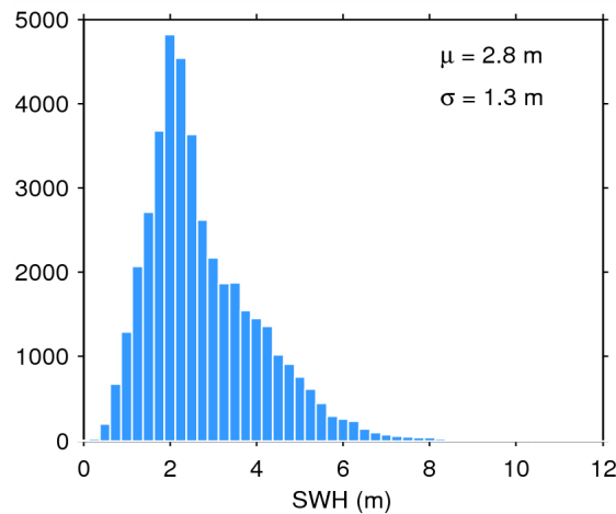
Figure 17. Histogram of flag-valid SWH over oceans and lakes for 11/04/2015. The mean ( \mu ) and standard deviation ( \sigma ) are also shown. Note that values larger than 12 m are excluded from the histogram for the sake of readability but not from the computation of \mu and \sigma .
