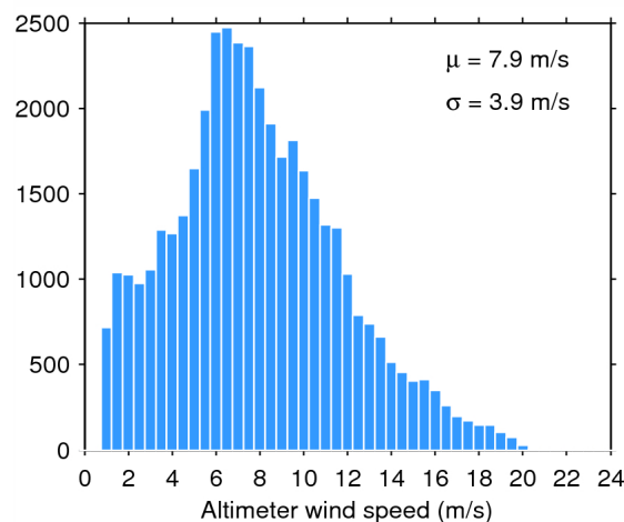
Figure 35. Histogram of science-valid wind over oceans and lakes for 11/04/2015. The mean ( \mu ) and standard deviation ( \sigma ) are also shown. Note that values larger than 24 m/s are excluded from the histogram for the sake of readability but not from the computation of \mu and \sigma .
