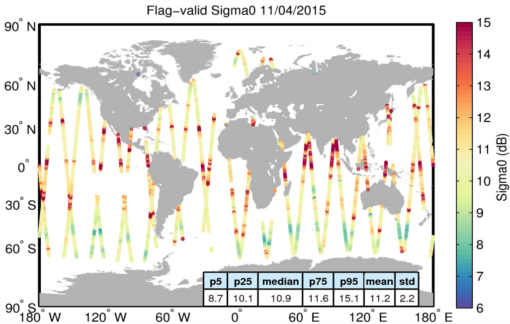
Figure 23. Geographical distribution of flag-valid sigma0 data over oceans and lakes for 11/04/2015. The statistical values shown in the table refer to the sigma0 in dB and are calculated over all measurements shown in the figure.
