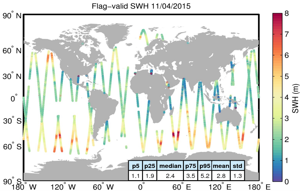
Figure 15. Geographical distribution of flag-valid SWH data over oceans and lakes for 11/04/2015. The statistical values shown in the table refer to the SWH in m and are calculated over all measurements shown in the figure.
