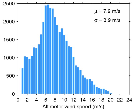
Figure 33. Histogram of flag-valid wind over oceans and lakes for 11/04/2015. The mean ( \mu ) and standard deviation ( \sigma ) are also shown. Note that values larger than 24 m/s are excluded from the histogram for the sake of readability but not from the computation of \mu and \sigma .
