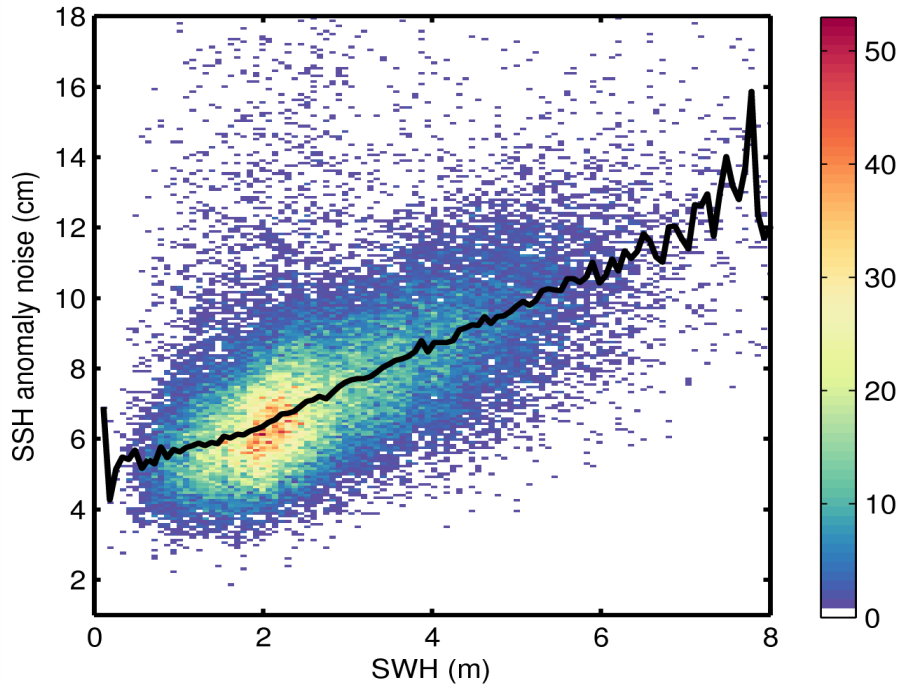
Figure 9. 2D histogram showing flag-valid SSH anomaly noise as a function of SWH for 11/04/2015. The black line denotes the median SSH anomaly as a function of SWH.
