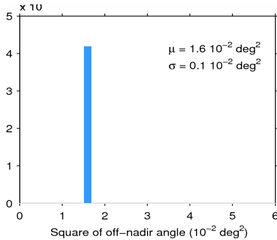
Figure 39. Histogram of flag-valid mispointing over oceans and lakes for 11/04/2015. The mean ( \mu ) and standard deviation ( \sigma ) are also shown. Note that values than 6 \times 10^{-2} \text{ deg}^2 are excluded from the histogram for the sake of readability but not from the computation of \mu and \sigma .
