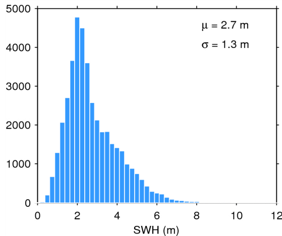
Figure 20. Histogram of science-valid SWH over oceans and lakes for 11/04/2015. The mean ( \mu ) and standard deviation ( \sigma ) are also shown. Note that values larger than 12 m are excluded from the histogram for the sake of readability but not from the computation of \mu and \sigma .
