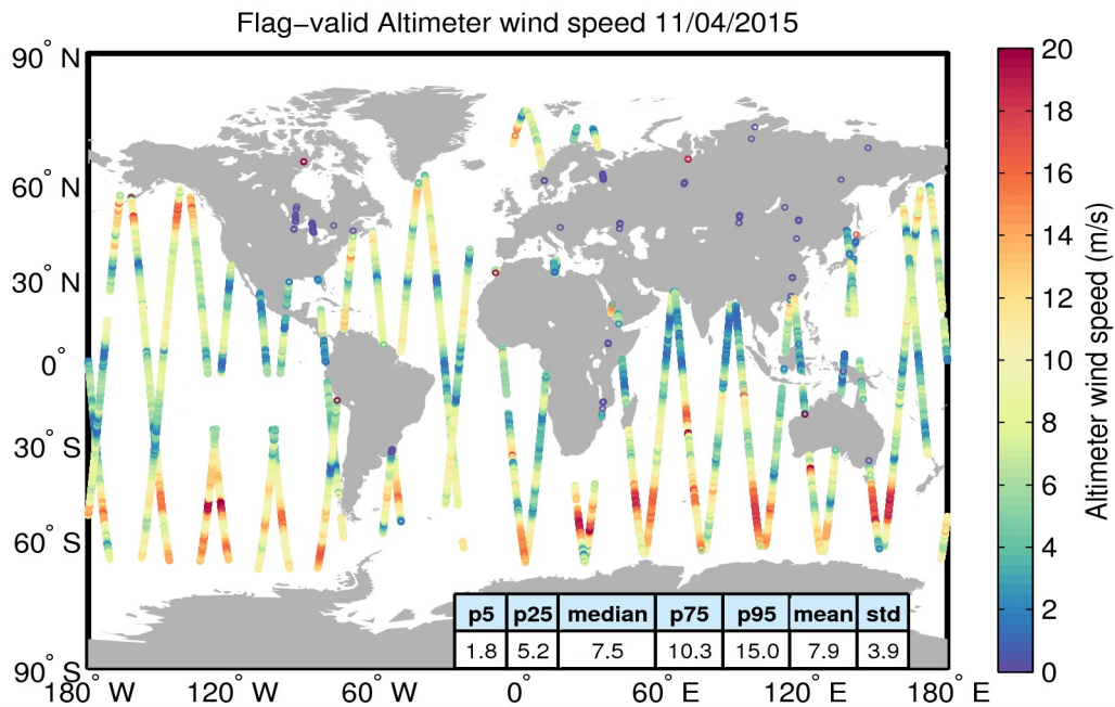
Figure 31. Geographical distribution of flag-valid wind data over oceans and lakes for 11/04/2015. The statistical values shown in the table refer to the wind in m/s and are calculated over all measurements shown in the figure.
