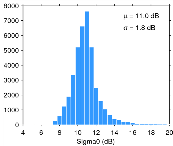
Figure 28. Histogram of science-valid sigma0 over oceans and lakes for 11/04/2015. The mean ( \mu ) and standard deviation ( \sigma ) are also shown. Note that values outside [4 20] dB are excluded from the histogram for the sake of readability but not from the computation of \mu and \sigma .
