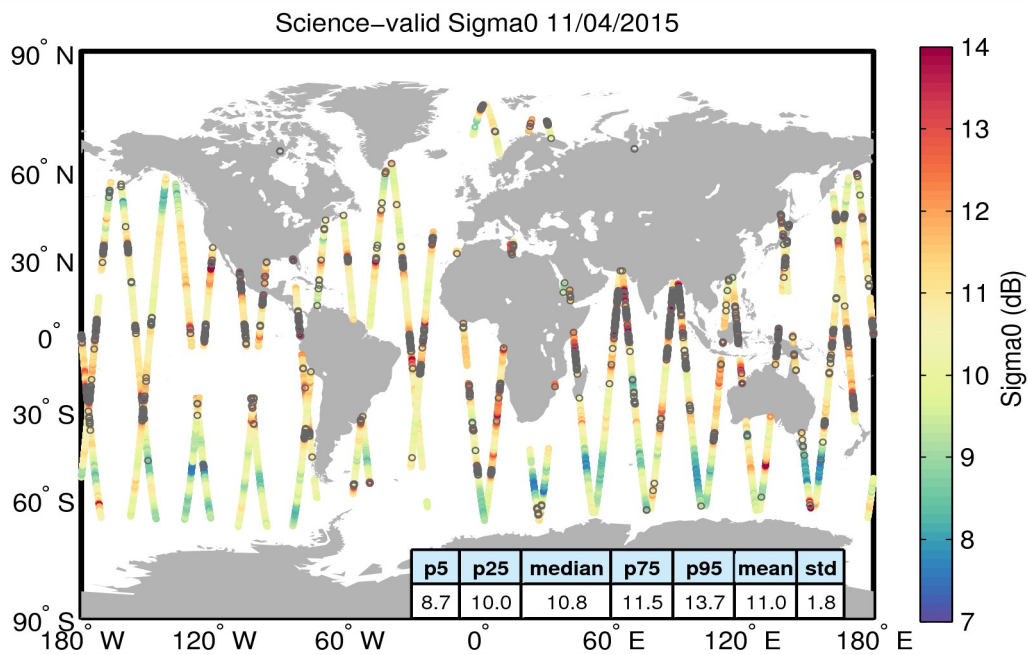
Figure 27. Geographical distribution of science-valid sigma0 data over oceans and lakes for 11/04/2015. The statistical values shown in the table refer to the sigma0 in dB and are calculated over all measurements shown in the figure. Gray circles denote records that have been rejected based on the editing criteria described in Table 4.
