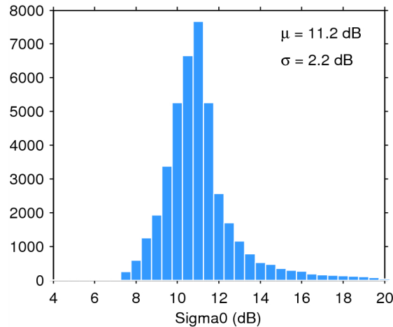
Figure 25. Histogram of flag-valid sigma0 over oceans and lakes for 11/04/2015. The mean ( \mu ) and standard deviation ( \sigma ) are also shown. Note that values outside [4 20] dB are excluded from the histogram for the sake of readability but not from the computation of \mu and \sigma .
