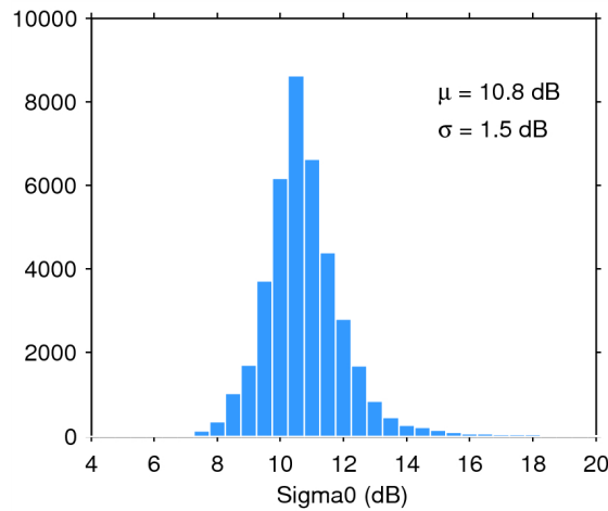
Figure 28. Histogram of science-valid sigma0 over oceans and lakes for 08/04/2015. The mean ( \mu ) and standard deviation ( \sigma ) are also shown. Note that values outside [4 20] dB are excluded from the histogram for the sake of readability but not from the computation of \mu and \sigma .
