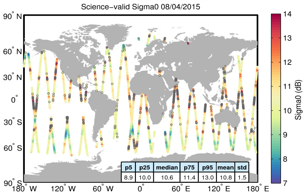
Figure 27. Geographical distribution of science-valid sigma0 data over oceans and lakes for 08/04/2015. The statistical values shown in the table refer to the sigma0 in dB and are calculated over all measurements shown in the figure. Gray circles denote records that have been rejected based on the editing criteria described in Table 4.
