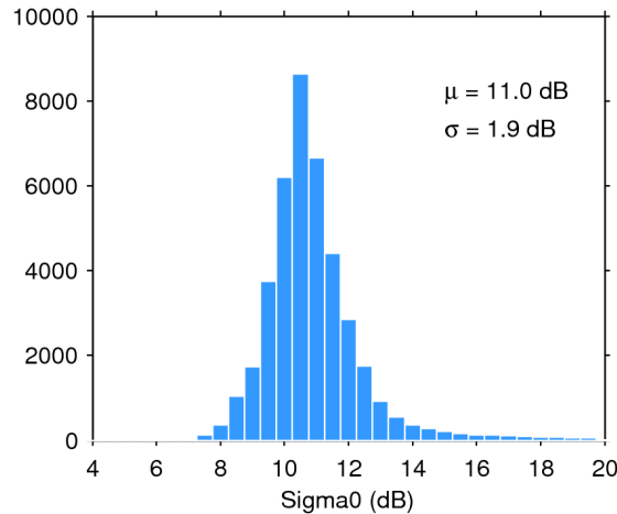
Figure 25. Histogram of flag-valid sigma0 over oceans and lakes for 08/04/2015. The mean ( \mu ) and standard deviation ( \sigma ) are also shown. Note that values outside [4 20] dB are excluded from the histogram for the sake of readability but not from the computation of \mu and \sigma .
