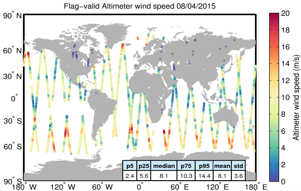
Figure 31. Geographical distribution of flag-valid wind data over oceans and lakes for 08/04/2015. The statistical values shown in the table refer to the wind in m/s and are calculated over all measurements shown in the figure.
