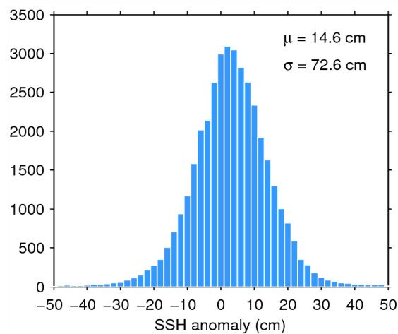
Figure 7. Histogram of flag-valid SSH anomaly over oceans and lakes for 08/04/2015. The mean ( \mu ) and standard deviation ( \sigma ) are also shown. Note that values outside [-50 \ 50] cm are excluded from the histogram for the sake of readability but not from the computation of \mu and \sigma .
