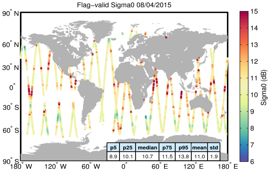
Figure 23. Geographical distribution of flag-valid sigma0 data over oceans and lakes for 08/04/2015. The statistical values shown in the table refer to the sigma0 in dB and are calculated over all measurements shown in the figure.
