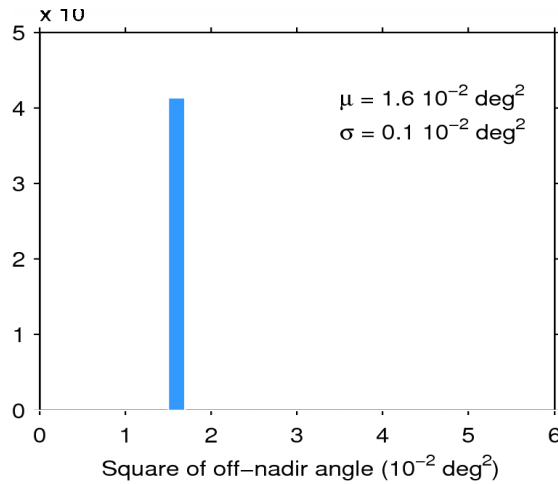
Figure 39. Histogram of flag-valid mispointing over oceans and lakes for 08/04/2015. The mean ( \mu ) and standard deviation ( \sigma ) are also shown. Note that values than 6 \times 10^{-2} \text{ deg}^2 are excluded from the histogram for the sake of readability but not from the computation of \mu and \sigma .
