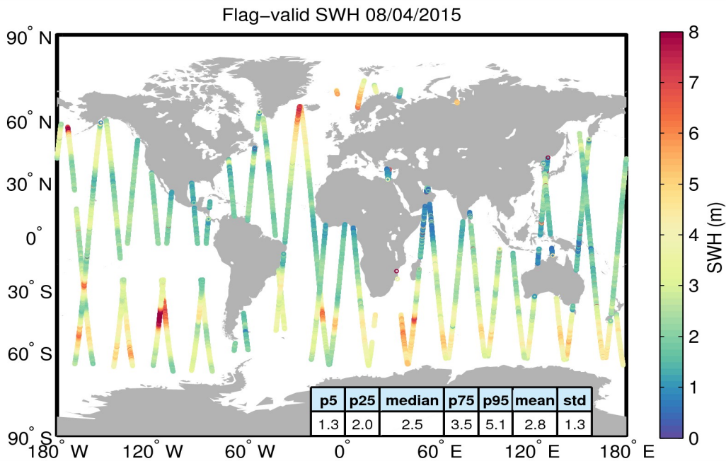
Figure 15. Geographical distribution of flag-valid SWH data over oceans and lakes for 08/04/2015. The statistical values shown in the figure refer to the SWH in m and are calculated over all measurements shown in the figure.
