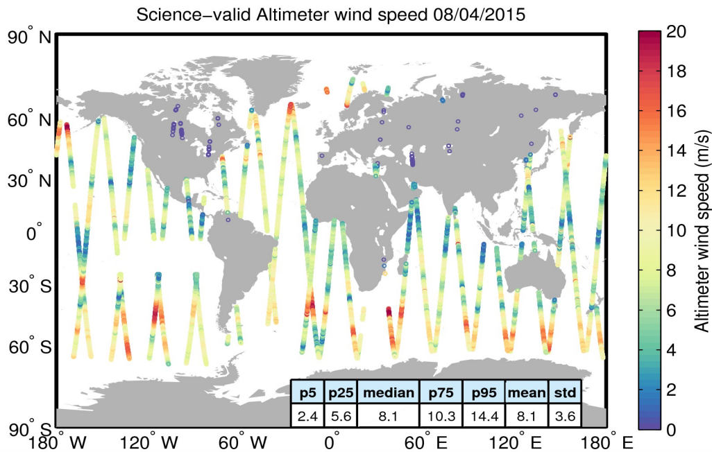
Figure 34. Geographical distribution of science-valid wind data over oceans and lakes for 08/04/2015. The statistical values shown in the table refer to the wind in m/s and are calculated over all measurements shown in the figure. Gray circles denote records that have been rejected based on the editing criteria described in Table 5.
