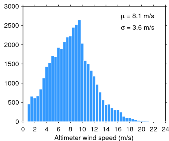
Figure 35. Histogram of science-valid wind over oceans and lakes for 08/04/2015. The mean ( \mu ) and standard deviation ( \sigma ) are also shown. Note that values larger than 24 m/s are excluded from the histogram for the sake of readability but not from the computation of \mu and \sigma .
