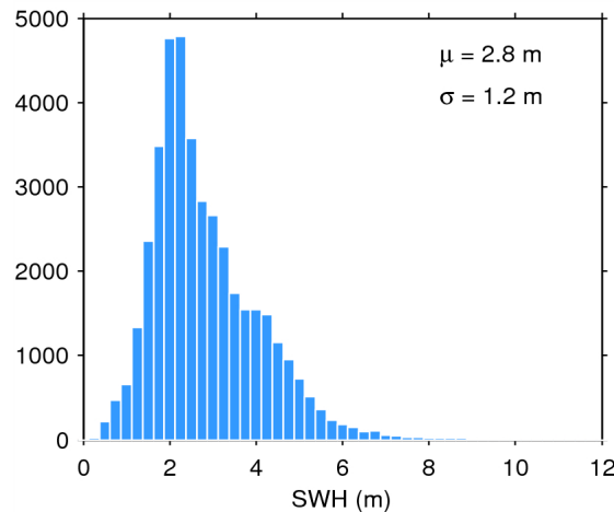
Figure 20. Histogram of science-valid SWH over oceans and lakes for 08/04/2015. The mean ( \mu ) and standard deviation ( \sigma ) are also shown. Note that values larger than 12 m are excluded from the histogram for the sake of readability but not from the computation of \mu and \sigma .
