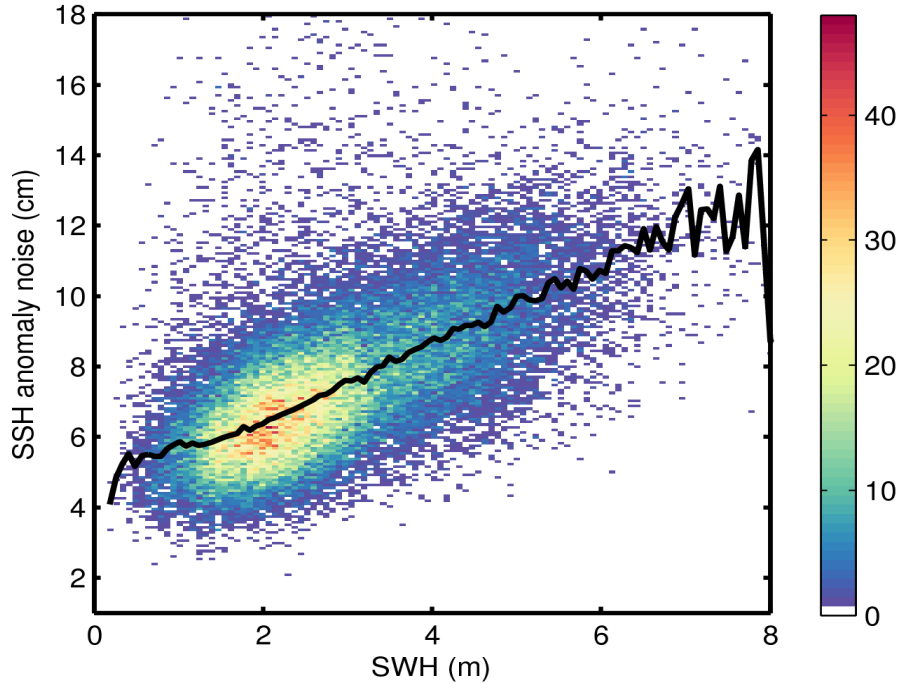
Figure 9. 2D histogram showing flag-valid SSH anomaly noise as a function of SWH for 04/04/2015. The black line denotes the median SSH anomaly as a function of SWH.
