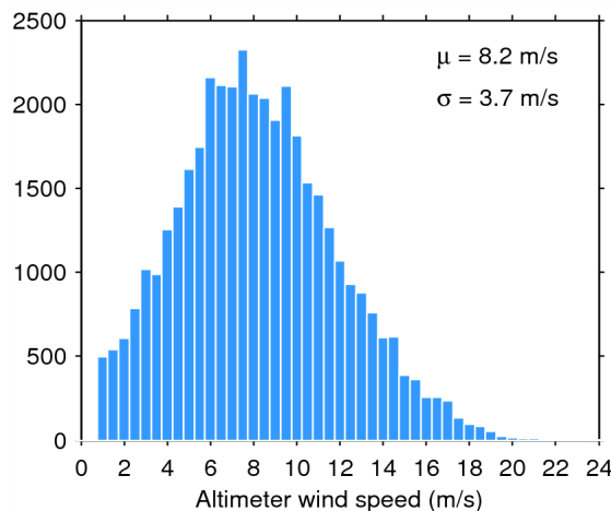
Figure 35. Histogram of science-valid wind over oceans and lakes for 04/04/2015. The mean ( \mu ) and standard deviation ( \sigma ) are also shown. Note that values larger than 24 m/s are excluded from the histogram for the sake of readability but not from the computation of \mu and \sigma .
