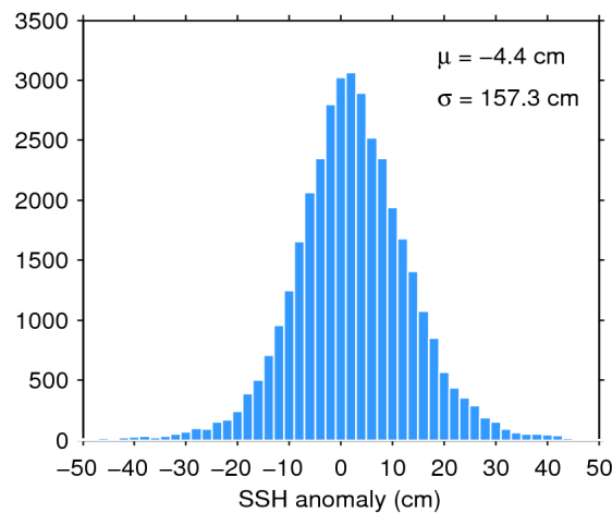
Figure 7. Histogram of flag-valid SSH anomaly over oceans and lakes for 04/04/2015. The mean ( \mu ) and standard deviation ( \sigma ) are also shown. Note that values outside [-50\ 50] cm are excluded from the histogram for the sake of readability but not from the computation of \mu and \sigma .
