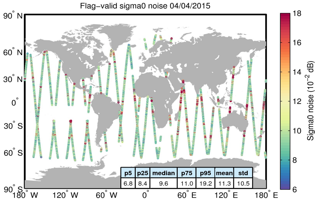
Figure 26. Geographical distribution of flag-valid 20-Hz sigma0 measurement noise over oceans and lakes for 04/04/2015. The statistical values shown in the table refer to the sigma0 noise and are calculated over all measurements shown in the figure.
