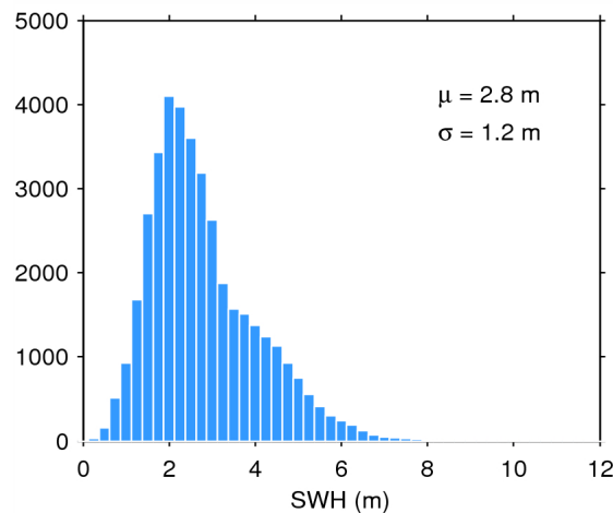
Figure 20. Histogram of science-valid SWH over oceans and lakes for 04/04/2015. The mean ( \mu ) and standard deviation ( \sigma ) are also shown. Note that values larger than 12 m are excluded from the histogram for the sake of readability but not from the computation of \mu and \sigma .
