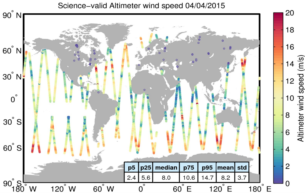
Figure 34. Geographical distribution of science-valid wind data over oceans and lakes for 04/04/2015. The statistical values shown in the table refer to the wind in m/s and are calculated over all measurements shown in the figure. Gray circles denote records that have been rejected based on the editing criteria described in Table 5.
