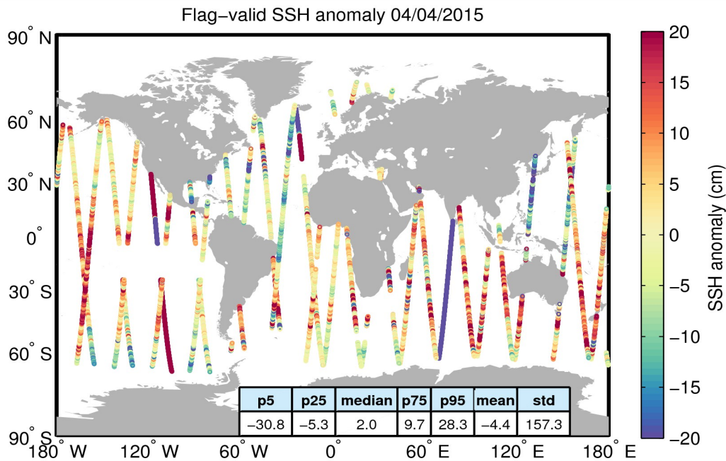
Figure 5. Geographical distribution of flag-valid 1-Hz SSH anomaly data over oceans and lakes for 04/04/2015. The statistical values shown in the table refer to the SSH anomaly in cm and are calculated over all measurements shown in the figure.
