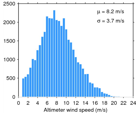
Figure 33. Histogram of flag-valid wind over oceans and lakes for 04/04/2015. The mean ( \mu ) and standard deviation ( \sigma ) are also shown. Note that values larger than 24 m/s are excluded from the histogram for the sake of readability but not from the computation of \mu and \sigma .
