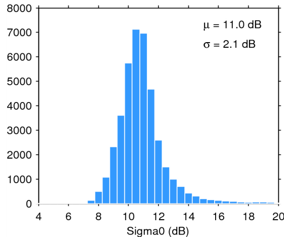
Figure 25. Histogram of flag-valid sigma0 over oceans and lakes for 04/04/2015. The mean ( \mu ) and standard deviation ( \sigma ) are also shown. Note that values outside [4 20] dB are excluded from the histogram for the sake of readability but not from the computation of \mu and \sigma .
