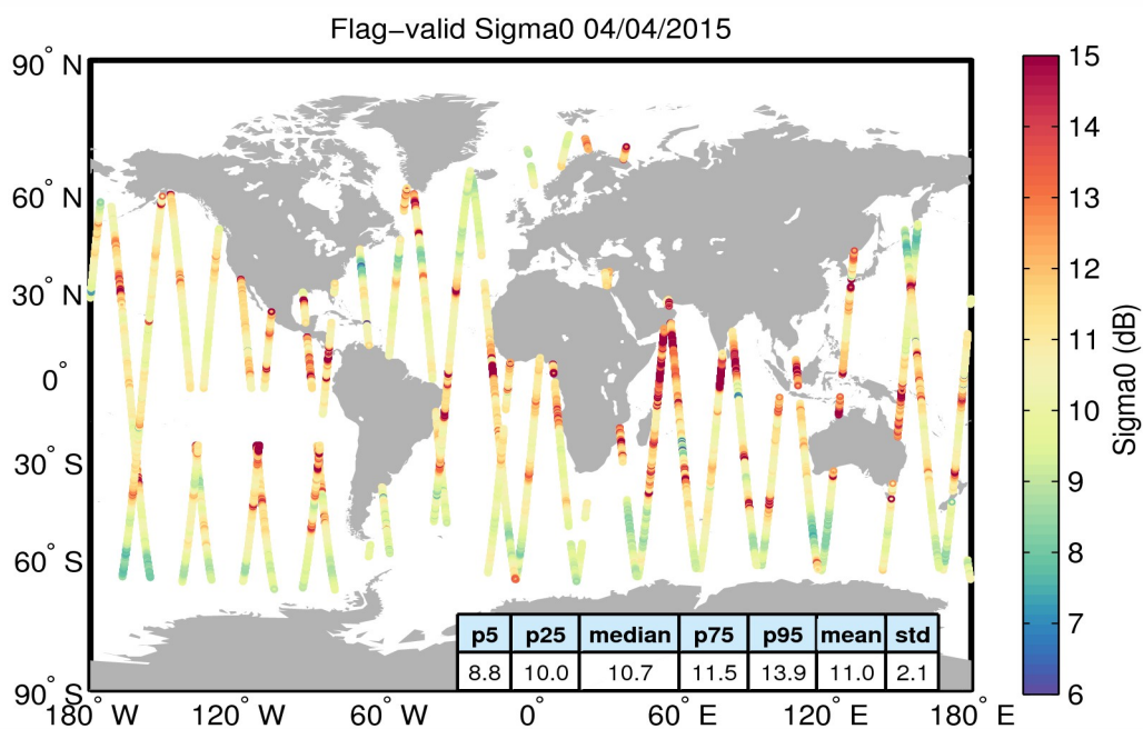
Figure 23. Geographical distribution of flag-valid sigma0 data over oceans and lakes for 04/04/2015. The statistical values shown in the table refer to the sigma0 in dB and are calculated over all measurements shown in the figure.
