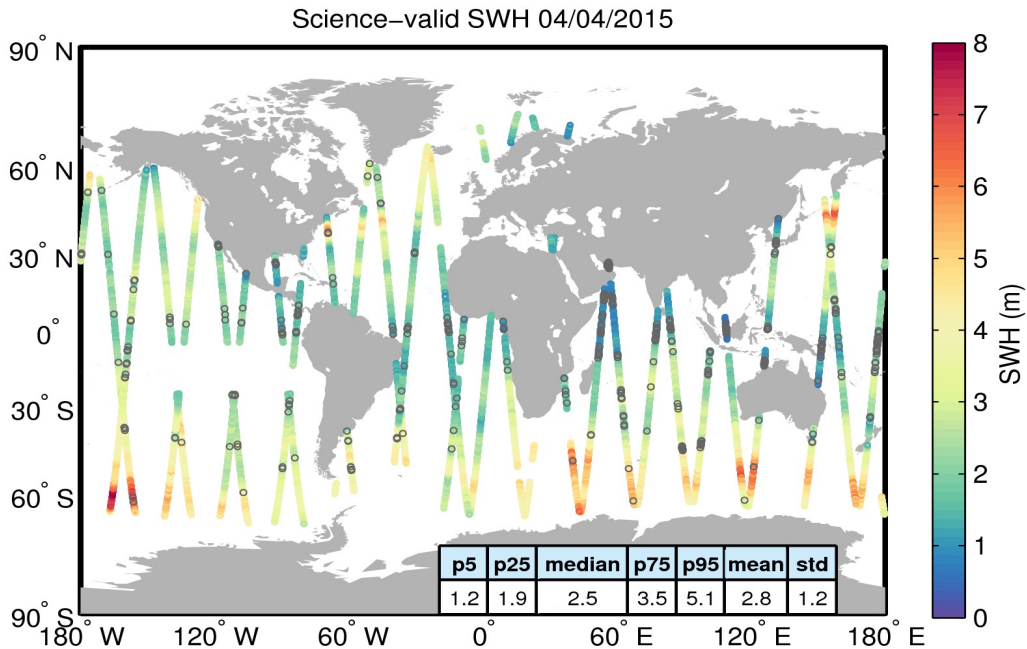
Figure 19. Geographical distribution of science-valid SWH data over oceans and lakes for 04/04/2015. The statistical values shown in the table refer to the SWH in m and are calculated over all measurements shown in the figure. Gray circles denote records that have been rejected based on the editing criteria described in Table 3.
