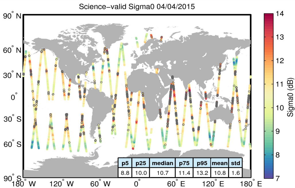
Figure 27. Geographical distribution of science-valid sigma0 data over oceans and lakes for 04/04/2015. The statistical values shown in the table refer to the sigma0 in dB and are calculated over all measurements shown in the figure. Gray circles denote records that have been rejected based on the editing criteria described in Table 4.
