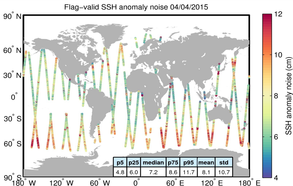
Figure 8. Geographical distribution of flag-valid 20-Hz SSH anomaly measurement noise over oceans and lakes for 04/04/2015. The statistical values shown in the table refer to the SSH anomaly noise and are calculated over all measurements shown in the figure.
