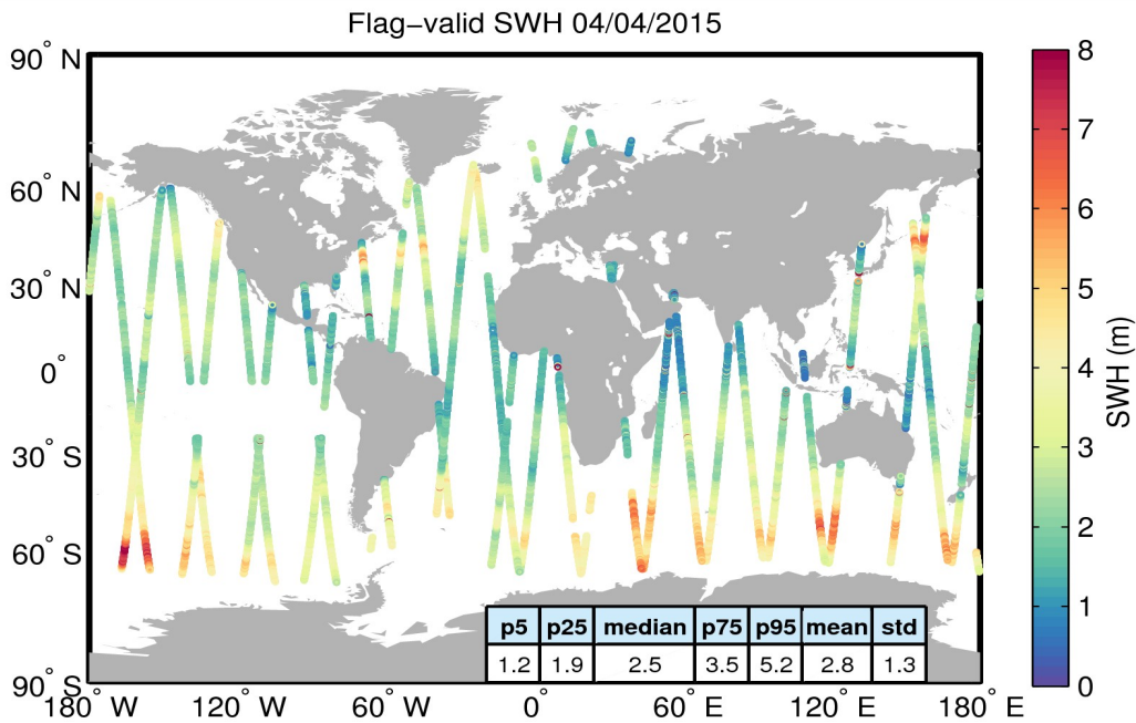
Figure 15. Geographical distribution of flag-valid SWH data over oceans and lakes for 04/04/2015. The statistical values shown in the table refer to the SWH in m and are calculated over all measurements shown in the figure.
