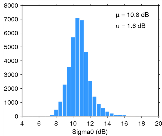
Figure 28. Histogram of science-valid sigma0 over oceans and lakes for 04/04/2015. The mean ( \mu ) and standard deviation ( \sigma ) are also shown. Note that values outside [4 20] dB are excluded from the histogram for the sake of readability but not from the computation of \mu and \sigma .
