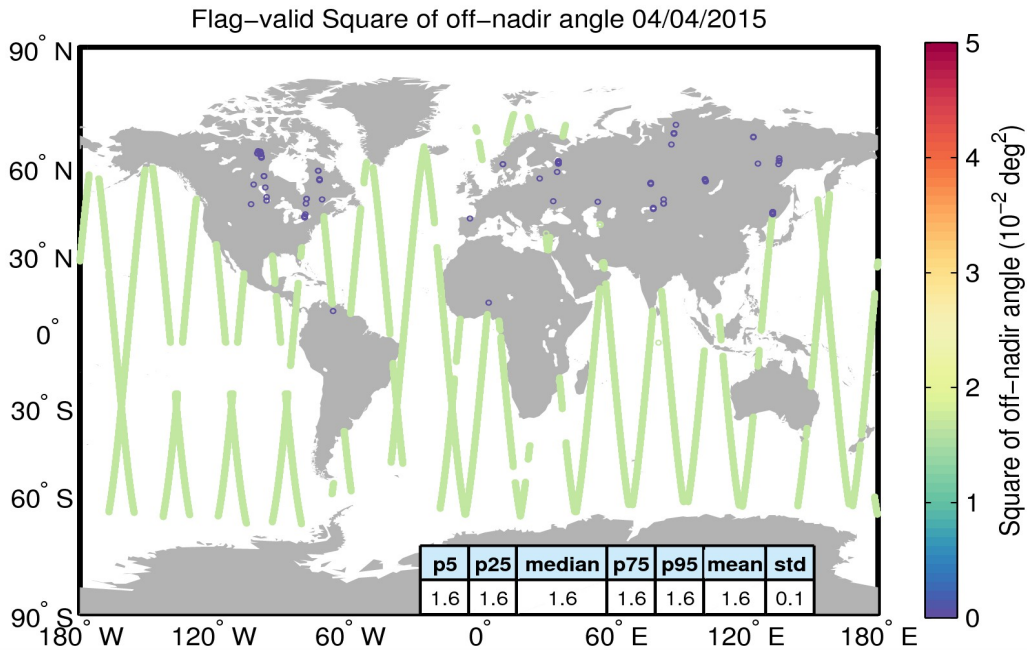
Figure 37. Geographical distribution of flag-valid mispointing data over oceans and lakes for 04/04/2015. The statistical values shown in the table refer to the mispointing in 10^{-2} \text{ deg}^2 and are calculated over all measurements shown in the figure.
