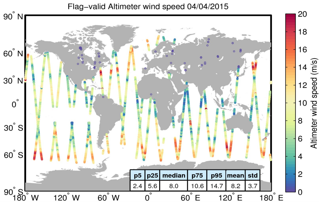
Figure 31. Geographical distribution of flag-valid wind data over oceans and lakes for 04/04/2015. The statistical values shown in the table refer to the wind in m/s and are calculated over all measurements shown in the figure.
