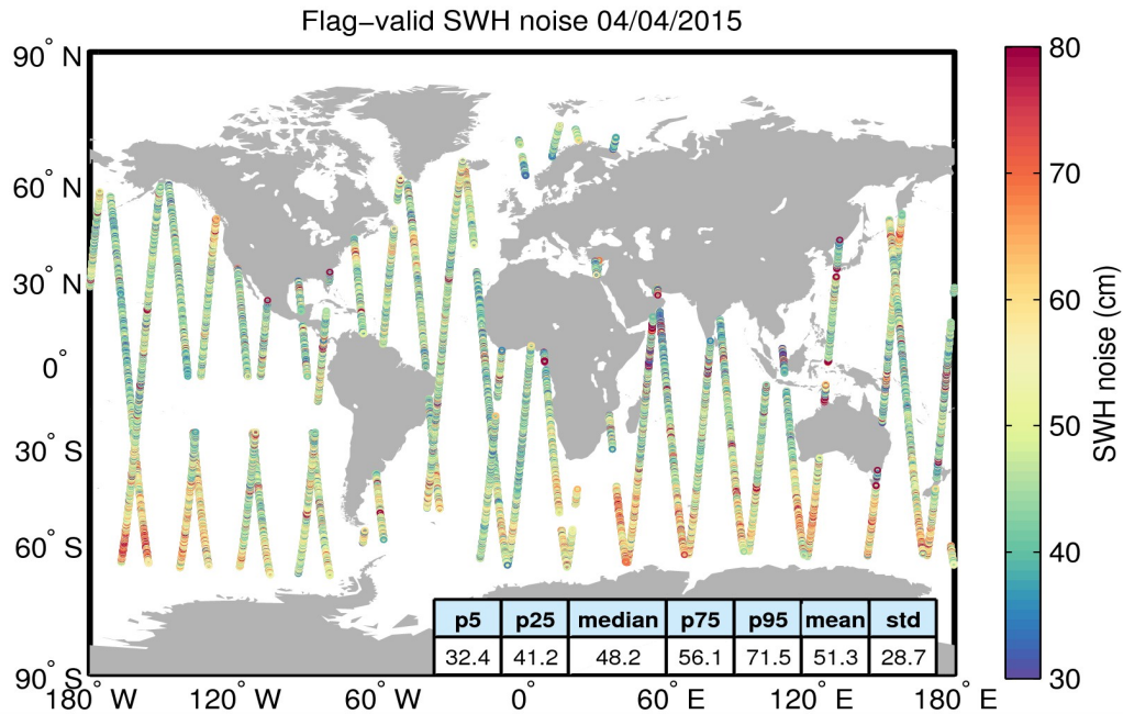
Figure 18. Geographical distribution of flag-valid 20-Hz SWH measurement noise over oceans and lakes for 04/04/2015. The statistical values shown in the figure refer to the SWH noise and are calculated over all measurements shown in the figure.
