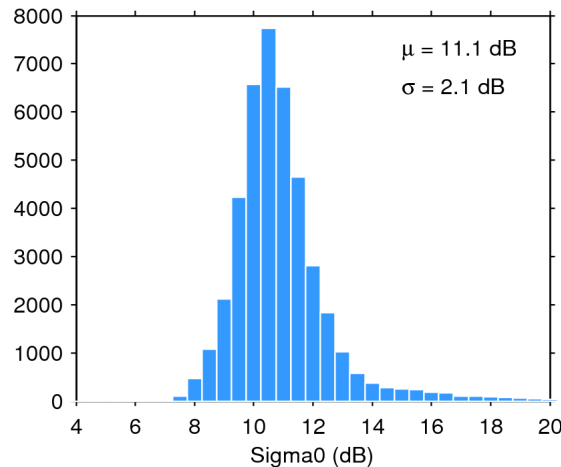
Figure 25. Histogram of flag-valid sigma0 over oceans and lakes for 29/03/2015. The mean ( \mu ) and standard deviation ( \sigma ) are also shown. Note that values outside [4 20] dB are excluded from the histogram for the sake of readability but not from the computation of \mu and \sigma .
