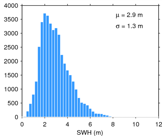
Figure 20. Histogram of science-valid SWH over oceans and lakes for 29/03/2015. The mean ( \mu ) and standard deviation ( \sigma ) are also shown. Note that values larger than 12 m are excluded from the histogram for the sake of readability but not from the computation of \mu and \sigma .
