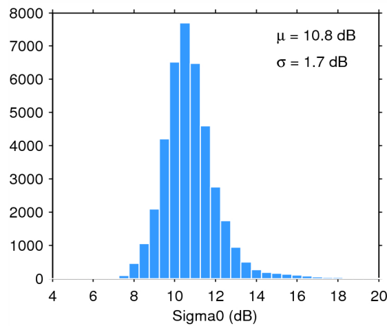
Figure 28. Histogram of science-valid sigma0 over oceans and lakes for 29/03/2015. The mean ( \mu ) and standard deviation ( \sigma ) are also shown. Note that values outside [4 20] dB are excluded from the histogram for the sake of readability but not from the computation of \mu and \sigma .
