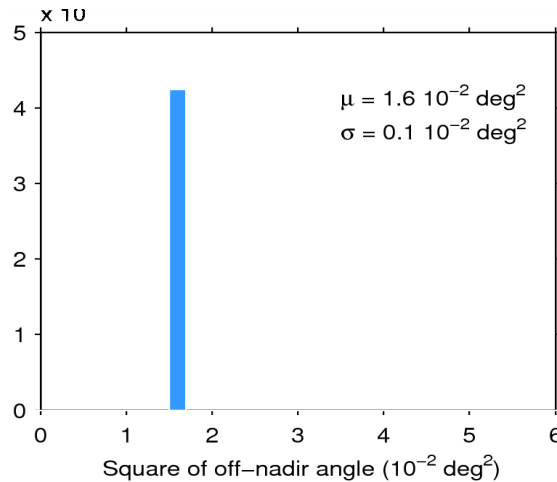
Figure 39. Histogram of flag-valid mispointing over oceans and lakes for 29/03/2015. The mean ( \mu ) and standard deviation ( \sigma ) are also shown. Note that values than 6 \times 10^{-2} \text{ deg}^2 are excluded from the histogram for the sake of readability but not from the computation of \mu and \sigma .
