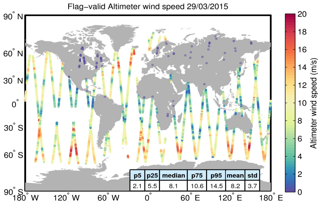
Figure 31. Geographical distribution of flag-valid wind data over oceans and lakes for 29/03/2015. The statistical values shown in the table refer to the wind in m/s and are calculated over all measurements shown in the figure.
