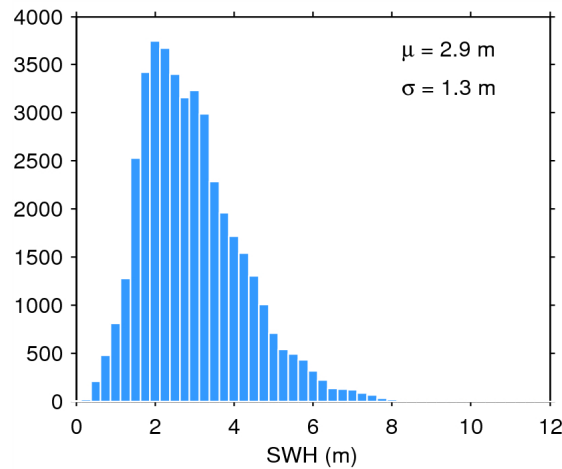
Figure 17. Histogram of flag-valid SWH over oceans and lakes for 29/03/2015. The mean ( \mu ) and standard deviation ( \sigma ) are also shown. Note that values larger than 12 m are excluded from the histogram for the sake of readability but not from the computation of \mu and \sigma .
