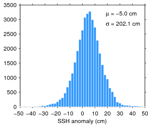
Figure 7. Histogram of flag-valid SSH anomaly over oceans and lakes for 29/03/2015. The mean ( \mu ) and standard deviation ( \sigma ) are also shown. Note that values outside [-50\ 50] cm are excluded from the histogram for the sake of readability but not from the computation of \mu and \sigma .
