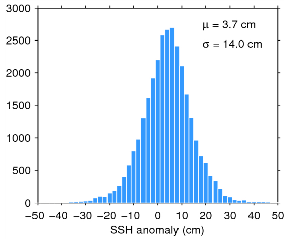
Figure 11. Histogram of science-valid SSH anomaly over oceans and lakes for 29/03/2015. The mean ( \mu ) and standard deviation ( \sigma ) are also shown. Note that values outside [-50 50] cm are excluded from the histogram for the sake of readability but not from the computation of \mu and \sigma .
