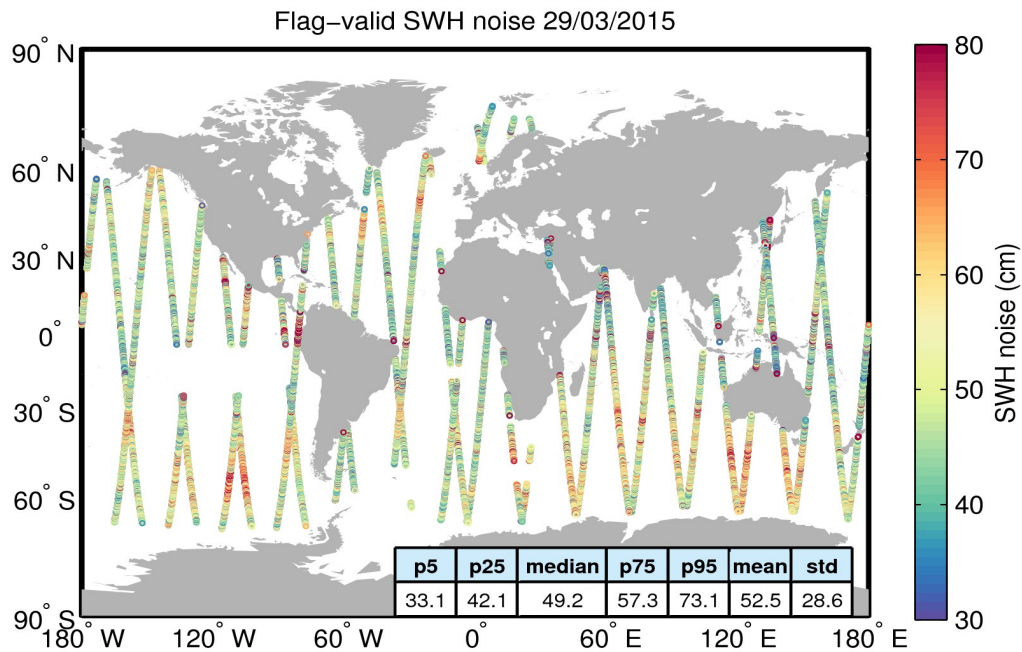
Figure 18. Geographical distribution of flag-valid 20-Hz SWH measurement noise over oceans and lakes for 29/03/2015. The statistical values shown in the figure refer to the SWH noise and are calculated over all measurements shown in the figure.
