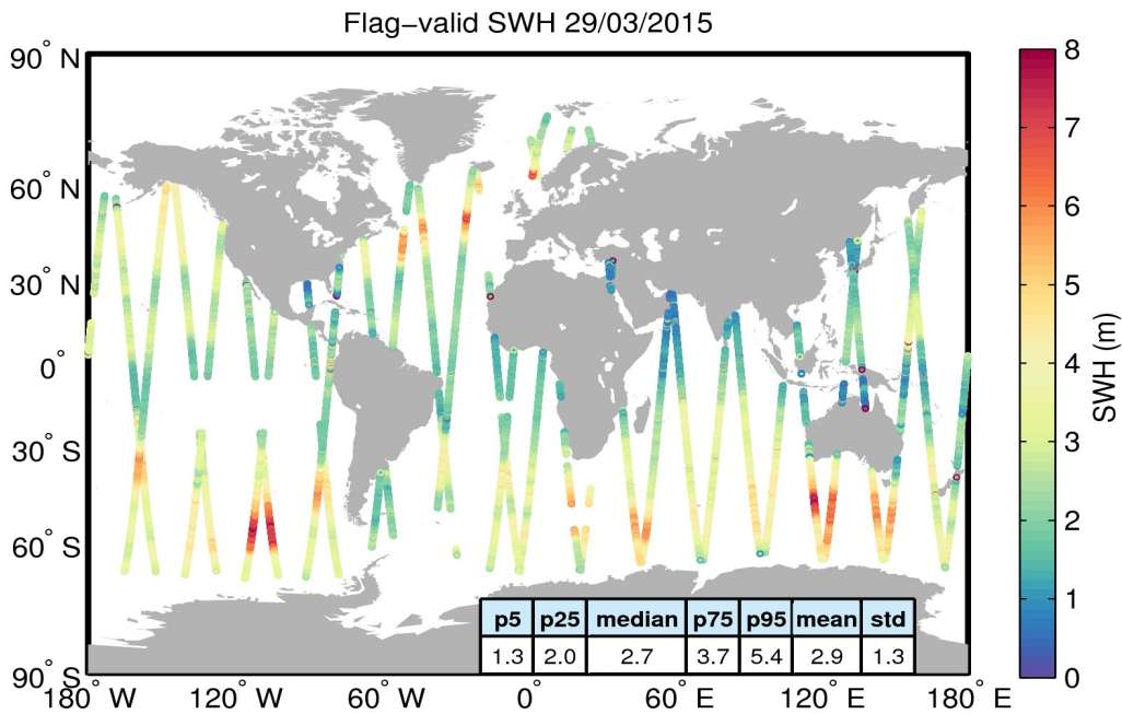
Figure 15. Geographical distribution of flag-valid SWH data over oceans and lakes for 29/03/2015. The statistical values shown in the table refer to the SWH in m and are calculated over all measurements shown in the figure.
