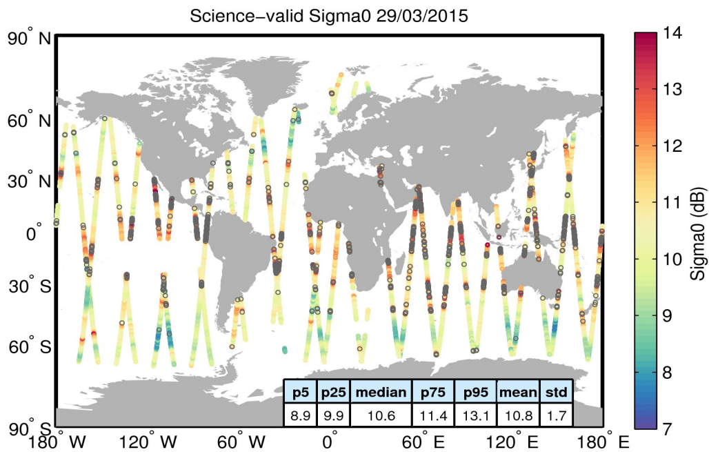
Figure 27. Geographical distribution of science-valid sigma0 data over oceans and lakes for 29/03/2015. The statistical values shown in the table refer to the sigma0 in dB and are calculated over all measurements shown in the figure. Gray circles denote records that have been rejected based on the editing criteria described in Table 4.
