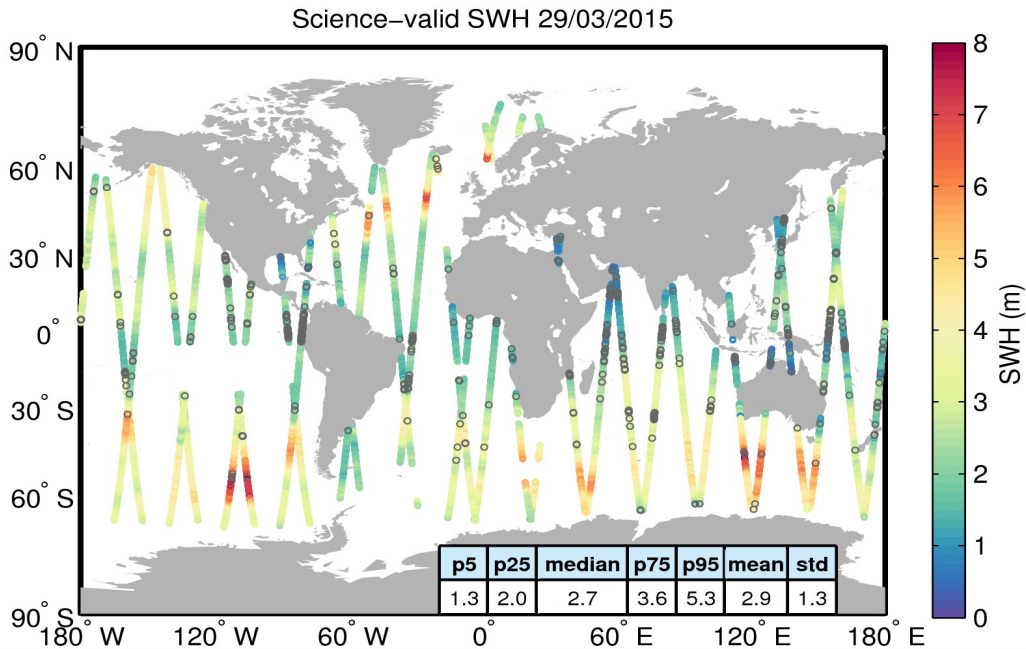
Figure 19. Geographical distribution of science-valid SWH data over oceans and lakes for 29/03/2015. The statistical values shown in the table refer to the SWH in m and are calculated over all measurements shown in the figure. Gray circles denote records that have been rejected based on the editing criteria described in Table 3.
