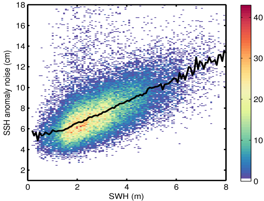
Figure 9. 2D histogram showing flag-valid SSH anomaly noise as a function of SWH for 29/03/2015. The black line denotes the median SSH anomaly as a function of SWH.
