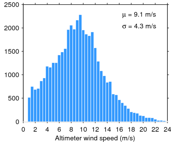
Figure 33. Histogram of flag-valid wind over oceans and lakes for 27/03/2015. The mean ( \mu ) and standard deviation ( \sigma ) are also shown. Note that values larger than 24 m/s are excluded from the histogram for the sake of readability but not from the computation of \mu and \sigma .
