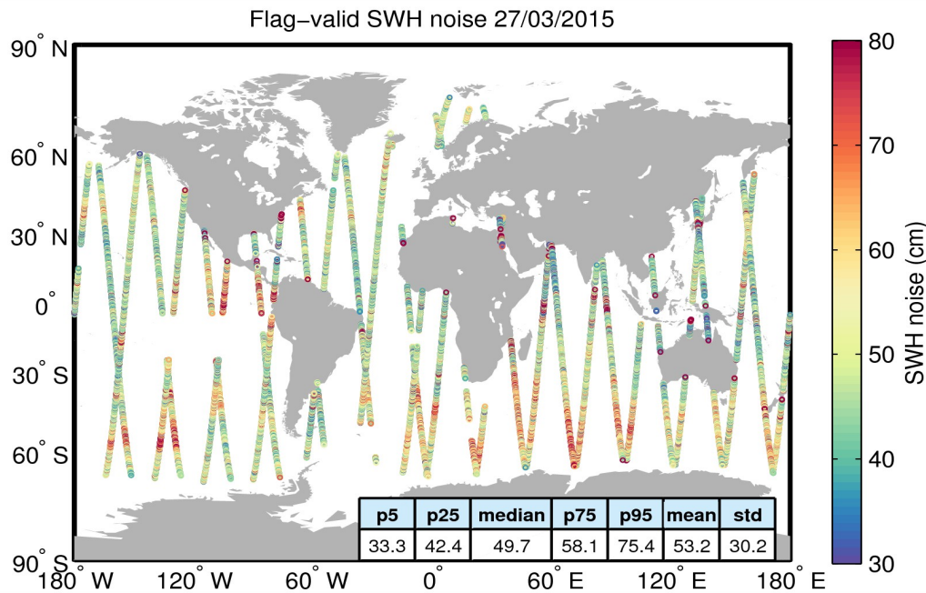
Figure 18. Geographical distribution of flag-valid 20-Hz SWH measurement noise over oceans and lakes for 27/03/2015. The statistical values shown in the figure refer to the SWH noise and are calculated over all measurements shown in the figure.
