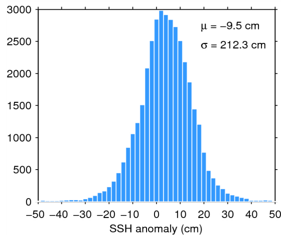
Figure 7. Histogram of flag-valid SSH anomaly over oceans and lakes for 27/03/2015. The mean ( \mu ) and standard deviation ( \sigma ) are also shown. Note that values outside [-50 50] cm are excluded from the histogram for the sake of readability but not from the computation of \mu and \sigma .
