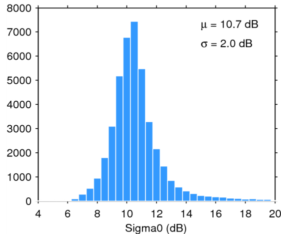
Figure 25. Histogram of flag-valid sigma0 over oceans and lakes for 27/03/2015. The mean ( \mu ) and standard deviation ( \sigma ) are also shown. Note that values outside [4 20] dB are excluded from the histogram for the sake of readability but not from the computation of \mu and \sigma .
