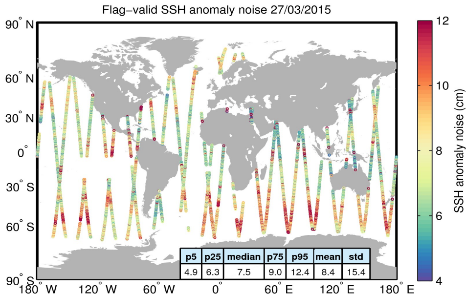
Figure 8. Geographical distribution of flag-valid 20-Hz SSH anomaly measurement noise over oceans and lakes for 27/03/2015. The statistical values shown in the table refer to the SSH anomaly noise and are calculated over all measurements shown in the figure.
