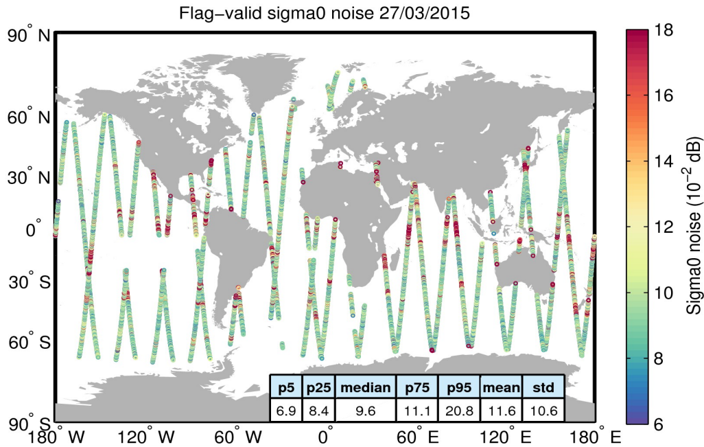
Figure 26. Geographical distribution of flag-valid 20-Hz sigma0 measurement noise over oceans and lakes for 27/03/2015. The statistical values shown in the table refer to the sigma0 noise and are calculated over all measurements shown in the figure.
