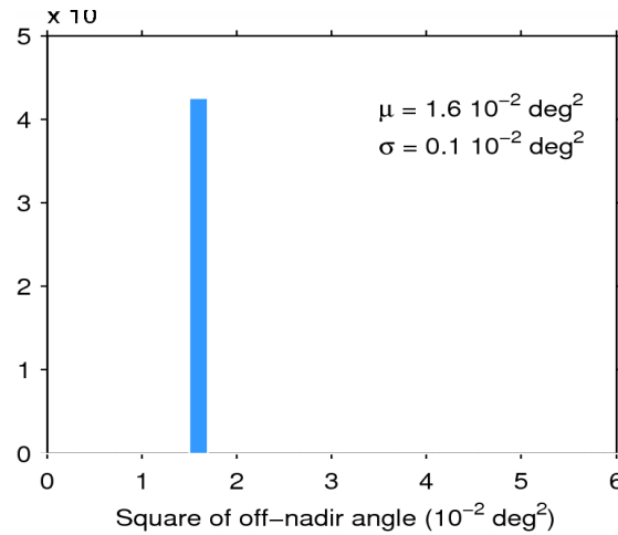
Figure 39. Histogram of flag-valid mispointing over oceans and lakes for 27/03/2015. The mean ( \mu ) and standard deviation ( \sigma ) are also shown. Note that values than 6 \cdot 10^{-2} \text{ deg}^2 are excluded from the histogram for the sake of readability but not from the computation of \mu and \sigma .
