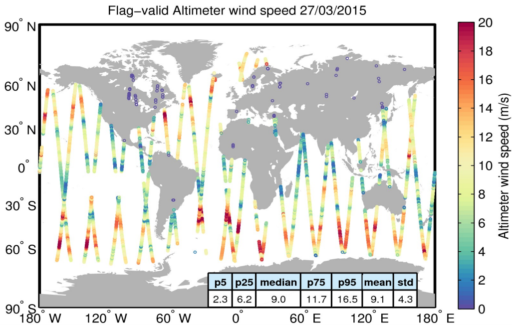
Figure 31. Geographical distribution of flag-valid wind data over oceans and lakes for 27/03/2015. The statistical values shown in the table refer to the wind in m/s and are calculated over all measurements shown in the figure.
