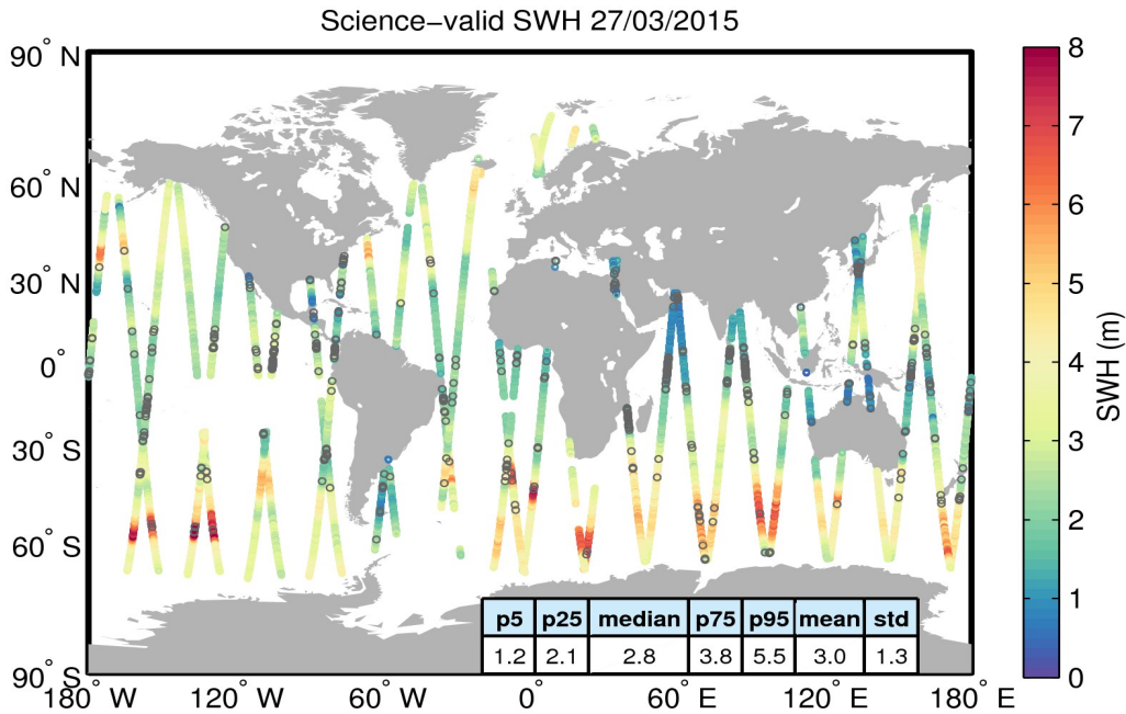
Figure 19. Geographical distribution of science-valid SWH data over oceans and lakes for 27/03/2015. The statistical values shown in the table refer to the SWH in m and are calculated over all measurements shown in the figure. Gray circles denote records that have been rejected based on the editing criteria described in Table 3.
