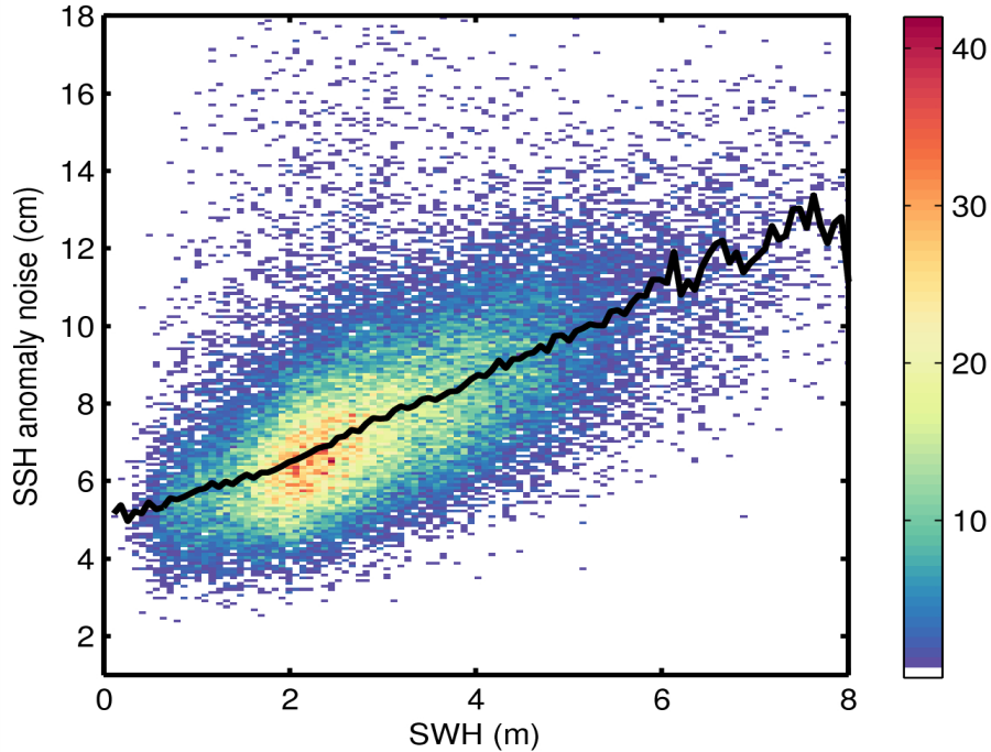
Figure 9. 2D histogram showing flag-valid SSH anomaly noise as a function of SWH for 27/03/2015. The black line denotes the median SSH anomaly as a function of SWH.
