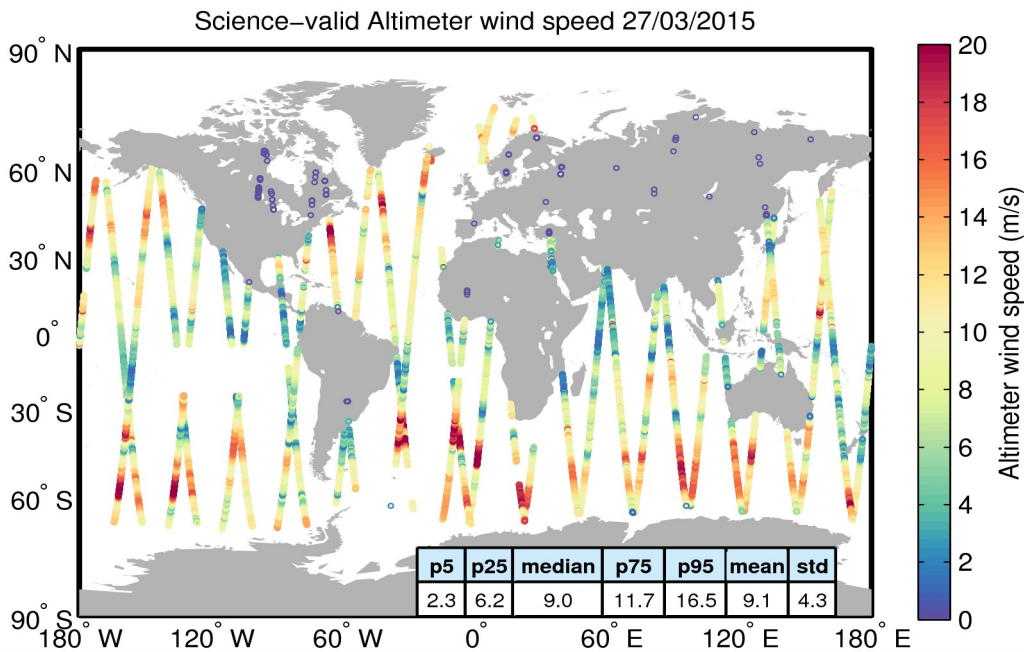
Figure 34. Geographical distribution of science-valid wind data over oceans and lakes for 27/03/2015. The statistical values shown in the table refer to the wind in m/s and are calculated over all measurements shown in the figure. Gray circles denote records that have been rejected based on the editing criteria described in Table 5.
