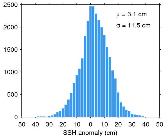
Figure 11. Histogram of science-valid SSH anomaly over oceans and lakes for 27/03/2015. The mean ( \mu ) and standard deviation ( \sigma ) are also shown. Note that values outside [-50 50] cm are excluded from the histogram for the sake of readability but not from the computation of \mu and \sigma .
