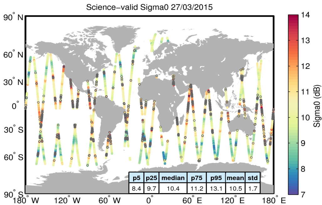
Figure 27. Geographical distribution of science-valid sigma0 data over oceans and lakes for 27/03/2015. The statistical values shown in the table refer to the sigma0 in dB and are calculated over all measurements shown in the figure. Gray circles denote records that have been rejected based on the editing criteria described in Table 4.
