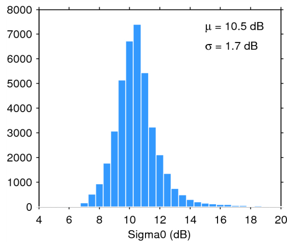
Figure 28. Histogram of science-valid sigma0 over oceans and lakes for 27/03/2015. The mean ( \mu ) and standard deviation ( \sigma ) are also shown. Note that values outside [4 20] dB are excluded from the histogram for the sake of readability but not from the computation of \mu and \sigma .
