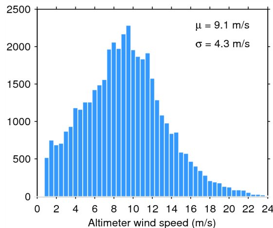
Figure 35. Histogram of science-valid wind over oceans and lakes for 27/03/2015. The mean ( \mu ) and standard deviation ( \sigma ) are also shown. Note that values larger than 24 m/s are excluded from the histogram for the sake of readability but not from the computation of \mu and \sigma .
