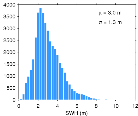
Figure 20. Histogram of science-valid SWH over oceans and lakes for 27/03/2015. The mean ( \mu ) and standard deviation ( \sigma ) are also shown. Note that values larger than 12 m are excluded from the histogram for the sake of readability but not from the computation of \mu and \sigma .
