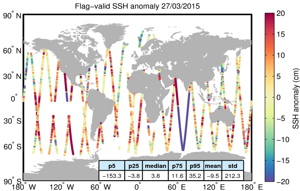
Figure 5. Geographical distribution of flag-valid 1-Hz SSH anomaly data over oceans and lakes for 27/03/2015. The statistical values shown in the table refer to the SSH anomaly in cm and are calculated over all measurements shown in the figure.
