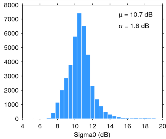
Figure 28. Histogram of science-valid sigma0 over oceans and lakes for 23/03/2015. The mean ( \mu ) and standard deviation ( \sigma ) are also shown. Note that values outside [4 20] dB are excluded from the histogram for the sake of readability but not from the computation of \mu and \sigma .
