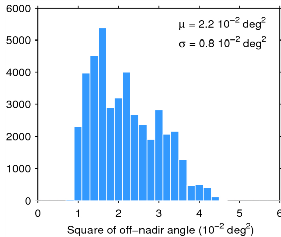
Figure 39. Histogram of flag-valid mispointing over oceans and lakes for 23/03/2015. The mean ( \mu ) and standard deviation ( \sigma ) are also shown. Note that values than 6 \cdot 10^{-2} \text{ deg}^2 are excluded from the histogram for the sake of readability but not from the computation of \mu and \sigma .
