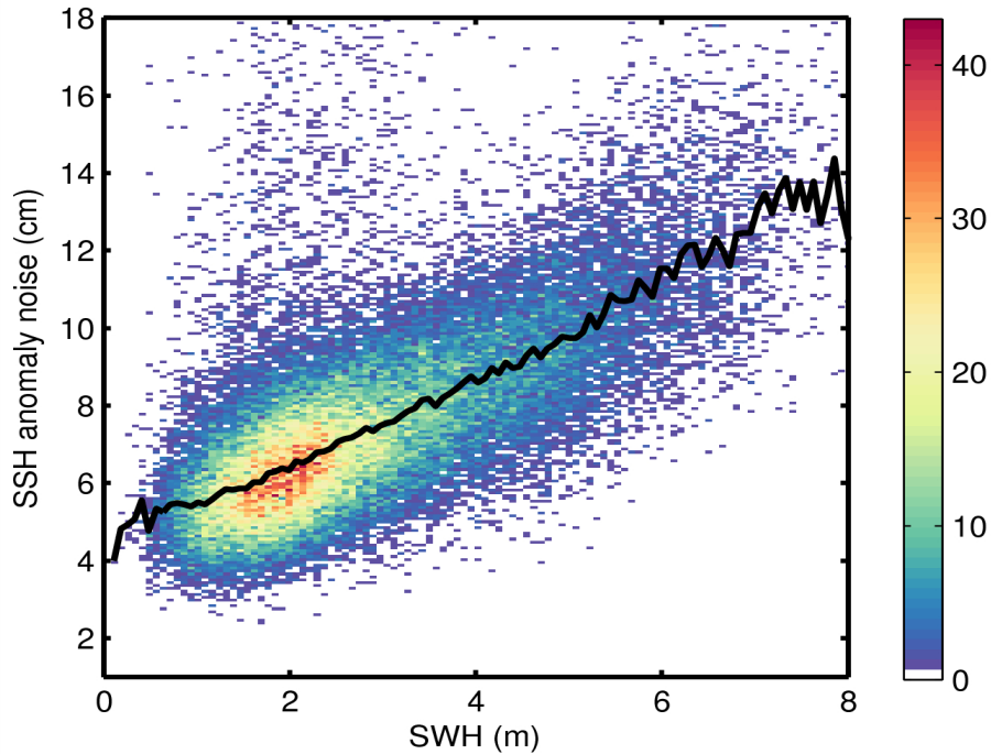
Figure 9. 2D histogram showing flag-valid SSH anomaly noise as a function of SWH for 23/03/2015. The black line denotes the median SSH anomaly as a function of SWH.
