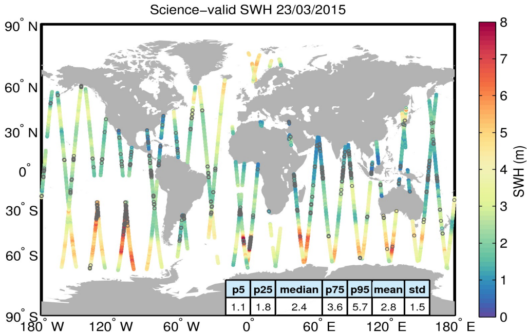
Figure 19. Geographical distribution of science-valid SWH data over oceans and lakes for 23/03/2015. The statistical values shown in the table refer to the SWH in m and are calculated over all measurements shown in the figure. Gray circles denote records that have been rejected based on the editing criteria described in Table 3.
