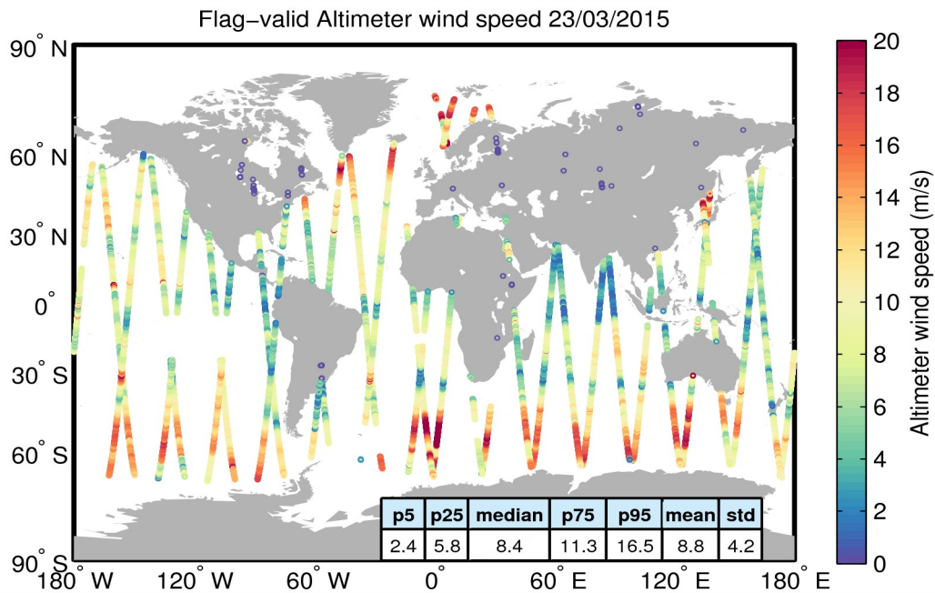
Figure 31. Geographical distribution of flag-valid wind data over oceans and lakes for 23/03/2015. The statistical values shown in the table refer to the wind in m/s and are calculated over all measurements shown in the figure.
