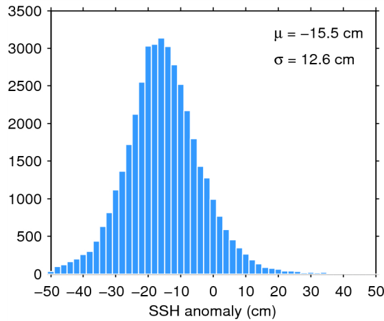
Figure 11. Histogram of science-valid SSH anomaly over oceans and lakes for 23/03/2015. The mean ( \mu ) and standard deviation ( \sigma ) are also shown. Note that values outside [-50 50] cm are excluded from the histogram for the sake of readability but not from the computation of \mu and \sigma .
