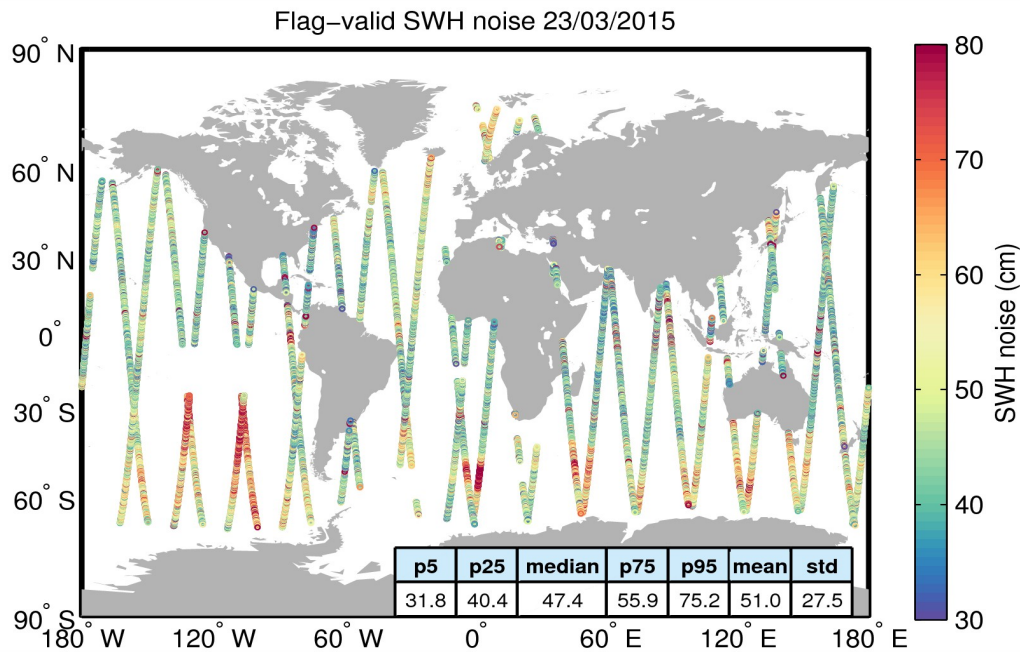
Figure 18. Geographical distribution of flag-valid 20-Hz SWH measurement noise over oceans and lakes for 23/03/2015. The statistical values shown in the figure refer to the SWH noise and are calculated over all measurements shown in the figure.
