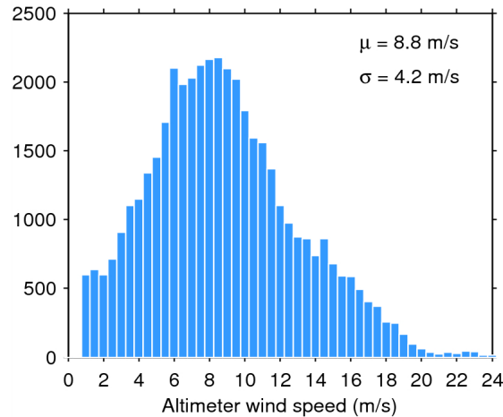
Figure 33. Histogram of flag-valid wind over oceans and lakes for 23/03/2015. The mean ( \mu ) and standard deviation ( \sigma ) are also shown. Note that values larger than 24 m/s are excluded from the histogram for the sake of readability but not from the computation of \mu and \sigma .
