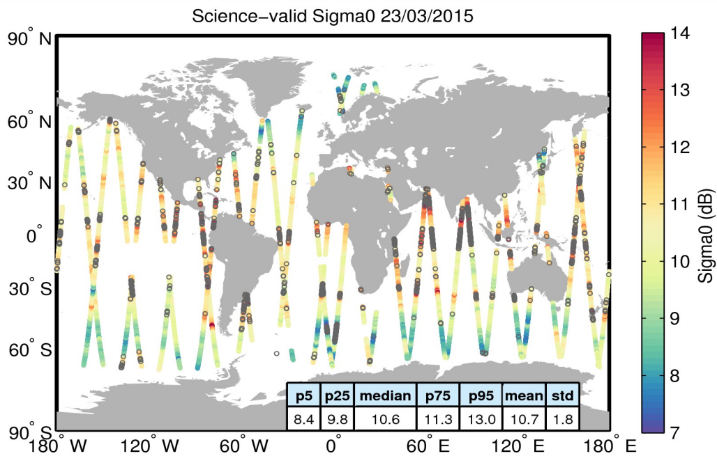
Figure 27. Geographical distribution of science-valid sigma0 data over oceans and lakes for 23/03/2015. The statistical values shown in the table refer to the sigma0 in dB and are calculated over all measurements shown in the figure. Gray circles denote records that have been rejected based on the editing criteria described in Table 4.
