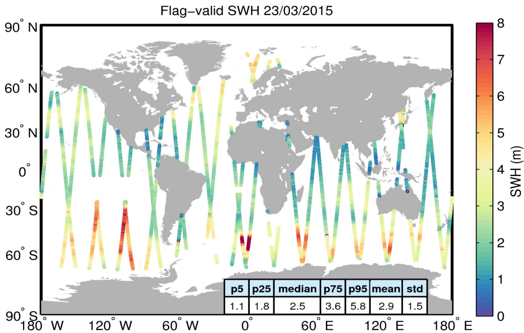
Figure 15. Geographical distribution of flag-valid SWH data over oceans and lakes for 23/03/2015. The statistical values shown in the table refer to the SWH in m and are calculated over all measurements shown in the figure.
