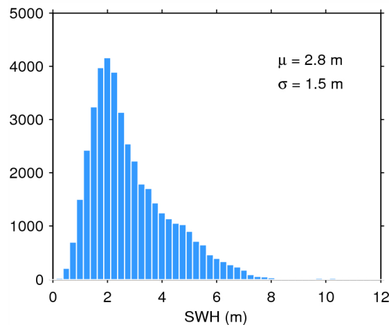
Figure 20. Histogram of science-valid SWH over oceans and lakes for 23/03/2015. The mean ( \mu ) and standard deviation ( \sigma ) are also shown. Note that values larger than 12 m are excluded from the histogram for the sake of readability but not from the computation of \mu and \sigma .
