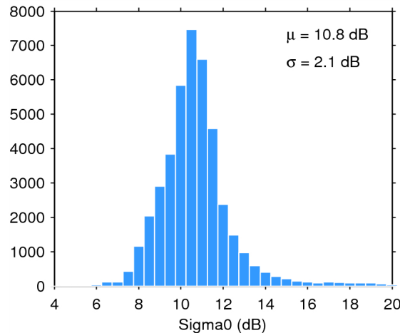
Figure 25. Histogram of flag-valid sigma0 over oceans and lakes for 23/03/2015. The mean ( \mu ) and standard deviation ( \sigma ) are also shown. Note that values outside [4 20] dB are excluded from the histogram for the sake of readability but not from the computation of \mu and \sigma .
