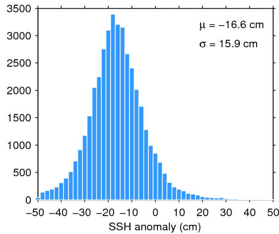
Figure 7. Histogram of flag-valid SSH anomaly over oceans and lakes for 21/03/2015. The mean ( \mu ) and standard deviation ( \sigma ) are also shown. Note that values outside [-50\ 50] cm are excluded from the histogram for the sake of readability but not from the computation of \mu and \sigma .
