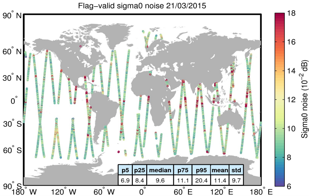
Figure 26. Geographical distribution of flag-valid 20-Hz sigma0 measurement noise over oceans and lakes for 21/03/2015. The statistical values shown in the table refer to the sigma0 noise and are calculated over all measurements shown in the figure.
