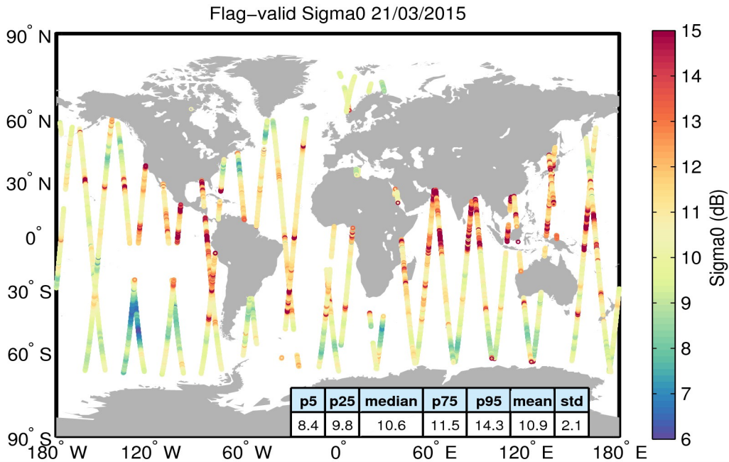
Figure 23. Geographical distribution of flag-valid sigma0 data over oceans and lakes for 21/03/2015. The statistical values shown in the table refer to the sigma0 in dB and are calculated over all measurements shown in the figure.
