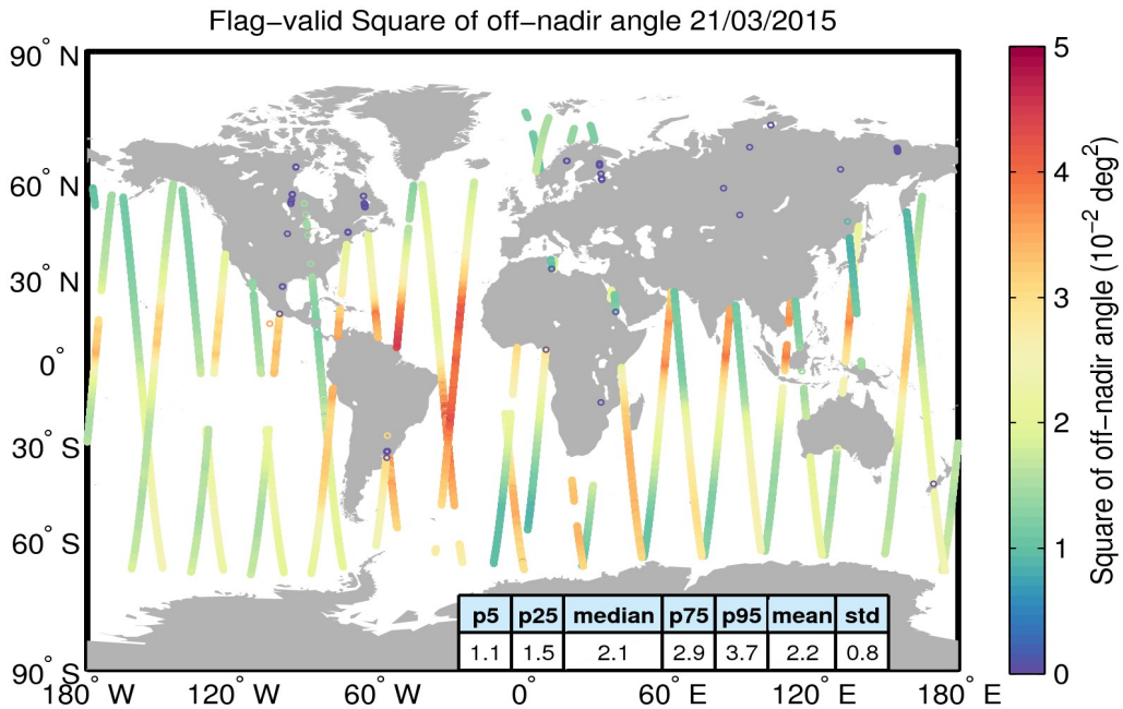
Figure 37. Geographical distribution of flag-valid mispointing data over oceans and lakes for 21/03/2015. The statistical values shown in the table refer to the mispointing in 10^{-2} \text{deg}^2 and are calculated over all measurements shown in the figure.
