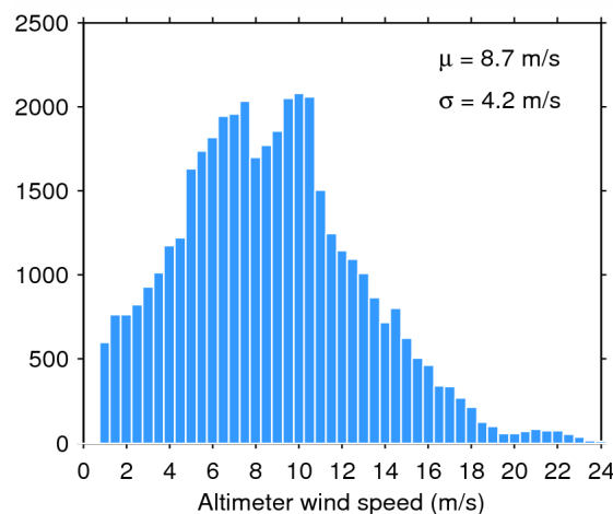
Figure 35. Histogram of science-valid wind over oceans and lakes for 21/03/2015. The mean ( \mu ) and standard deviation ( \sigma ) are also shown. Note that values larger than 24 m/s are excluded from the histogram for the sake of readability but not from the computation of \mu and \sigma .
