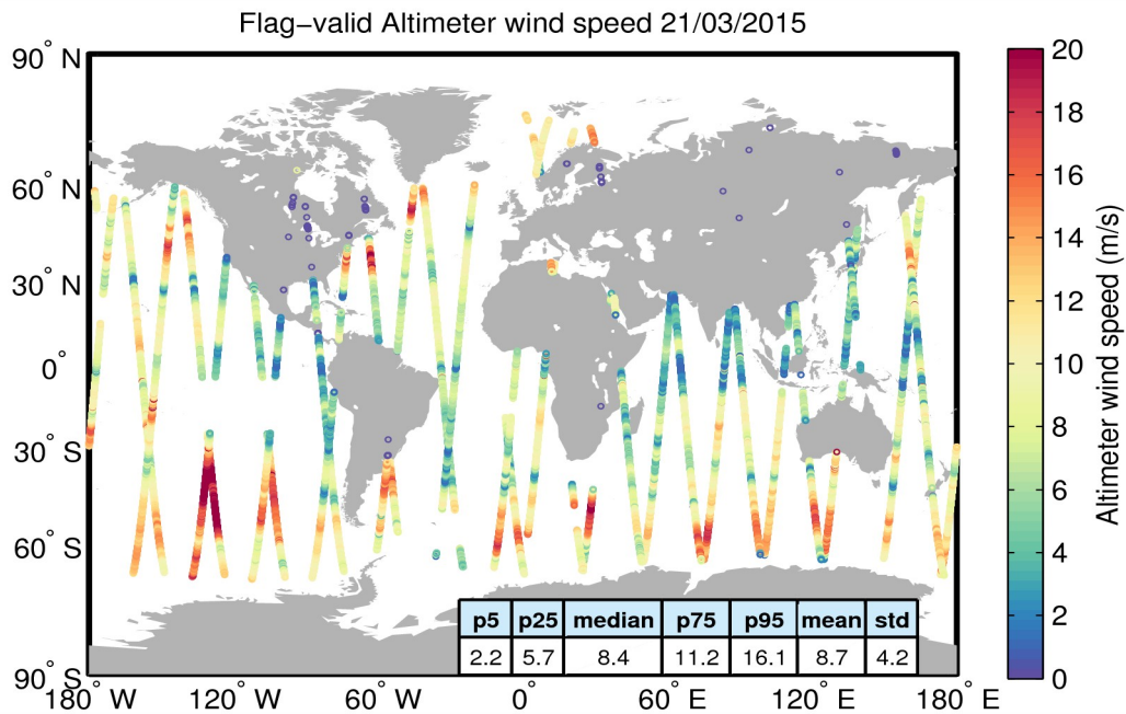
Figure 31. Geographical distribution of flag-valid wind data over oceans and lakes for 21/03/2015. The statistical values shown in the table refer to the wind in m/s and are calculated over all measurements shown in the figure.
