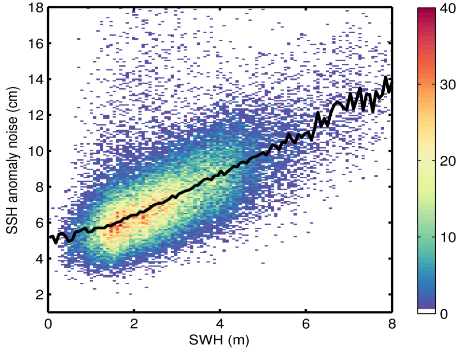
Figure 9. 2D histogram showing flag-valid SSH anomaly noise as a function of SWH for 21/03/2015. The black line denotes the median SSH anomaly as a function of SWH.
