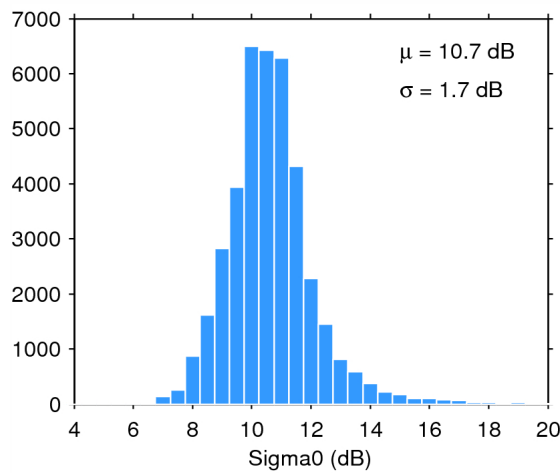
Figure 28. Histogram of science-valid sigma0 over oceans and lakes for 21/03/2015. The mean ( \mu ) and standard deviation ( \sigma ) are also shown. Note that values outside [4 20] dB are excluded from the histogram for the sake of readability but not from the computation of \mu and \sigma .
