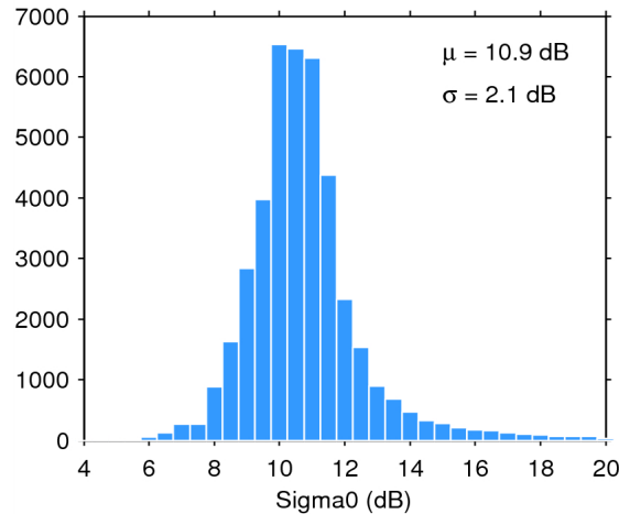
Figure 25. Histogram of flag-valid sigma0 over oceans and lakes for 21/03/2015. The mean ( \mu ) and standard deviation ( \sigma ) are also shown. Note that values outside [4 20] dB are excluded from the histogram for the sake of readability but not from the computation of \mu and \sigma .
