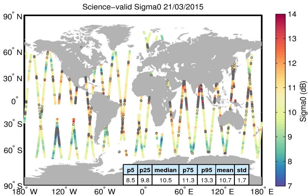
Figure 27. Geographical distribution of science-valid sigma0 data over oceans and lakes for 21/03/2015. The statistical values shown in the table refer to the sigma0 in dB and are calculated over all measurements shown in the figure. Gray circles denote records that have been rejected based on the editing criteria described in Table 4.
