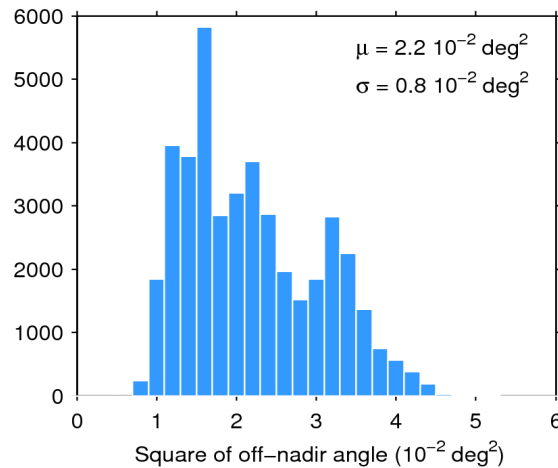
Figure 39. Histogram of flag-valid mispointing over oceans and lakes for 21/03/2015. The mean ( \mu ) and standard deviation ( \sigma ) are also shown. Note that values than 6 \cdot 10^{-2} \text{ deg}^2 are excluded from the histogram for the sake of readability but not from the computation of \mu and \sigma .
