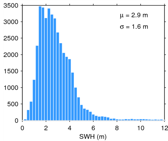
Figure 17. Histogram of flag-valid SWH over oceans and lakes for 21/03/2015. The mean ( \mu ) and standard deviation ( \sigma ) are also shown. Note that values larger than 12 m are excluded from the histogram for the sake of readability but not from the computation of \mu and \sigma .
