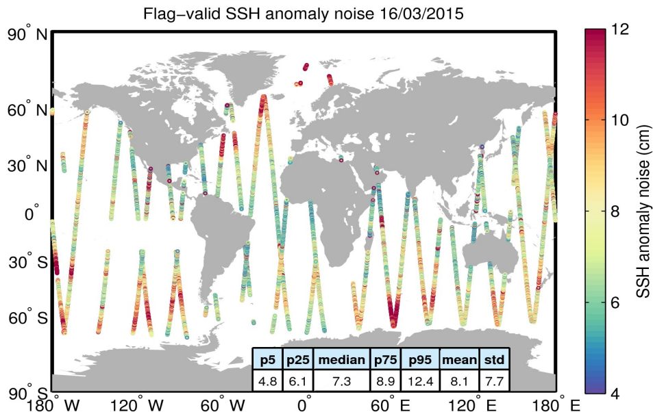
Figure 8. Geographical distribution of flag-valid 20-Hz SSH anomaly measurement noise over oceans and lakes for 16/03/2015. The statistical values shown in the table refer to the SSH anomaly noise and are calculated over all measurements shown in the figure.
