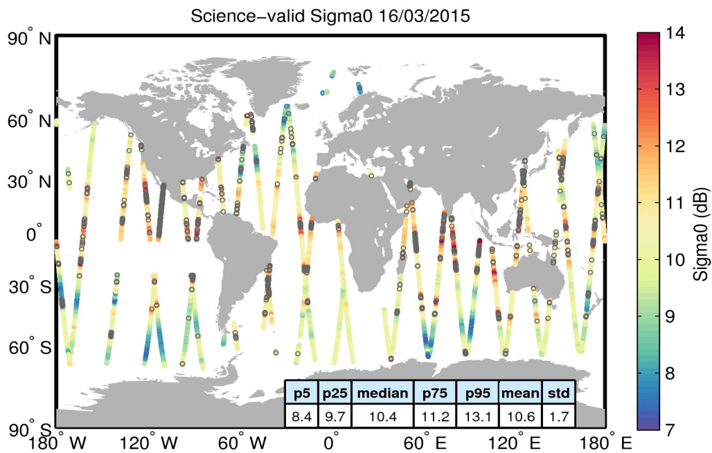
Figure 27. Geographical distribution of science-valid sigma0 data over oceans and lakes for 16/03/2015. The statistical values shown in the table refer to the sigma0 in dB and are calculated over all measurements shown in the figure. Gray circles denote records that have been rejected based on the editing criteria described in Table 4.
