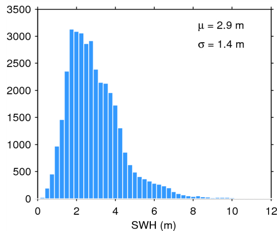
Figure 20. Histogram of science-valid SWH over oceans and lakes for 16/03/2015. The mean ( \mu ) and standard deviation ( \sigma ) are also shown. Note that values larger than 12 m are excluded from the histogram for the sake of readability but not from the computation of \mu and \sigma .
