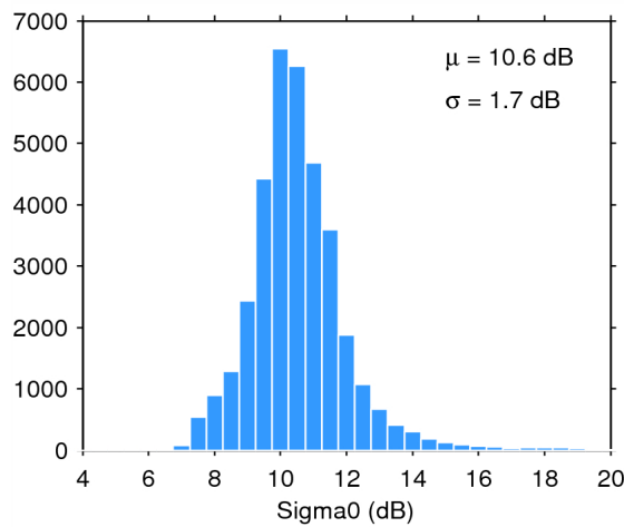
Figure 28. Histogram of science-valid sigma0 over oceans and lakes for 16/03/2015. The mean ( \mu ) and standard deviation ( \sigma ) are also shown. Note that values outside [4 20] dB are excluded from the histogram for the sake of readability but not from the computation of \mu and \sigma .
