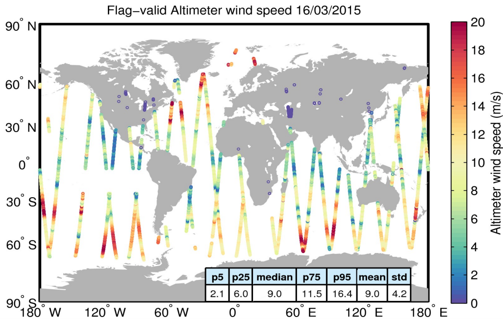
Figure 31. Geographical distribution of flag-valid wind data over oceans and lakes for 16/03/2015. The statistical values shown in the table refer to the wind in m/s and are calculated over all measurements shown in the figure.
