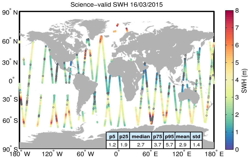
Figure 19. Geographical distribution of science-valid SWH data over oceans and lakes for 16/03/2015. The statistical values shown in the table refer to the SWH in m and are calculated over all measurements shown in the figure. Gray circles denote records that have been rejected based on the editing criteria described in Table 3.
