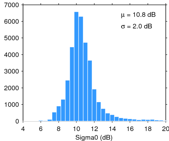
Figure 25. Histogram of flag-valid sigma0 over oceans and lakes for 16/03/2015. The mean ( \mu ) and standard deviation ( \sigma ) are also shown. Note that values outside [4 20] dB are excluded from the histogram for the sake of readability but not from the computation of \mu and \sigma .
