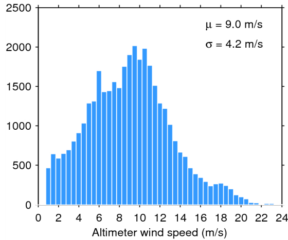
Figure 33. Histogram of flag-valid wind over oceans and lakes for 16/03/2015. The mean ( \mu ) and standard deviation ( \sigma ) are also shown. Note that values larger than 24 m/s are excluded from the histogram for the sake of readability but not from the computation of \mu and \sigma .
