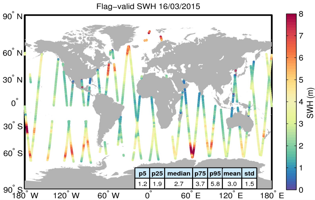
Figure 15. Geographical distribution of flag-valid SWH data over oceans and lakes for 16/03/2015. The statistical values shown in the table refer to the SWH in m and are calculated over all measurements shown in the figure.
