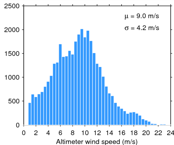
Figure 35. Histogram of science-valid wind over oceans and lakes for 16/03/2015. The mean ( \mu ) and standard deviation ( \sigma ) are also shown. Note that values larger than 24 m/s are excluded from the histogram for the sake of readability but not from the computation of \mu and \sigma .
