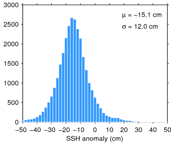
Figure 11. Histogram of science-valid SSH anomaly over oceans and lakes for 16/03/2015. The mean ( \mu ) and standard deviation ( \sigma ) are also shown. Note that values outside [-50 50] cm are excluded from the histogram for the sake of readability but not from the computation of \mu and \sigma .
