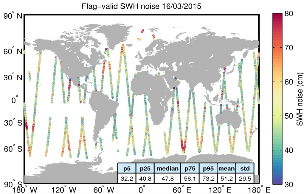
Figure 18. Geographical distribution of flag-valid 20-Hz SWH measurement noise over oceans and lakes for 16/03/2015. The statistical values shown in the figure refer to the SWH noise and are calculated over all measurements shown in the figure.
