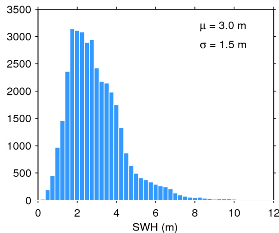
Figure 17. Histogram of flag-valid SWH over oceans and lakes for 16/03/2015. The mean ( \mu ) and standard deviation ( \sigma ) are also shown. Note that values larger than 12 m are excluded from the histogram for the sake of readability but not from the computation of \mu and \sigma .
