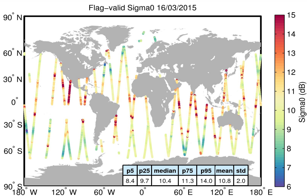
Figure 23. Geographical distribution of flag-valid sigma0 data over oceans and lakes for 16/03/2015. The statistical values shown in the table refer to the sigma0 in dB and are calculated over all measurements shown in the figure.
