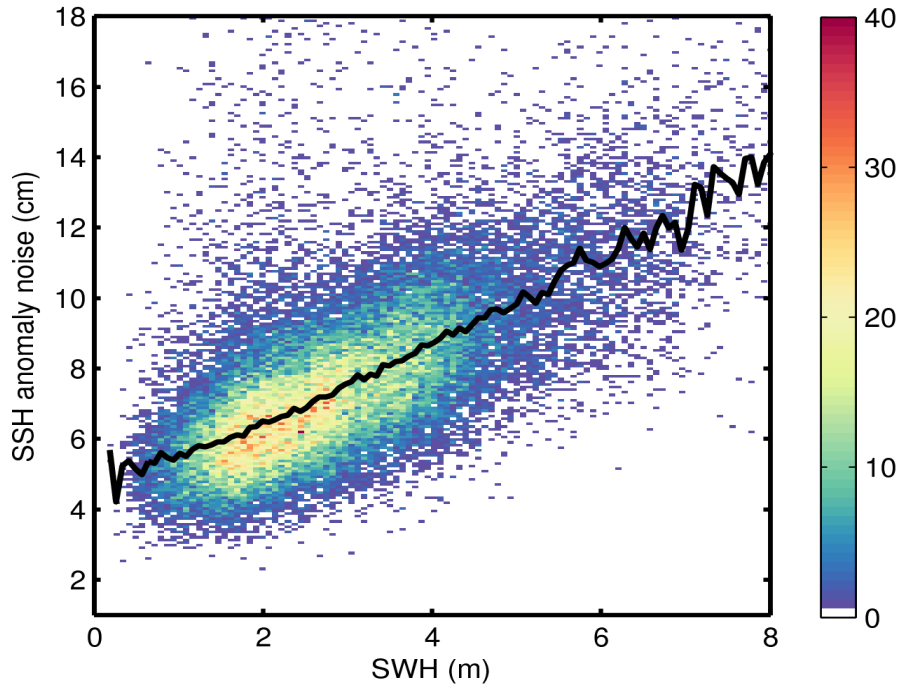
Figure 9. 2D histogram showing flag-valid SSH anomaly noise as a function of SWH for 16/03/2015. The black line denotes the median SSH anomaly as a function of SWH.
