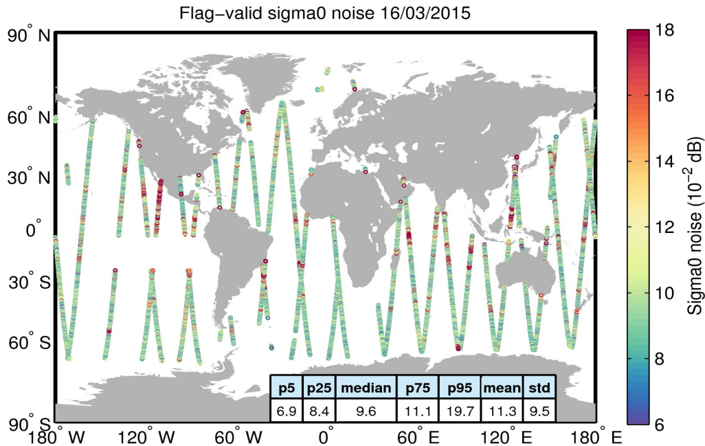
Figure 26. Geographical distribution of flag-valid 20-Hz sigma0 measurement noise over oceans and lakes for 16/03/2015. The statistical values shown in the table refer to the sigma0 noise and are calculated over all measurements shown in the figure.
