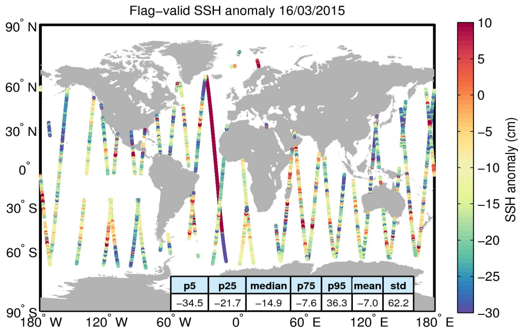
Figure 5. Geographical distribution of flag-valid 1-Hz SSH anomaly data over oceans and lakes for 16/03/2015. The statistical values shown in the table refer to the SSH anomaly in cm and are calculated over all measurements shown in the figure.
