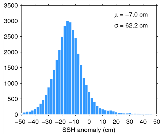
Figure 7. Histogram of flag-valid SSH anomaly over oceans and lakes for 16/03/2015. The mean ( \mu ) and standard deviation ( \sigma ) are also shown. Note that values outside [-50\ 50] cm are excluded from the histogram for the sake of readability but not from the computation of \mu and \sigma .
