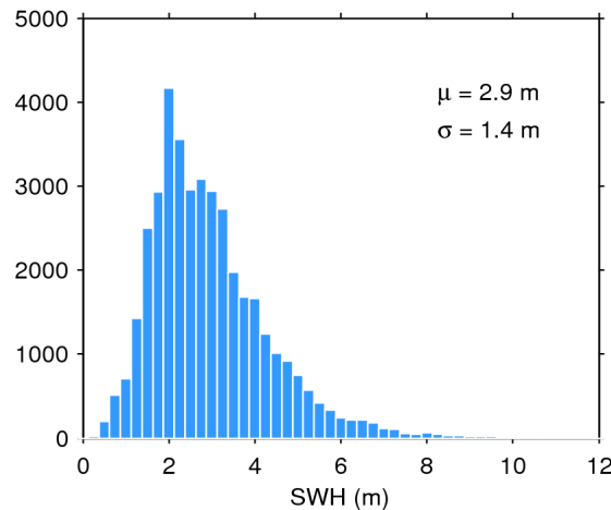
Figure 20. Histogram of science-valid SWH over oceans and lakes for 14/03/2015. The mean ( \mu ) and standard deviation ( \sigma ) are also shown. Note that values larger than 12 m are excluded from the histogram for the sake of readability but not from the computation of \mu and \sigma .
