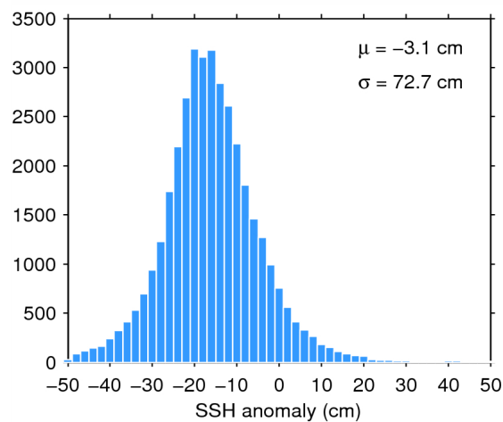
Figure 7. Histogram of flag-valid SSH anomaly over oceans and lakes for 14/03/2015. The mean ( \mu ) and standard deviation ( \sigma ) are also shown. Note that values outside [-50 50] cm are excluded from the histogram for the sake of readability but not from the computation of \mu and \sigma .
