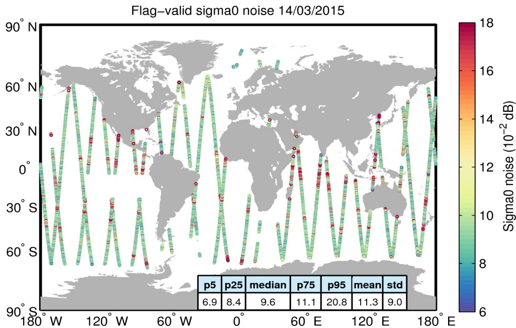
Figure 26. Geographical distribution of flag-valid 20-Hz sigma0 measurement noise over oceans and lakes for 14/03/2015. The statistical values shown in the table refer to the sigma0 noise and are calculated over all measurements shown in the figure.
