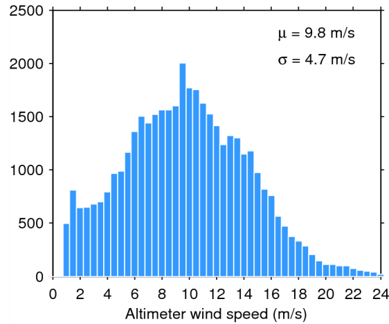
Figure 33. Histogram of flag-valid wind over oceans and lakes for 14/03/2015. The mean ( \mu ) and standard deviation ( \sigma ) are also shown. Note that values larger than 24 m/s are excluded from the histogram for the sake of readability but not from the computation of \mu and \sigma .
