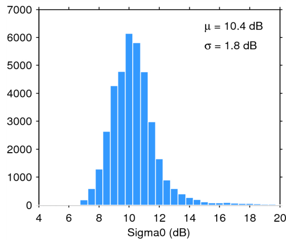
Figure 28. Histogram of science-valid sigma0 over oceans and lakes for 14/03/2015. The mean ( \mu ) and standard deviation ( \sigma ) are also shown. Note that values outside [4 20] dB are excluded from the histogram for the sake of readability but not from the computation of \mu and \sigma .
