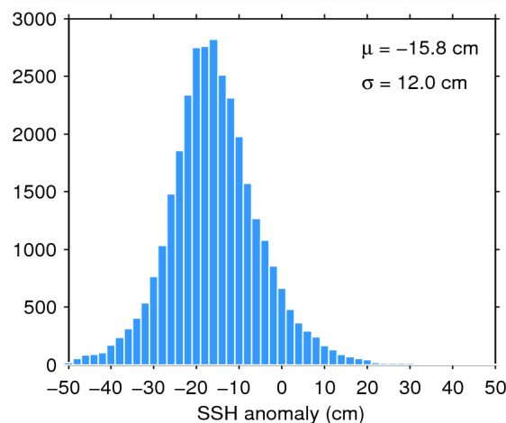
Figure 11. Histogram of science-valid SSH anomaly over oceans and lakes for 14/03/2015. The mean ( \mu ) and standard deviation ( \sigma ) are also shown. Note that values outside [-50 50] cm are excluded from the histogram for the sake of readability but not from the computation of \mu and \sigma .
