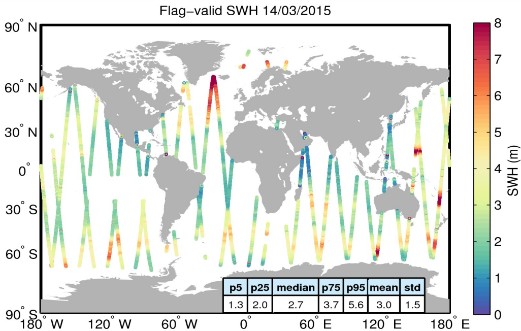
Figure 15. Geographical distribution of flag-valid SWH data over oceans and lakes for 14/03/2015. The statistical values shown in the table refer to the SWH in m and are calculated over all measurements shown in the figure.
