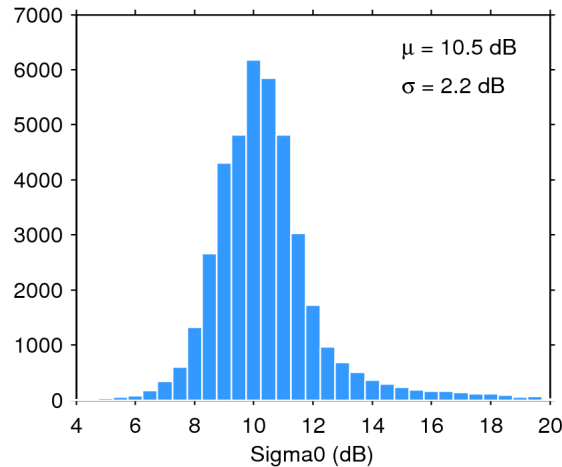
Figure 25. Histogram of flag-valid sigma0 over oceans and lakes for 14/03/2015. The mean ( \mu ) and standard deviation ( \sigma ) are also shown. Note that values outside [4 20] dB are excluded from the histogram for the sake of readability but not from the computation of \mu and \sigma .
