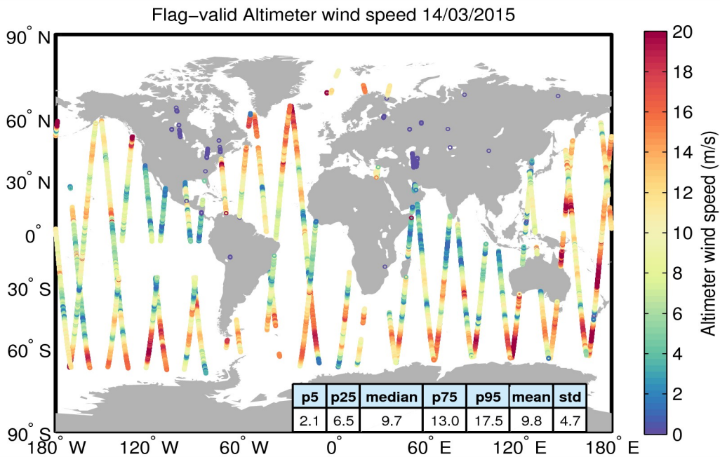
Figure 31. Geographical distribution of flag-valid wind data over oceans and lakes for 14/03/2015. The statistical values shown in the table refer to the wind in m/s and are calculated over all measurements shown in the figure.
