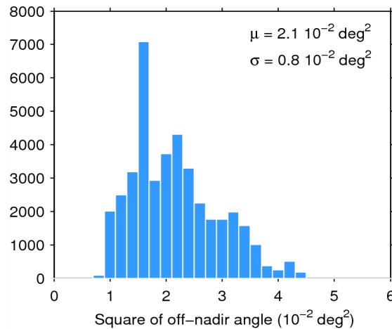
Figure 39. Histogram of flag-valid mispointing over oceans and lakes for 14/03/2015. The mean ( \mu ) and standard deviation ( \sigma ) are also shown. Note that values than 6 \cdot 10^{-2} \text{ deg}^2 are excluded from the histogram for the sake of readability but not from the computation of \mu and \sigma .
