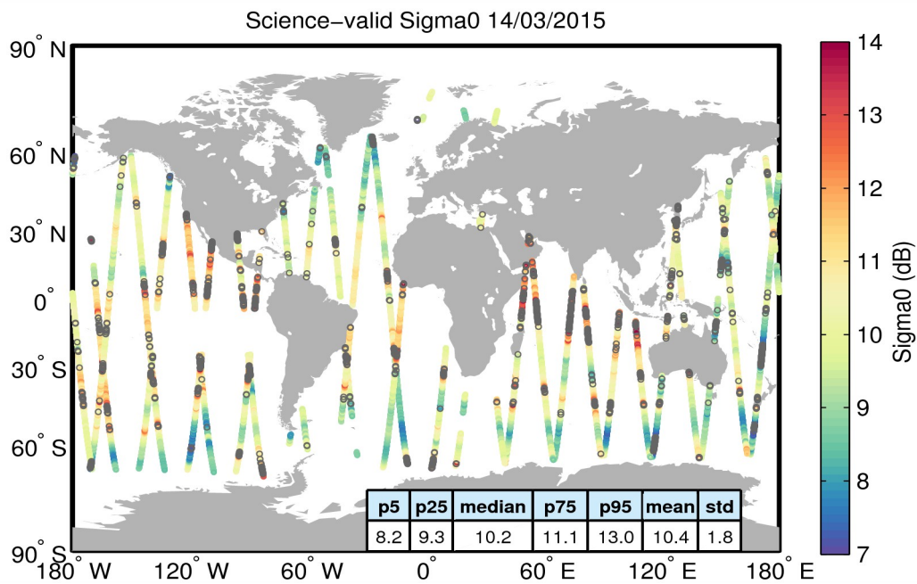
Figure 27. Geographical distribution of science-valid sigma0 data over oceans and lakes for 14/03/2015. The statistical values shown in the table refer to the sigma0 in dB and are calculated over all measurements shown in the figure. Gray circles denote records that have been rejected based on the editing criteria described in Table 4.
