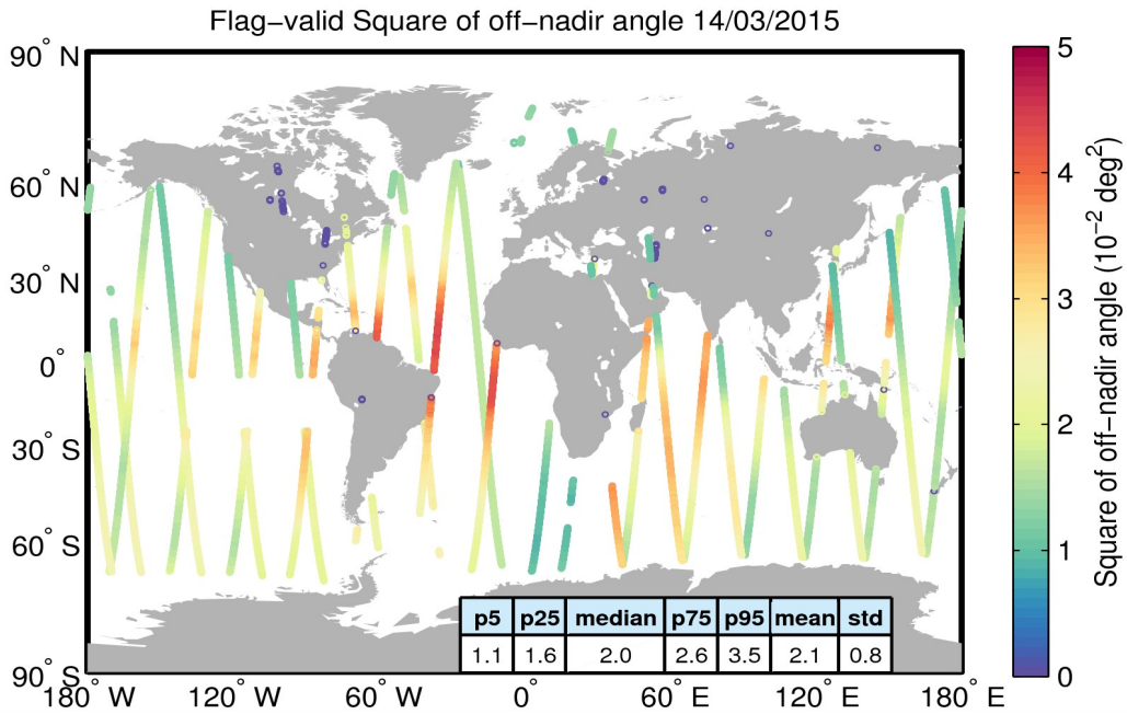
Figure 37. Geographical distribution of flag-valid mispointing data over oceans and lakes for 14/03/2015. The statistical values shown in the table refer to the mispointing in 10^{-2} deg 2 and are calculated over all measurements shown in the figure.
