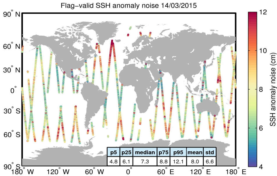
Figure 8. Geographical distribution of flag-valid 20-Hz SSH anomaly measurement noise over oceans and lakes for 14/03/2015. The statistical values shown in the table refer to the SSH anomaly noise and are calculated over all measurements shown in the figure.
