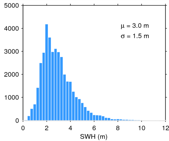
Figure 17. Histogram of flag-valid SWH over oceans and lakes for 14/03/2015. The mean ( \mu ) and standard deviation ( \sigma ) are also shown. Note that values larger than 12 m are excluded from the histogram for the sake of readability but not from the computation of \mu and \sigma .
