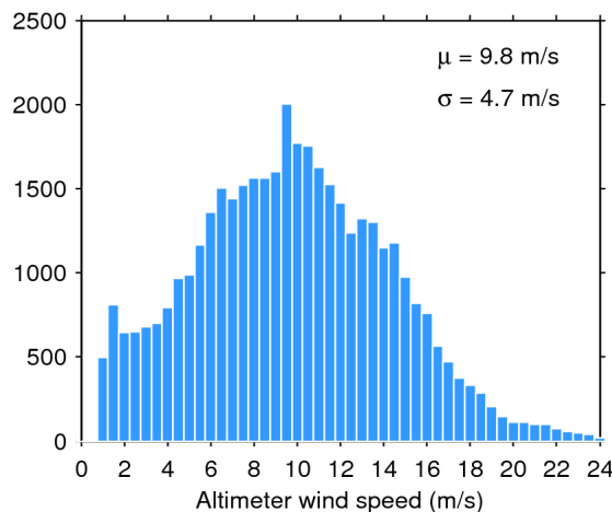
Figure 35. Histogram of science-valid wind over oceans and lakes for 14/03/2015. The mean ( \mu ) and standard deviation ( \sigma ) are also shown. Note that values larger than 24 m/s are excluded from the histogram for the sake of readability but not from the computation of \mu and \sigma .
