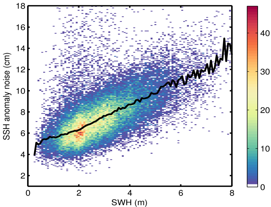
Figure 9. 2D histogram showing flag-valid SSH anomaly noise as a function of SWH for 14/03/2015. The black line denotes the median SSH anomaly as a function of SWH.
