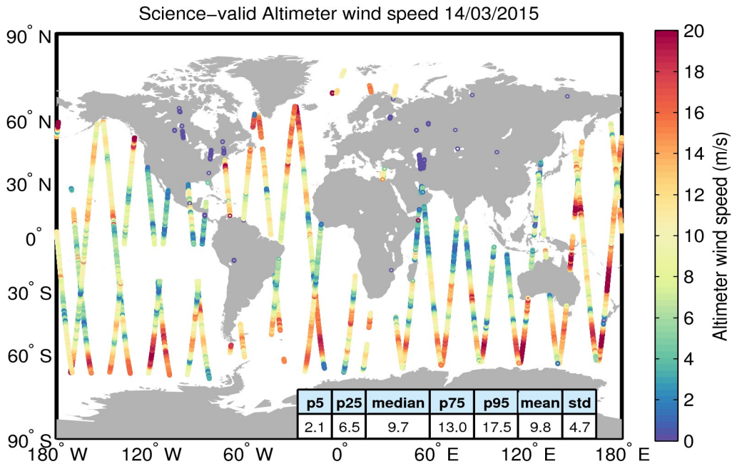
Figure 34. Geographical distribution of science-valid wind data over oceans and lakes for 14/03/2015. The statistical values shown in the table refer to the wind in m/s and are calculated over all measurements shown in the figure. Gray circles denote records that have been rejected based on the editing criteria described in Table 5.
