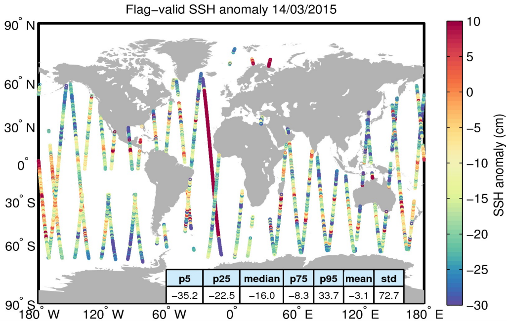
Figure 5. Geographical distribution of flag-valid 1-Hz SSH anomaly data over oceans and lakes for 14/03/2015. The statistical values shown in the table refer to the SSH anomaly in cm and are calculated over all measurements shown in the figure.
