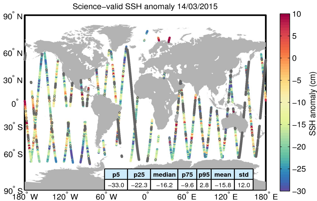
Figure 10. Geographical distribution of science-valid SSH anomaly data over oceans and lakes for 14/03/2015. The statistical values shown in the table refer to the SSH anomaly in cm and are calculated over all measurements shown in the figure. Gray circles denote records that have been rejected based on the editing criteria described in Table 2.
