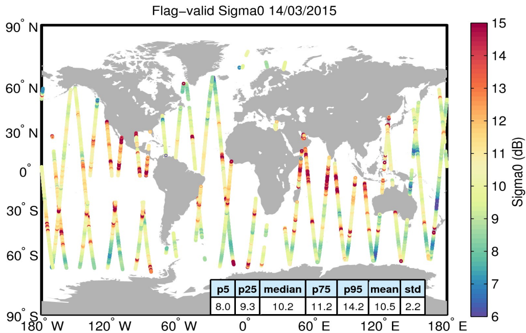
Figure 23. Geographical distribution of flag-valid sigma0 data over oceans and lakes for 14/03/2015. The statistical values shown in the table refer to the sigma0 in dB and are calculated over all measurements shown in the figure.
