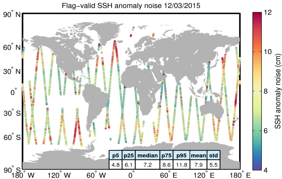
Figure 8. Geographical distribution of flag-valid 20-Hz SSH anomaly measurement noise over oceans and lakes for 12/03/2015. The statistical values shown in the table refer to the SSH anomaly noise and are calculated over all measurements shown in the figure.
