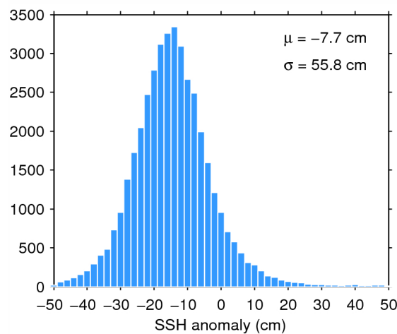
Figure 7. Histogram of flag-valid SSH anomaly over oceans and lakes for 12/03/2015. The mean ( \mu ) and standard deviation ( \sigma ) are also shown. Note that values outside [-50 50] cm are excluded from the histogram for the sake of readability but not from the computation of \mu and \sigma .
