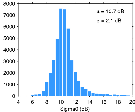
Figure 25. Histogram of flag-valid sigma0 over oceans and lakes for 12/03/2015. The mean ( \mu ) and standard deviation ( \sigma ) are also shown. Note that values outside [4 20] dB are excluded from the histogram for the sake of readability but not from the computation of \mu and \sigma .
