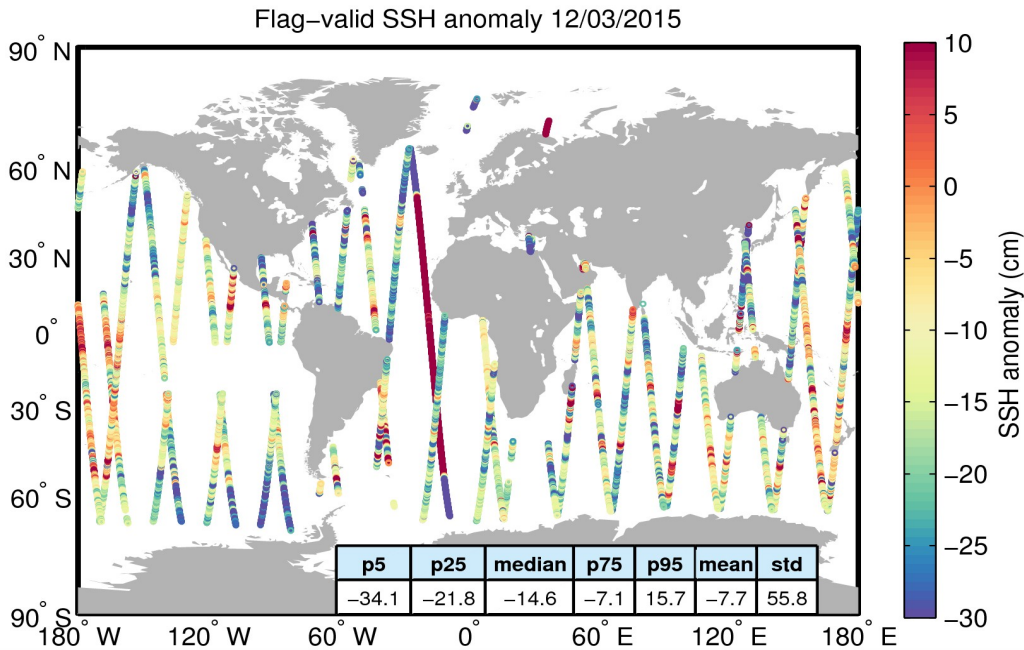
Figure 5. Geographical distribution of flag-valid 1-Hz SSH anomaly data over oceans and lakes for 12/03/2015. The statistical values shown in the table refer to the SSH anomaly in cm and are calculated over all measurements shown in the figure.
