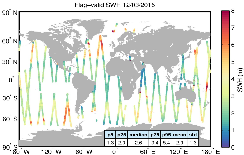
Figure 15. Geographical distribution of flag-valid SWH data over oceans and lakes for 12/03/2015. The statistical values shown in the table refer to the SWH in m and are calculated over all measurements shown in the figure.
