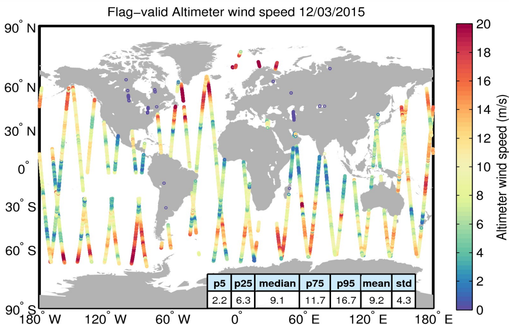
Figure 31. Geographical distribution of flag-valid wind data over oceans and lakes for 12/03/2015. The statistical values shown in the table refer to the wind in m/s and are calculated over all measurements shown in the figure.
