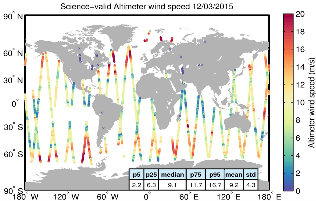
Figure 34. Geographical distribution of science-valid wind data over oceans and lakes for 12/03/2015. The statistical values shown in the table refer to the wind in m/s and are calculated over all measurements shown in the figure. Gray circles denote records that have been rejected based on the editing criteria described in Table 5.
