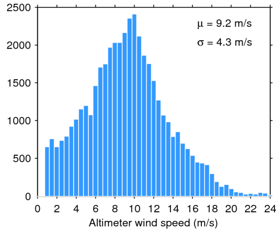
Figure 33. Histogram of flag-valid wind over oceans and lakes for 12/03/2015. The mean ( \mu ) and standard deviation ( \sigma ) are also shown. Note that values larger than 24 m/s are excluded from the histogram for the sake of readability but not from the computation of \mu and \sigma .
