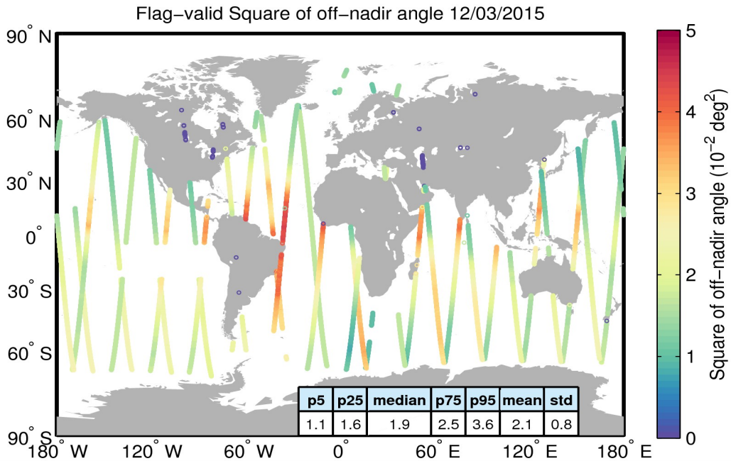
Figure 37. Geographical distribution of flag-valid mispointing data over oceans and lakes for 12/03/2015. The statistical values shown in the table refer to the mispointing in 10^{-2} \text{ deg}^2 and are calculated over all measurements shown in the figure.
