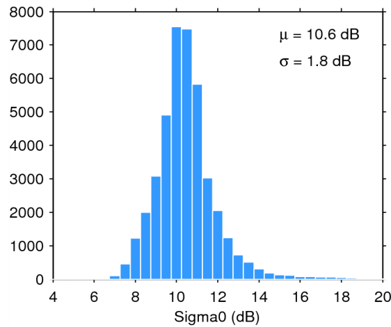
Figure 28. Histogram of science-valid sigma0 over oceans and lakes for 12/03/2015. The mean ( \mu ) and standard deviation ( \sigma ) are also shown. Note that values outside [4 20] dB are excluded from the histogram for the sake of readability but not from the computation of \mu and \sigma .
