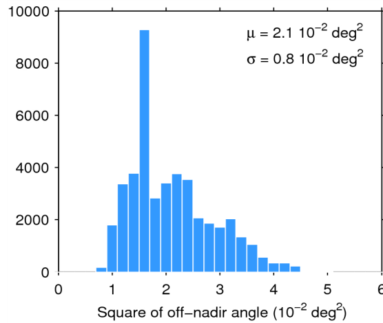
Figure 39. Histogram of flag-valid mispointing over oceans and lakes for 12/03/2015. The mean ( \mu ) and standard deviation ( \sigma ) are also shown. Note that values than 6 \cdot 10^{-2} \text{ deg}^2 are excluded from the histogram for the sake of readability but not from the computation of \mu and \sigma .
