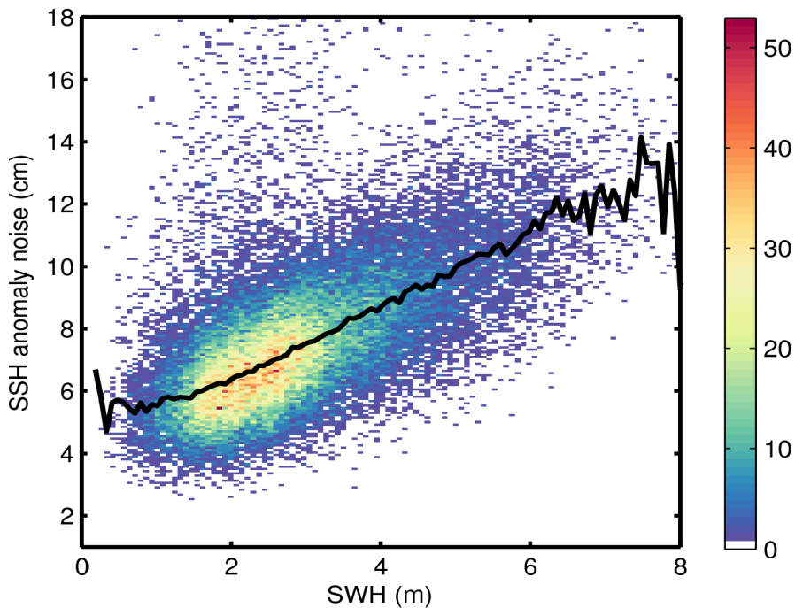
Figure 9. 2D histogram showing flag-valid SSH anomaly noise as a function of SWH for 12/03/2015. The black line denotes the median SSH anomaly as a function of SWH.
