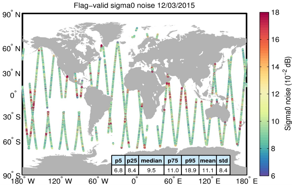
Figure 26. Geographical distribution of flag-valid 20-Hz sigma0 measurement noise over oceans and lakes for 12/03/2015. The statistical values shown in the figure refer to the sigma0 noise and are calculated over all measurements shown in the figure.
