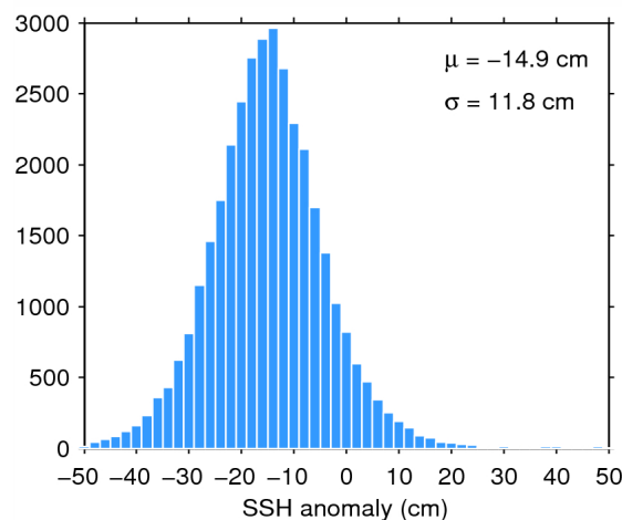
Figure 11. Histogram of science-valid SSH anomaly over oceans and lakes for 12/03/2015. The mean ( \mu ) and standard deviation ( \sigma ) are also shown. Note that values outside [-50 50] cm are excluded from the histogram for the sake of readability but not from the computation of \mu and \sigma .
