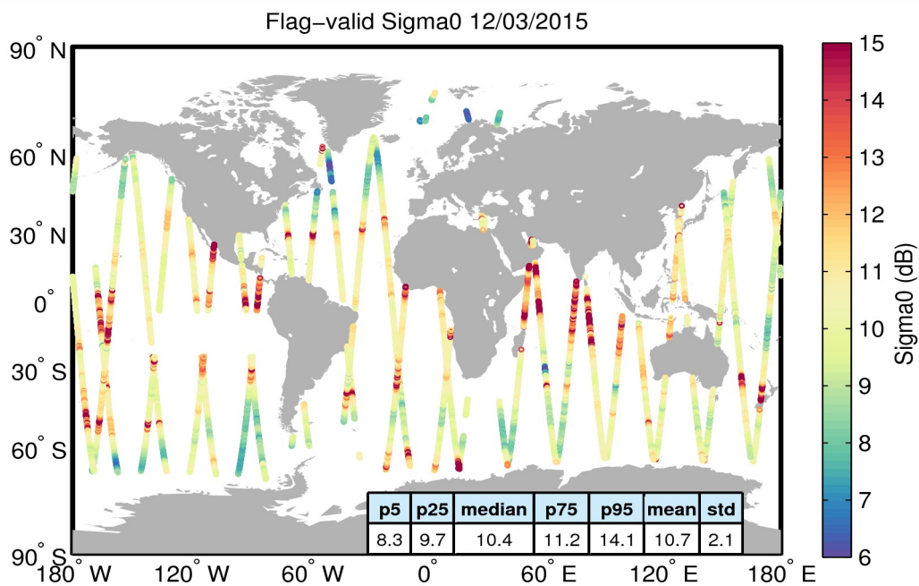
Figure 23. Geographical distribution of flag-valid sigma0 data over oceans and lakes for 12/03/2015. The statistical values shown in the table refer to the sigma0 in dB and are calculated over all measurements shown in the figure.
