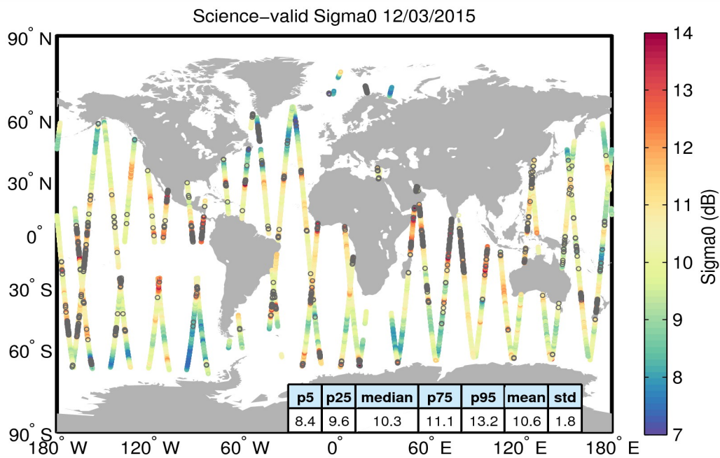
Figure 27. Geographical distribution of science-valid sigma0 data over oceans and lakes for 12/03/2015. The statistical values shown in the table refer to the sigma0 in dB and are calculated over all measurements shown in the figure. Gray circles denote records that have been rejected based on the editing criteria described in Table 4.
