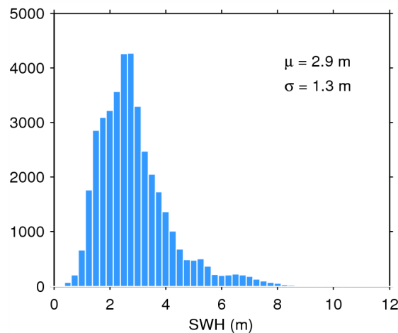
Figure 20. Histogram of science-valid SWH over oceans and lakes for 11/03/2015. The mean ( \mu ) and standard deviation ( \sigma ) are also shown. Note that values larger than 12 m are excluded from the histogram for the sake of readability but not from the computation of \mu and \sigma .
