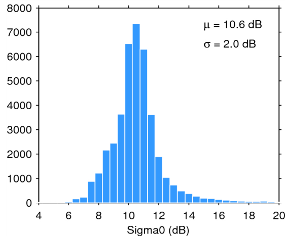
Figure 25. Histogram of flag-valid sigma0 over oceans and lakes for 11/03/2015. The mean ( \mu ) and standard deviation ( \sigma ) are also shown. Note that values outside [4 20] dB are excluded from the histogram for the sake of readability but not from the computation of \mu and \sigma .
