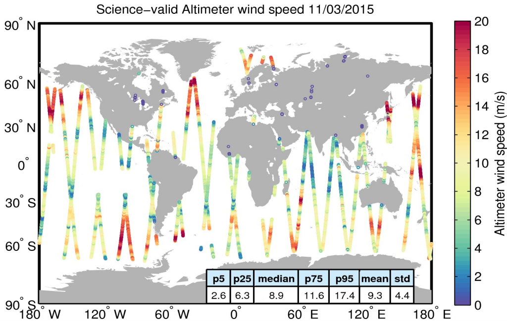
Figure 34. Geographical distribution of science-valid wind data over oceans and lakes for 11/03/2015. The statistical values shown in the table refer to the wind in m/s and are calculated over all measurements shown in the figure. Gray circles denote records that have been rejected based on the editing criteria described in Table 5.
