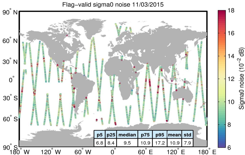
Figure 26. Geographical distribution of flag-valid 20-Hz sigma0 measurement noise over oceans and lakes for 11/03/2015. The statistical values shown in the table refer to the sigma0 noise and are calculated over all measurements shown in the figure.
