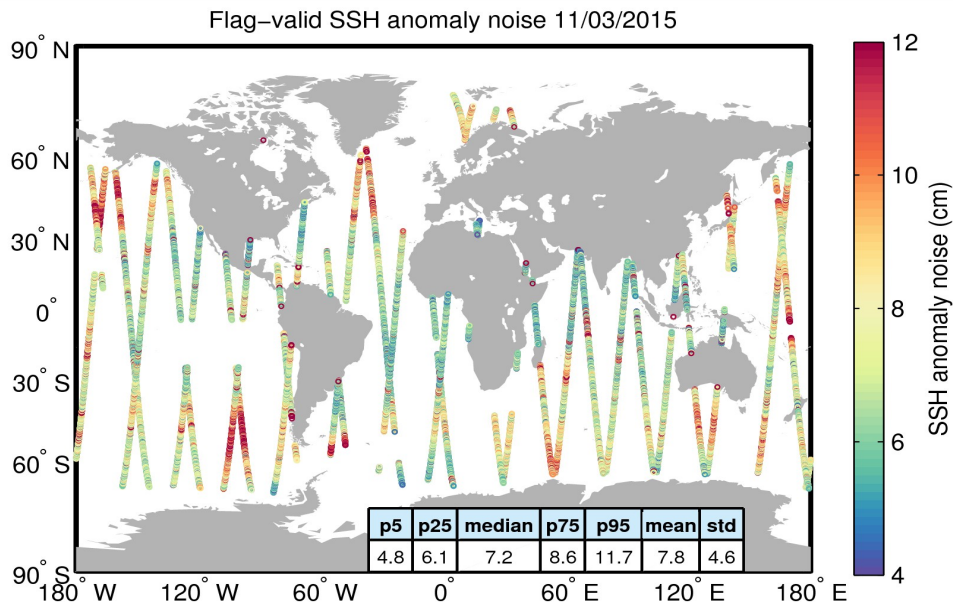
Figure 8. Geographical distribution of flag-valid 20-Hz SSH anomaly measurement noise over oceans and lakes for 11/03/2015. The statistical values shown in the table refer to the SSH anomaly noise and are calculated over all measurements shown in the figure.
