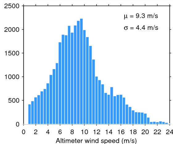
Figure 35. Histogram of science-valid wind over oceans and lakes for 11/03/2015. The mean ( \mu ) and standard deviation ( \sigma ) are also shown. Note that values larger than 24 m/s are excluded from the histogram for the sake of readability but not from the computation of \mu and \sigma .
