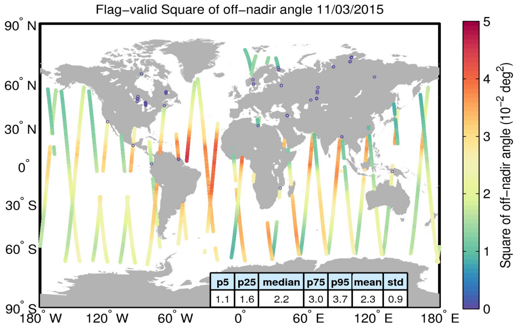
Figure 37. Geographical distribution of flag-valid mispointing data over oceans and lakes for 11/03/2015. The statistical values shown in the table refer to the mispointing in 10^{-2} \text{deg}^2 and are calculated over all measurements shown in the figure.
