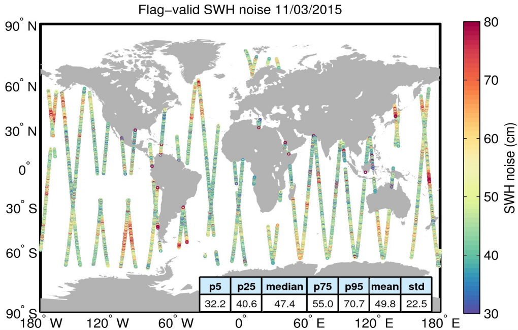
Figure 18. Geographical distribution of flag-valid 20-Hz SWH measurement noise over oceans and lakes for 11/03/2015. The statistical values shown in the figure refer to the SWH noise and are calculated over all measurements shown in the figure.
