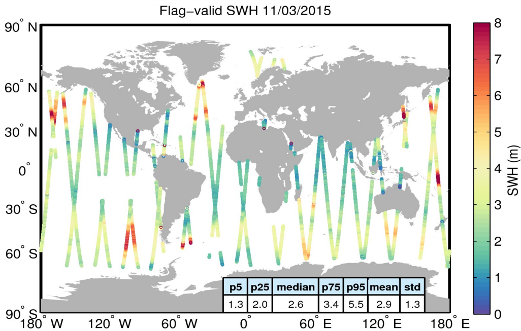
Figure 15. Geographical distribution of flag-valid SWH data over oceans and lakes for 11/03/2015. The statistical values shown in the table refer to the SWH in m and are calculated over all measurements shown in the figure.
