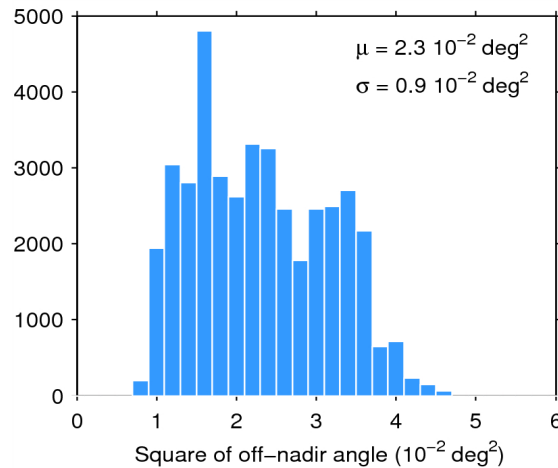
Figure 39. Histogram of flag-valid mispointing over oceans and lakes for 11/03/2015. The mean ( \mu ) and standard deviation ( \sigma ) are also shown. Note that values than 6 \cdot 10^{-2} \text{ deg}^2 are excluded from the histogram for the sake of readability but not from the computation of \mu and \sigma .
