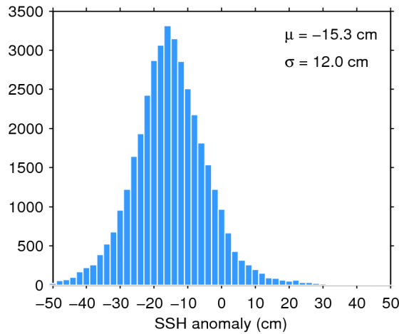
Figure 11. Histogram of science-valid SSH anomaly over oceans and lakes for 11/03/2015. The mean ( \mu ) and standard deviation ( \sigma ) are also shown. Note that values outside [-50 50] cm are excluded from the histogram for the sake of readability but not from the computation of \mu and \sigma .
