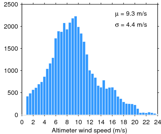
Figure 33. Histogram of flag-valid wind over oceans and lakes for 11/03/2015. The mean ( \mu ) and standard deviation ( \sigma ) are also shown. Note that values larger than 24 m/s are excluded from the histogram for the sake of readability but not from the computation of \mu and \sigma .
