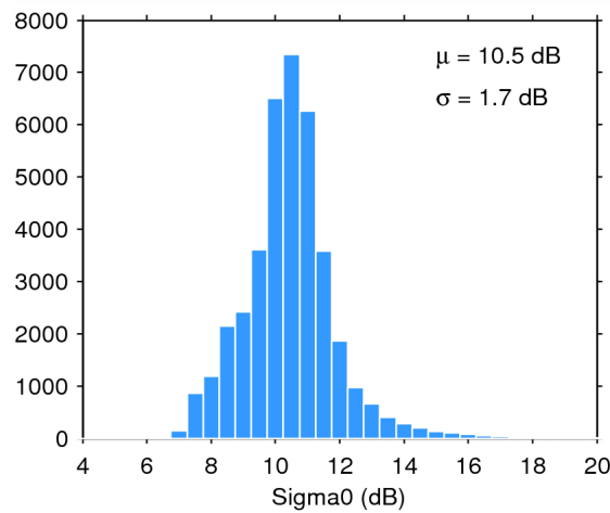
Figure 28. Histogram of science-valid sigma0 over oceans and lakes for 11/03/2015. The mean ( \mu ) and standard deviation ( \sigma ) are also shown. Note that values outside [4 20] dB are excluded from the histogram for the sake of readability but not from the computation of \mu and \sigma .
