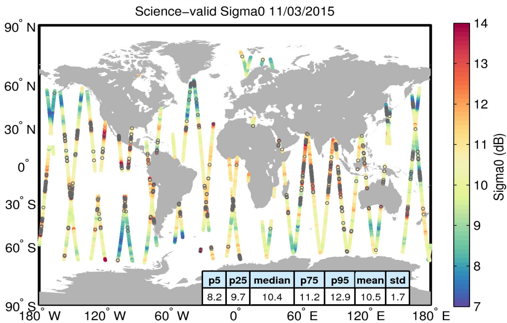
Figure 27. Geographical distribution of science-valid sigma0 data over oceans and lakes for 11/03/2015. The statistical values shown in the table refer to the sigma0 in dB and are calculated over all measurements shown in the figure. Gray circles denote records that have been rejected based on the editing criteria described in Table 4.
