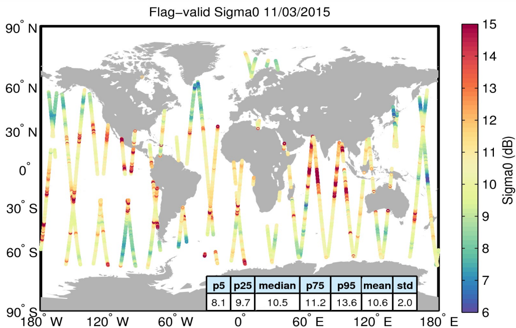
Figure 23. Geographical distribution of flag-valid sigma0 data over oceans and lakes for 11/03/2015. The statistical values shown in the table refer to the sigma0 in dB and are calculated over all measurements shown in the figure.
