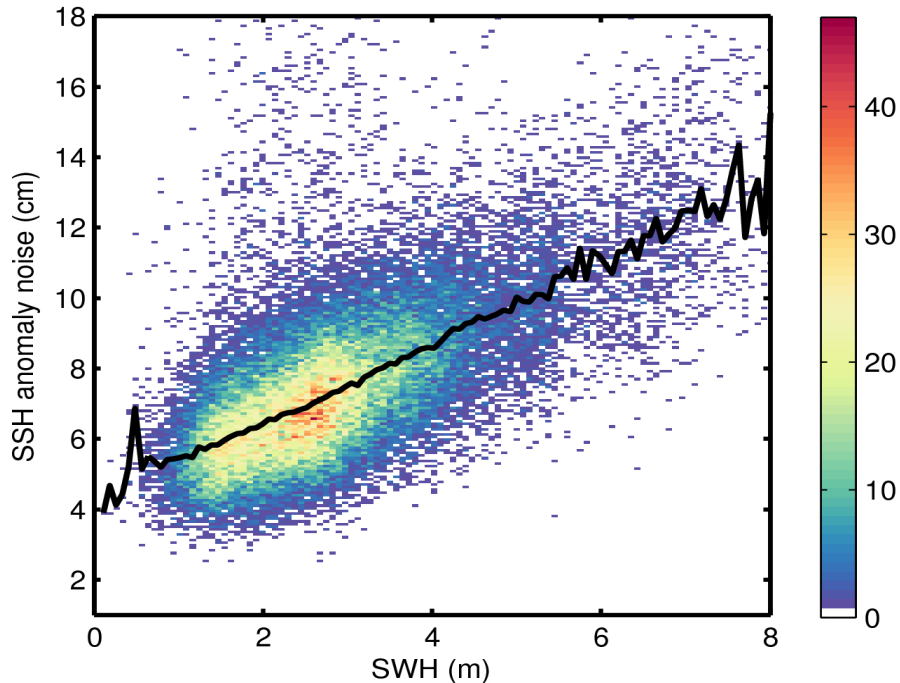
Figure 9. 2D histogram showing flag-valid SSH anomaly noise as a function of SWH for 11/03/2015. The black line denotes the median SSH anomaly as a function of SWH.
