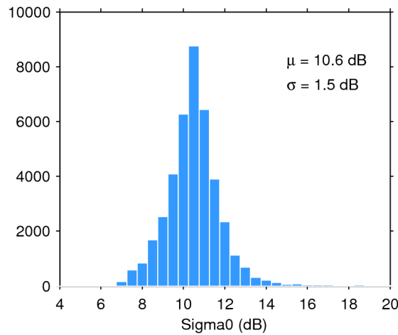
Figure 28. Histogram of science-valid sigma0 over oceans and lakes for 10/03/2015. The mean ( \mu ) and standard deviation ( \sigma ) are also shown. Note that values outside [4 20] dB are excluded from the histogram for the sake of readability but not from the computation of \mu and \sigma .
