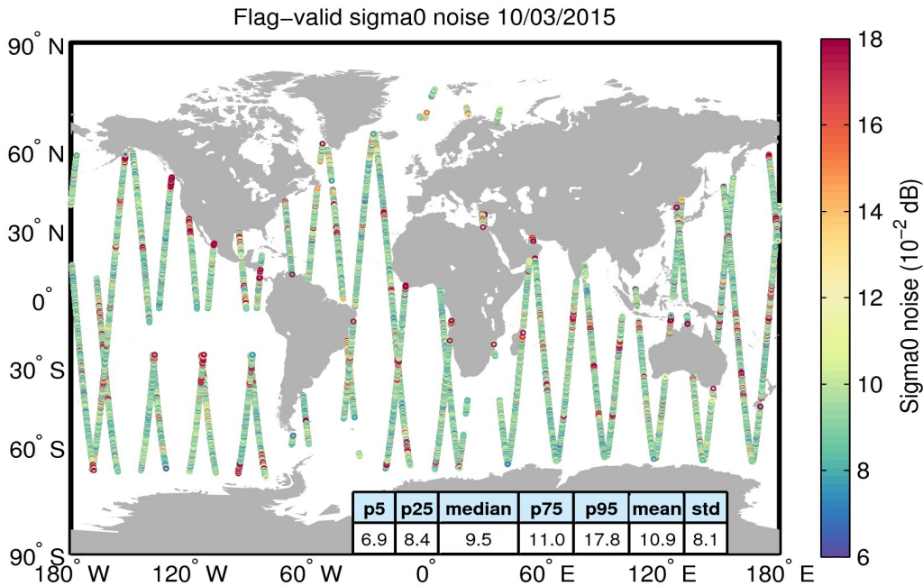
Figure 26. Geographical distribution of flag-valid 20-Hz sigma0 measurement noise over oceans and lakes for 10/03/2015. The statistical values shown in the table refer to the sigma0 noise and are calculated over all measurements shown in the figure.
