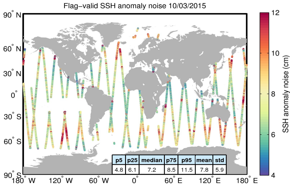
Figure 8. Geographical distribution of flag-valid 20-Hz SSH anomaly measurement noise over oceans and lakes for 10/03/2015. The statistical values shown in the table refer to the SSH anomaly noise and are calculated over all measurements shown in the figure.
