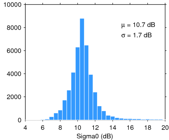
Figure 25. Histogram of flag-valid sigma0 over oceans and lakes for 10/03/2015. The mean ( \mu ) and standard deviation ( \sigma ) are also shown. Note that values outside [4 20] dB are excluded from the histogram for the sake of readability but not from the computation of \mu and \sigma .
