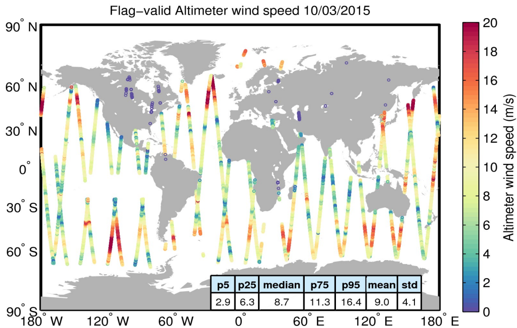
Figure 31. Geographical distribution of flag-valid wind data over oceans and lakes for 10/03/2015. The statistical values shown in the table refer to the wind in m/s and are calculated over all measurements shown in the figure.
