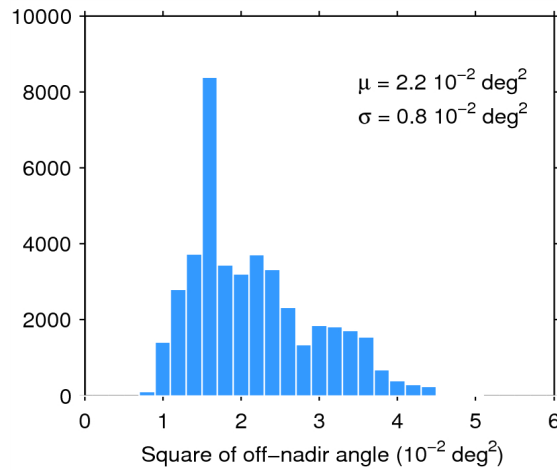
Figure 39. Histogram of flag-valid mispointing over oceans and lakes for 10/03/2015. The mean ( \mu ) and standard deviation ( \sigma ) are also shown. Note that values than 6 \cdot 10^{-2} \text{ deg}^2 are excluded from the histogram for the sake of readability but not from the computation of \mu and \sigma .
