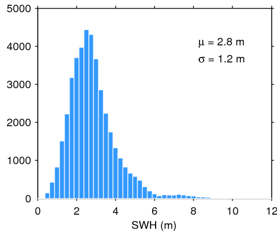
Figure 20. Histogram of science-valid SWH over oceans and lakes for 10/03/2015. The mean ( \mu ) and standard deviation ( \sigma ) are also shown. Note that values larger than 12 m are excluded from the histogram for the sake of readability but not from the computation of \mu and \sigma .
