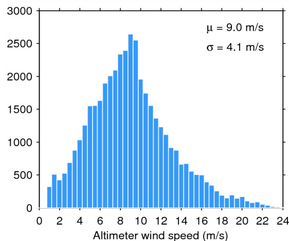
Figure 35. Histogram of science-valid wind over oceans and lakes for 10/03/2015. The mean ( \mu ) and standard deviation ( \sigma ) are also shown. Note that values larger than 24 m/s are excluded from the histogram for the sake of readability but not from the computation of \mu and \sigma .
