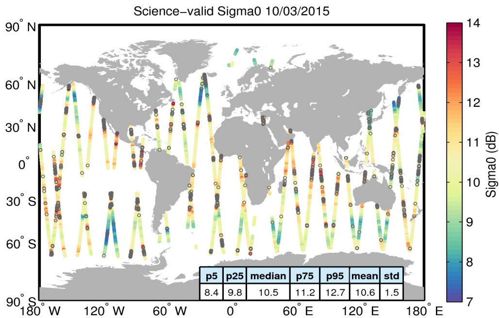
Figure 27. Geographical distribution of science-valid sigma0 data over oceans and lakes for 10/03/2015. The statistical values shown in the table refer to the sigma0 in dB and are calculated over all measurements shown in the figure. Gray circles denote records that have been rejected based on the editing criteria described in Table 4.
