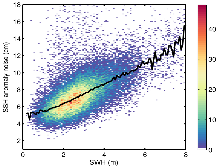
Figure 9. 2D histogram showing flag-valid SSH anomaly noise as a function of SWH for 10/03/2015. The black line denotes the median SSH anomaly as a function of SWH.
