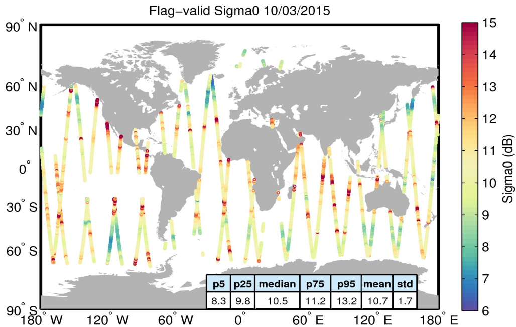
Figure 23. Geographical distribution of flag-valid sigma0 data over oceans and lakes for 10/03/2015. The statistical values shown in the table refer to the sigma0 in dB and are calculated over all measurements shown in the figure.
