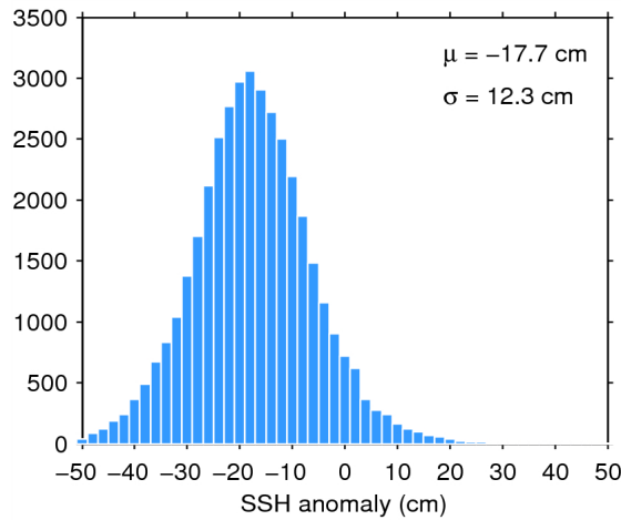
Figure 11. Histogram of science-valid SSH anomaly over oceans and lakes for 09/03/2015. The mean ( \mu ) and standard deviation ( \sigma ) are also shown. Note that values outside [-50 50] cm are excluded from the histogram for the sake of readability but not from the computation of \mu and \sigma .
