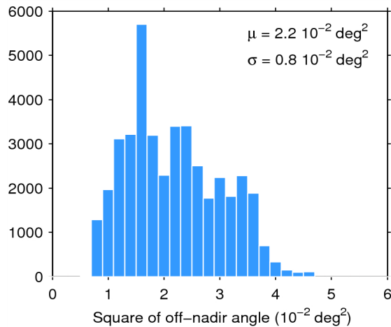
Figure 39. Histogram of flag-valid mispointing over oceans and lakes for 09/03/2015. The mean ( \mu ) and standard deviation ( \sigma ) are also shown. Note that values than 6 \cdot 10^{-2} \text{ deg}^2 are excluded from the histogram for the sake of readability but not from the computation of \mu and \sigma .
