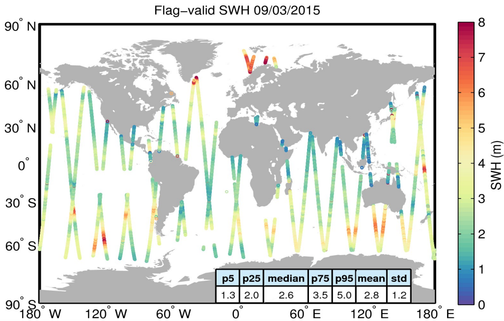
Figure 15. Geographical distribution of flag-valid SWH data over oceans and lakes for 09/03/2015. The statistical values shown in the table refer to the SWH in m and are calculated over all measurements shown in the figure.
