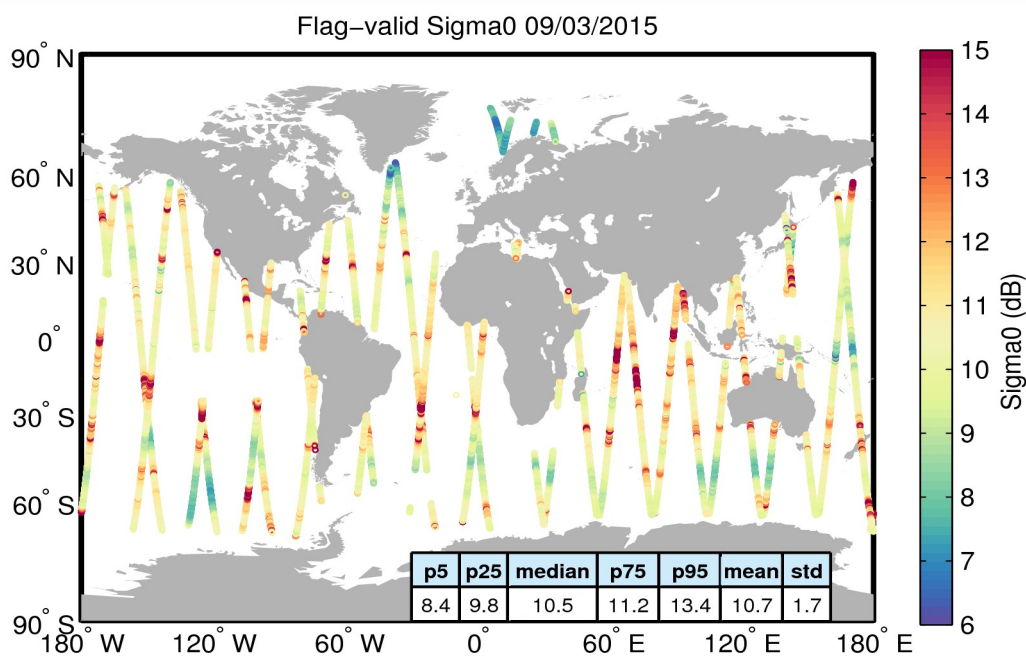
Figure 23. Geographical distribution of flag-valid sigma0 data over oceans and lakes for 09/03/2015. The statistical values shown in the table refer to the sigma0 in dB and are calculated over all measurements shown in the figure.
