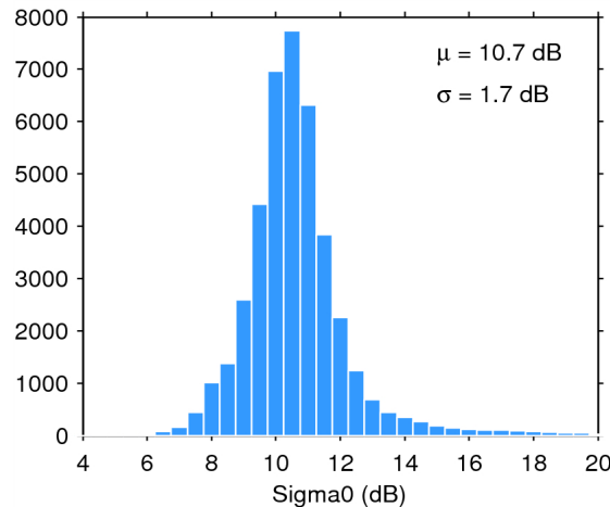
Figure 25. Histogram of flag-valid sigma0 over oceans and lakes for 09/03/2015. The mean ( \mu ) and standard deviation ( \sigma ) are also shown. Note that values outside [4 20] dB are excluded from the histogram for the sake of readability but not from the computation of \mu and \sigma .
