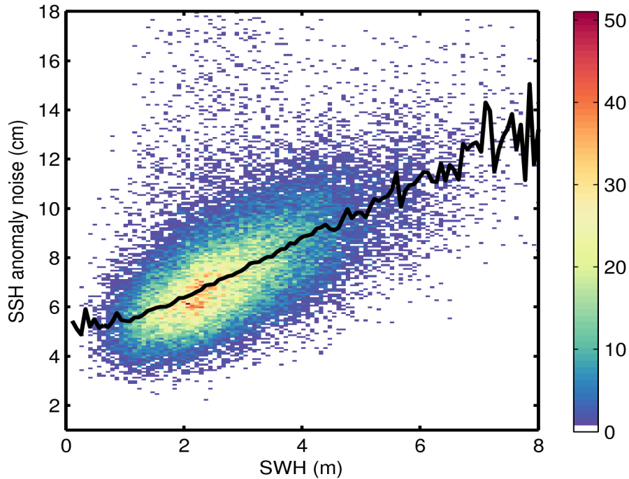
Figure 9. 2D histogram showing flag-valid SSH anomaly noise as a function of SWH for 09/03/2015. The black line denotes the median SSH anomaly as a function of SWH.
