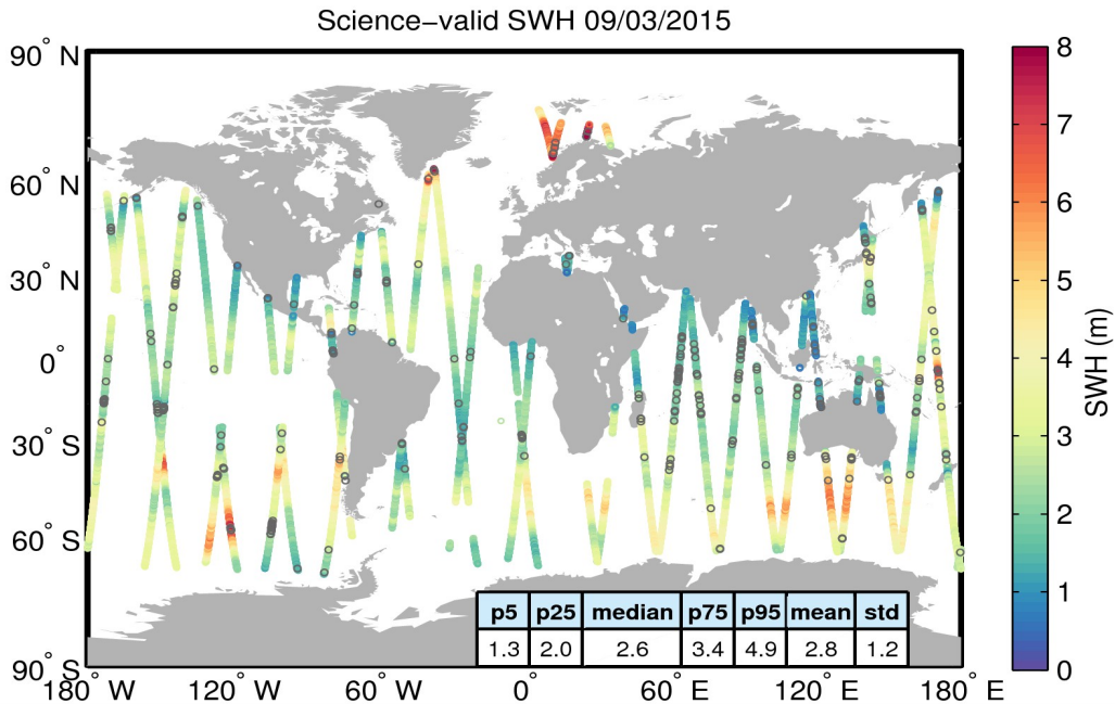
Figure 19. Geographical distribution of science-valid SWH data over oceans and lakes for 09/03/2015. The statistical values shown in the table refer to the SWH in m and are calculated over all measurements shown in the figure. Gray circles denote records that have been rejected based on the editing criteria described in Table 3.
