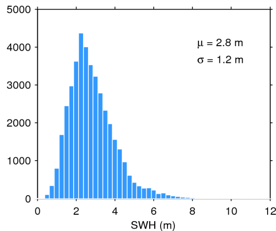
Figure 20. Histogram of science-valid SWH over oceans and lakes for 09/03/2015. The mean ( \mu ) and standard deviation ( \sigma ) are also shown. Note that values larger than 12 m are excluded from the histogram for the sake of readability but not from the computation of \mu and \sigma .
