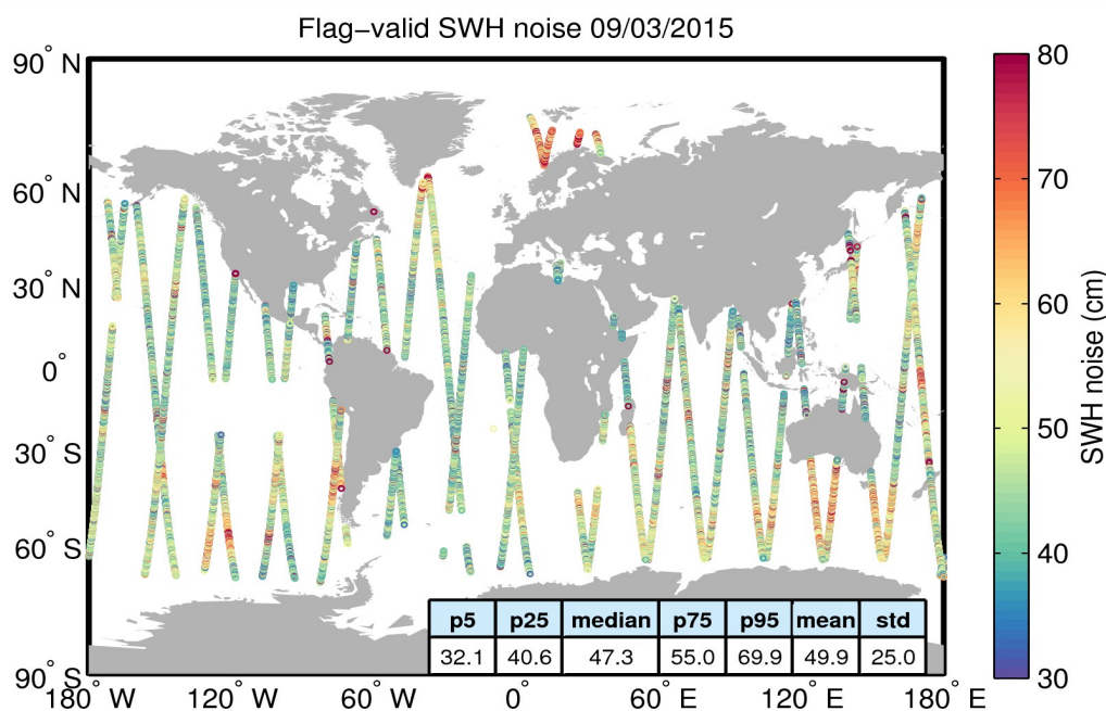
Figure 18. Geographical distribution of flag-valid 20-Hz SWH measurement noise over oceans and lakes for 09/03/2015. The statistical values shown in the figure refer to the SWH noise and are calculated over all measurements shown in the figure.
