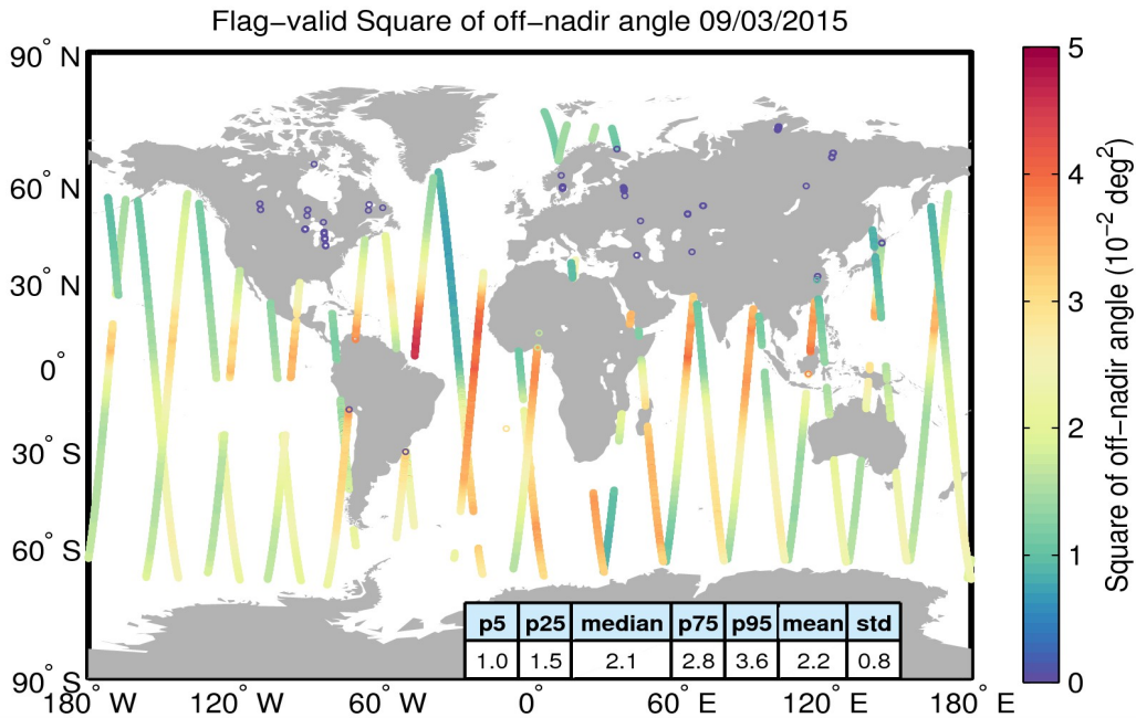
Figure 37. Geographical distribution of flag-valid mispointing data over oceans and lakes for 09/03/2015. The statistical values shown in the table refer to the mispointing in 10^{-2} \text{deg}^2 and are calculated over all measurements shown in the figure.
