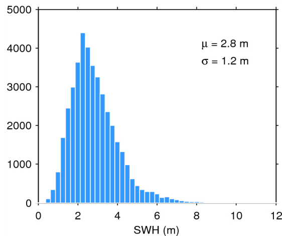
Figure 17. Histogram of flag-valid SWH over oceans and lakes for 09/03/2015. The mean ( \mu ) and standard deviation ( \sigma ) are also shown. Note that values larger than 12 m are excluded from the histogram for the sake of readability but not from the computation of \mu and \sigma .
