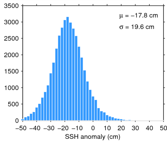
Figure 7. Histogram of flag-valid SSH anomaly over oceans and lakes for 09/03/2015. The mean ( \mu ) and standard deviation ( \sigma ) are also shown. Note that values outside [-50\ 50] cm are excluded from the histogram for the sake of readability but not from the computation of \mu and \sigma .
