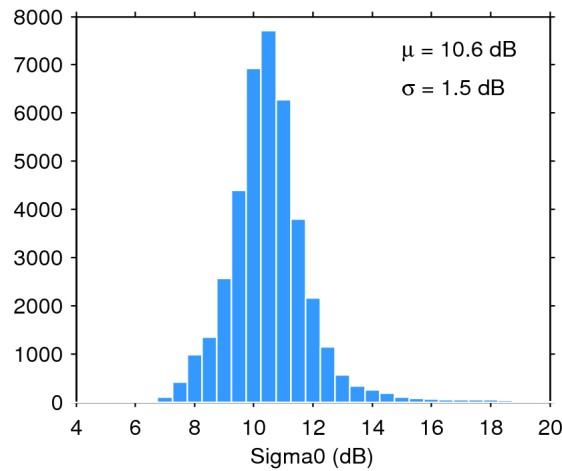
Figure 28. Histogram of science-valid sigma0 over oceans and lakes for 09/03/2015. The mean ( \mu ) and standard deviation ( \sigma ) are also shown. Note that values outside [4 20] dB are excluded from the histogram for the sake of readability but not from the computation of \mu and \sigma .
