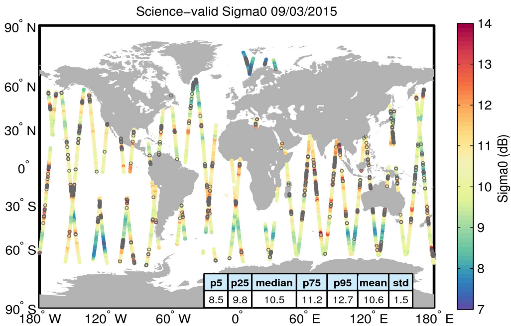
Figure 27. Geographical distribution of science-valid sigma0 data over oceans and lakes for 09/03/2015. The statistical values shown in the table refer to the sigma0 in dB and are calculated over all measurements shown in the figure. Gray circles denote records that have been rejected based on the editing criteria described in Table 4.
