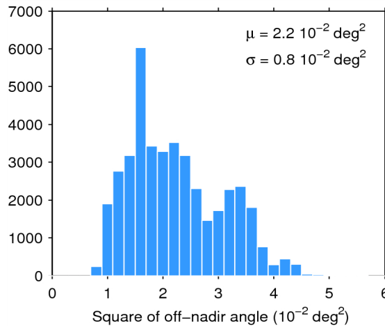
Figure 39. Histogram of flag-valid mispointing over oceans and lakes for 08/03/2015. The mean ( \mu ) and standard deviation ( \sigma ) are also shown. Note that values than 6 \cdot 10^{-2} \text{ deg}^2 are excluded from the histogram for the sake of readability but not from the computation of \mu and \sigma .
