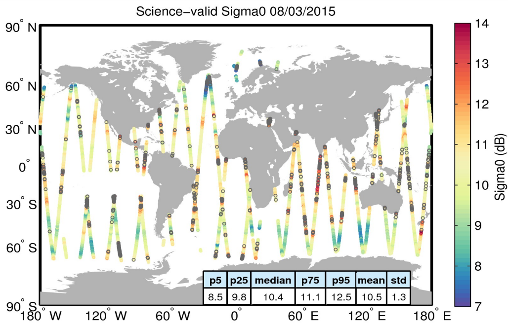
Figure 27. Geographical distribution of science-valid sigma0 data over oceans and lakes for 08/03/2015. The statistical values shown in the table refer to the sigma0 in dB and are calculated over all measurements shown in the figure. Gray circles denote records that have been rejected based on the editing criteria described in Table 4.
