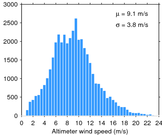
Figure 33. Histogram of flag-valid wind over oceans and lakes for 08/03/2015. The mean ( \mu ) and standard deviation ( \sigma ) are also shown. Note that values larger than 24 m/s are excluded from the histogram for the sake of readability but not from the computation of \mu and \sigma .
