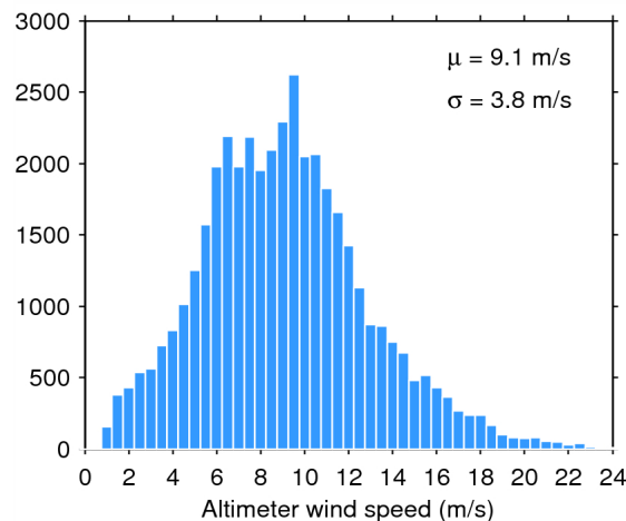
Figure 35. Histogram of science-valid wind over oceans and lakes for 08/03/2015. The mean ( \mu ) and standard deviation ( \sigma ) are also shown. Note that values larger than 24 m/s are excluded from the histogram for the sake of readability but not from the computation of \mu and \sigma .
