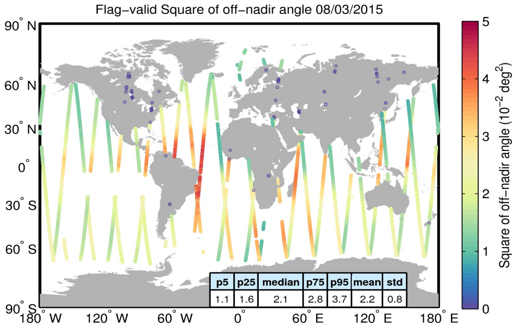
Figure 37. Geographical distribution of flag-valid mispointing data over oceans and lakes for 08/03/2015. The statistical values shown in the table refer to the mispointing in 10^{-2} \text{ deg}^2 and are calculated over all measurements shown in the figure.
