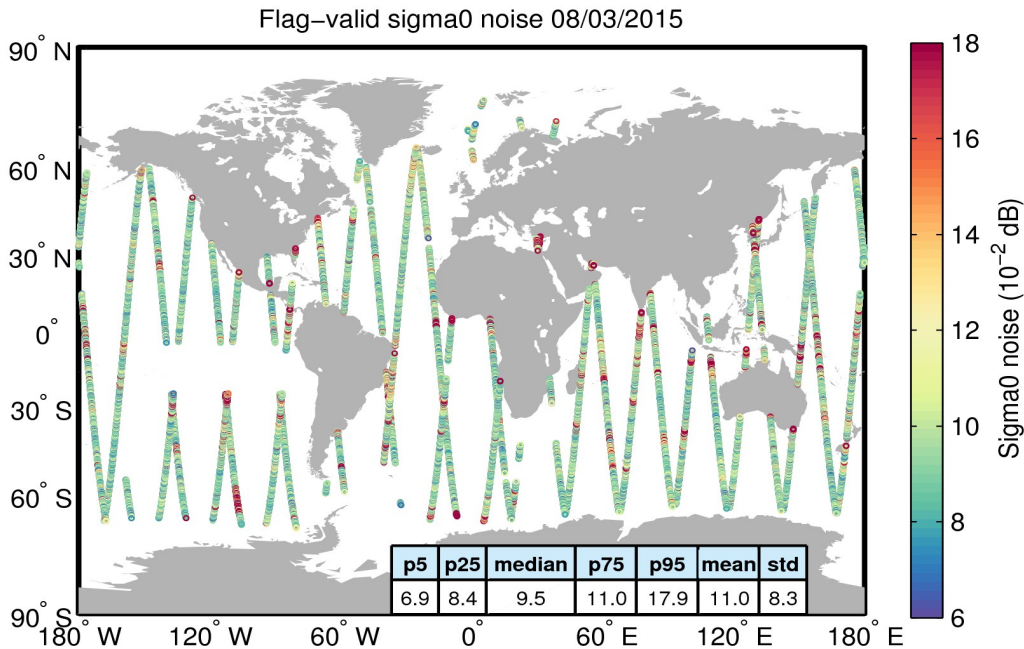
Figure 26. Geographical distribution of flag-valid 20-Hz sigma0 measurement noise over oceans and lakes for 08/03/2015. The statistical values shown in the table refer to the sigma0 noise and are calculated over all measurements shown in the figure.
