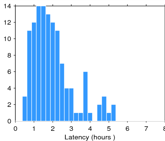
Figure 2. Histogram of the data latency for 08/03/2015. The y-axis denotes the number of files that are made available with a delay of x-hours with respect to the mean time of the records stored in the file.
