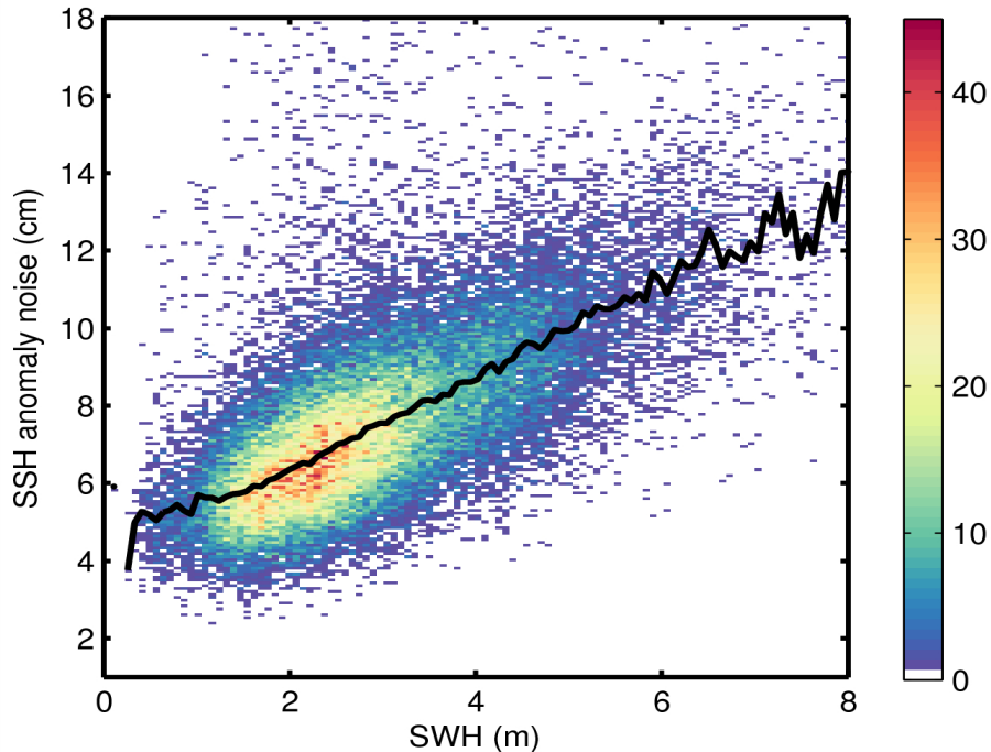
Figure 9. 2D histogram showing flag-valid SSH anomaly noise as a function of SWH for 08/03/2015. The black line denotes the median SSH anomaly as a function of SWH.
