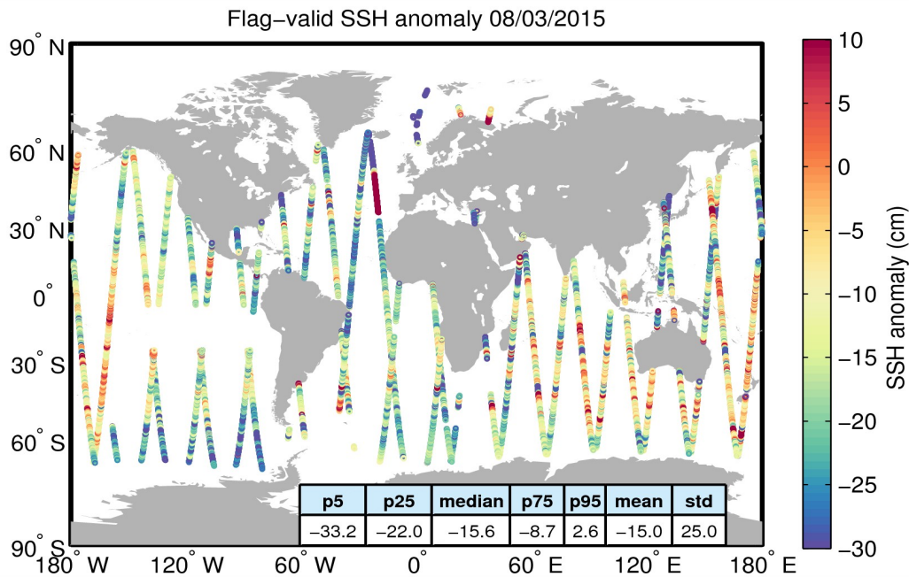
Figure 5. Geographical distribution of flag-valid 1-Hz SSH anomaly data over oceans and lakes for 08/03/2015. The statistical values shown in the table refer to the SSH anomaly in cm and are calculated over all measurements shown in the figure.
