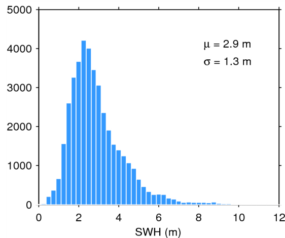
Figure 20. Histogram of science-valid SWH over oceans and lakes for 08/03/2015. The mean ( \mu ) and standard deviation ( \sigma ) are also shown. Note that values larger than 12 m are excluded from the histogram for the sake of readability but not from the computation of \mu and \sigma .
