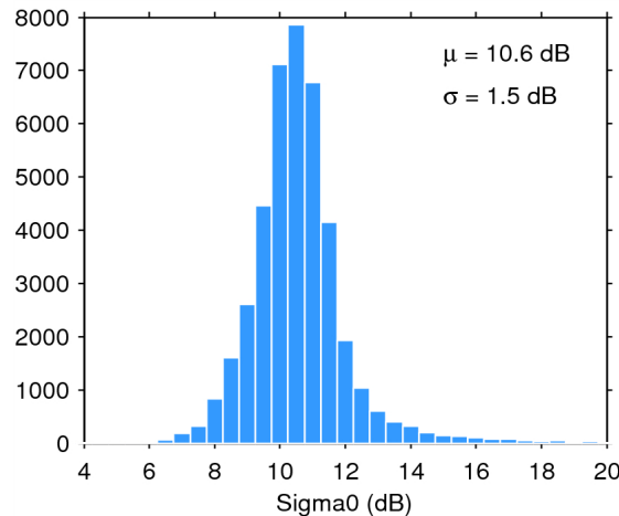
Figure 25. Histogram of flag-valid sigma0 over oceans and lakes for 08/03/2015. The mean ( \mu ) and standard deviation ( \sigma ) are also shown. Note that values outside [4 20] dB are excluded from the histogram for the sake of readability but not from the computation of \mu and \sigma .
