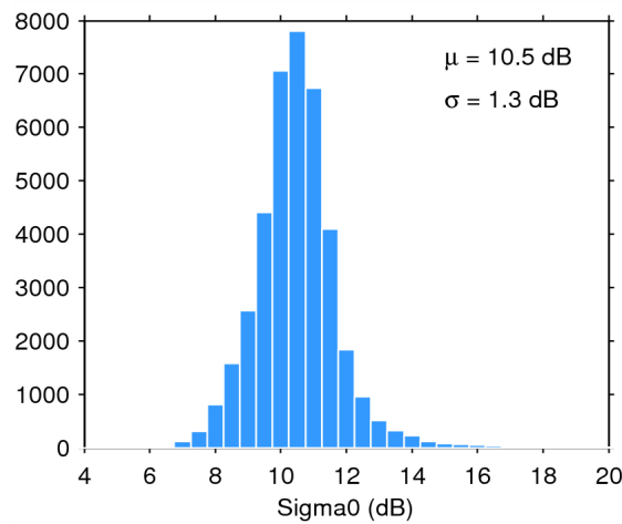
Figure 28. Histogram of science-valid sigma0 over oceans and lakes for 08/03/2015. The mean ( \mu ) and standard deviation ( \sigma ) are also shown. Note that values outside [4 20] dB are excluded from the histogram for the sake of readability but not from the computation of \mu and \sigma .
