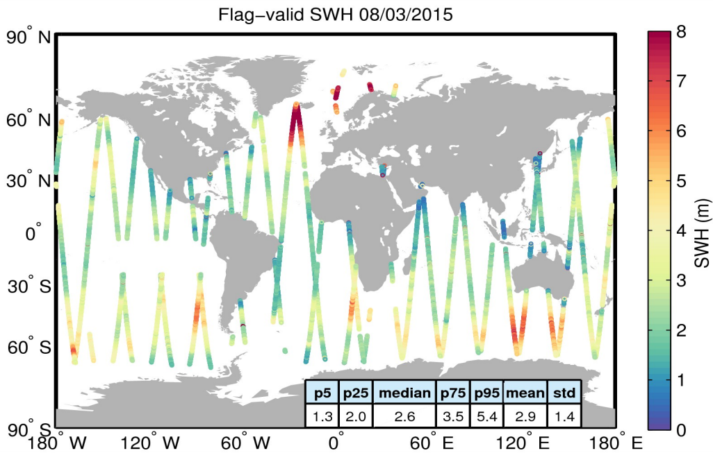
Figure 15. Geographical distribution of flag-valid SWH data over oceans and lakes for 08/03/2015. The statistical values shown in the table refer to the SWH in m and are calculated over all measurements shown in the figure.
