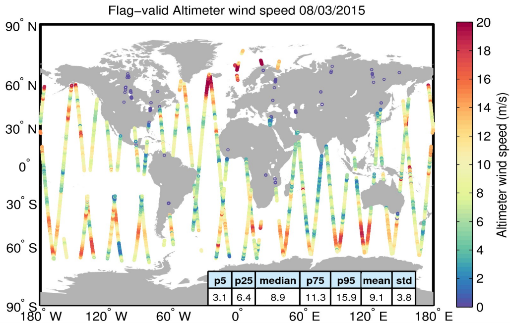
Figure 31. Geographical distribution of flag-valid wind data over oceans and lakes for 08/03/2015. The statistical values shown in the table refer to the wind in m/s and are calculated over all measurements shown in the figure.
