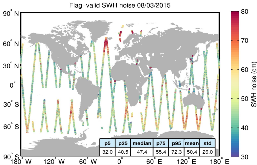
Figure 18. Geographical distribution of flag-valid 20-Hz SWH measurement noise over oceans and lakes for 08/03/2015. The statistical values shown in the figure refer to the SWH noise and are calculated over all measurements shown in the figure.
