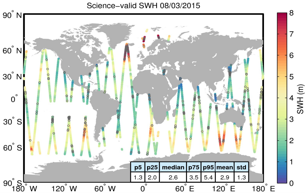
Figure 19. Geographical distribution of science-valid SWH data over oceans and lakes for 08/03/2015. The statistical values shown in the table refer to the SWH in m and are calculated over all measurements shown in the figure. Gray circles denote records that have been rejected based on the editing criteria described in Table 3.
