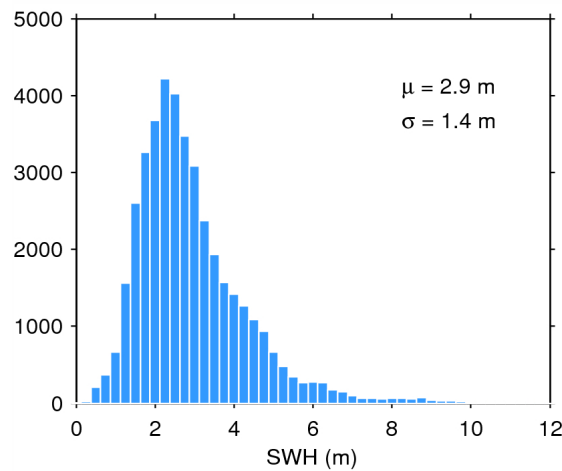
Figure 17. Histogram of flag-valid SWH over oceans and lakes for 08/03/2015. The mean ( \mu ) and standard deviation ( \sigma ) are also shown. Note that values larger than 12 m are excluded from the histogram for the sake of readability but not from the computation of \mu and \sigma .
