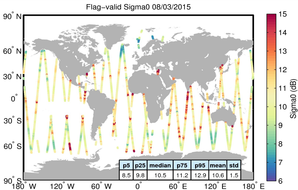
Figure 23. Geographical distribution of flag-valid sigma0 data over oceans and lakes for 08/03/2015. The statistical values shown in the table refer to the sigma0 in dB and are calculated over all measurements shown in the figure.
