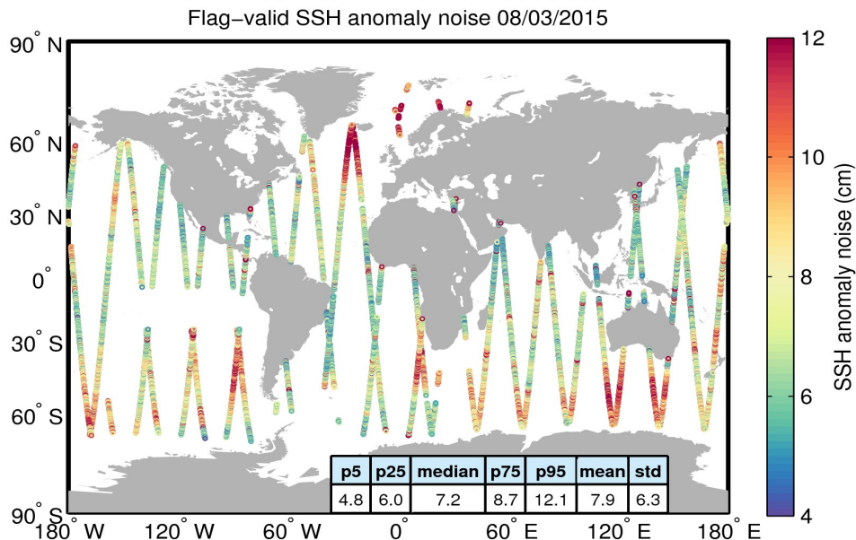
Figure 8. Geographical distribution of flag-valid 20-Hz SSH anomaly measurement noise over oceans and lakes for 08/03/2015. The statistical values shown in the table refer to the SSH anomaly noise and are calculated over all measurements shown in the figure.
