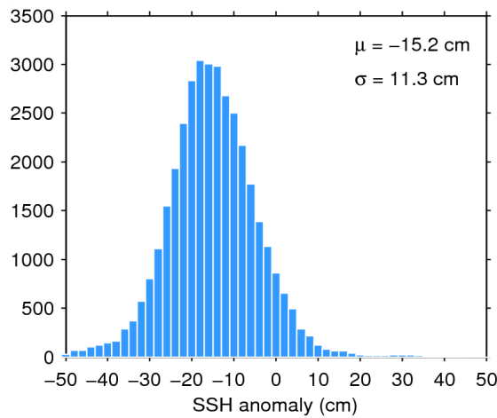
Figure 11. Histogram of science-valid SSH anomaly over oceans and lakes for 08/03/2015. The mean ( \mu ) and standard deviation ( \sigma ) are also shown. Note that values outside [-50 50] cm are excluded from the histogram for the sake of readability but not from the computation of \mu and \sigma .
