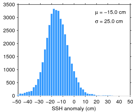
Figure 7. Histogram of flag-valid SSH anomaly over oceans and lakes for 08/03/2015. The mean ( \mu ) and standard deviation ( \sigma ) are also shown. Note that values outside [-50\ 50] cm are excluded from the histogram for the sake of readability but not from the computation of \mu and \sigma .
