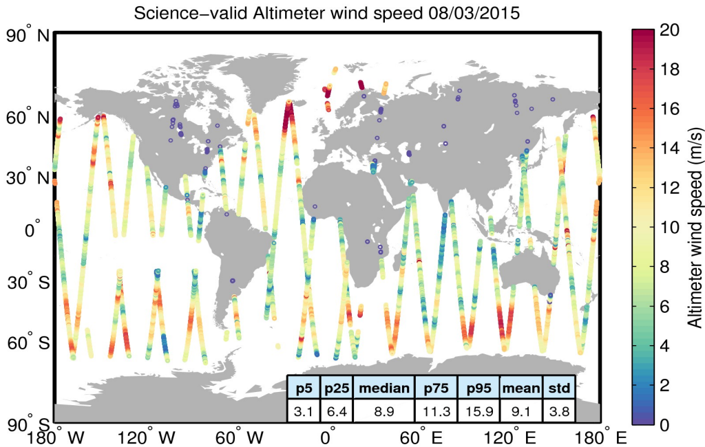
Figure 34. Geographical distribution of science-valid wind data over oceans and lakes for 08/03/2015. The statistical values shown in the table refer to the wind in m/s and are calculated over all measurements shown in the figure. Gray circles denote records that have been rejected based on the editing criteria described in Table 5.
