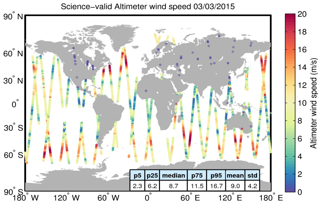
Figure 34. Geographical distribution of science-valid wind data over oceans and lakes for 03/03/2015. The statistical values shown in the table refer to the wind in m/s and are calculated over all measurements shown in the figure. Gray circles denote records that have been rejected based on the editing criteria described in Table 5.
