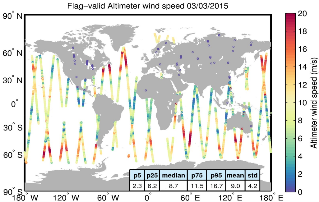
Figure 31. Geographical distribution of flag-valid wind data over oceans and lakes for 03/03/2015. The statistical values shown in the table refer to the wind in m/s and are calculated over all measurements shown in the figure.
