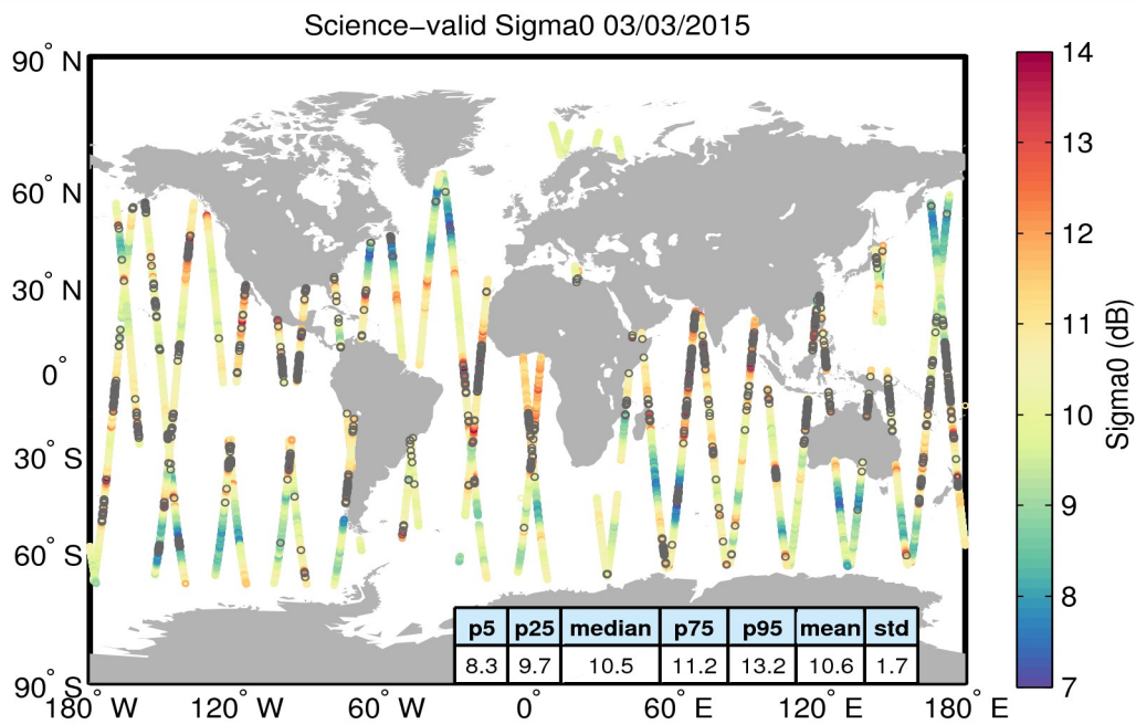
Figure 27. Geographical distribution of science-valid sigma0 data over oceans and lakes for 03/03/2015. The statistical values shown in the table refer to the sigma0 in dB and are calculated over all measurements shown in the figure. Gray circles denote records that have been rejected based on the editing criteria described in Table 4.
