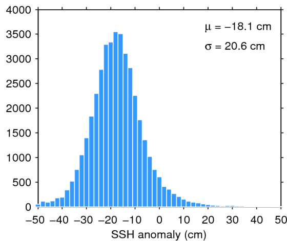
Figure 7. Histogram of flag-valid SSH anomaly over oceans and lakes for 03/03/2015. The mean ( \mu ) and standard deviation ( \sigma ) are also shown. Note that values outside [-50\ 50] cm are excluded from the histogram for the sake of readability but not from the computation of \mu and \sigma .
