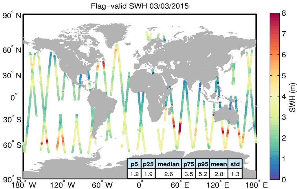
Figure 15. Geographical distribution of flag-valid SWH data over oceans and lakes for 03/03/2015. The statistical values shown in the figure refer to the SWH in m and are calculated over all measurements shown in the figure.
