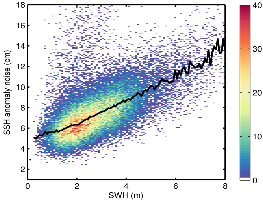
Figure 9. 2D histogram showing flag-valid SSH anomaly noise as a function of SWH for 03/03/2015. The black line denotes the median SSH anomaly as a function of SWH.
