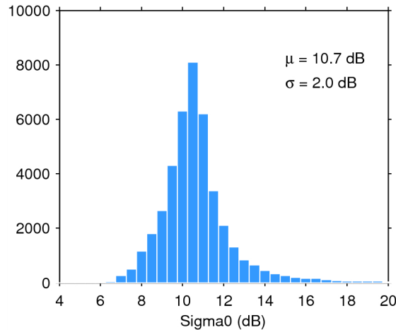
Figure 25. Histogram of flag-valid sigma0 over oceans and lakes for 03/03/2015. The mean ( \mu ) and standard deviation ( \sigma ) are also shown. Note that values outside [4 20] dB are excluded from the histogram for the sake of readability but not from the computation of \mu and \sigma .
