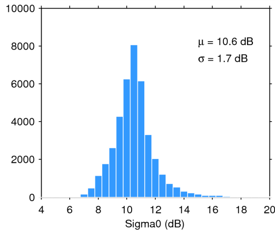
Figure 28. Histogram of science-valid sigma0 over oceans and lakes for 03/03/2015. The mean ( \mu ) and standard deviation ( \sigma ) are also shown. Note that values outside [4 20] dB are excluded from the histogram for the sake of readability but not from the computation of \mu and \sigma .
