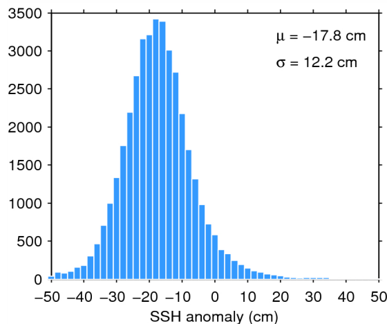
Figure 11. Histogram of science-valid SSH anomaly over oceans and lakes for 03/03/2015. The mean ( \mu ) and standard deviation ( \sigma ) are also shown. Note that values outside [-50 50] cm are excluded from the histogram for the sake of readability but not from the computation of \mu and \sigma .
