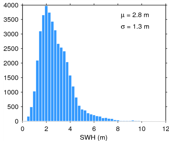
Figure 20. Histogram of science-valid SWH over oceans and lakes for 03/03/2015. The mean ( \mu ) and standard deviation ( \sigma ) are also shown. Note that values larger than 12 m are excluded from the histogram for the sake of readability but not from the computation of \mu and \sigma .
