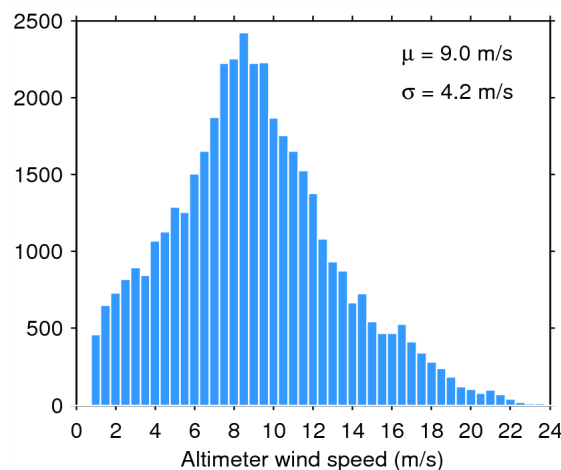
Figure 35. Histogram of science-valid wind over oceans and lakes for 03/03/2015. The mean ( \mu ) and standard deviation ( \sigma ) are also shown. Note that values larger than 24 m/s are excluded from the histogram for the sake of readability but not from the computation of \mu and \sigma .
