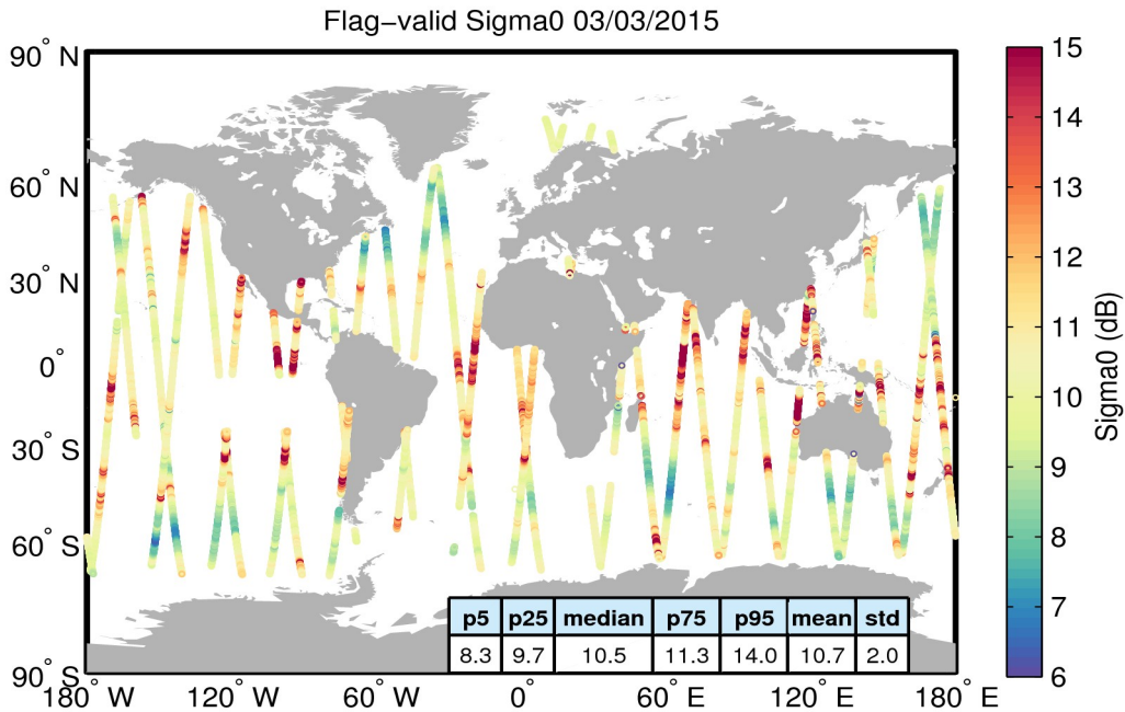
Figure 23. Geographical distribution of flag-valid sigma0 data over oceans and lakes for 03/03/2015. The statistical values shown in the table refer to the sigma0 in dB and are calculated over all measurements shown in the figure.
