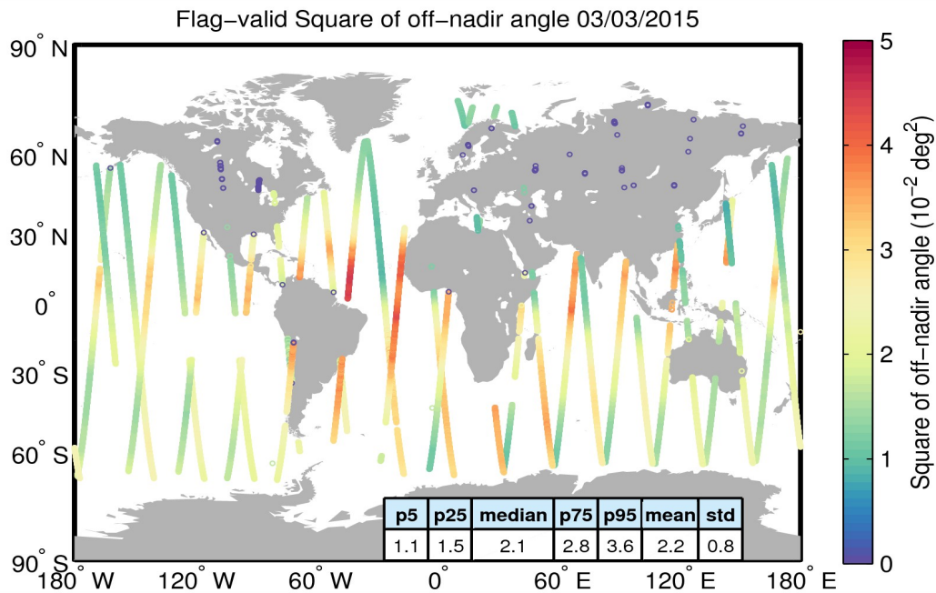
Figure 37. Geographical distribution of flag-valid mispointing data over oceans and lakes for 03/03/2015. The statistical values shown in the table refer to the mispointing in 10^{-2} \text{ deg}^2 and are calculated over all measurements shown in the figure.
