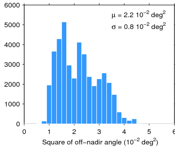
Figure 39. Histogram of flag-valid mispointing over oceans and lakes for 03/03/2015. The mean ( \mu ) and standard deviation ( \sigma ) are also shown. Note that values than 6 \cdot 10^{-2} \text{ deg}^2 are excluded from the histogram for the sake of readability but not from the computation of \mu and \sigma .
