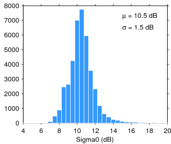
Figure 28. Histogram of science-valid sigma0 over oceans and lakes for 02/03/2015. The mean ( \mu ) and standard deviation ( \sigma ) are also shown. Note that values outside [4 20] dB are excluded from the histogram for the sake of readability but not from the computation of \mu and \sigma .
