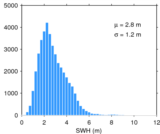
Figure 17. Histogram of flag-valid SWH over oceans and lakes for 02/03/2015. The mean ( \mu ) and standard deviation ( \sigma ) are also shown. Note that values larger than 12 m are excluded from the histogram for the sake of readability but not from the computation of \mu and \sigma .
