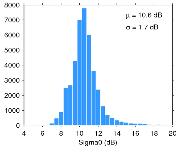
Figure 25. Histogram of flag-valid sigma0 over oceans and lakes for 02/03/2015. The mean ( \mu ) and standard deviation ( \sigma ) are also shown. Note that values outside [4 20] dB are excluded from the histogram for the sake of readability but not from the computation of \mu and \sigma .
