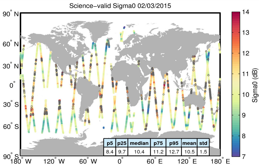
Figure 27. Geographical distribution of science-valid sigma0 data over oceans and lakes for 02/03/2015. The statistical values shown in the table refer to the sigma0 in dB and are calculated over all measurements shown in the figure. Gray circles denote records that have been rejected based on the editing criteria described in Table 4.
