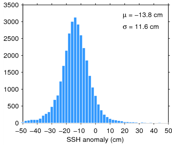
Figure 11. Histogram of science-valid SSH anomaly over oceans and lakes for 02/03/2015. The mean ( \mu ) and standard deviation ( \sigma ) are also shown. Note that values outside [-50 50] cm are excluded from the histogram for the sake of readability but not from the computation of \mu and \sigma .
