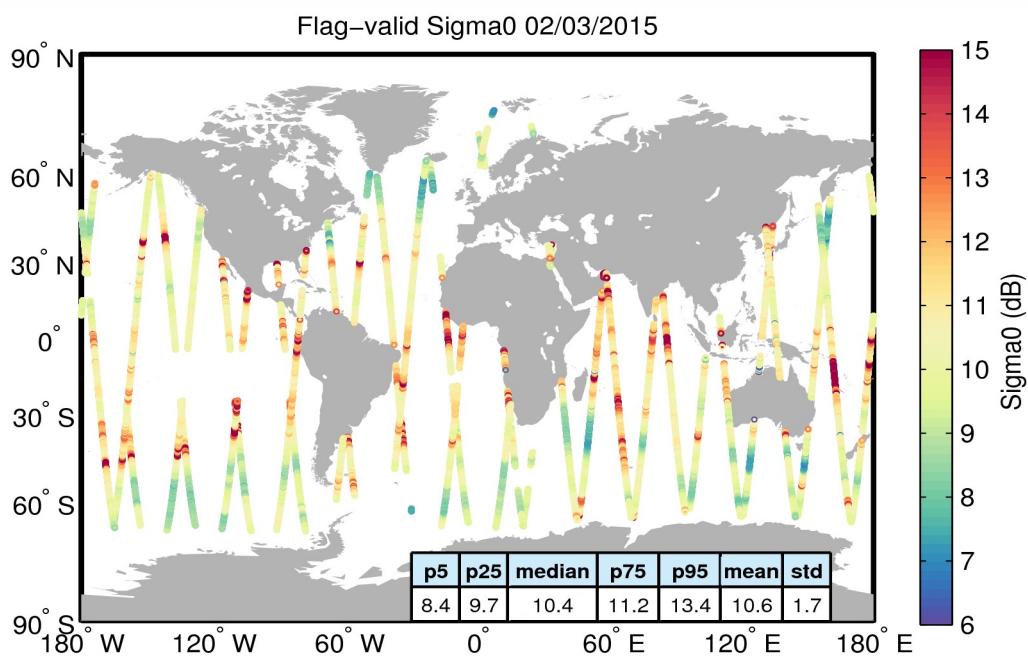
Figure 23. Geographical distribution of flag-valid sigma0 data over oceans and lakes for 02/03/2015. The statistical values shown in the table refer to the sigma0 in dB and are calculated over all measurements shown in the figure.
