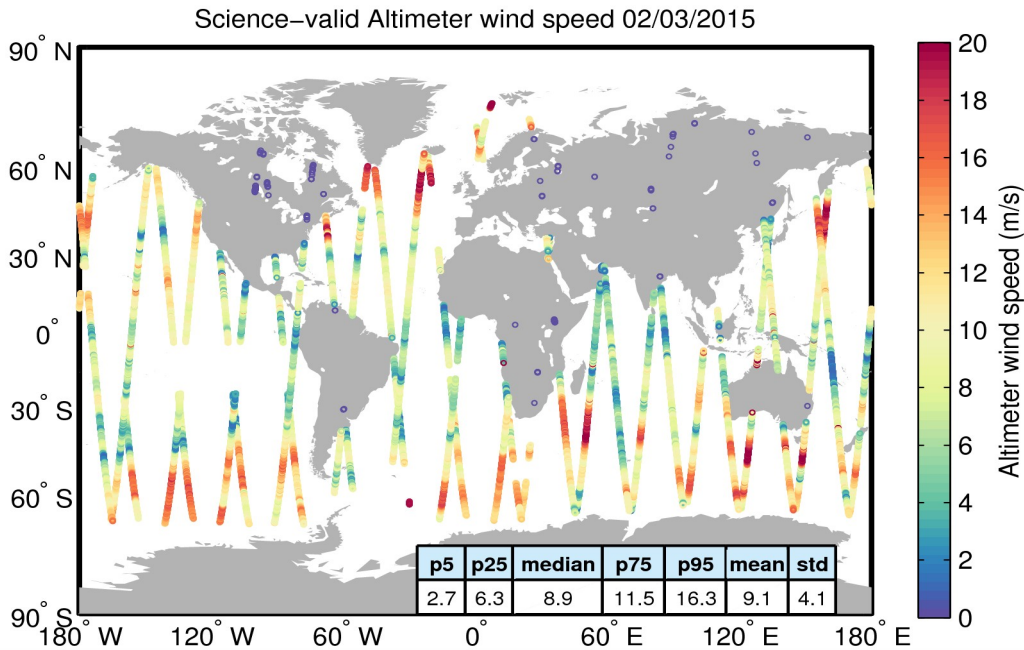
Figure 34. Geographical distribution of science-valid wind data over oceans and lakes for 02/03/2015. The statistical values shown in the table refer to the wind in m/s and are calculated over all measurements shown in the figure. Gray circles denote records that have been rejected based on the editing criteria described in Table 5.
