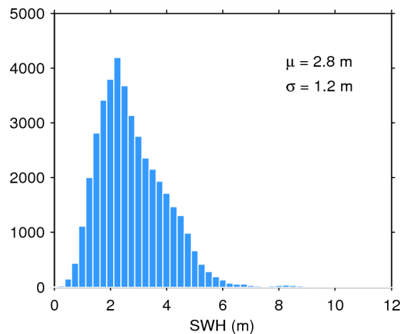
Figure 20. Histogram of science-valid SWH over oceans and lakes for 02/03/2015. The mean ( \mu ) and standard deviation ( \sigma ) are also shown. Note that values larger than 12 m are excluded from the histogram for the sake of readability but not from the computation of \mu and \sigma .
