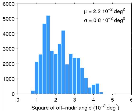
Figure 39. Histogram of flag-valid mispointing over oceans and lakes for 02/03/2015. The mean ( \mu ) and standard deviation ( \sigma ) are also shown. Note that values than 6 \cdot 10^{-2} \text{ deg}^2 are excluded from the histogram for the sake of readability but not from the computation of \mu and \sigma .
