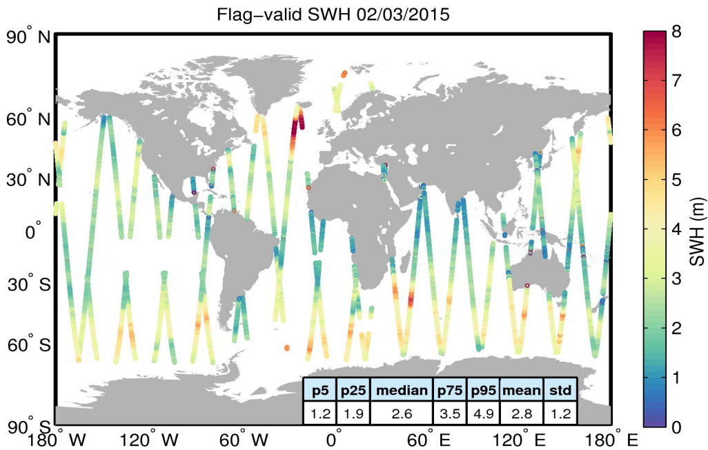
Figure 15. Geographical distribution of flag-valid SWH data over oceans and lakes for 02/03/2015. The statistical values shown in the table refer to the SWH in m and are calculated over all measurements shown in the figure.
