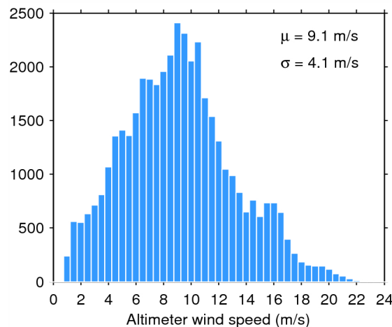
Figure 35. Histogram of science-valid wind over oceans and lakes for 02/03/2015. The mean ( \mu ) and standard deviation ( \sigma ) are also shown. Note that values larger than 24 m/s are excluded from the histogram for the sake of readability but not from the computation of \mu and \sigma .
