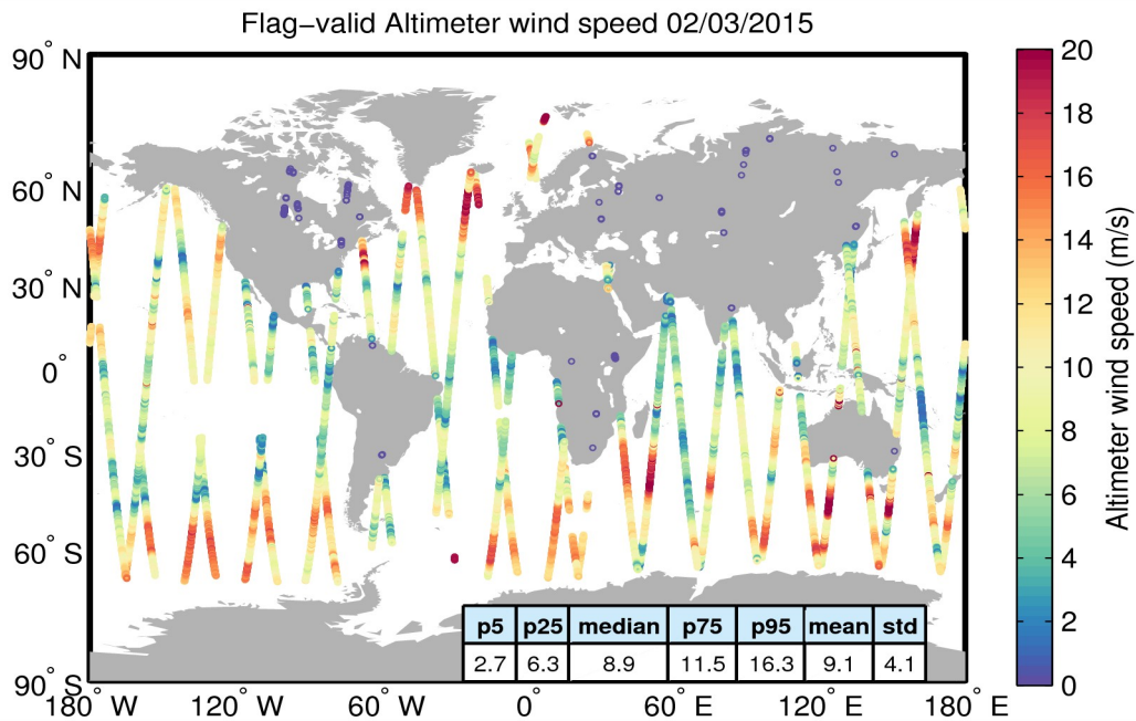
Figure 31. Geographical distribution of flag-valid wind data over oceans and lakes for 02/03/2015. The statistical values shown in the table refer to the wind in m/s and are calculated over all measurements shown in the figure.
