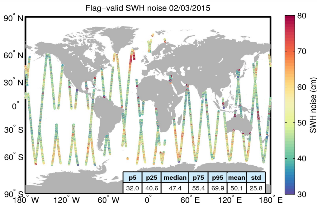
Figure 18. Geographical distribution of flag-valid 20-Hz SWH measurement noise over oceans and lakes for 02/03/2015. The statistical values shown in the figure refer to the SWH noise and are calculated over all measurements shown in the figure.
