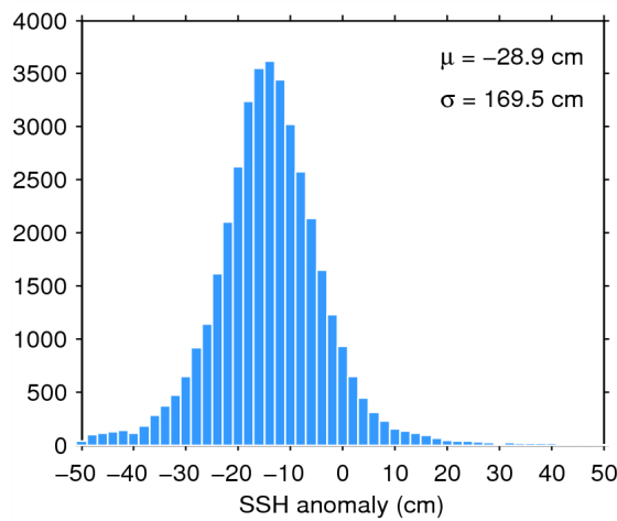
Figure 7. Histogram of flag-valid SSH anomaly over oceans and lakes for 02/03/2015. The mean ( \mu ) and standard deviation ( \sigma ) are also shown. Note that values outside [-50\ 50] cm are excluded from the histogram for the sake of readability but not from the computation of \mu and \sigma .
