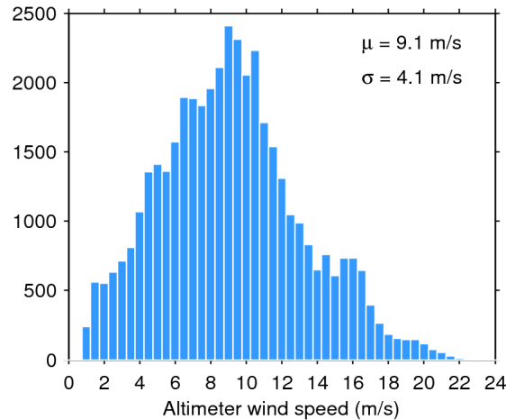
Figure 33. Histogram of flag-valid wind over oceans and lakes for 02/03/2015. The mean ( \mu ) and standard deviation ( \sigma ) are also shown. Note that values larger than 24 m/s are excluded from the histogram for the sake of readability but not from the computation of \mu and \sigma .
