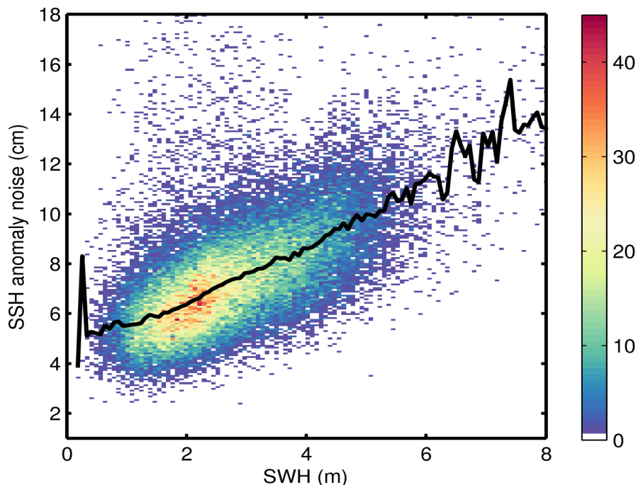
Figure 9. 2D histogram showing flag-valid SSH anomaly noise as a function of SWH for 02/03/2015. The black line denotes the median SSH anomaly as a function of SWH.
