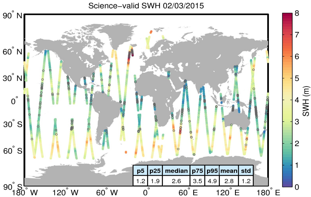
Figure 19. Geographical distribution of science-valid SWH data over oceans and lakes for 02/03/2015. The statistical values shown in the table refer to the SWH in m and are calculated over all measurements shown in the figure. Gray circles denote records that have been rejected based on the editing criteria described in Table 3.
