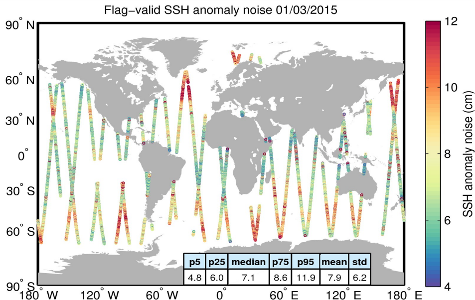
Figure 8. Geographical distribution of flag-valid 20-Hz SSH anomaly measurement noise over oceans and lakes for 01/03/2015. The statistical values shown in the table refer to the SSH anomaly noise and are calculated over all measurements shown in the figure.
