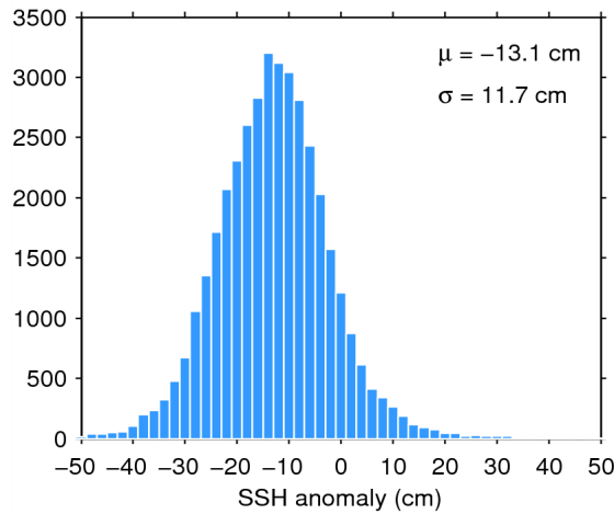
Figure 11. Histogram of science-valid SSH anomaly over oceans and lakes for 01/03/2015. The mean ( \mu ) and standard deviation ( \sigma ) are also shown. Note that values outside [-50 50] cm are excluded from the histogram for the sake of readability but not from the computation of \mu and \sigma .
