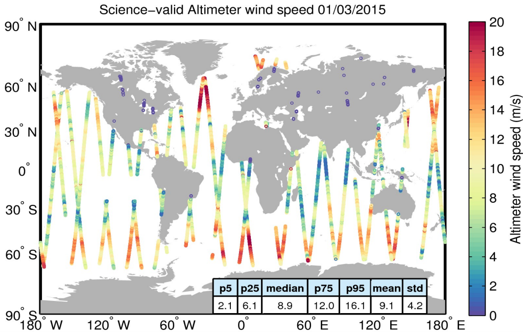
Figure 34. Geographical distribution of science-valid wind data over oceans and lakes for 01/03/2015. The statistical values shown in the table refer to the wind in m/s and are calculated over all measurements shown in the figure. Gray circles denote records that have been rejected based on the editing criteria described in Table 5.
