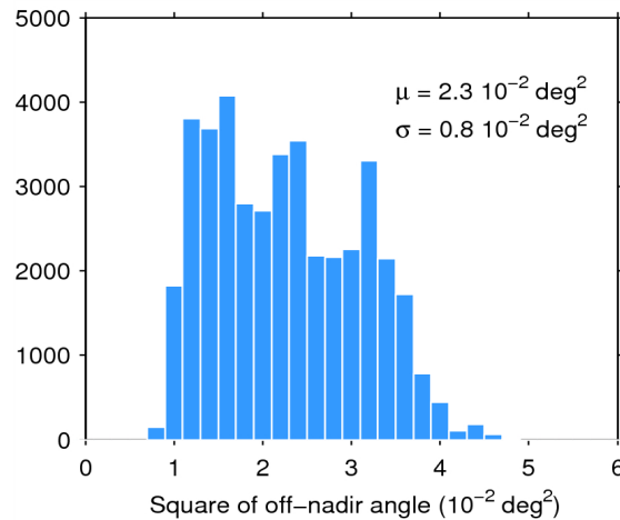
Figure 39. Histogram of flag-valid mispointing over oceans and lakes for 01/03/2015. The mean ( \mu ) and standard deviation ( \sigma ) are also shown. Note that values than 6 \cdot 10^{-2} \text{ deg}^2 are excluded from the histogram for the sake of readability but not from the computation of \mu and \sigma .
