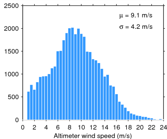
Figure 35. Histogram of science-valid wind over oceans and lakes for 01/03/2015. The mean ( \mu ) and standard deviation ( \sigma ) are also shown. Note that values larger than 24 m/s are excluded from the histogram for the sake of readability but not from the computation of \mu and \sigma .
