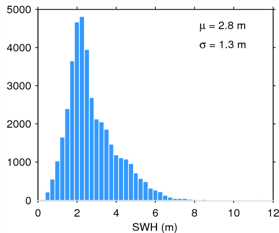
Figure 20. Histogram of science-valid SWH over oceans and lakes for 01/03/2015. The mean ( \mu ) and standard deviation ( \sigma ) are also shown. Note that values larger than 12 m are excluded from the histogram for the sake of readability but not from the computation of \mu and \sigma .
