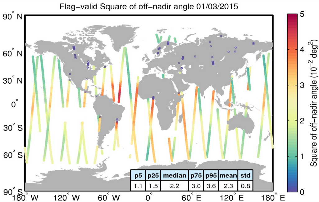
Figure 37. Geographical distribution of flag-valid mispointing data over oceans and lakes for 01/03/2015. The statistical values shown in the table refer to the mispointing in 10^{-2} \text{deg}^2 and are calculated over all measurements shown in the figure.
