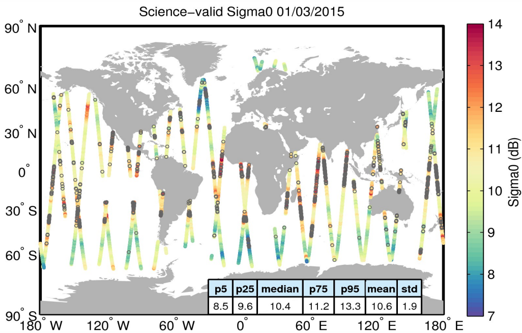
Figure 27. Geographical distribution of science-valid sigma0 data over oceans and lakes for 01/03/2015. The statistical values shown in the table refer to the sigma0 in dB and are calculated over all measurements shown in the figure. Gray circles denote records that have been rejected based on the editing criteria described in Table 4.
