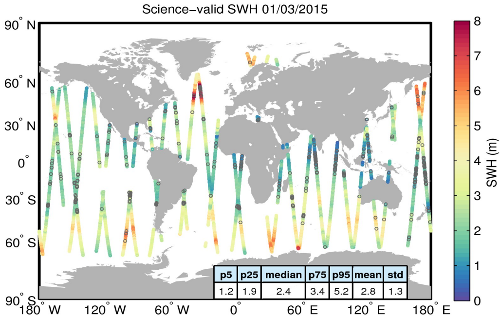
Figure 19. Geographical distribution of science-valid SWH data over oceans and lakes for 01/03/2015. The statistical values shown in the table refer to the SWH in m and are calculated over all measurements shown in the figure. Gray circles denote records that have been rejected based on the editing criteria described in Table 3.
