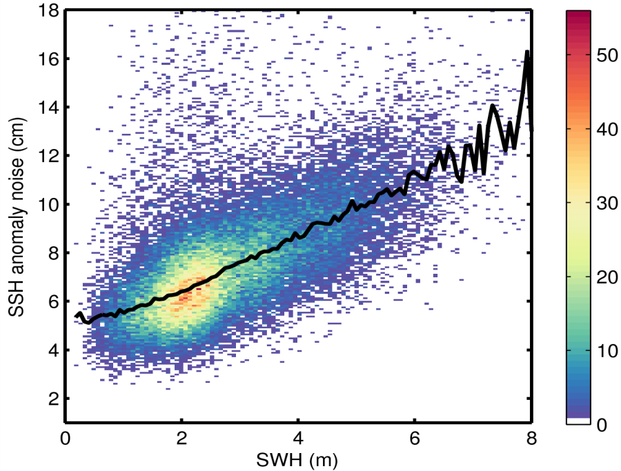
Figure 9. 2D histogram showing flag-valid SSH anomaly noise as a function of SWH for 01/03/2015. The black line denotes the median SSH anomaly as a function of SWH.
