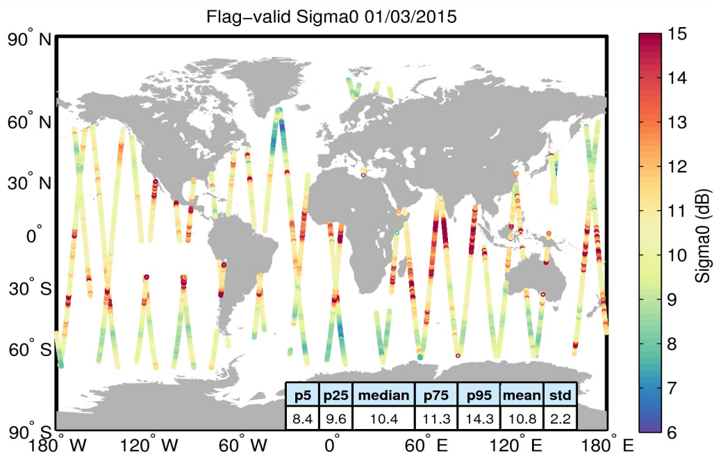
Figure 23. Geographical distribution of flag-valid sigma0 data over oceans and lakes for 01/03/2015. The statistical values shown in the table refer to the sigma0 in dB and are calculated over all measurements shown in the figure.
