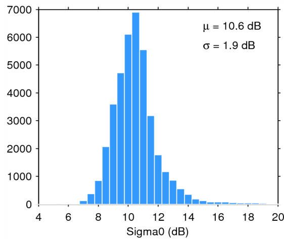
Figure 28. Histogram of science-valid sigma0 over oceans and lakes for 01/03/2015. The mean ( \mu ) and standard deviation ( \sigma ) are also shown. Note that values outside [4 20] dB are excluded from the histogram for the sake of readability but not from the computation of \mu and \sigma .
