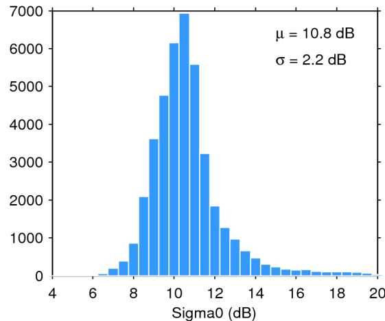
Figure 25. Histogram of flag-valid sigma0 over oceans and lakes for 01/03/2015. The mean ( \mu ) and standard deviation ( \sigma ) are also shown. Note that values outside [4 20] dB are excluded from the histogram for the sake of readability but not from the computation of \mu and \sigma .
