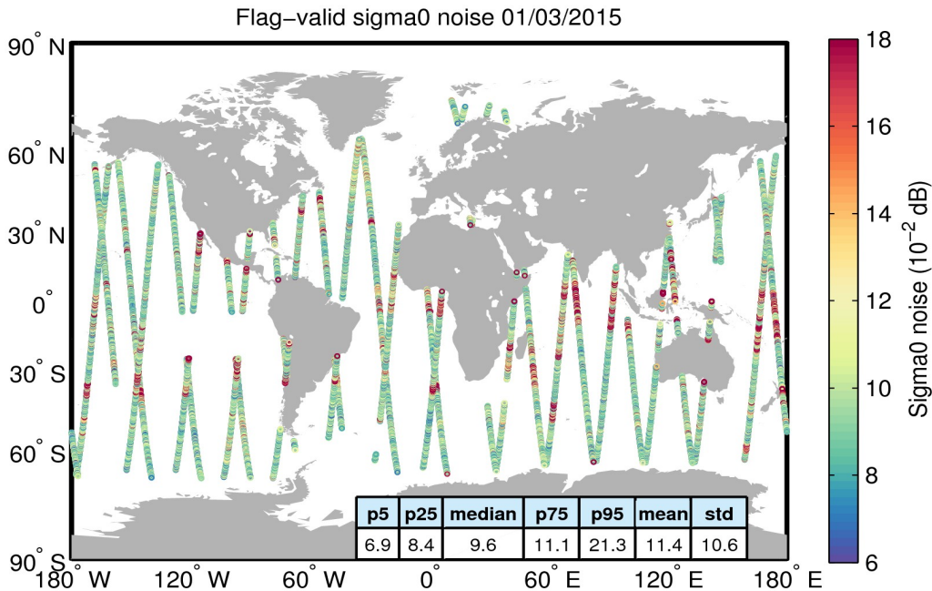
Figure 26. Geographical distribution of flag-valid 20-Hz sigma0 measurement noise over oceans and lakes for 01/03/2015. The statistical values shown in the table refer to the sigma0 noise and are calculated over all measurements shown in the figure.
