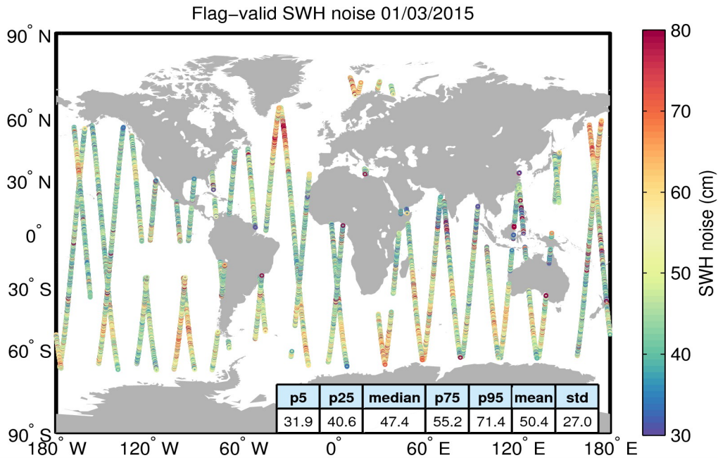
Figure 18. Geographical distribution of flag-valid 20-Hz SWH measurement noise over oceans and lakes for 01/03/2015. The statistical values shown in the figure refer to the SWH noise and are calculated over all measurements shown in the figure.
