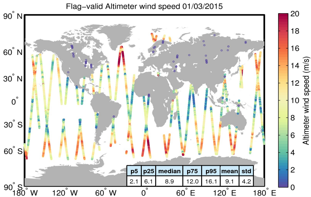
Figure 31. Geographical distribution of flag-valid wind data over oceans and lakes for 01/03/2015. The statistical values shown in the table refer to the wind in m/s and are calculated over all measurements shown in the figure.
