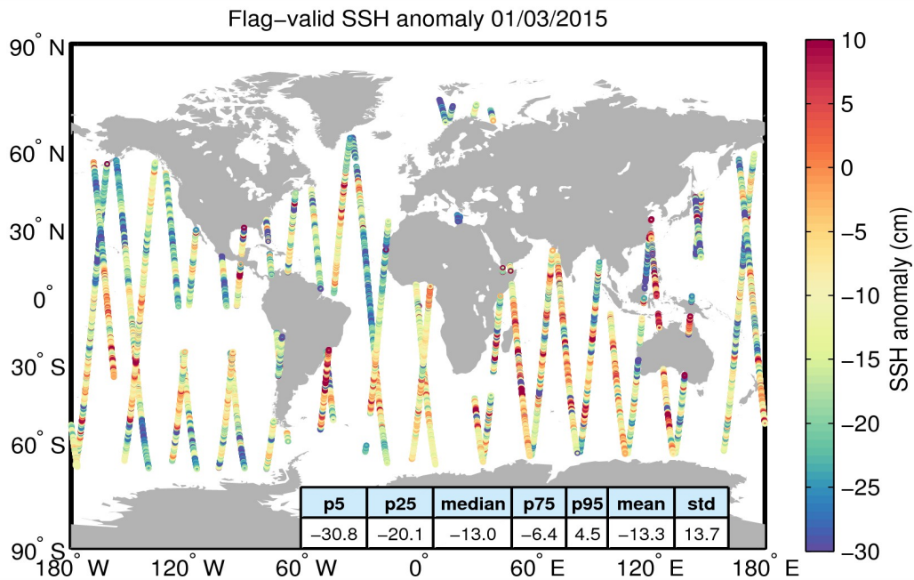
Figure 5. Geographical distribution of flag-valid 1-Hz SSH anomaly data over oceans and lakes for 01/03/2015. The statistical values shown in the table refer to the SSH anomaly in cm and are calculated over all measurements shown in the figure.
