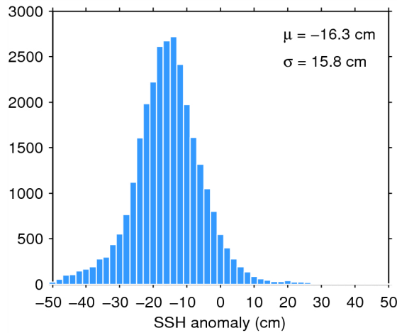
Figure 11. Histogram of science-valid SSH anomaly over oceans and lakes for 28/02/2015. The mean ( \mu ) and standard deviation ( \sigma ) are also shown. Note that values outside [-50 50] cm are excluded from the histogram for the sake of readability but not from the computation of \mu and \sigma .
