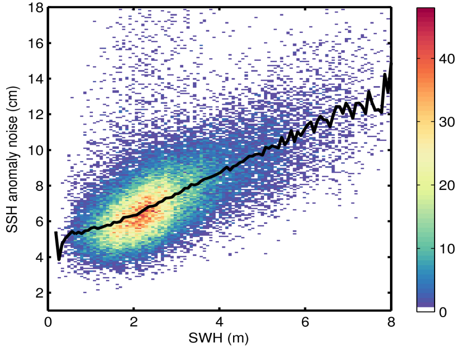
Figure 9. 2D histogram showing flag-valid SSH anomaly noise as a function of SWH for 28/02/2015. The black line denotes the median SSH anomaly as a function of SWH.
