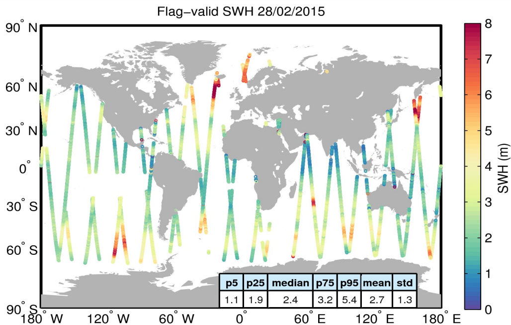
Figure 15. Geographical distribution of flag-valid SWH data over oceans and lakes for 28/02/2015. The statistical values shown in the table refer to the SWH in m and are calculated over all measurements shown in the figure.
