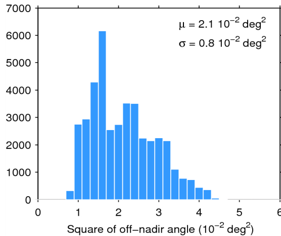
Figure 39. Histogram of flag-valid mispointing over oceans and lakes for 28/02/2015. The mean ( \mu ) and standard deviation ( \sigma ) are also shown. Note that values than 6 \cdot 10^{-2} \text{ deg}^2 are excluded from the histogram for the sake of readability but not from the computation of \mu and \sigma .
