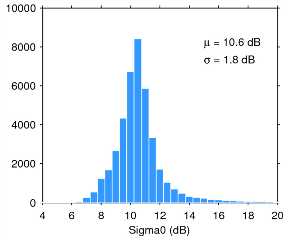
Figure 25. Histogram of flag-valid sigma0 over oceans and lakes for 28/02/2015. The mean ( \mu ) and standard deviation ( \sigma ) are also shown. Note that values outside [4 20] dB are excluded from the histogram for the sake of readability but not from the computation of \mu and \sigma .
