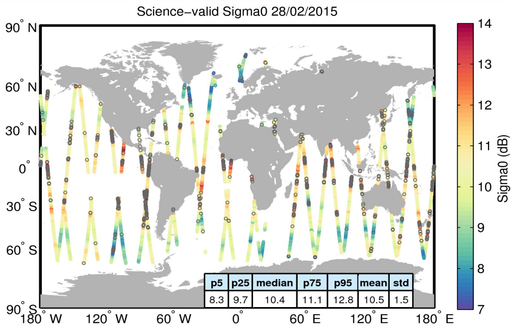
Figure 27. Geographical distribution of science-valid sigma0 data over oceans and lakes for 28/02/2015. The statistical values shown in the table refer to the sigma0 in dB and are calculated over all measurements shown in the figure. Gray circles denote records that have been rejected based on the editing criteria described in Table 4.
