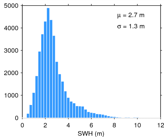
Figure 17. Histogram of flag-valid SWH over oceans and lakes for 28/02/2015. The mean ( \mu ) and standard deviation ( \sigma ) are also shown. Note that values larger than 12 m are excluded from the histogram for the sake of readability but not from the computation of \mu and \sigma .
