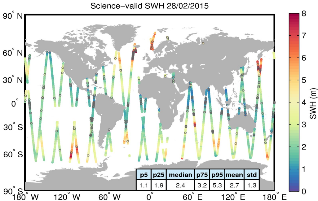
Figure 19. Geographical distribution of science-valid SWH data over oceans and lakes for 28/02/2015. The statistical values shown in the table refer to the SWH in m and are calculated over all measurements shown in the figure. Gray circles denote records that have been rejected based on the editing criteria described in Table 3.
