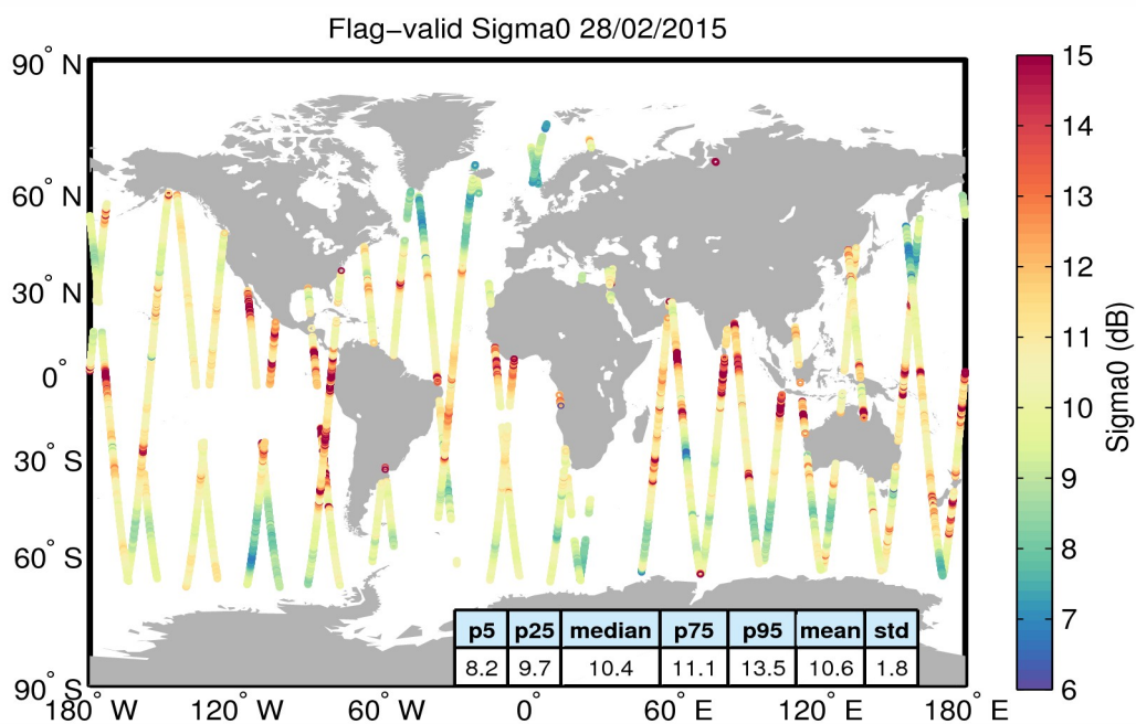
Figure 23. Geographical distribution of flag-valid sigma0 data over oceans and lakes for 28/02/2015. The statistical values shown in the table refer to the sigma0 in dB and are calculated over all measurements shown in the figure.
