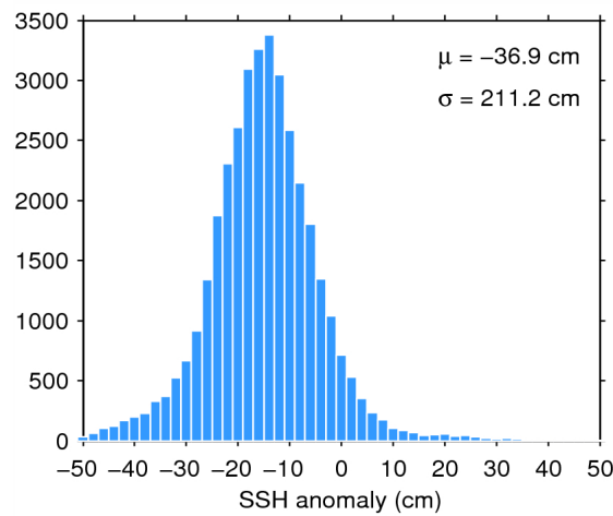
Figure 7. Histogram of flag-valid SSH anomaly over oceans and lakes for 28/02/2015. The mean ( \mu ) and standard deviation ( \sigma ) are also shown. Note that values outside [-50\ 50] cm are excluded from the histogram for the sake of readability but not from the computation of \mu and \sigma .
