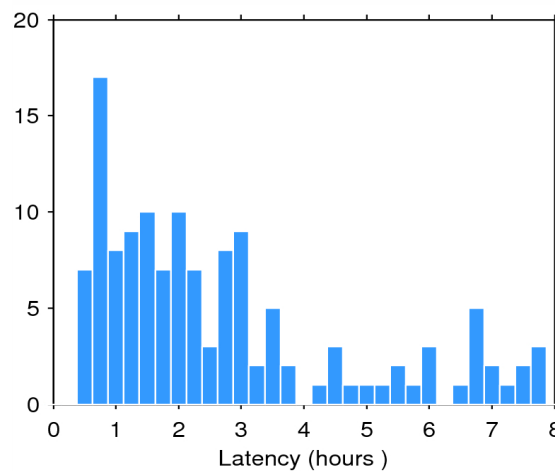
Figure 2. Histogram of the data latency for 28/02/2015. The y-axis denotes the number of files that are made available with a delay of x-hours with respect to the mean time of the records stored in the file.
