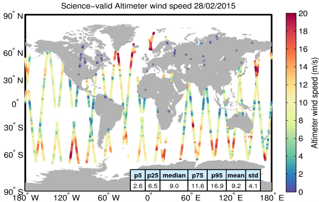
Figure 34. Geographical distribution of science-valid wind data over oceans and lakes for 28/02/2015. The statistical values shown in the table refer to the wind in m/s and are calculated over all measurements shown in the figure. Gray circles denote records that have been rejected based on the editing criteria described in Table 5.
