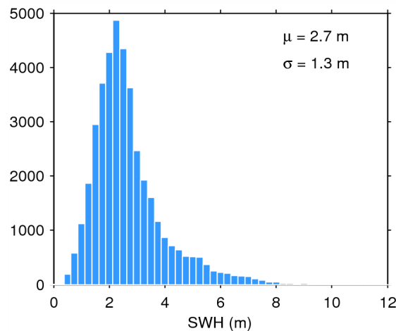
Figure 20. Histogram of science-valid SWH over oceans and lakes for 28/02/2015. The mean ( \mu ) and standard deviation ( \sigma ) are also shown. Note that values larger than 12 m are excluded from the histogram for the sake of readability but not from the computation of \mu and \sigma .
