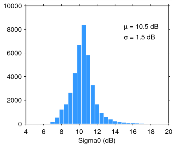
Figure 28. Histogram of science-valid sigma0 over oceans and lakes for 28/02/2015. The mean ( \mu ) and standard deviation ( \sigma ) are also shown. Note that values outside [4 20] dB are excluded from the histogram for the sake of readability but not from the computation of \mu and \sigma .
