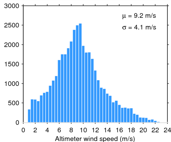
Figure 35. Histogram of science-valid wind over oceans and lakes for 28/02/2015. The mean ( \mu ) and standard deviation ( \sigma ) are also shown. Note that values larger than 24 m/s are excluded from the histogram for the sake of readability but not from the computation of \mu and \sigma .
