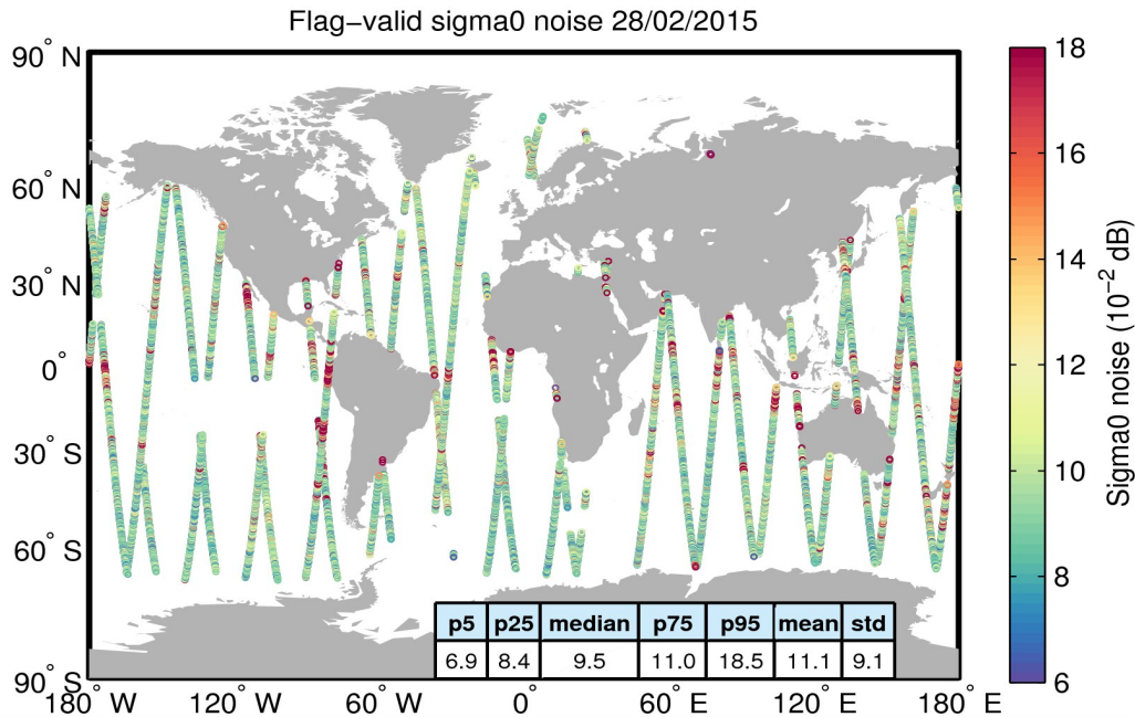
Figure 26. Geographical distribution of flag-valid 20-Hz sigma0 measurement noise over oceans and lakes for 28/02/2015. The statistical values shown in the table refer to the sigma0 noise and are calculated over all measurements shown in the figure.
