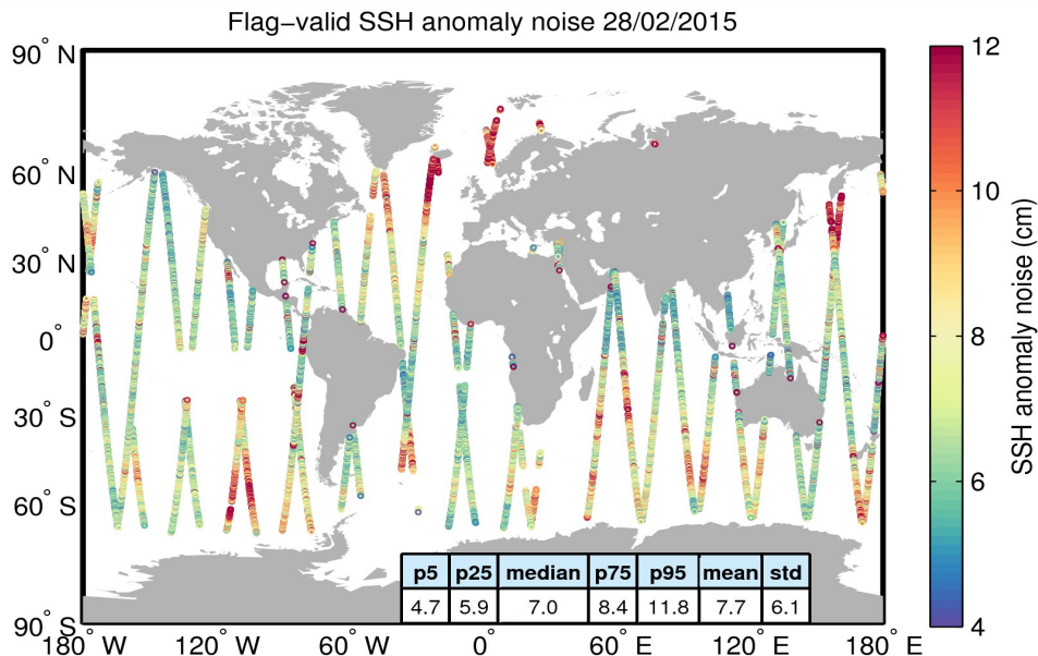
Figure 8. Geographical distribution of flag-valid 20-Hz SSH anomaly measurement noise over oceans and lakes for 28/02/2015. The statistical values shown in the table refer to the SSH anomaly noise and are calculated over all measurements shown in the figure.
