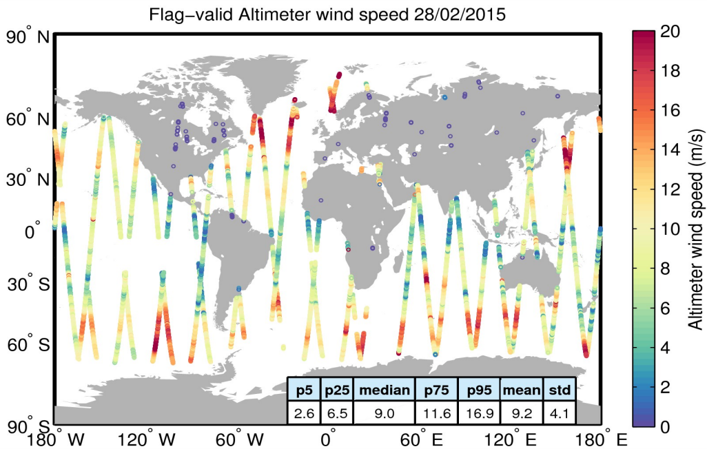
Figure 31. Geographical distribution of flag-valid wind data over oceans and lakes for 28/02/2015. The statistical values shown in the table refer to the wind in m/s and are calculated over all measurements shown in the figure.
