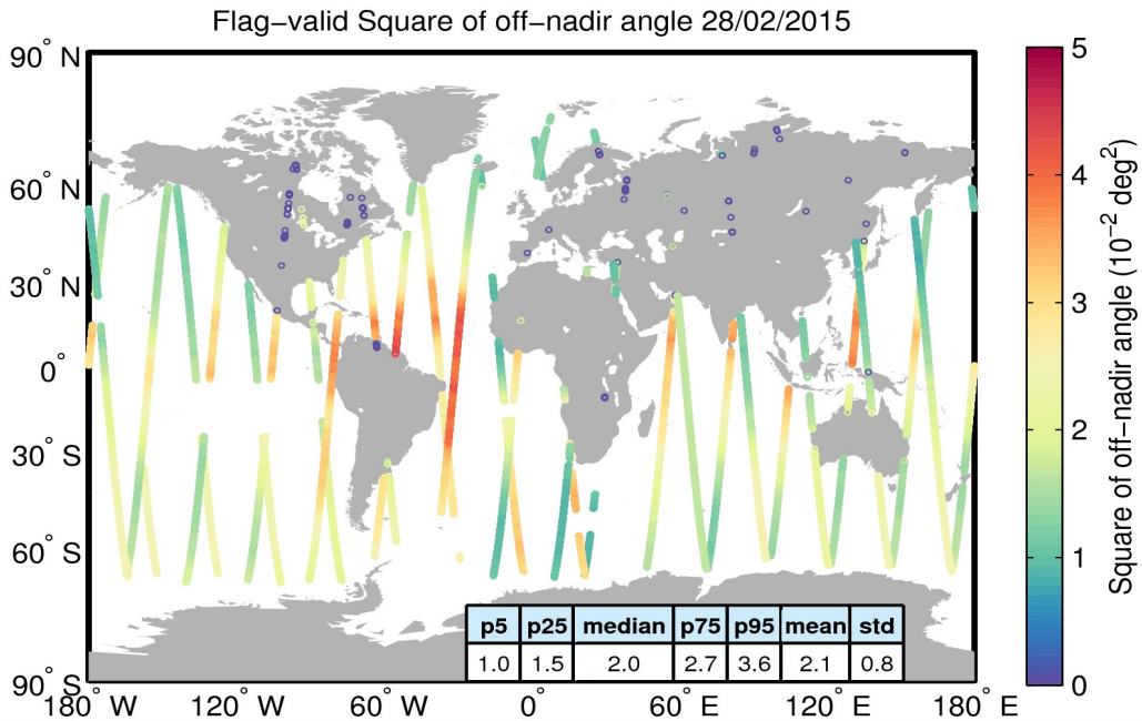
Figure 37. Geographical distribution of flag-valid mispointing data over oceans and lakes for 28/02/2015. The statistical values shown in the table refer to the mispointing in 10^{-2} \text{ deg}^2 and are calculated over all measurements shown in the figure.
