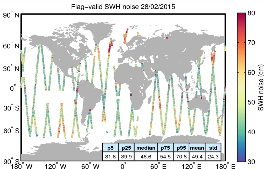
Figure 18. Geographical distribution of flag-valid 20-Hz SWH measurement noise over oceans and lakes for 28/02/2015. The statistical values shown in the figure refer to the SWH noise and are calculated over all measurements shown in the figure.
