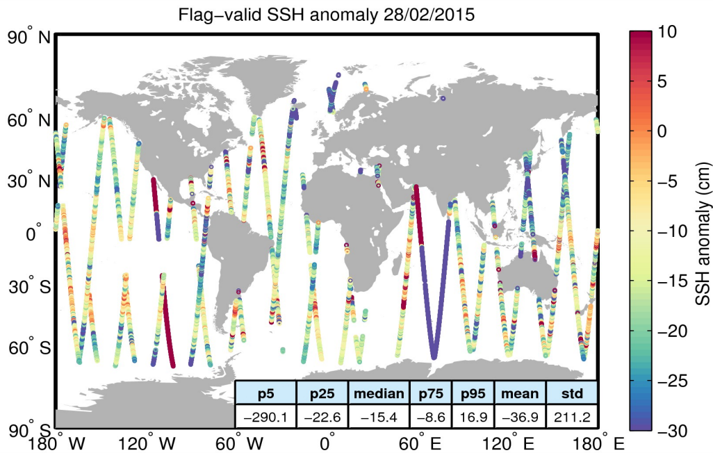
Figure 5. Geographical distribution of flag-valid 1-Hz SSH anomaly data over oceans and lakes for 28/02/2015. The statistical values shown in the table refer to the SSH anomaly in cm and are calculated over all measurements shown in the figure.
