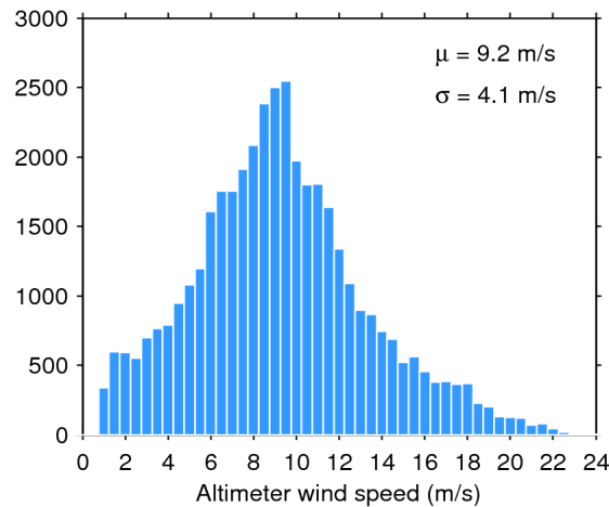
Figure 33. Histogram of flag-valid wind over oceans and lakes for 28/02/2015. The mean ( \mu ) and standard deviation ( \sigma ) are also shown. Note that values larger than 24 m/s are excluded from the histogram for the sake of readability but not from the computation of \mu and \sigma .
