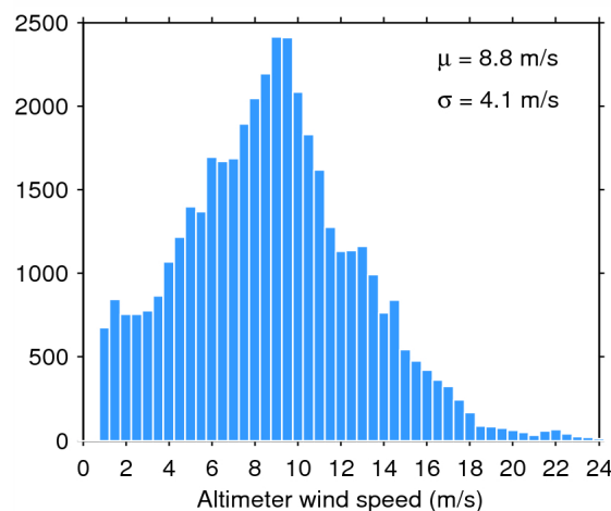
Figure 35. Histogram of science-valid wind over oceans and lakes for 27/02/2015. The mean ( \mu ) and standard deviation ( \sigma ) are also shown. Note that values larger than 24 m/s are excluded from the histogram for the sake of readability but not from the computation of \mu and \sigma .
