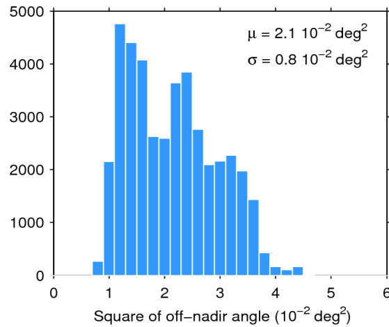
Figure 39. Histogram of flag-valid mispointing over oceans and lakes for 27/02/2015. The mean ( \mu ) and standard deviation ( \sigma ) are also shown. Note that values than 6 \cdot 10^{-2} \text{ deg}^2 are excluded from the histogram for the sake of readability but not from the computation of \mu and \sigma .
