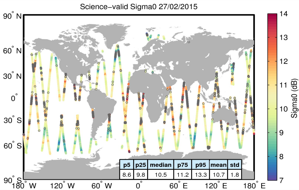
Figure 27. Geographical distribution of science-valid sigma0 data over oceans and lakes for 27/02/2015. The statistical values shown in the table refer to the sigma0 in dB and are calculated over all measurements shown in the figure. Gray circles denote records that have been rejected based on the editing criteria described in Table 4.
