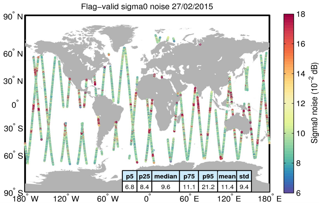
Figure 26. Geographical distribution of flag-valid 20-Hz sigma0 measurement noise over oceans and lakes for 27/02/2015. The statistical values shown in the table refer to the sigma0 noise and are calculated over all measurements shown in the figure.
