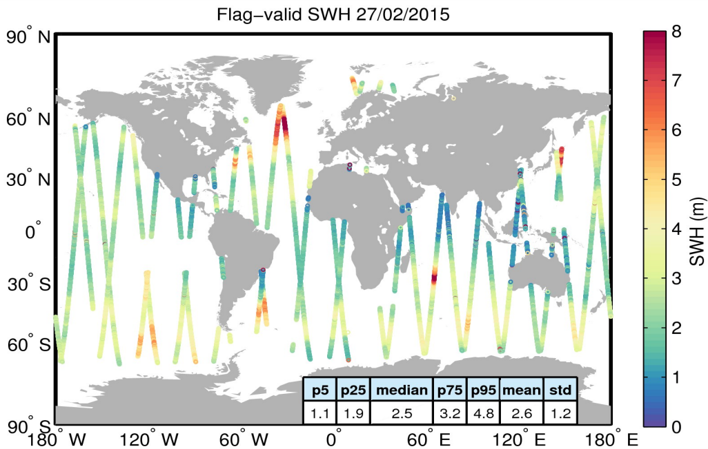
Figure 15. Geographical distribution of flag-valid SWH data over oceans and lakes for 27/02/2015. The statistical values shown in the table refer to the SWH in m and are calculated over all measurements shown in the figure.
