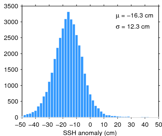
Figure 11. Histogram of science-valid SSH anomaly over oceans and lakes for 27/02/2015. The mean ( \mu ) and standard deviation ( \sigma ) are also shown. Note that values outside [-50 50] cm are excluded from the histogram for the sake of readability but not from the computation of \mu and \sigma .
