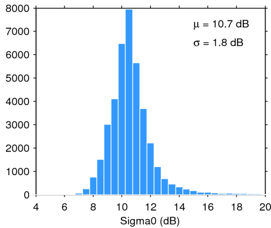
Figure 28. Histogram of science-valid sigma0 over oceans and lakes for 27/02/2015. The mean ( \mu ) and standard deviation ( \sigma ) are also shown. Note that values outside [4 20] dB are excluded from the histogram for the sake of readability but not from the computation of \mu and \sigma .
