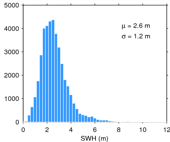
Figure 20. Histogram of science-valid SWH over oceans and lakes for 27/02/2015. The mean ( \mu ) and standard deviation ( \sigma ) are also shown. Note that values larger than 12 m are excluded from the histogram for the sake of readability but not from the computation of \mu and \sigma .
