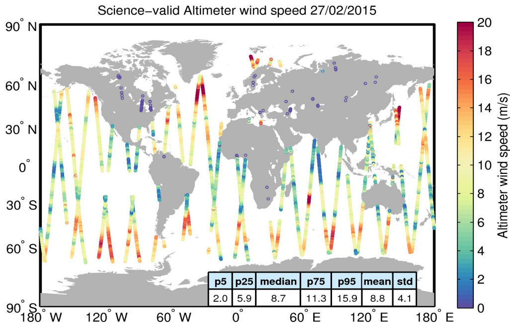
Figure 34. Geographical distribution of science-valid wind data over oceans and lakes for 27/02/2015. The statistical values shown in the table refer to the wind in m/s and are calculated over all measurements shown in the figure. Gray circles denote records that have been rejected based on the editing criteria described in Table 5.
