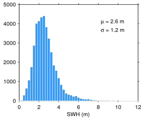
Figure 17. Histogram of flag-valid SWH over oceans and lakes for 27/02/2015. The mean ( \mu ) and standard deviation ( \sigma ) are also shown. Note that values larger than 12 m are excluded from the histogram for the sake of readability but not from the computation of \mu and \sigma .
