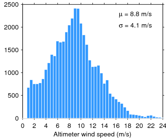
Figure 33. Histogram of flag-valid wind over oceans and lakes for 27/02/2015. The mean ( \mu ) and standard deviation ( \sigma ) are also shown. Note that values larger than 24 m/s are excluded from the histogram for the sake of readability but not from the computation of \mu and \sigma .
