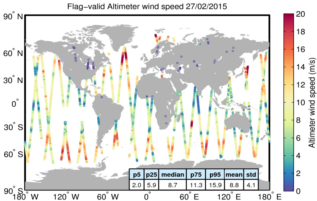
Figure 31. Geographical distribution of flag-valid wind data over oceans and lakes for 27/02/2015. The statistical values shown in the table refer to the wind in m/s and are calculated over all measurements shown in the figure.
