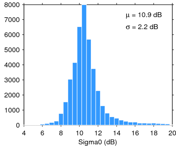
Figure 25. Histogram of flag-valid sigma0 over oceans and lakes for 27/02/2015. The mean ( \mu ) and standard deviation ( \sigma ) are also shown. Note that values outside [4 20] dB are excluded from the histogram for the sake of readability but not from the computation of \mu and \sigma .
