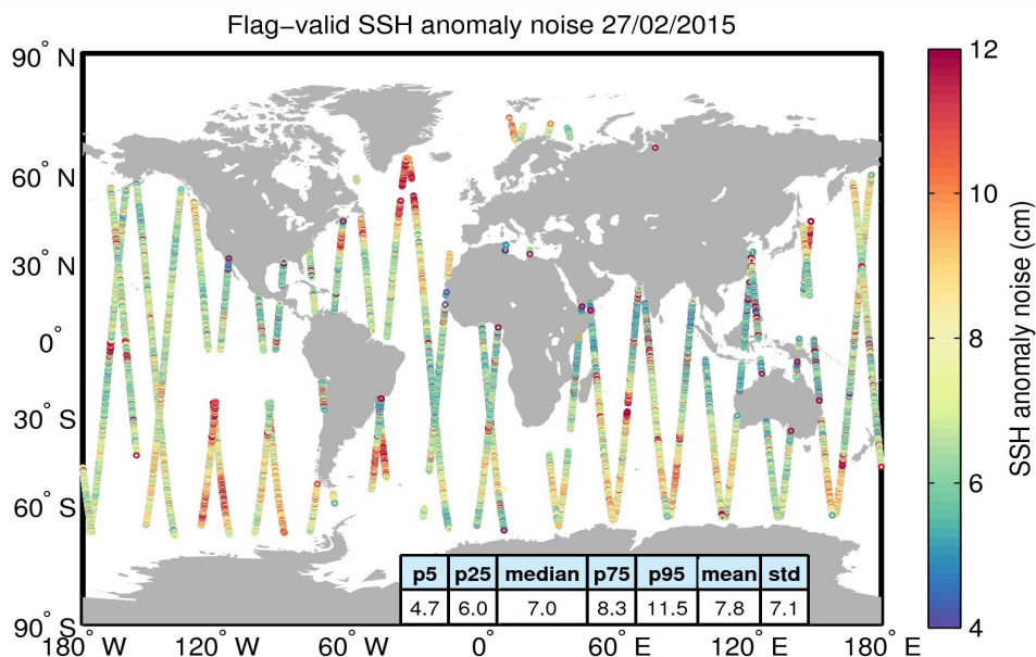
Figure 8. Geographical distribution of flag-valid 20-Hz SSH anomaly measurement noise over oceans and lakes for 27/02/2015. The statistical values shown in the table refer to the SSH anomaly noise and are calculated over all measurements shown in the figure.
