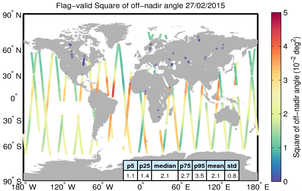
Figure 37. Geographical distribution of flag-valid mispointing data over oceans and lakes for 27/02/2015. The statistical values shown in the table refer to the mispointing in 10^{-2} \text{ deg}^2 and are calculated over all measurements shown in the figure.
