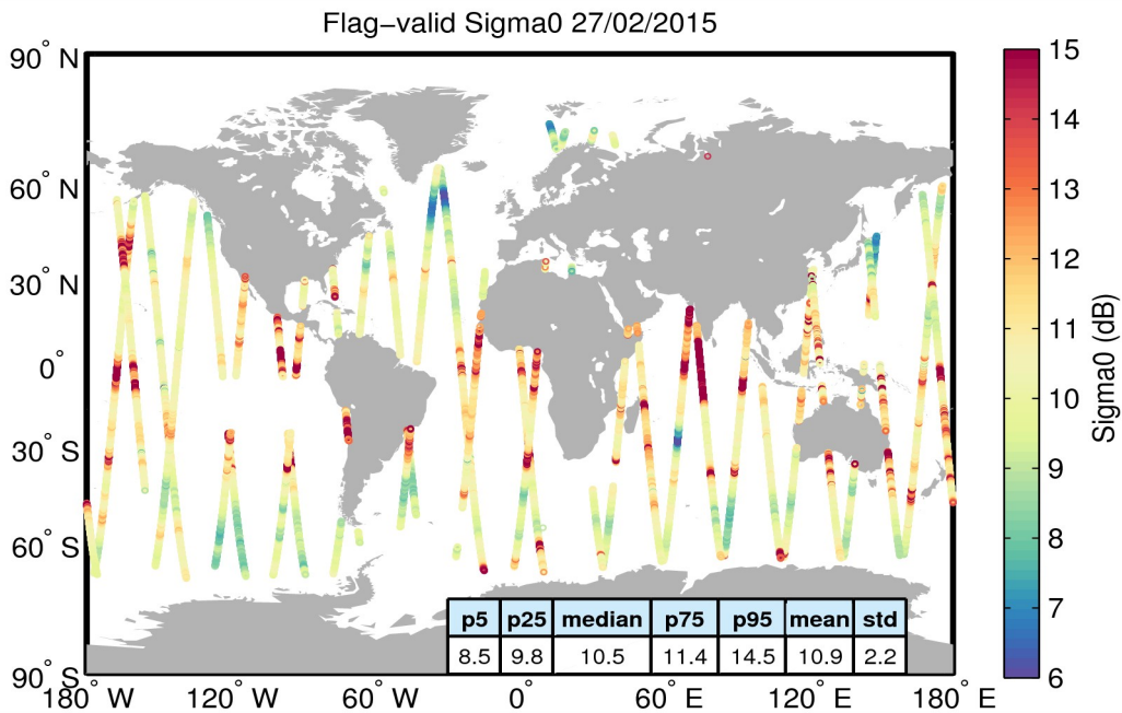
Figure 23. Geographical distribution of flag-valid sigma0 data over oceans and lakes for 27/02/2015. The statistical values shown in the table refer to the sigma0 in dB and are calculated over all measurements shown in the figure.
